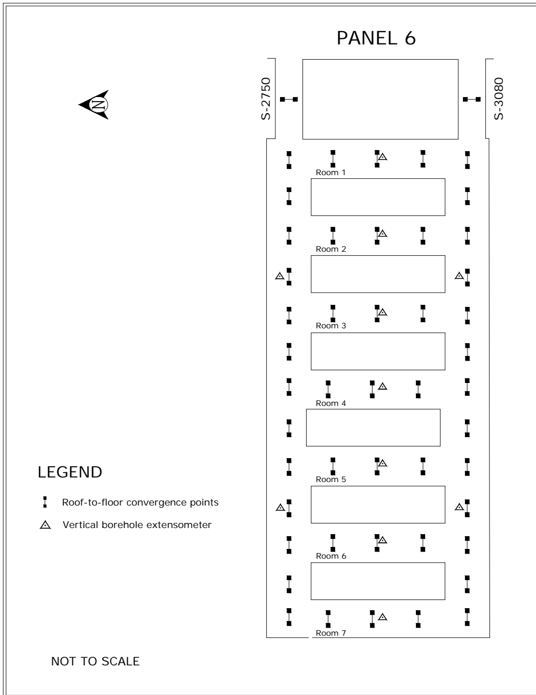
Figure 6-4 – Location of Panel 6 Geotechnical Instruments
