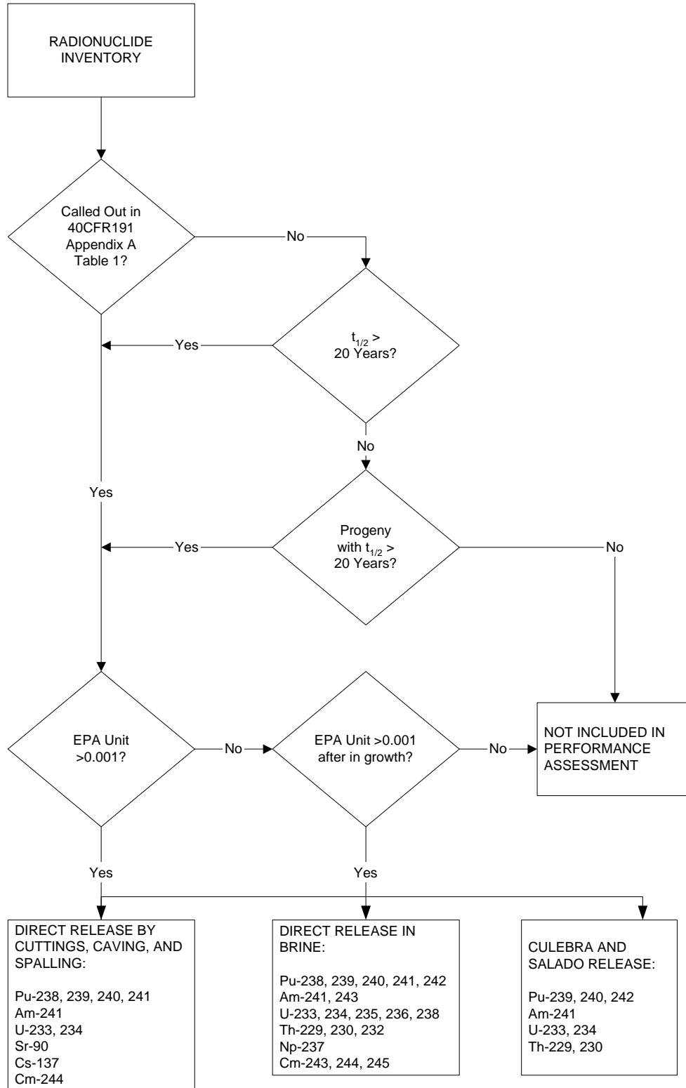
1 2 Figure TRU WASTE-5. Flow Diagram for Selecting Radionuclides for the Release 3 Pathways Conceptualized by Performance Assessment (The top part of the diagram 4 describes the criteria for selecting radionuclides in Table TRU WASTE-9)
