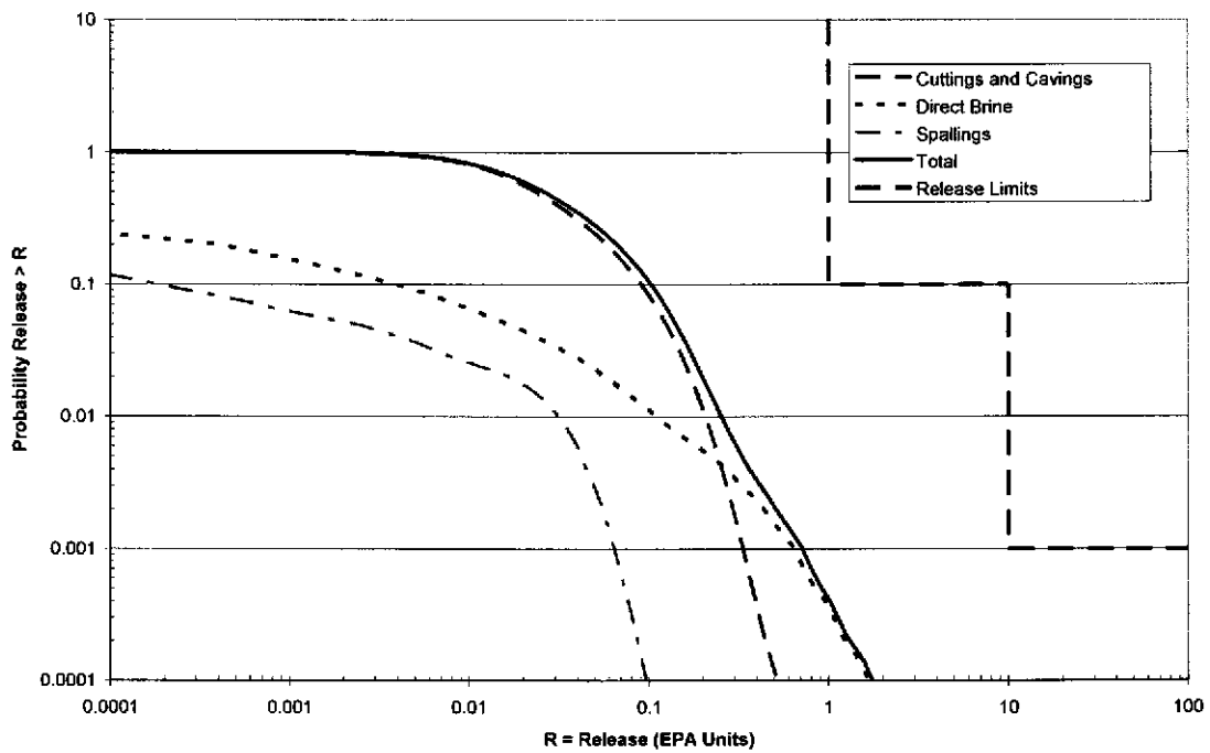
Figure 4. 6. Mean CCDFs for Components of Total Normalized Releases: Replicate 1 of CRA-2009 PA
