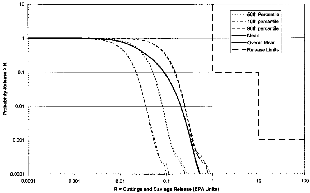
Figure 4.17. Mean and Percentile CCDFs for Cuttings and Cavings Normalized Releases: All Replicates of the CRA-2009 PA
