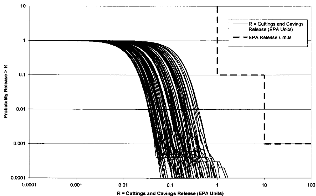
Figure 4.14. Cuttings and Cavings Normalized Releases: Replicate 2 of the CRA-2009 PA
