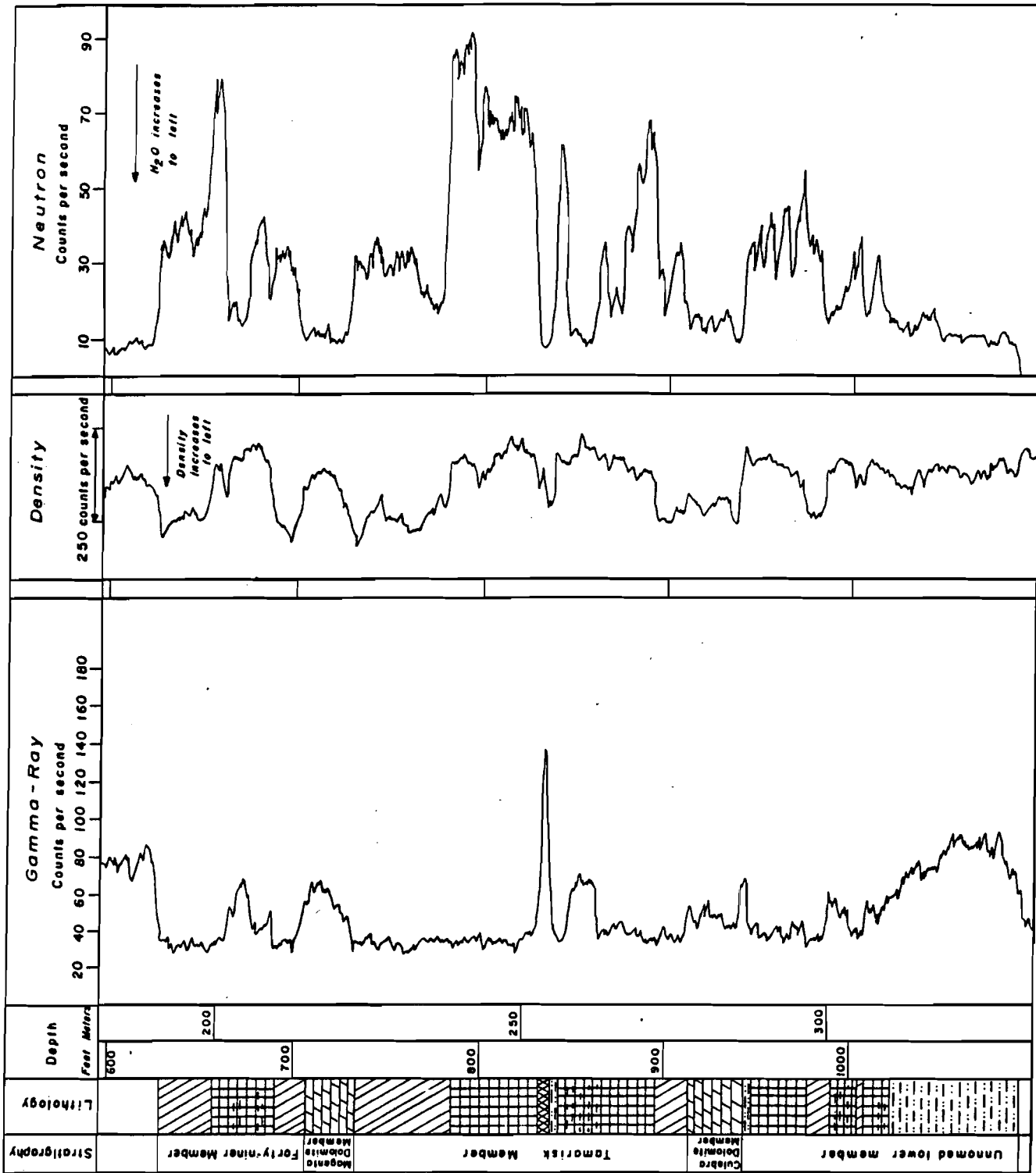
Figure 3.--Comparison of lithologic and geophysical logs in the Rustler Formation, drill hole P-18. (Logs from U.S. Geological Survey, Water Resources Division, published in Jones, 1978; see figure 2 for explanation of symbols.)
