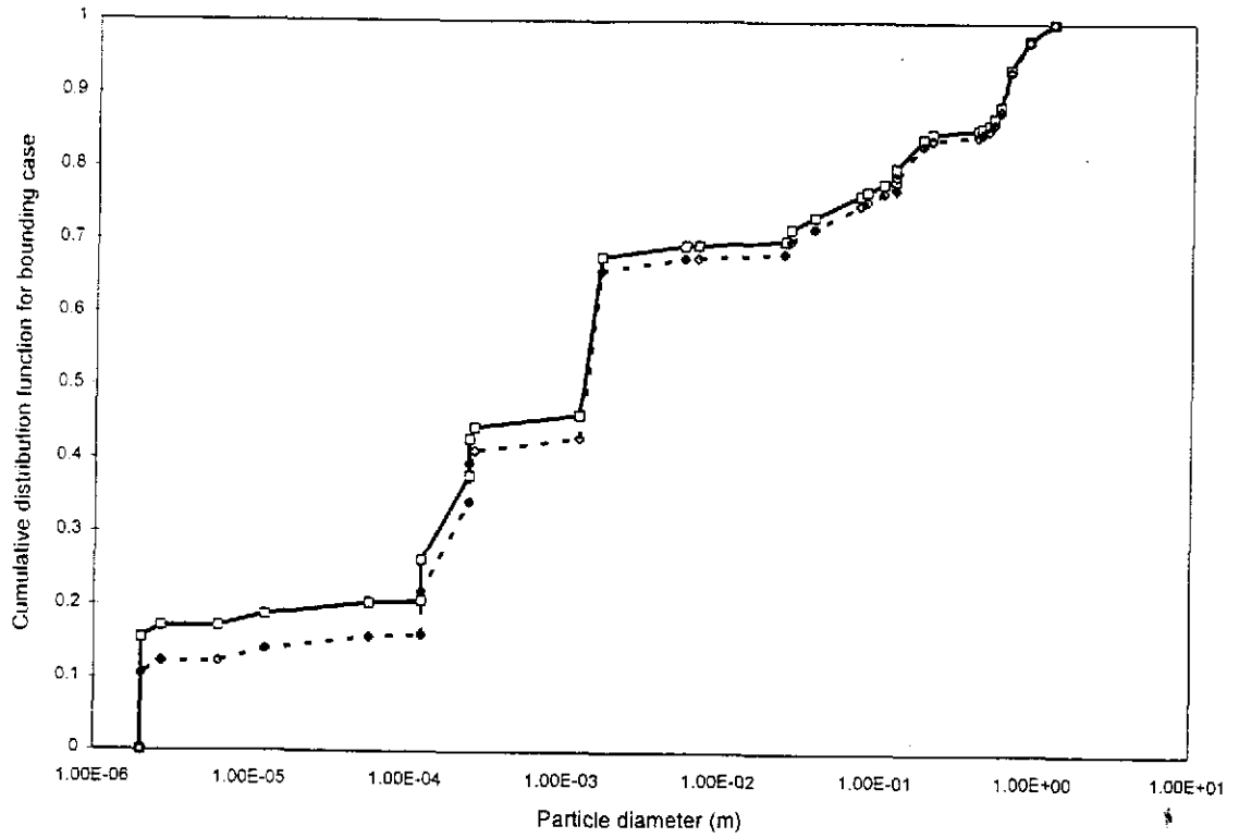
Figure 4. Cumulative distribution function of particle size for the lower bounding case. Solid line - Cement volume is not accounted in total solid volume. Dashed line - Cement volume is accounted in total solid volume and the cements are assumed to have the same particle size distribution as that in waste group 4 and salt.
