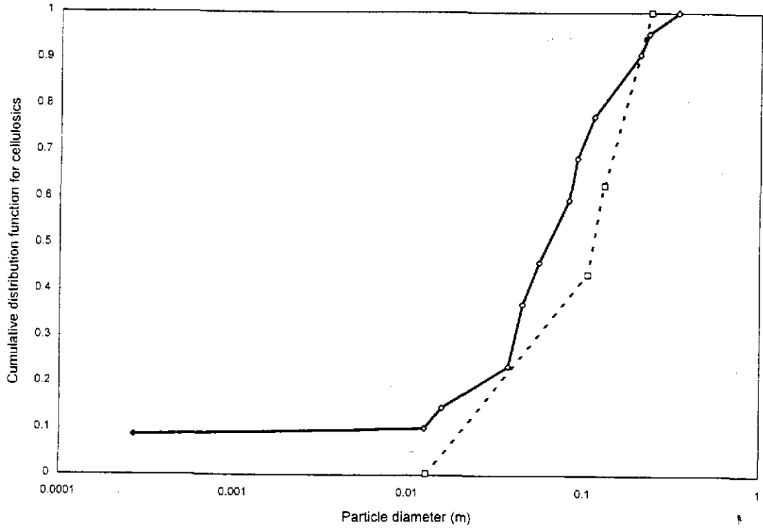
Figure 3. Comparison of particle size distributions between degraded (dashed line) and initial (solid line) cellulose. The dashed line represents 96% of cellulose biodegraded and is calculated in Table 5.
