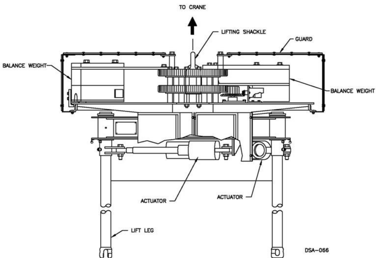
Figure 2.6-31. Adjustable Center-of-Gravity Lifting Fixture
