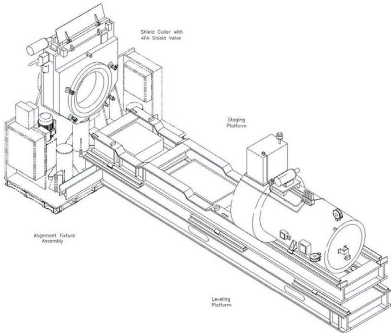
Figure 2.5-23. Waste Transfer Machine Assembly Installed on the Alignment Fixture
