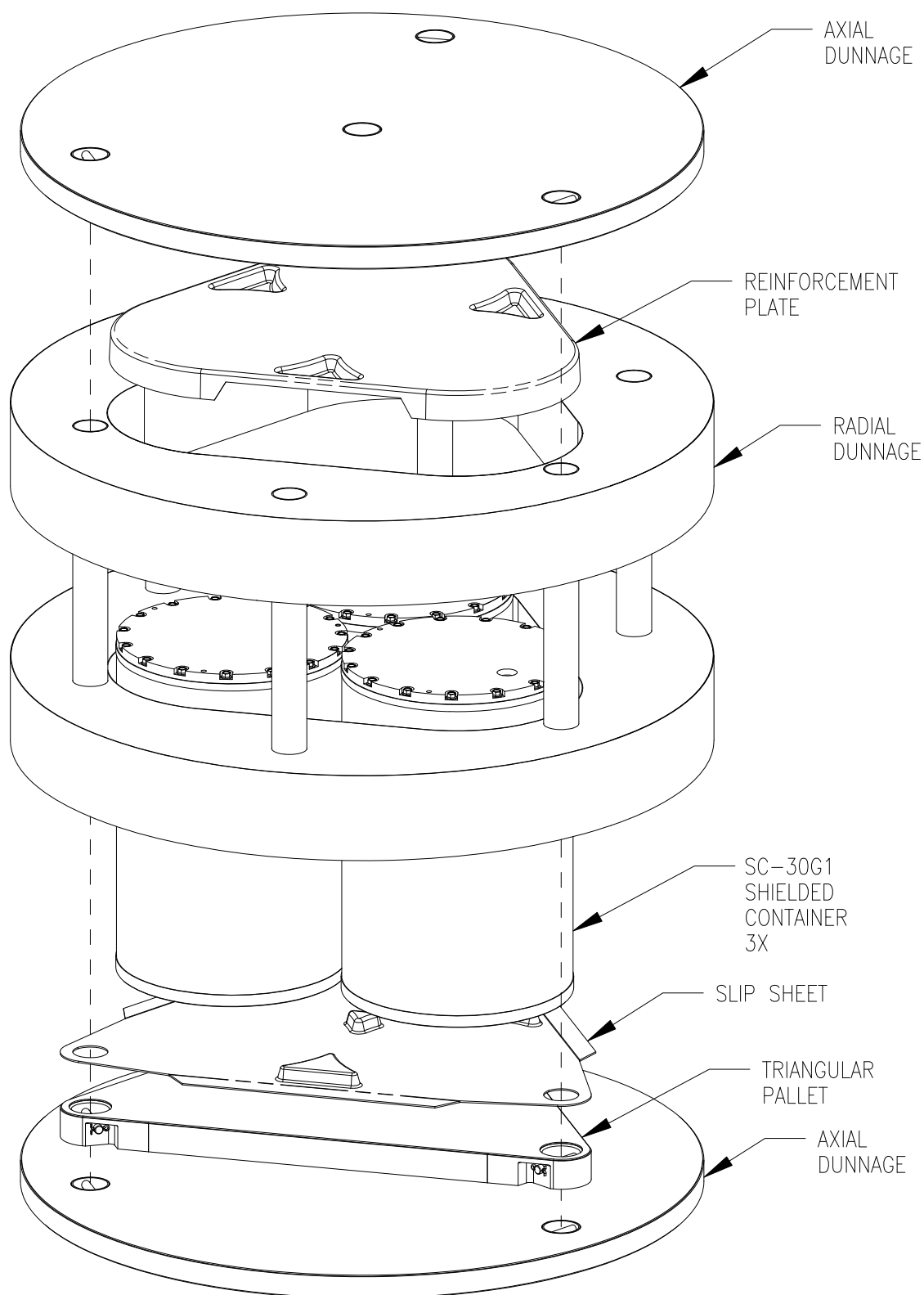
Figure 2.6-19. SC-30G1 Payload Assembly
