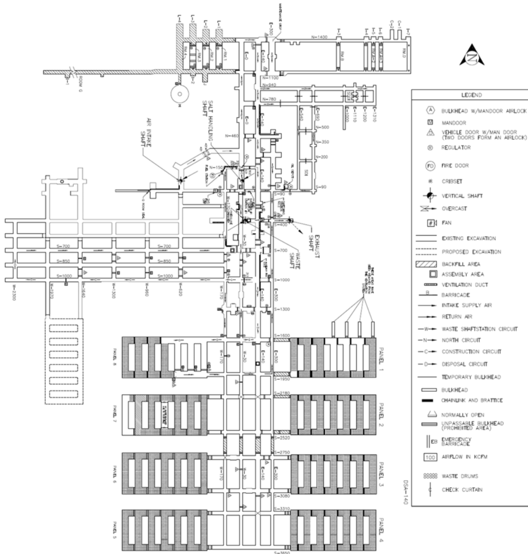
Figure 2.4-14. Underground Ventilation without Utility Shaft and Fans
