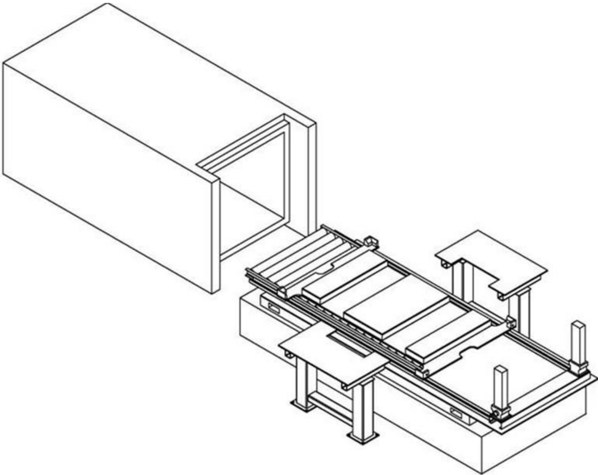
Figure 2.6-39. Payload Transfer Station
