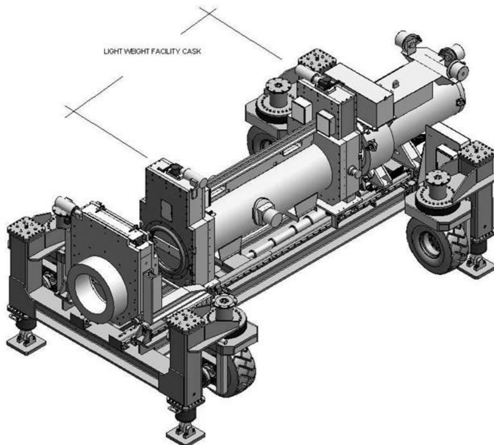
Figure 2.5-24. Horizontal Emplacement Machine with Light Weight Facility Cask
