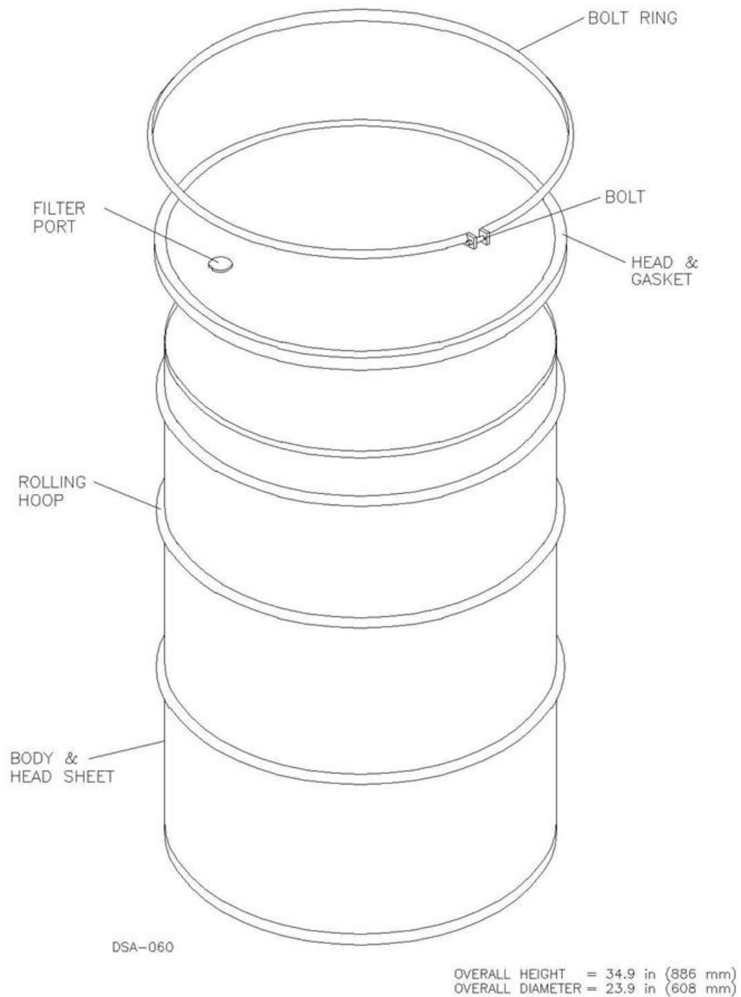
Figure 2.6-6. 55-gallon Drum
