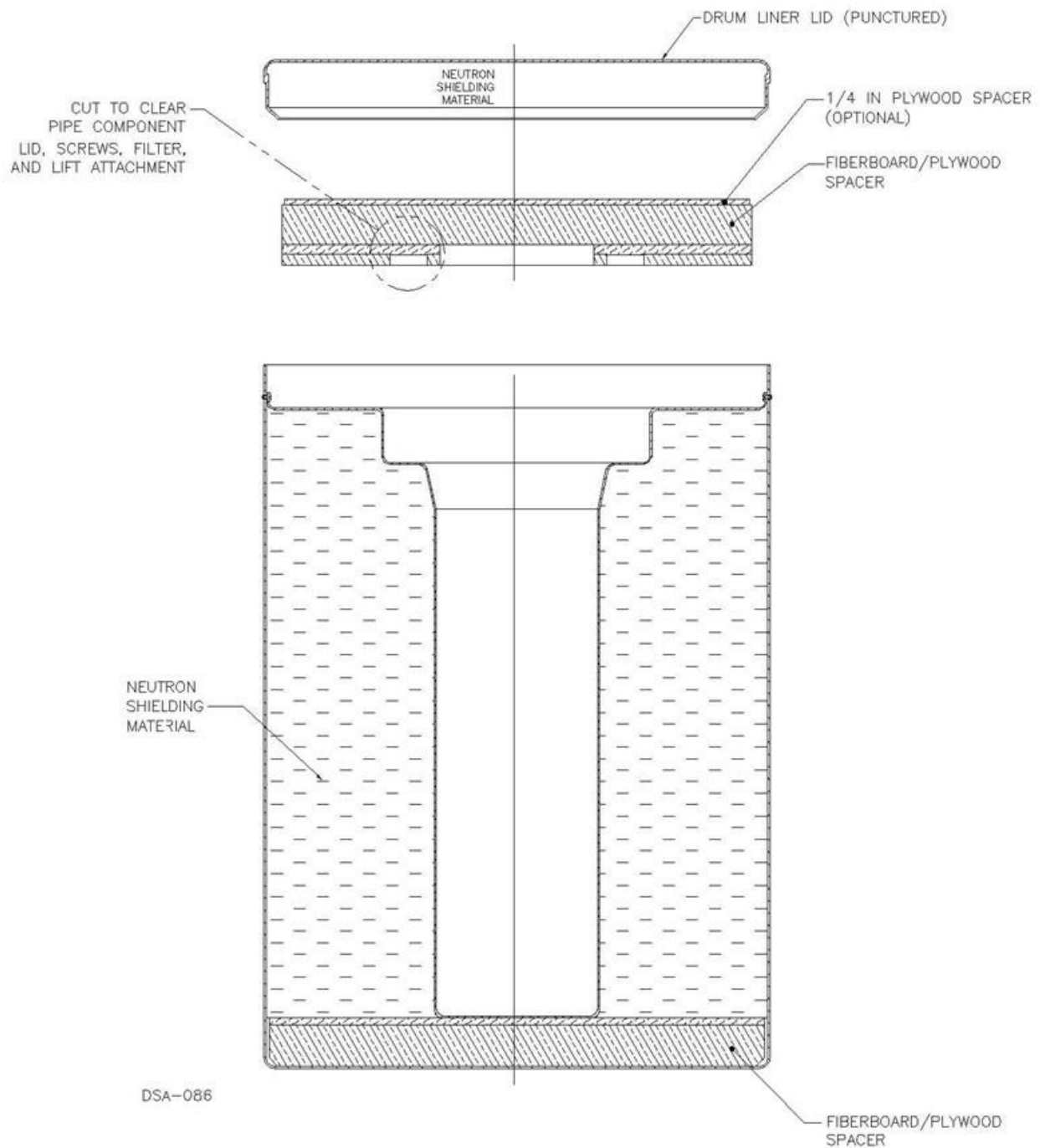
Figure 2.6-15. S300 Pipe Overpack Shield Insert
