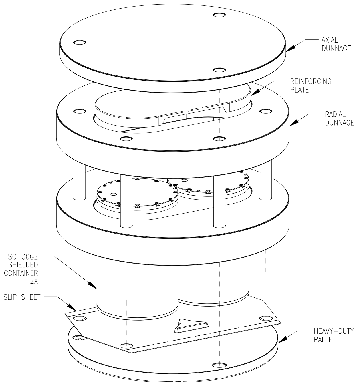
Figure 2.6-21. SC-30G2 Payload Assembly
