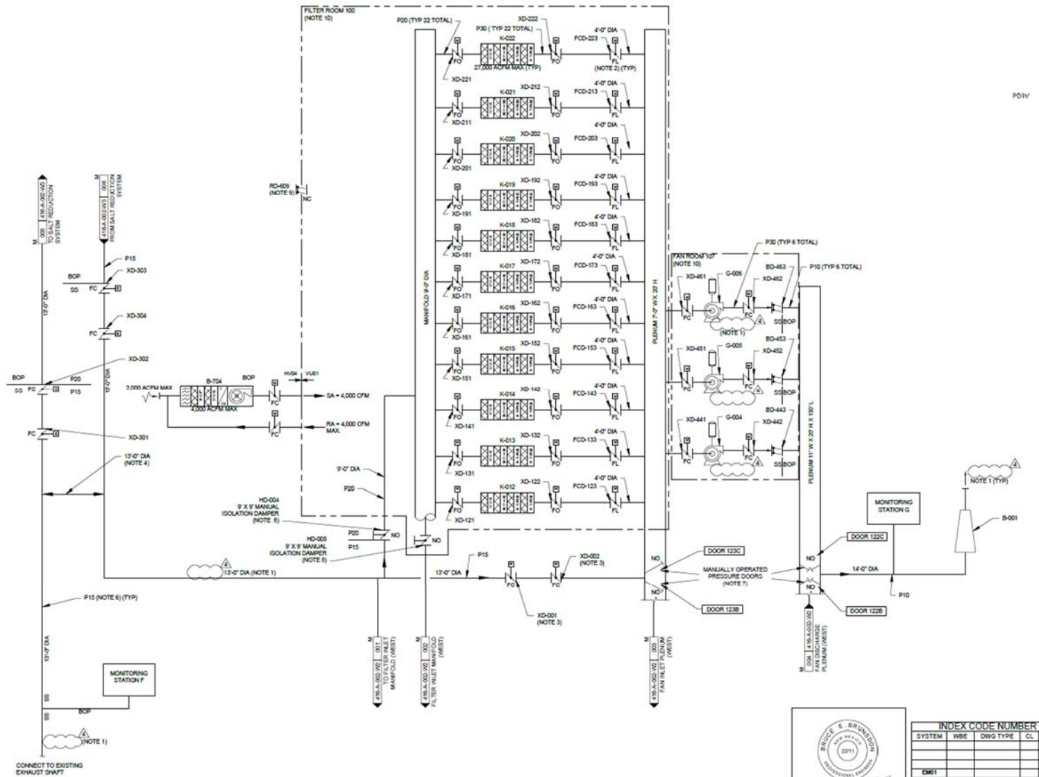
Figure 2.4-13. Underground Ventilation System (Safety Significant Confinement Ventilation System) (Sheet 1 of 2)
