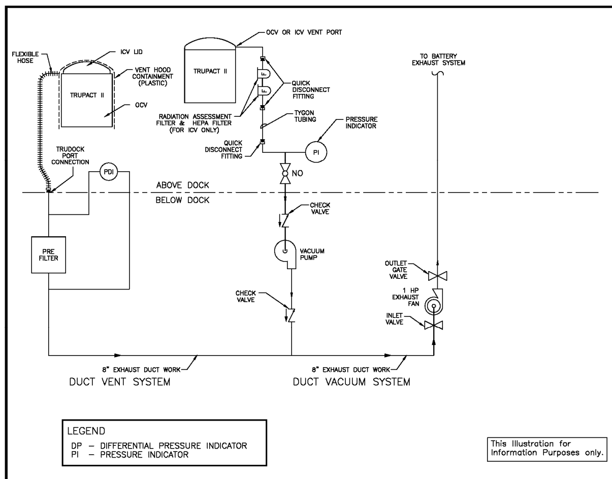
Figure 2.6-32. TRUDOCK Vent Hood System
