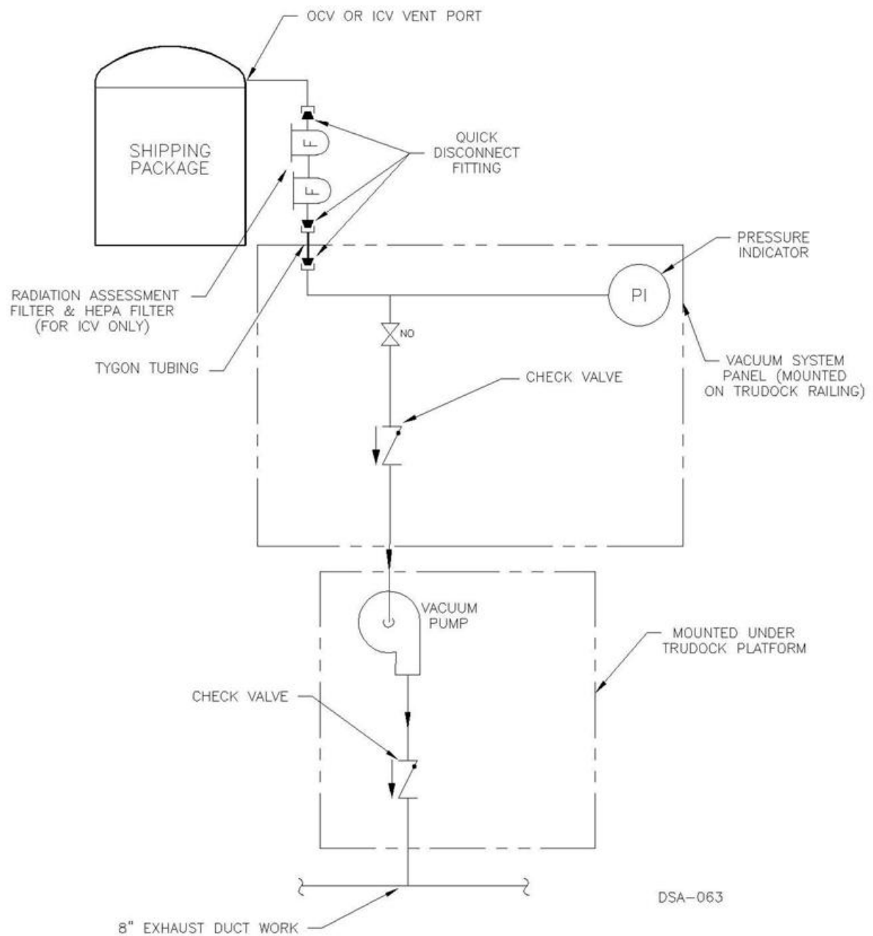
Figure 2.6-33. TRUDOCK Vacuum System
