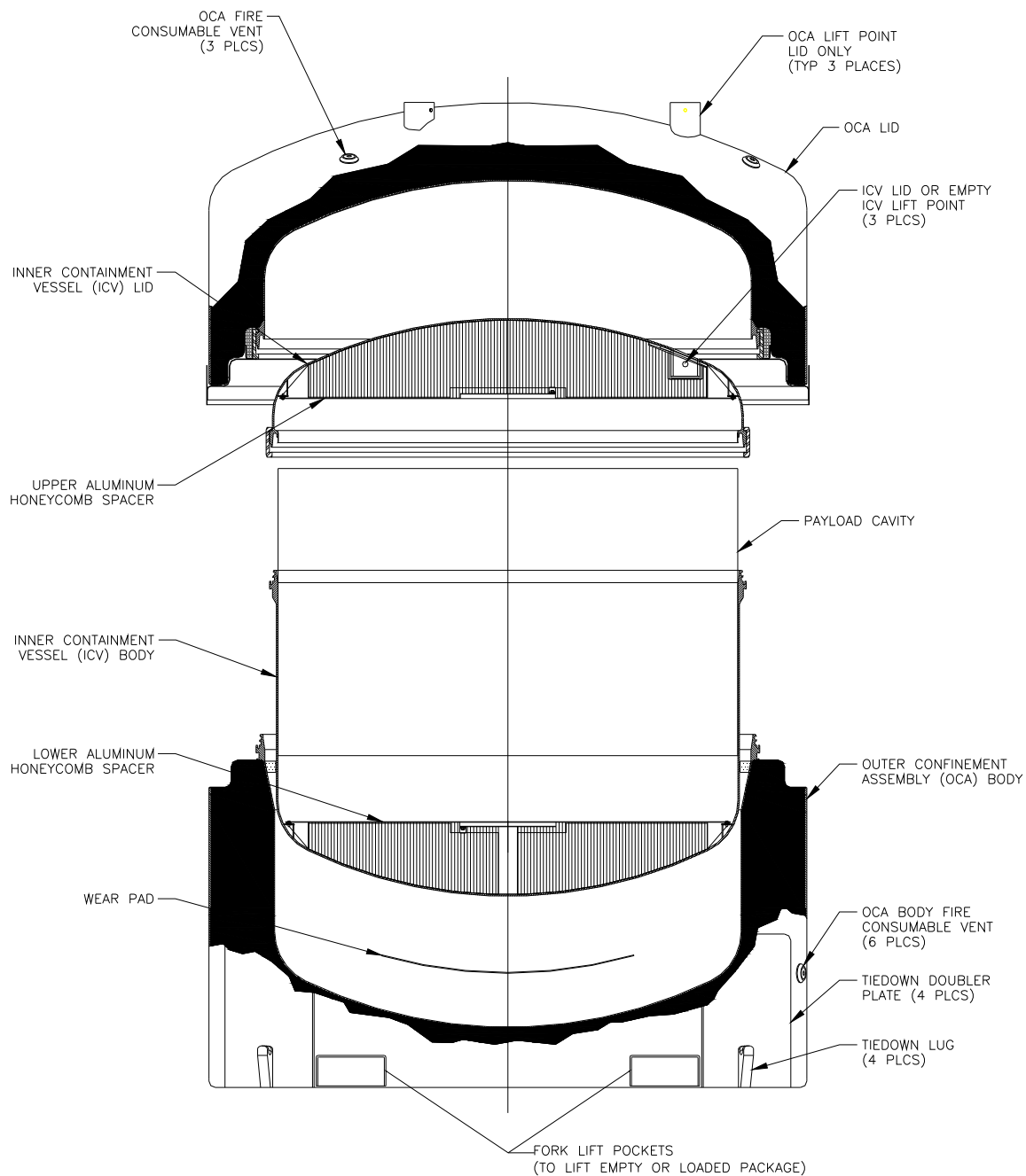
Figure 2.6-4. HalfPACT Shipping Package
