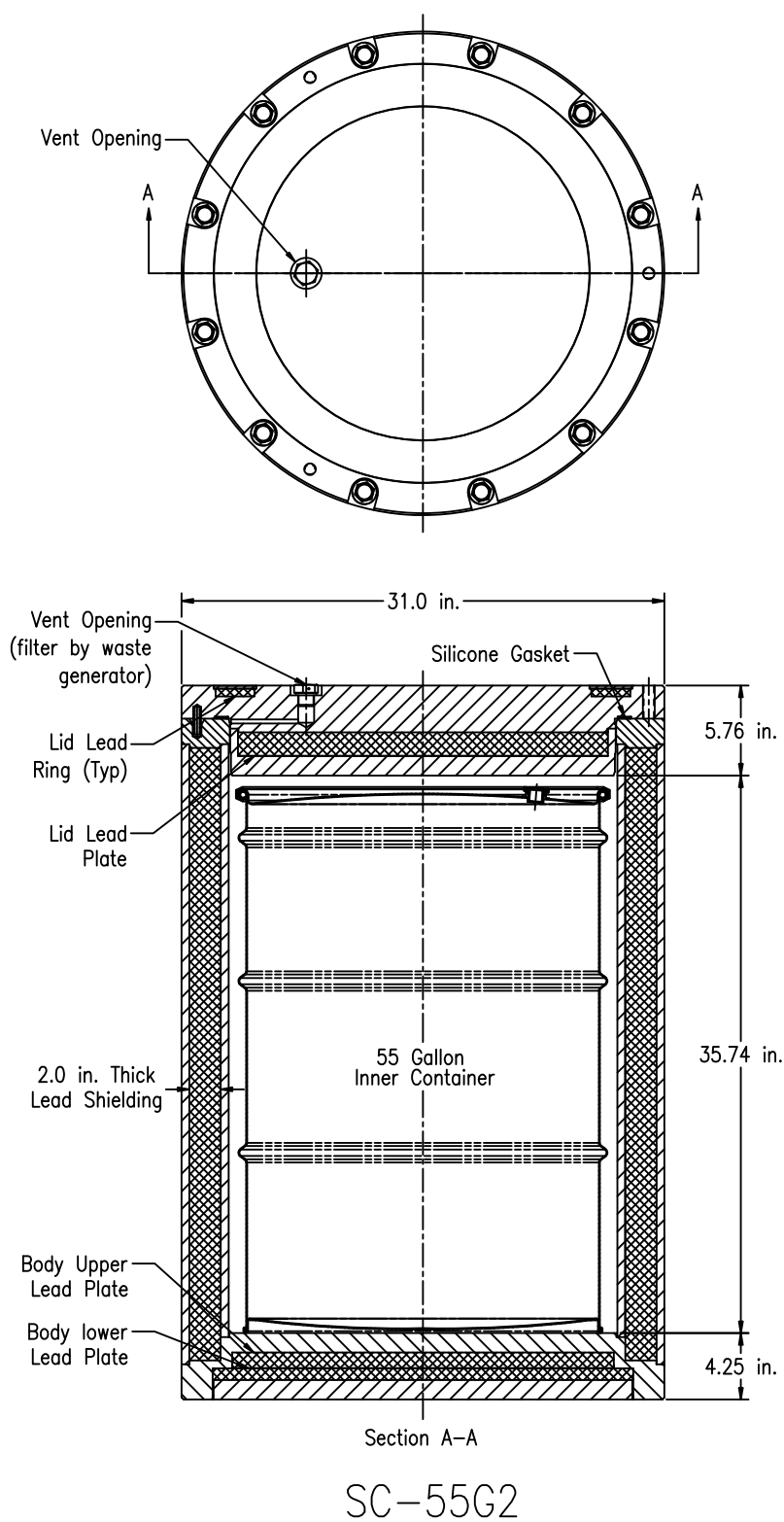
Figure 2.6-28. SC-55G2 Container
