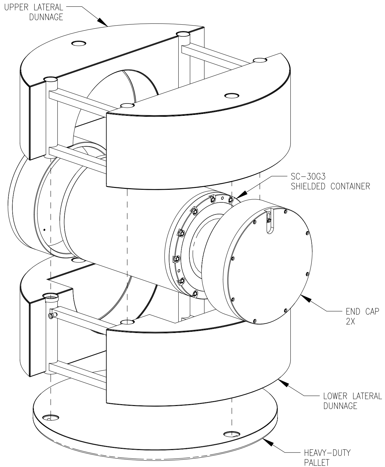
Figure 2.6-23. SC-30G3 Payload Assembly
