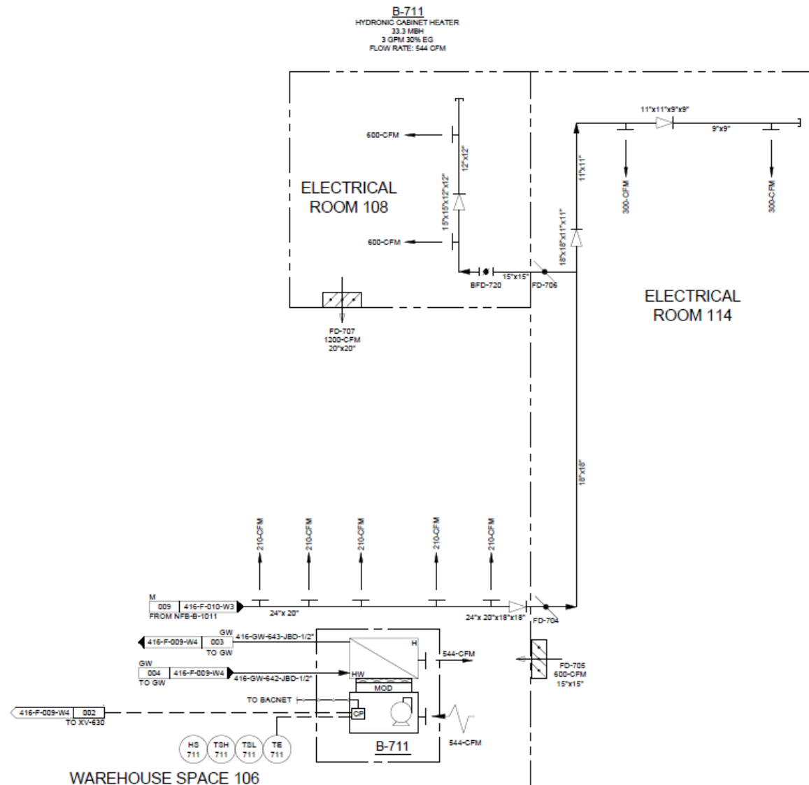
Figure 2.7-5. UVS Filter Building Heating, Ventilation, and Air Conditioning Flow Diagram (Sheet 3 of 4)
