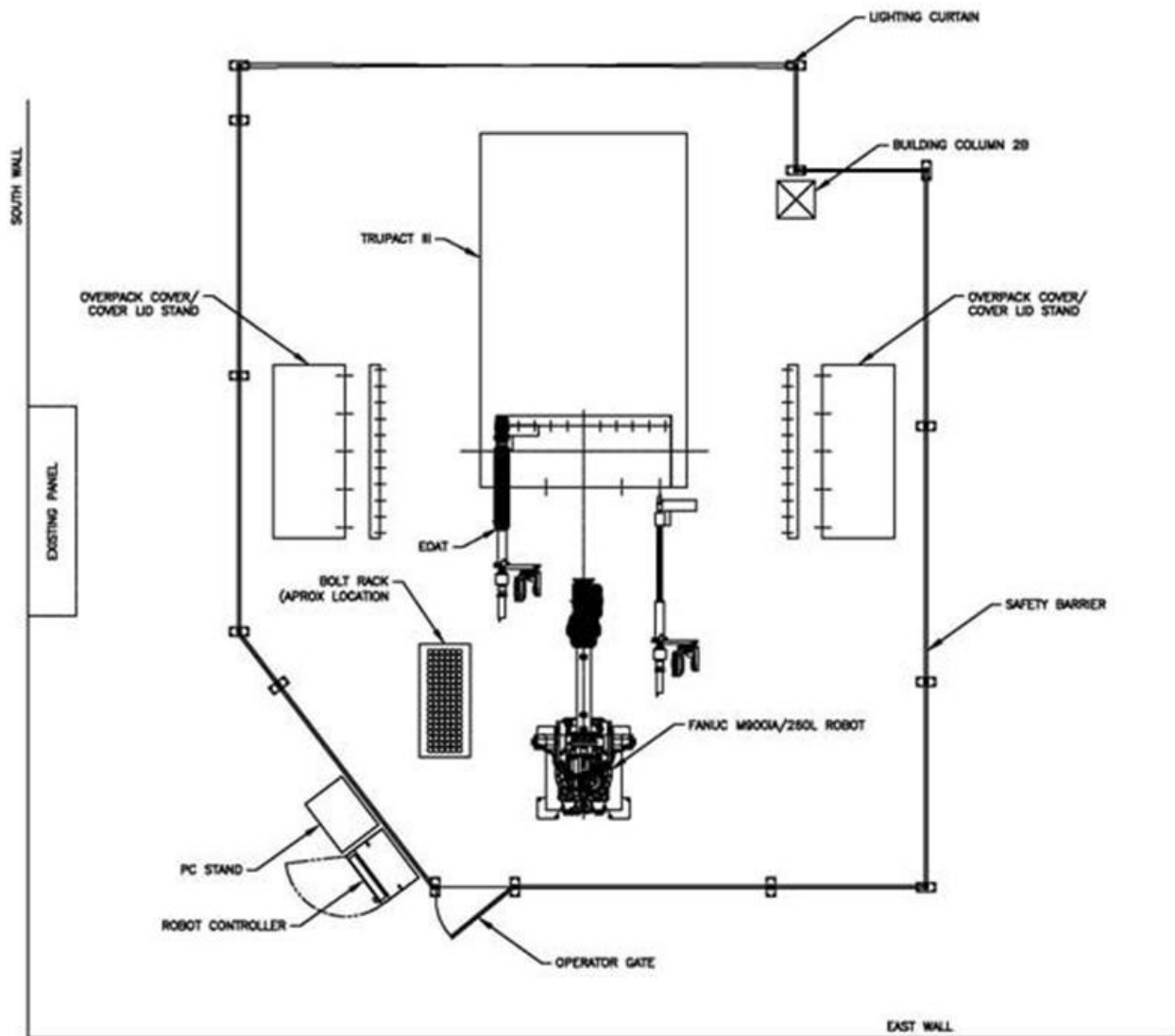
Figure 2.6-38. Bolting Station
