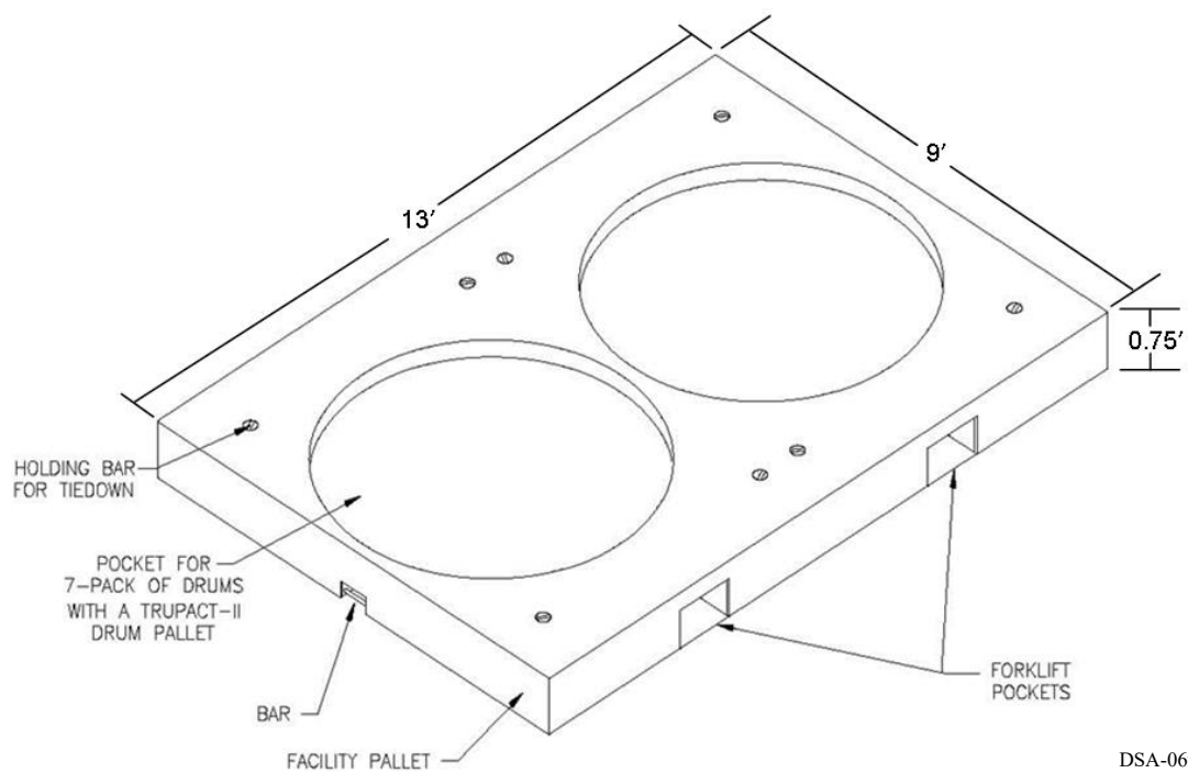
Figure 2.6-37. Facility Pallet
