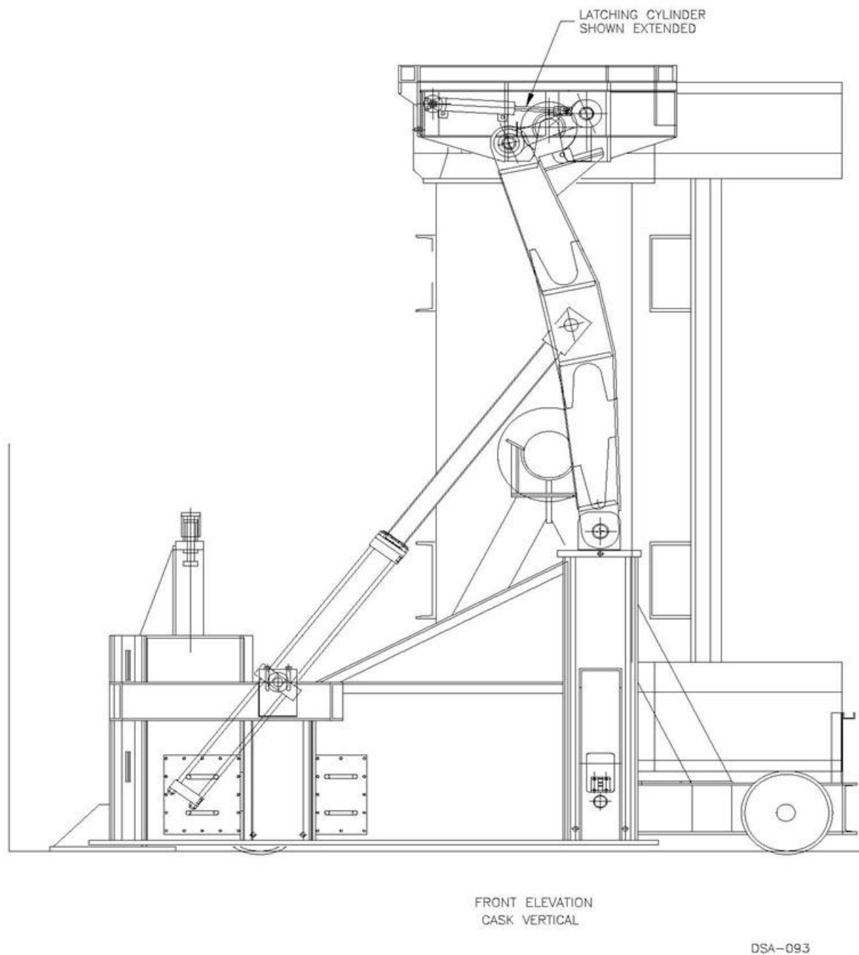
Figure 2.5-17. Facility Cask Rotating Device
