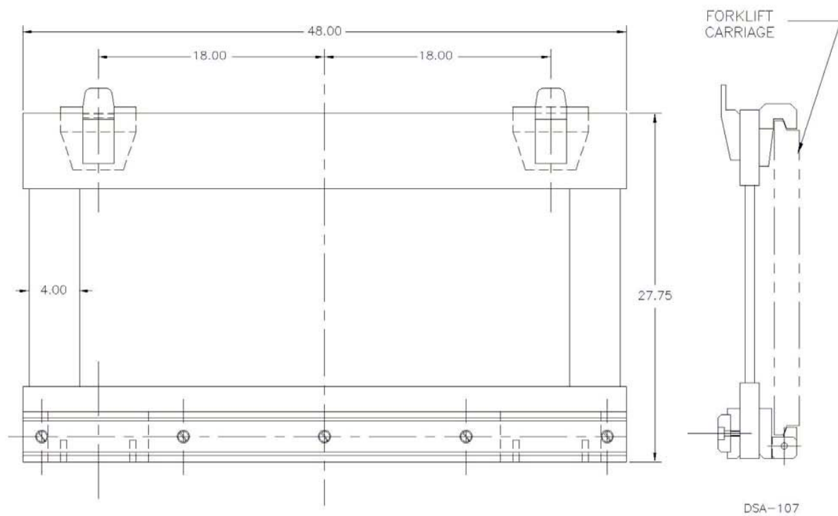
Figure 2.6-35. Standard Waste Box Forklift Fixture
