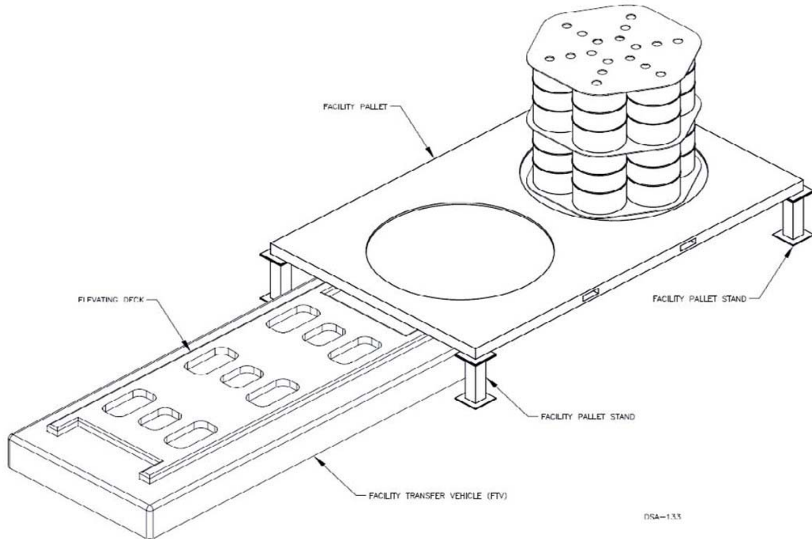
Figure 2.6-40. Facility Pallet on Stand and Facility Transfer Vehicle
