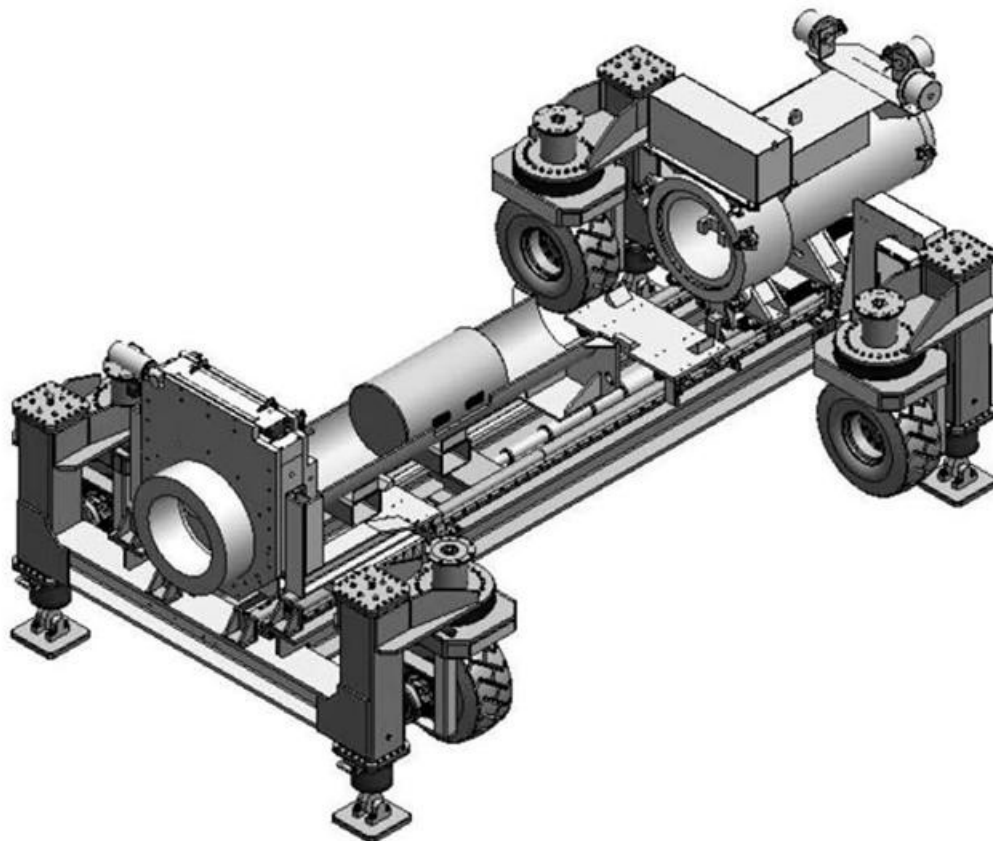
Figure 2.5-27. Horizontal Emplacement Machine with Shield Plug
