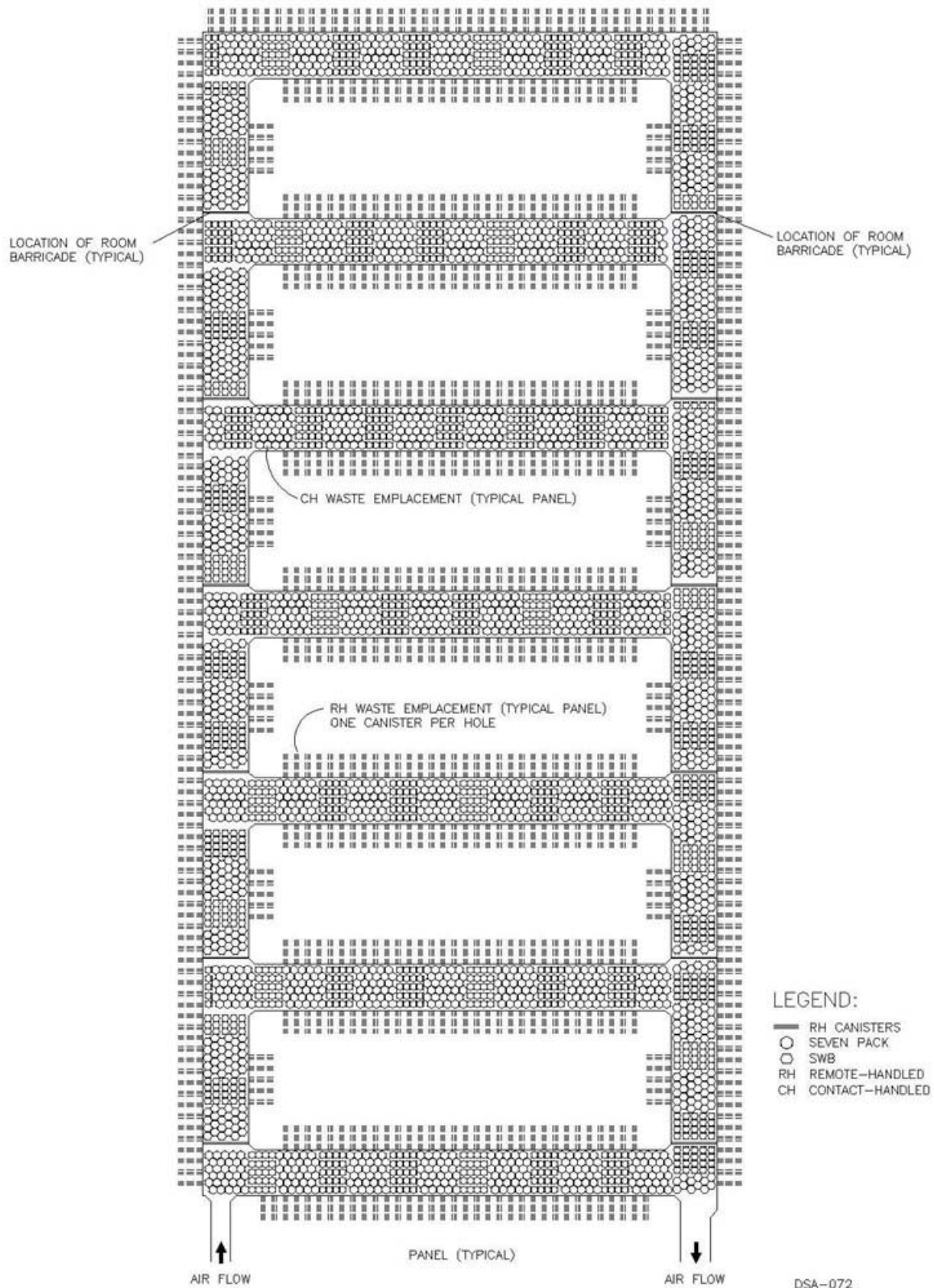
Figure 2.4-17. Typical Waste Disposal Configuration
