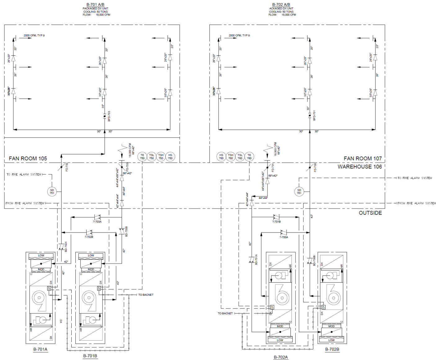
Figure 2.7-5. UVS Filter Building Heating, Ventilation, and Air Conditioning Flow Diagram (Sheet 1 of 4)
