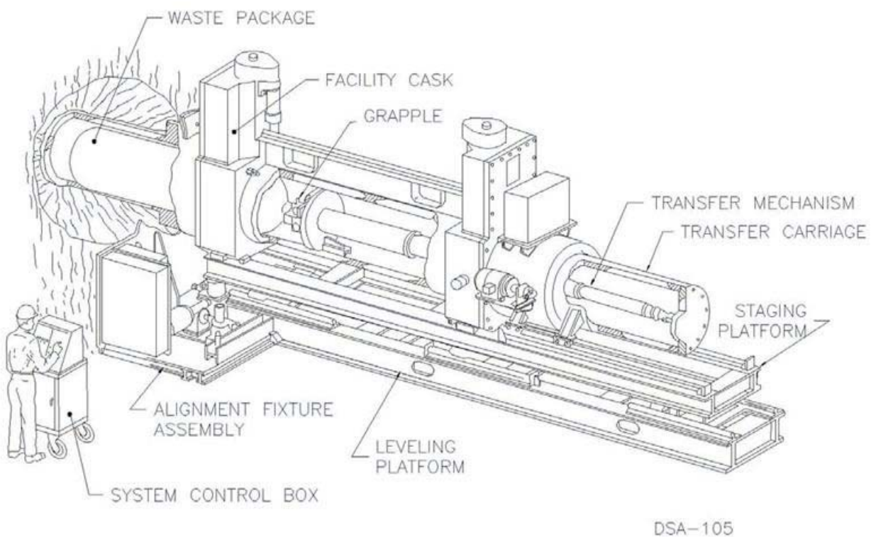
Figure 2.5-26. Remote-Handled Waste Canister Emplacement
