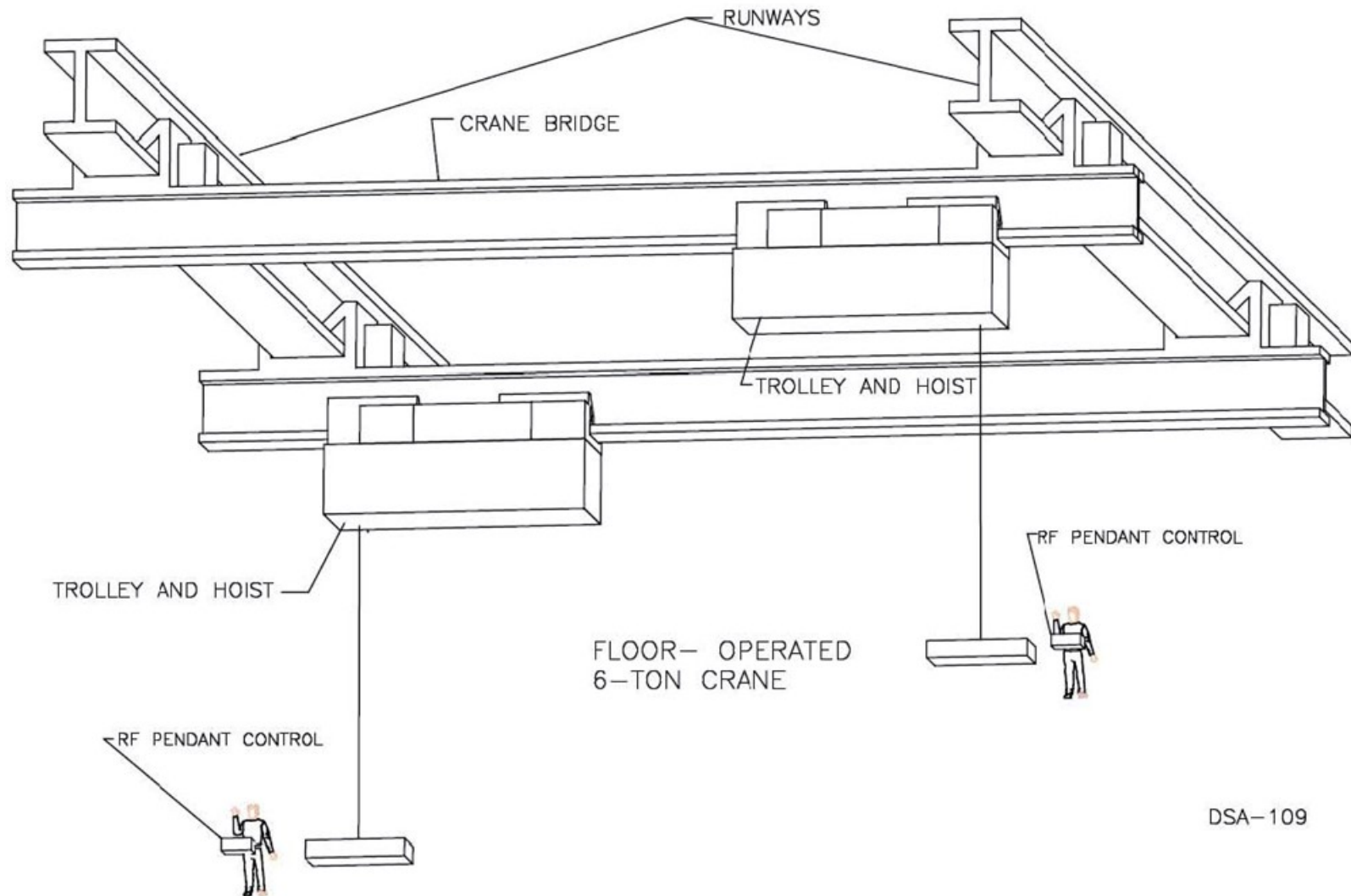
Figure 2.6-30. Typical Overhead Crane
