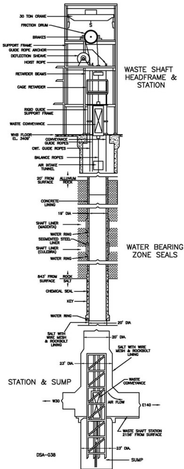
Figure 2.4-15. Waste Shaft, Hoist, and Conveyance Arrangement
