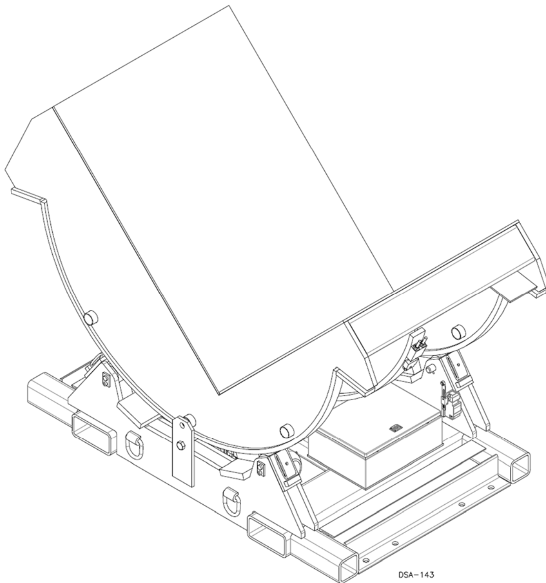
Figure 2.6-17. SCA Upender
