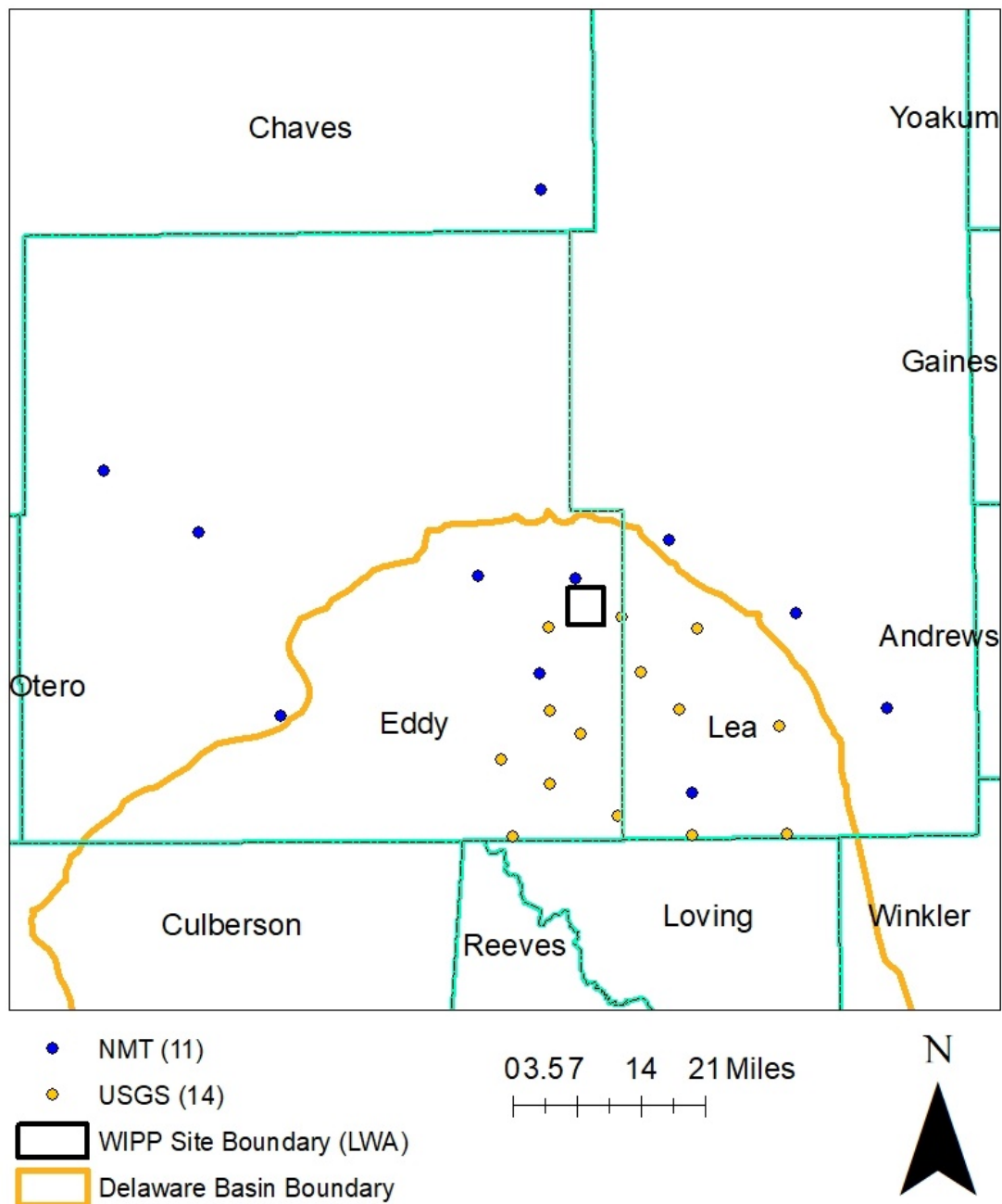
Figure 1.5-1 Seismograph Stations in the WIPP Network
