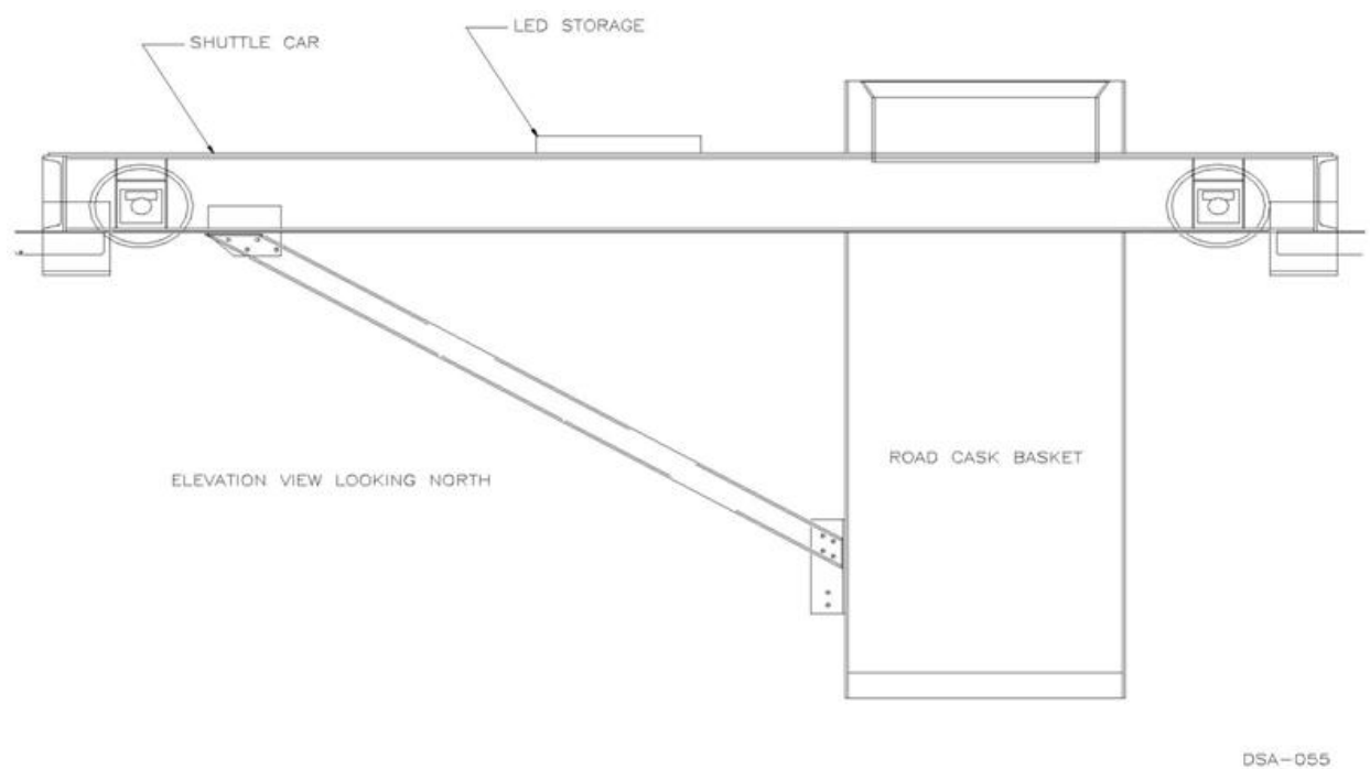
Figure 2.5-15. Transfer Cell Shuttle Car
