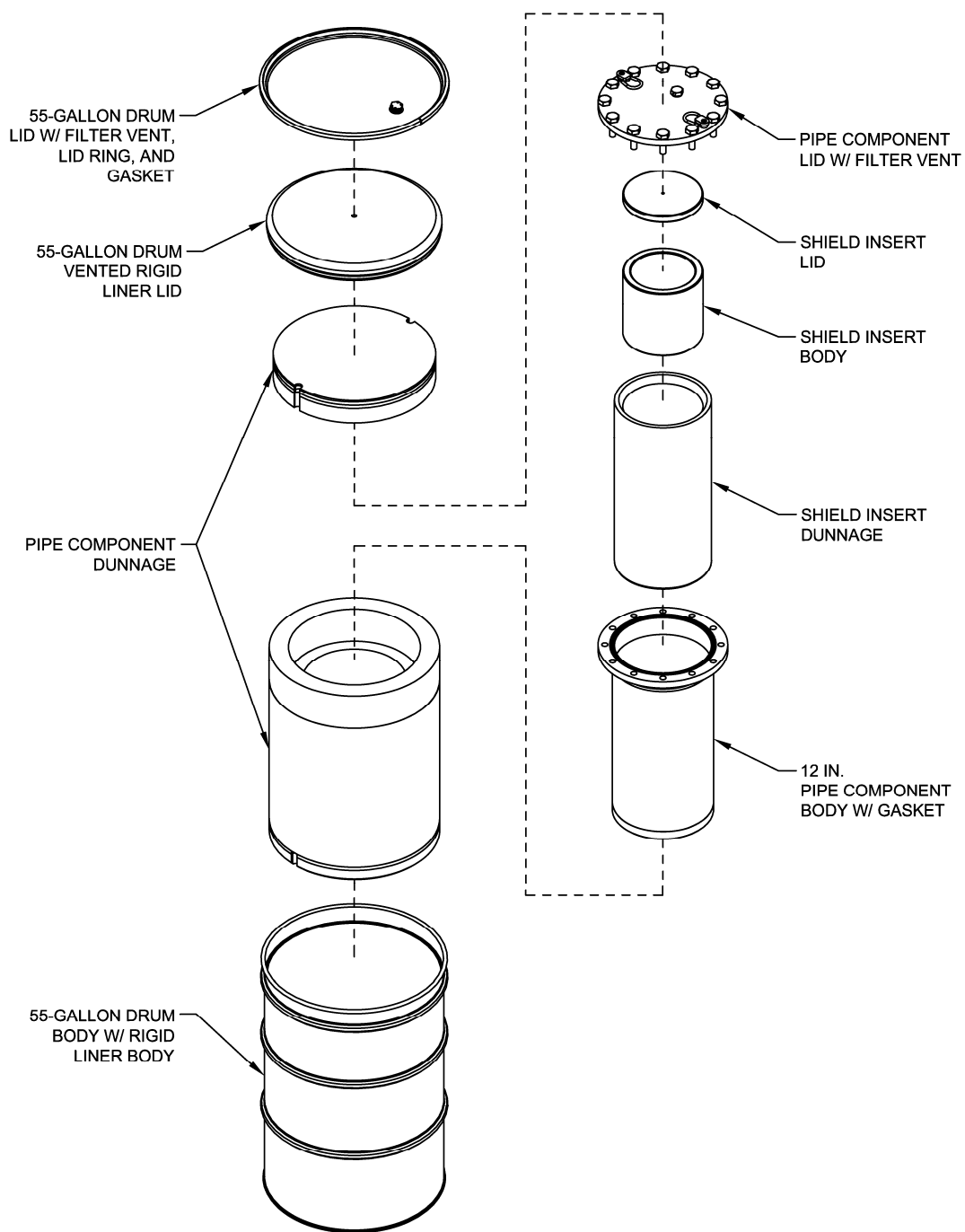
Figure 2.6-14. S200 Pipe Overpack
