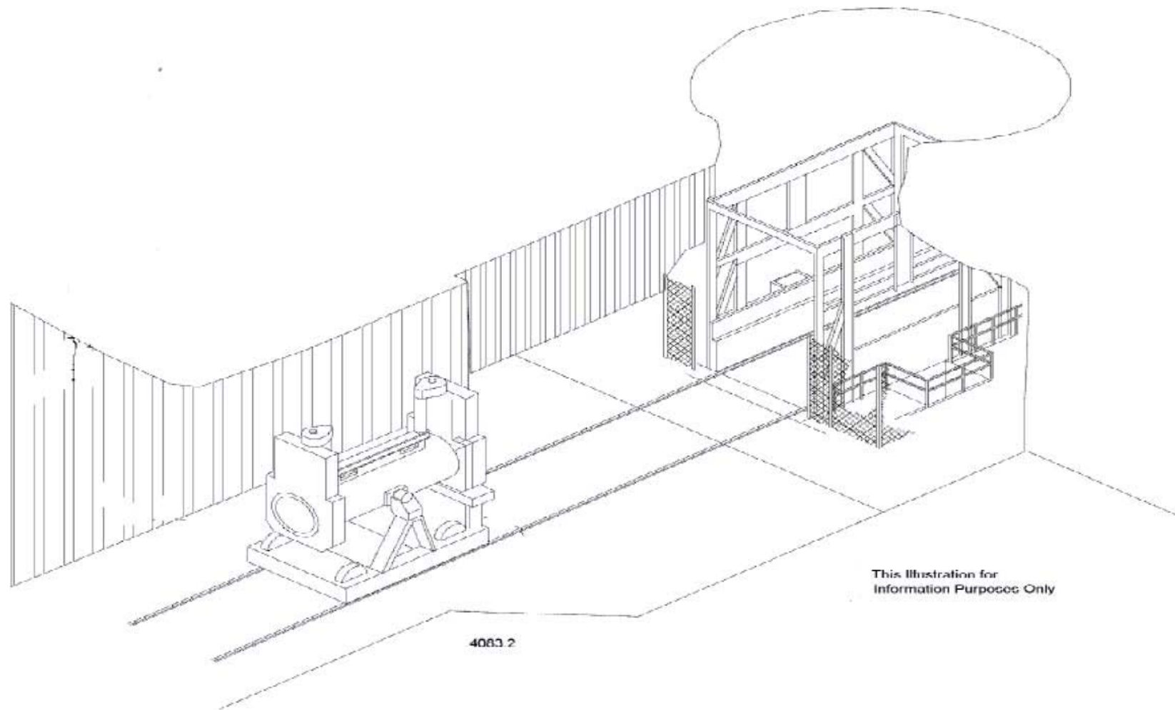
Figure 2.5-28. Remote-Handled Waste Handling Facility Cask Unloading from Conveyance
