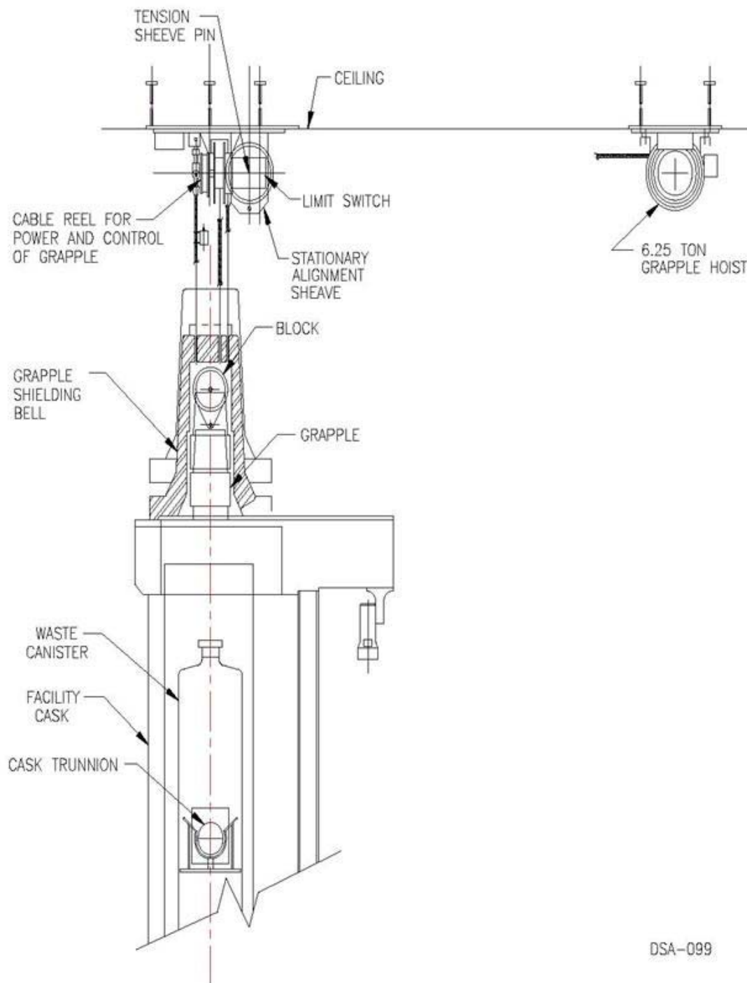
Figure 2.5-18. 6.25-ton Facility Cask Loading Room Grapple Hoist
