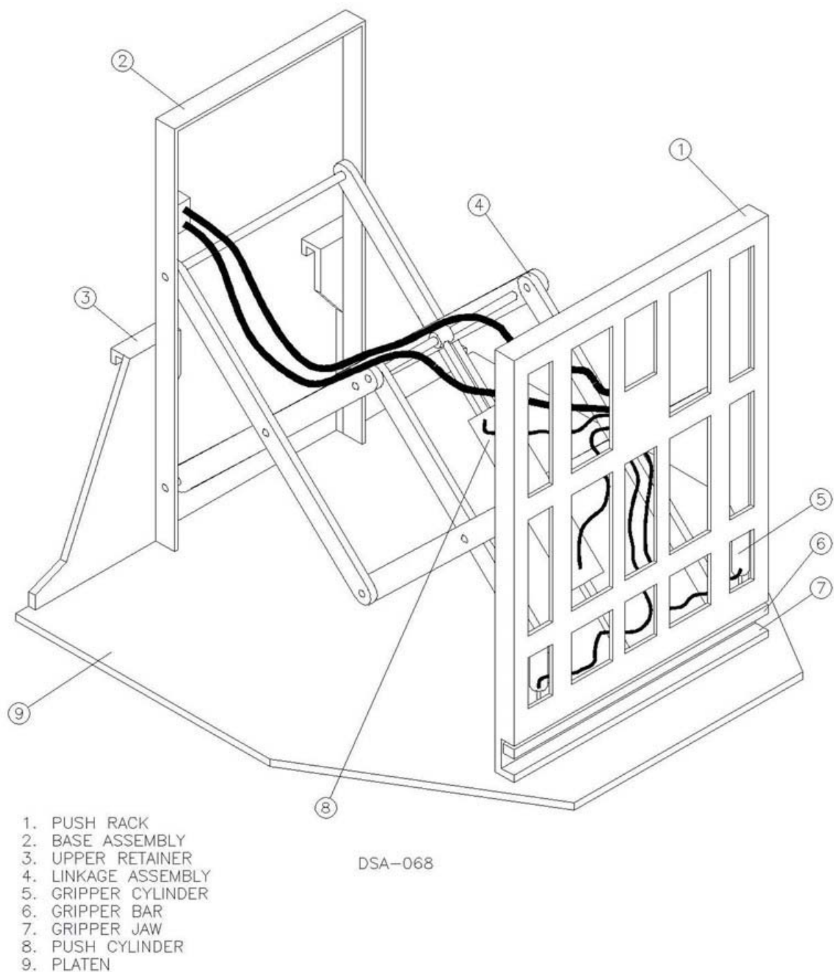
Figure 2.6-42. Push/Pull Attachment Requiring Forklift Tine Removal
