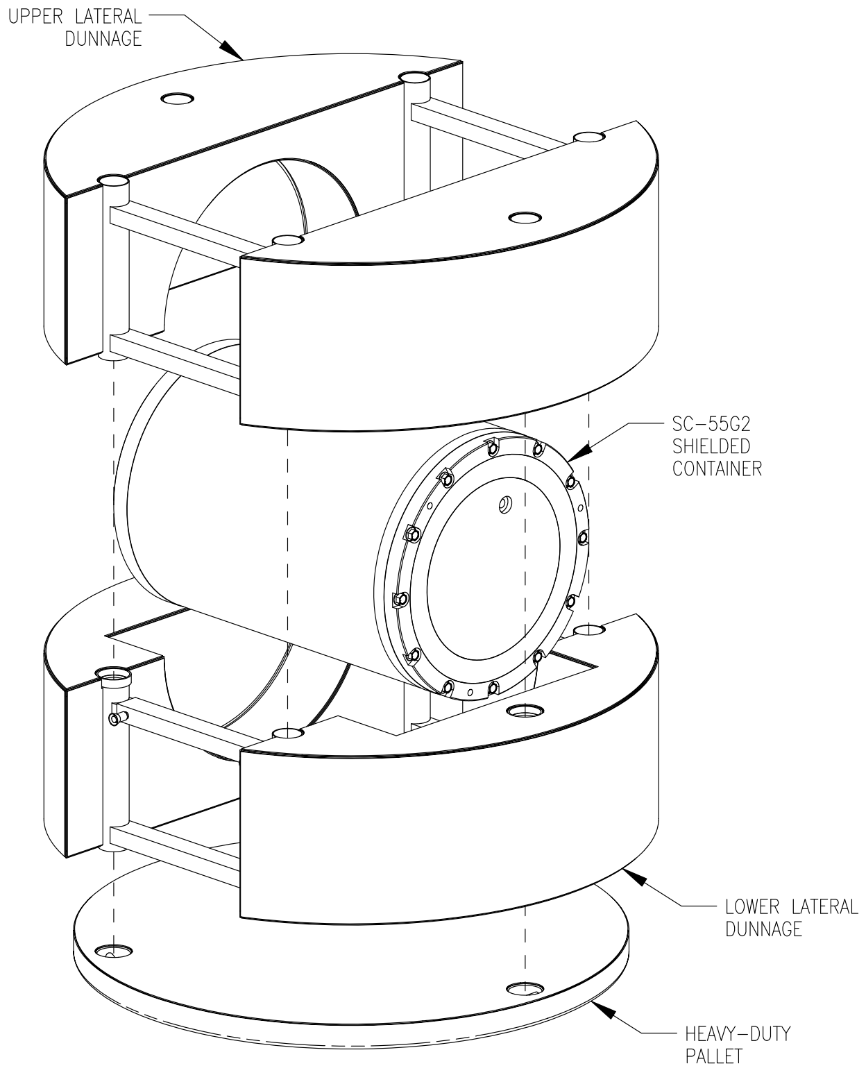
Figure 2.6-27. SC-55G2 Payload Assembly
