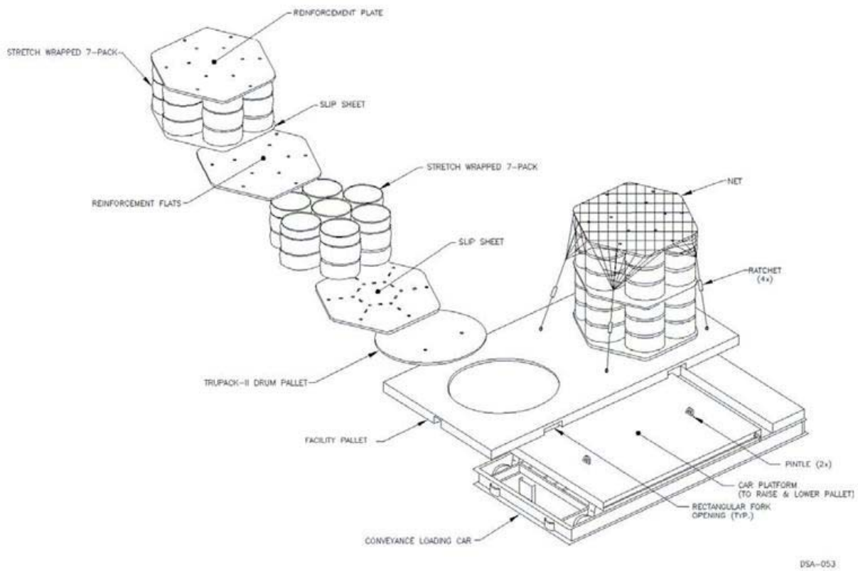
Figure 2.6-41. Facility Pallet on Conveyance Loading Car
