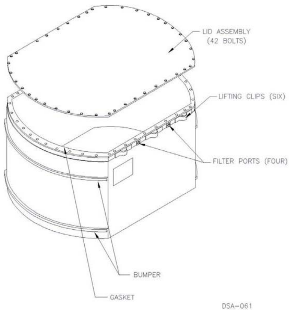
Figure 2.6-9. Standard Waste Box
