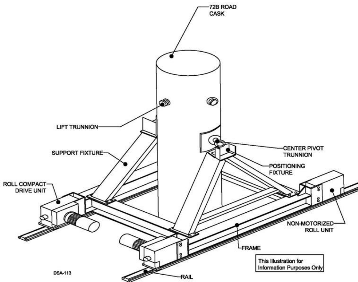
Figure 2.5-11. Remote-Handled Transuranic 72-B Shipping Package on Transfer Car
