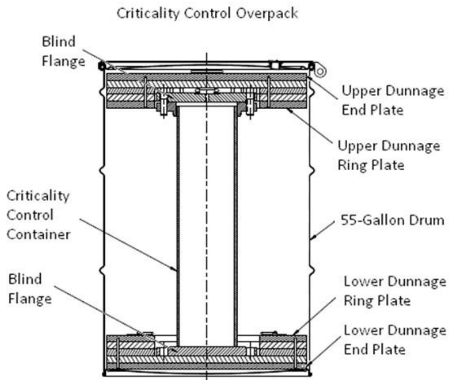
Figure 2.6-29. Criticality Control Overpack
