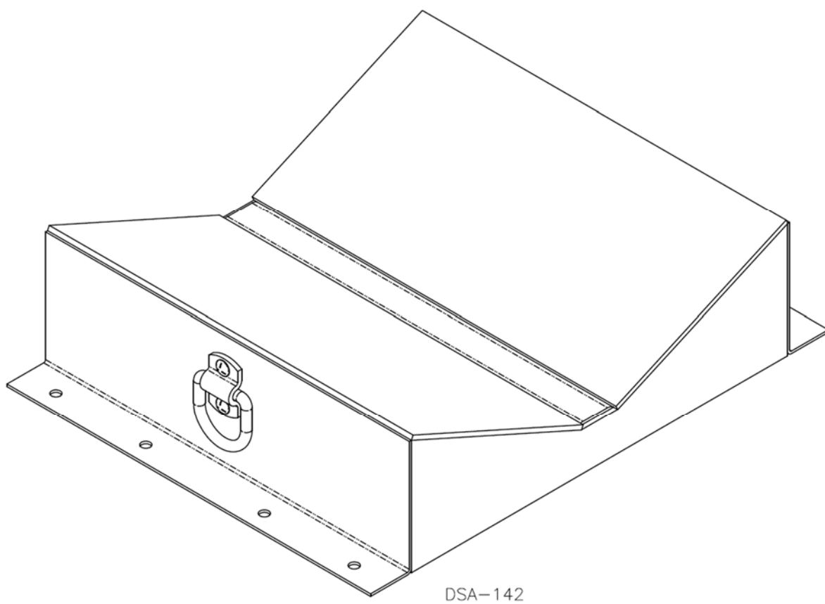
Figure 2.6-18. Cradle
