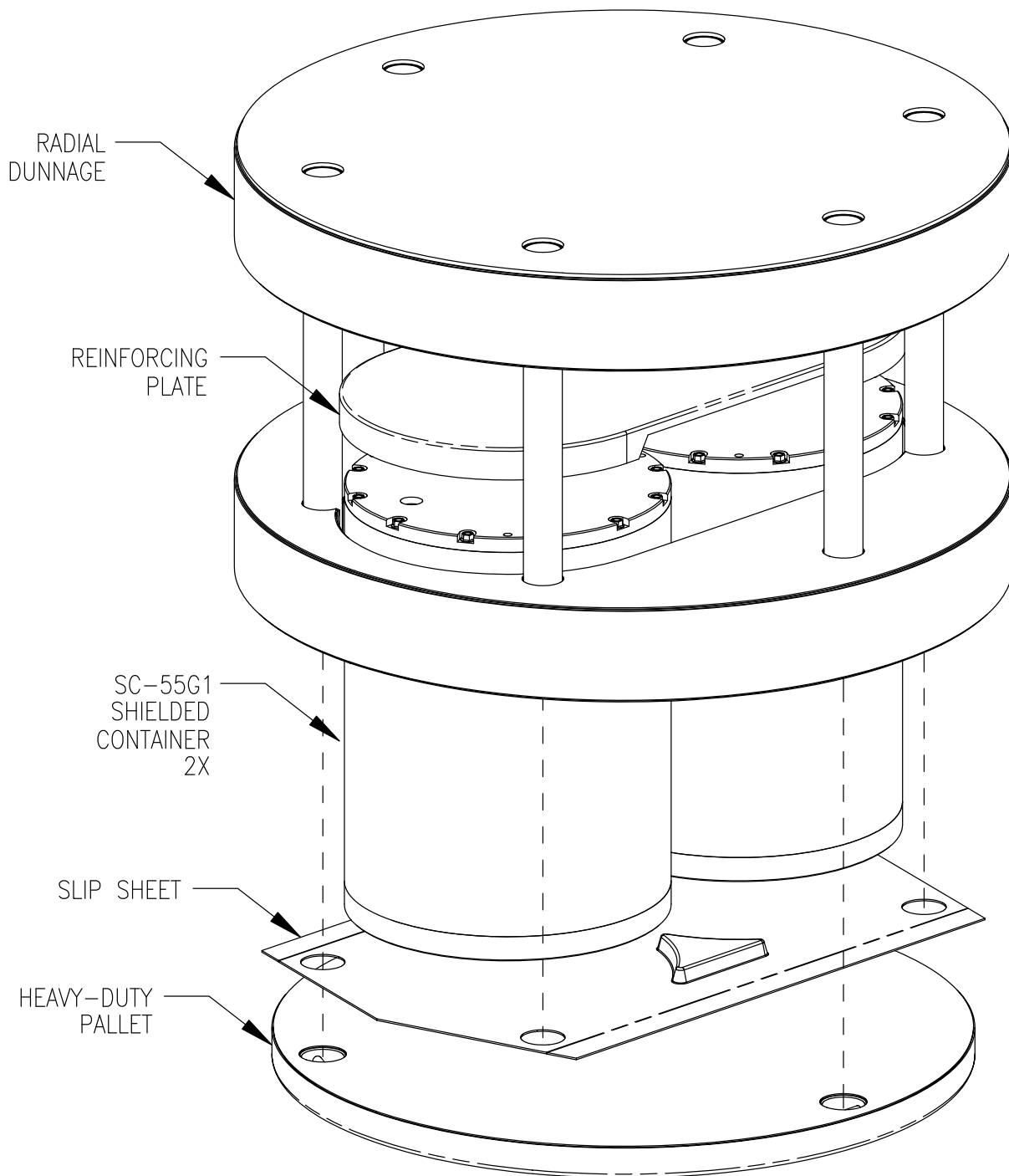
Figure 2.6-25. SC-55G1 Payload Assembly
