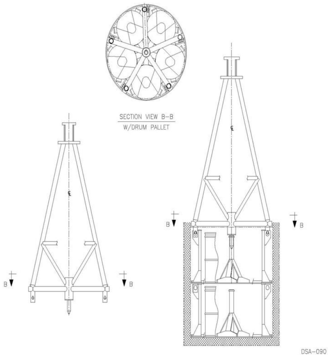
Figure 2.5-13. 10-160B Drum Carriage Lifting Fixture
