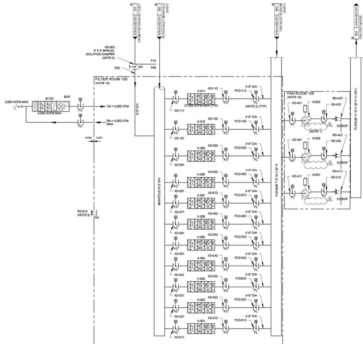
Figure 2.4-13. Underground Ventilation System (Safety Significant Confinement Ventilation System) (Sheet 2 of 2)
