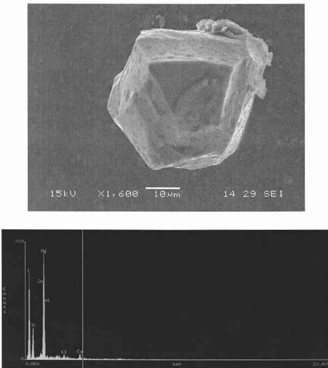
Figure 5. SEM image (top) and associated EDS spectrum (bottom) of a particle that remained after dissolving the MgO in nitric acid. The top SEM image is stored in the file 123h1i10.bmp, the bottom EDS spectra is in 1023h1i10.eds. Both are located in: WIPP-MM MgO-4 SEM/EDS supplemental binder-1.
