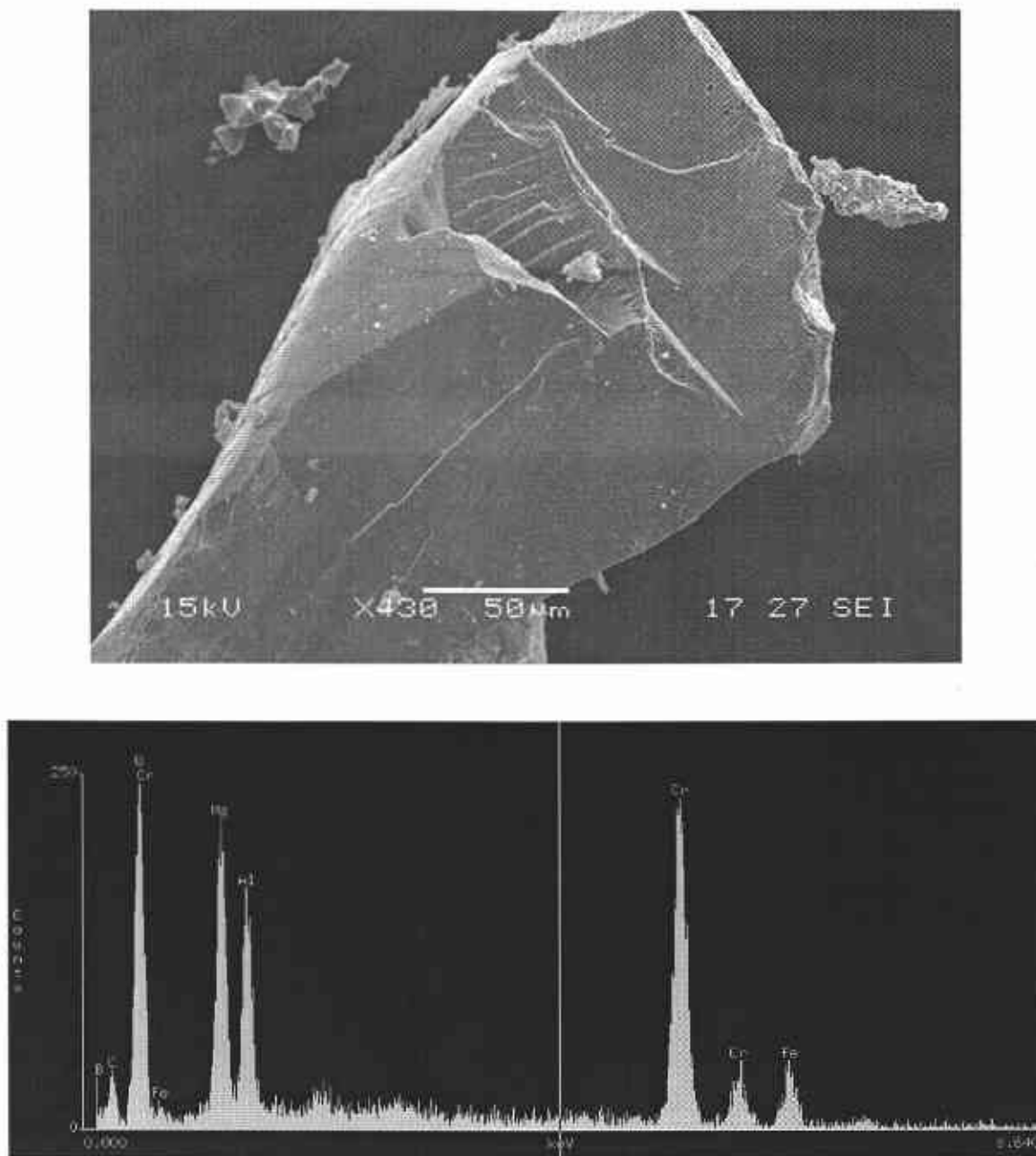
Figure 4. SEM image (top) and associated EDS spectrum (bottom) of a particle that remained after dissolving the MgO in nitric acid. Notice the conchoidal fractures in the SEM image; spinels (in general) have a lack of cleavage (Deer et al., 1992). The top SEM image is stored in the file 718h1i5a.bmp, the bottom EDS spectra is in 718h1i5as1.eds. Both are located in: WIPP-MM MgO-2 SEM/EDS supplemental binder-1.
