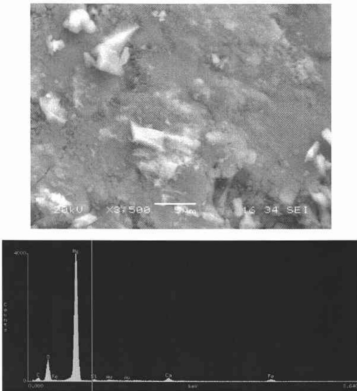
Figure 2. SEM image (top) and EDS spectrum (bottom) of a piece of unusual as-received MgO. Gold is from Au-Pd coating prior to imaging, carbon is from the carbon tape mount. The top SEM image is stored in the file 816h4i2a.bmp, the bottom EDS spectra is in 816h4i2a.eds. Both are located in: WIPP-MM MgO-2 SEM/EDS supplemental binder-1.
