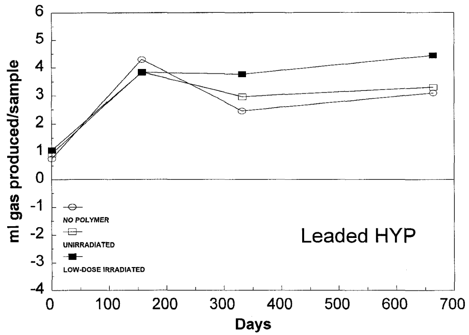
Figure 39. Total gas produced in anaerobic amended samples containing ledged hypalon.
