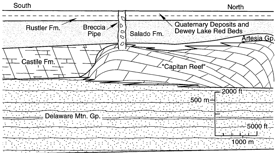
Generalized Cross Section
