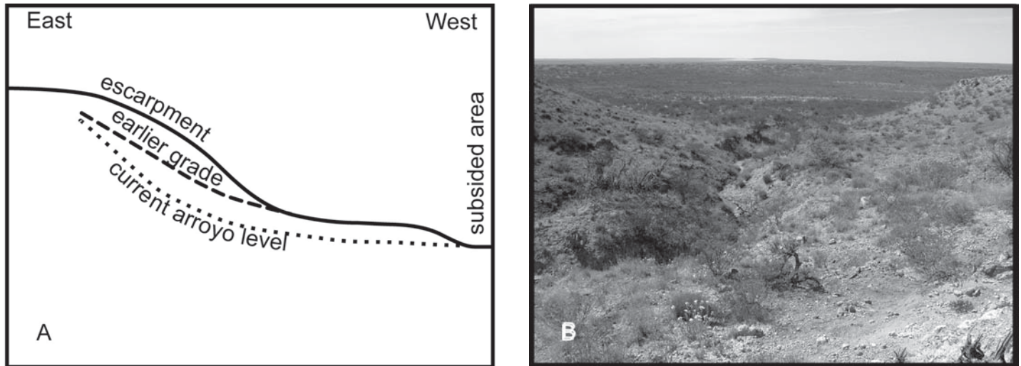
FIGURE 4. A. Diagrammatic cross-section of Livingston Ridge and the depression west of it illustrating the regrading arroyo responding to a subsidence event. B. Photograph of modern cut of arroyo regrading to the depression
