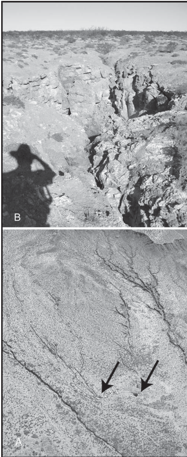
FIGURE 7. A. Low-angle aerial photograph of vertical-walled collapse sinks (arrows) that have captured local drainage. The left sink is shown in B and is more linear, along fracture trends. The southern (right) sink is circular, but vertical-walled. The escarpment of Livingston Ridge at the top right corner of the photograph is the Dewey Lake Formation of Permian or Triassic age. B. Surface photograph of northern (left) collapse sink in A. The sink developed in exposed uppermost gypsum (A-5) of the Forty-niner Member of the Rustler Formation.
