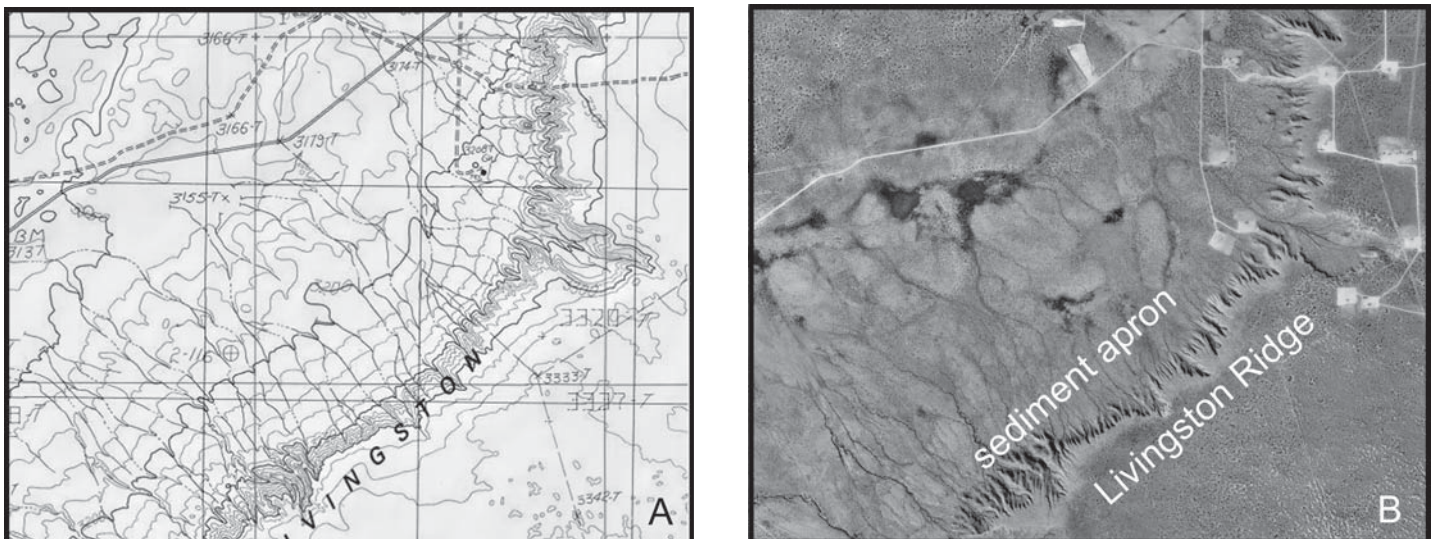
FIGURE 5. Topographic map segment (A) and equivalent segment of an aerial photograph (B) (NAPP frame 9610-248, dated 10/22/1996) illustrating the embayment on Livingston Ridge, sediment apron, and straight arroyos leading to a shallow depression.
