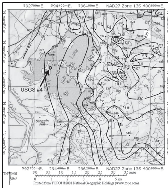
FIGURE 6. Topography of Laguna Grande de la Sal, with superimposed contours (m amsl) and values for the elevation of the top of halite in the Salado. “USGS #4” is the location of a borehole reported by Robinson and Lang (1938) with the elevation of halite. Drainages not visible at this map scale have been traced with arrows at the downstream end and star patterns at low points. A possible pathway for brine follows a series of enclosed valleys south of Laguna Grande along the inferred low on the surface of Salado halite.
