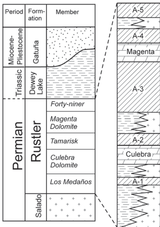
FIGURE 2. Basic stratigraphic units involved in the Nash Draw processes. Informal units of the Rustler Formation are also used in Powers et al. (2006).
