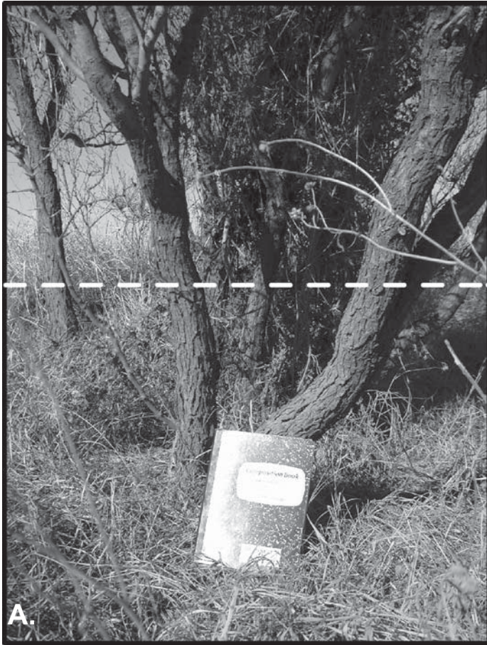
FIGURE 12. Silt-stained mesquite trunks (A) and floating cow patties (B, just below dashed line at arrow) show levels of standing water consistent with debris strandlines along the edge of the karst valley (Figure 10). The depth is estimated to be 1 m or more in the deepest part of the depression. This area was examined late in 2004 (when the photos were taken), and the likely cause of the runoff event was a major rainfall in late September 2004 (see Hillesheim et al., 2006).
