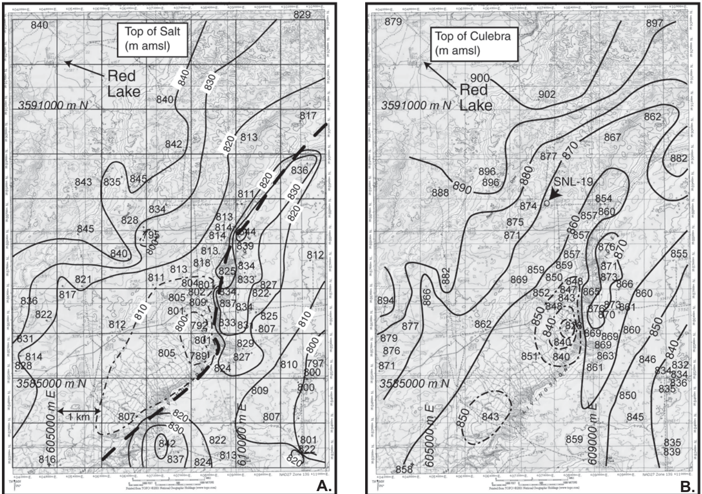
FIGURE 3. A. Elevation of the top of halite in the Permian Salado Formation (m amsl). The heavy dashed line along Livingston Ridge marks the margin of halite dissolution for the Salado inferred by Powers et al. (2003) by examining changes in thickness of the upper Salado and lower Rustler. Depressions are shown with dash-dot contour patterns. B. The elevation of the Culebra Dolomite Member of the Permian Rustler Formation, which overlies the Salado, exhibits structure similar to that shown by Salado halite and other units above halite. Similar “relief” across both surfaces indicates that the Culebra has subsided consistent with the proposed dissolution of halite.
