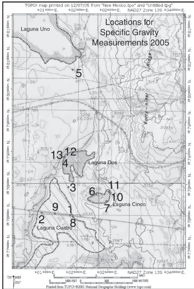
FIGURE 13. A. Topographic map segment showing the location of lakes near the mouth of the southeastern arm of Nash Draw where specific gravity measurements were taken in 2005 to differentiate waters. (see also Figure 1 for locations). B. Surface photograph from December 2005 of the upwelling sulfate-rich northern spring in Laguna Cinco (near location 11 in A). The upwelling spring is about 30 cm in diameter. Photograph view is toward the southeast.
