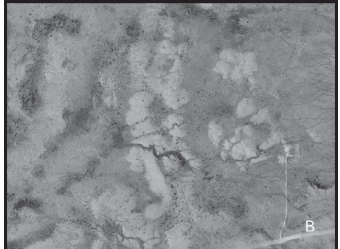
FIGURE 8. A. Surface photograph of collapse sink with sloping sides of gypsum and alluvial fill. B. Segment of aerial photograph (NAPP frame 9611-50, dated 10/22/1996) showing this same sink and the drainage that connects such features.
