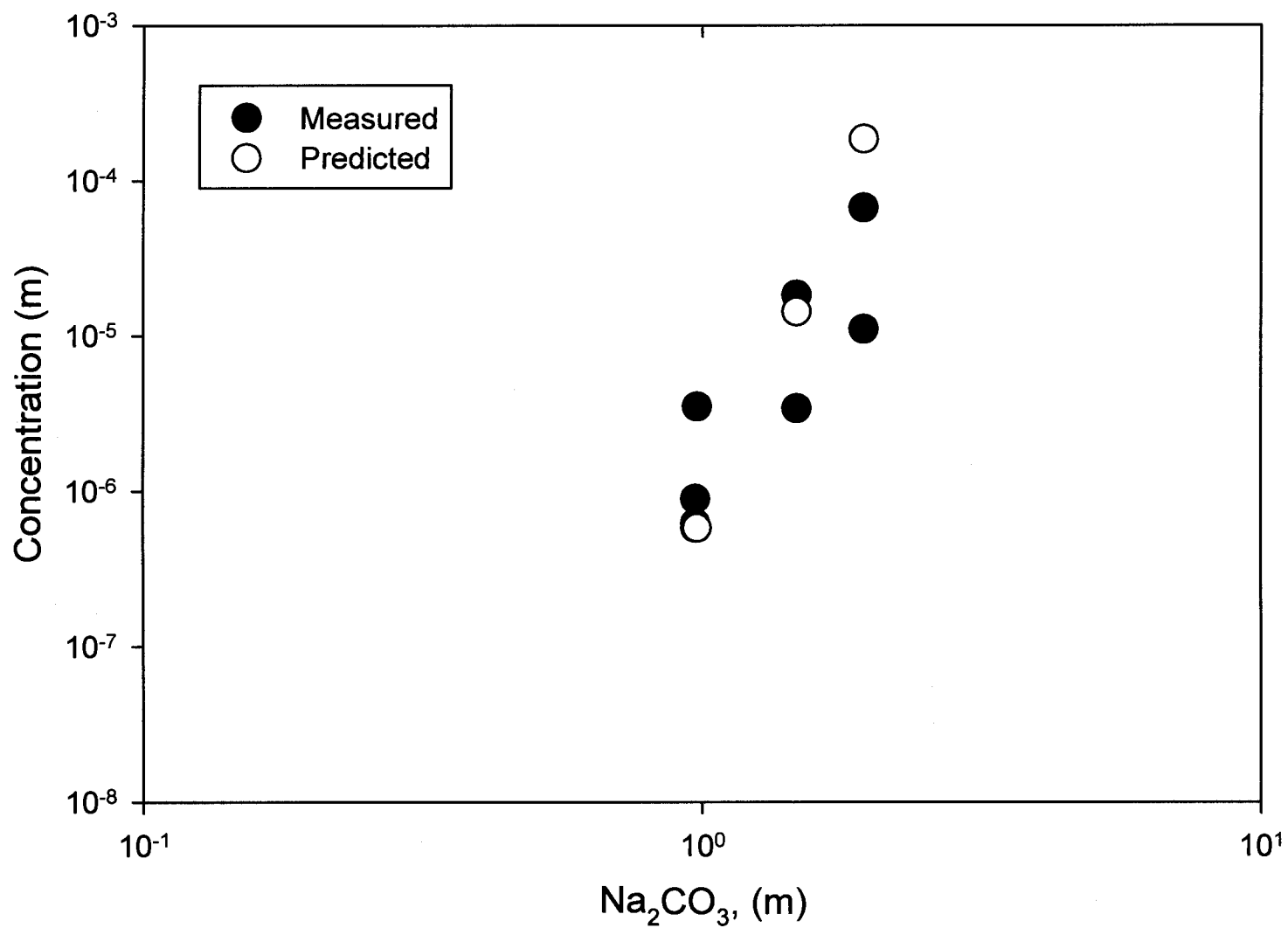
Figure 16. Comparison of the seven Th(IV) solubilities measured in solutions with I \geq 3 M (Rai et al., 1995, Figure 4) with those predicted by FMT (this analysis). The solutions used in these runs contained 1 \times 10^{-1} M NaOH had calculated pcH values of 12.36 to 12.52 (Table 20, this report).
