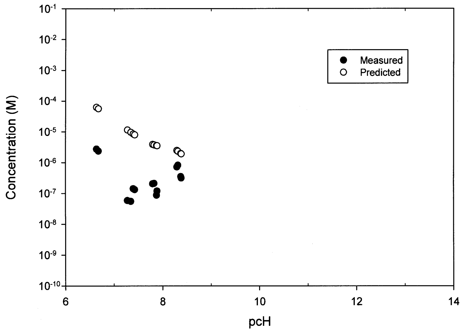
Figure 12. Comparison of the ^{14}\text{Nd(III)} solubilities measured in GWB with an initial \text{CO}_3^{2-} concentration of 1 \times 10^{-5} \text{ M} (Borkowski et al., 2009) with those predicted by FMT (Table 16, this report).
