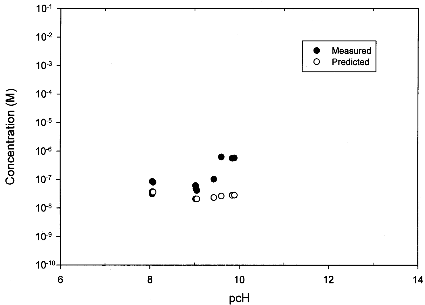
Figure 9. Comparison of the 12 Nd(III) solubilities measured in ERDA-6 with an initial \text{CO}_3^{2-} concentration of 1 \times 10^{-3} M (Borkowski et al., 2009) with those predicted by FMT (Table 13, this report).
