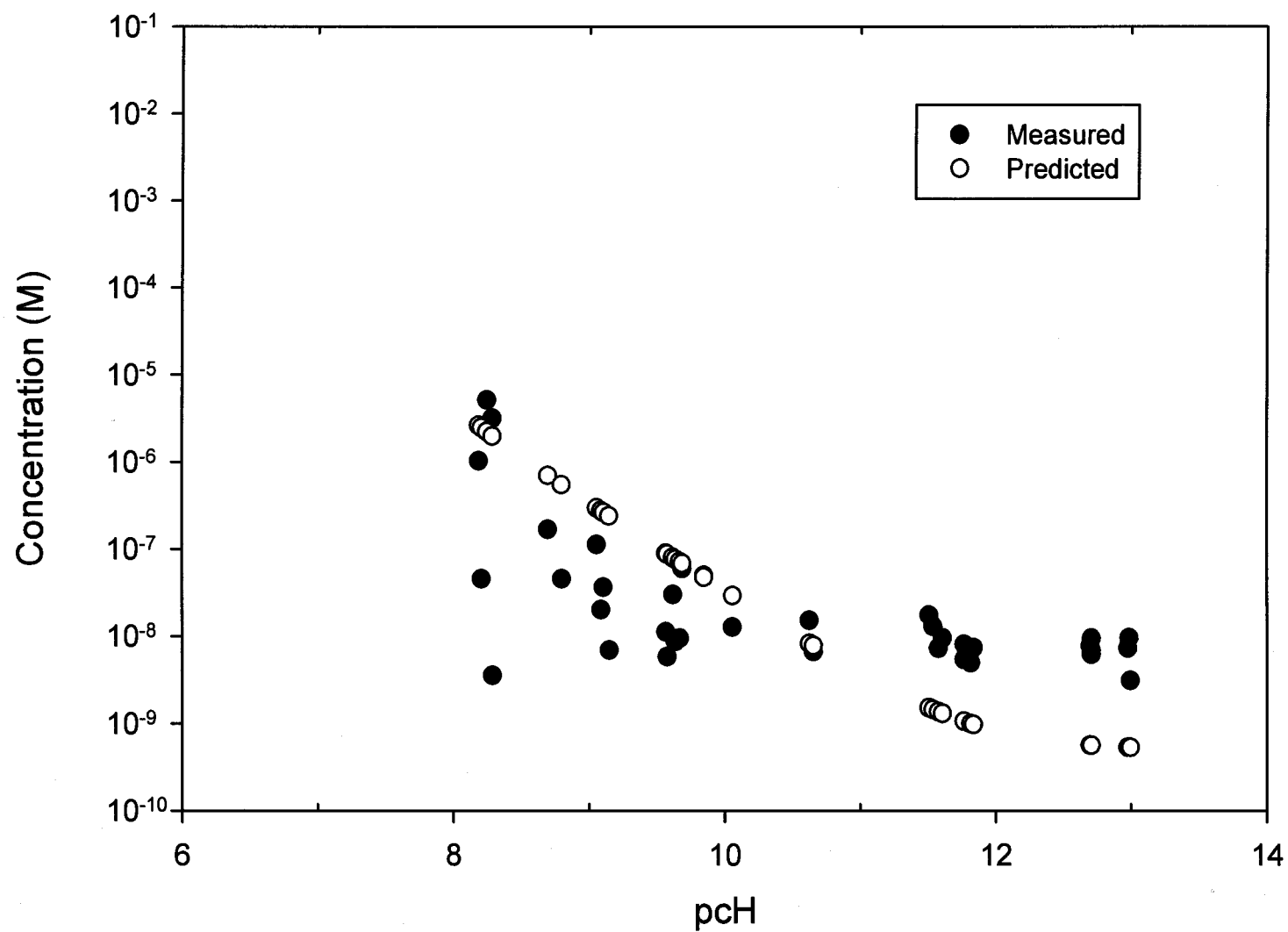
Figure 1. Comparison of the ^{36}\text{Nd(III)} solubilities measured in \text{CO}_3^{2-} -free 5 M NaCl (Borkowski et al., 2009) with those predicted by FMT (Table 5, this report).
