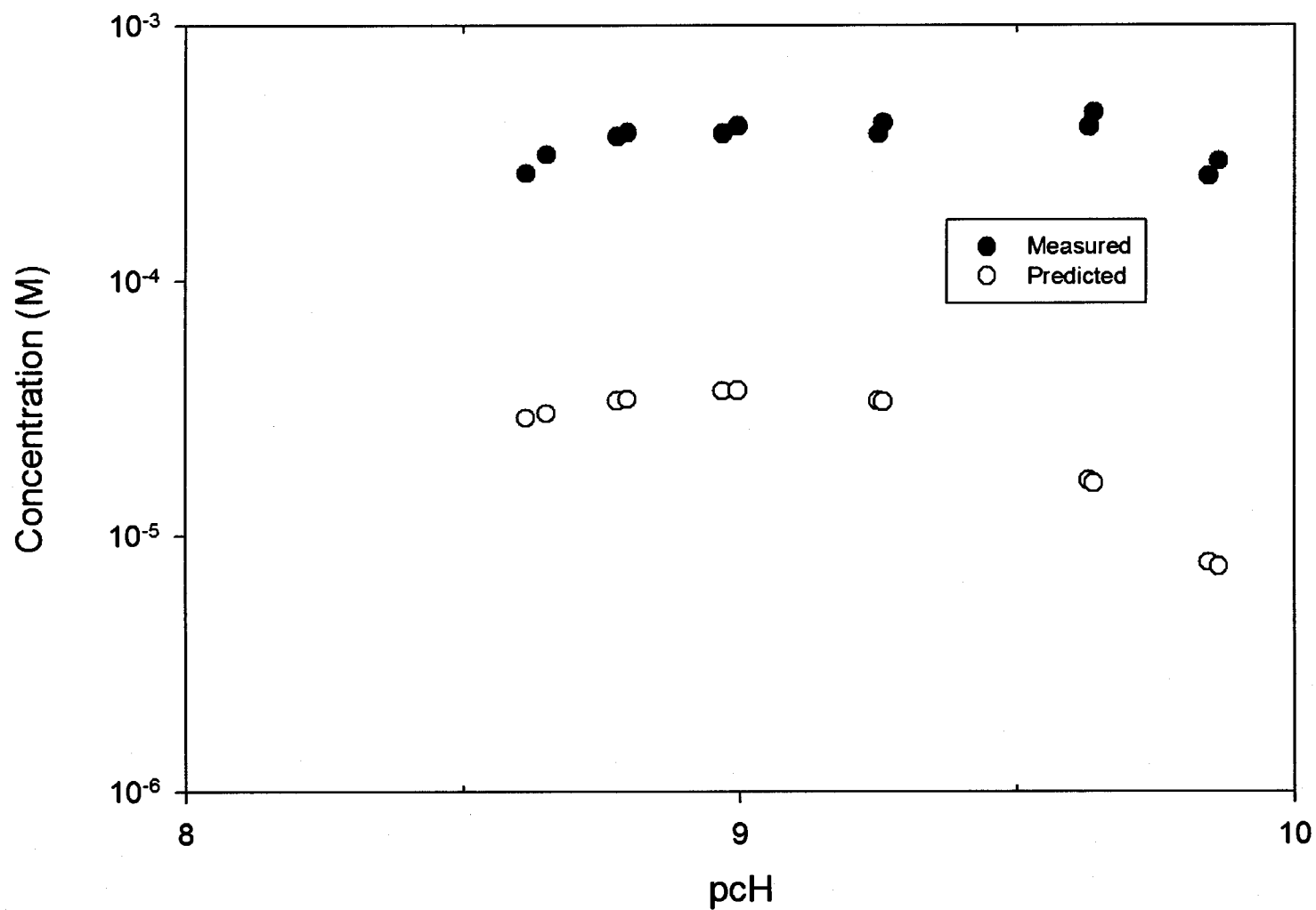
Figure 19. Comparison of the 12 Th(IV) solubilities measured in solutions with I \geq 3 M (Altmaier et al., 2006, Figure 2) with those predicted by FMT (this analysis). The solutions used in these runs contained 3.98 M NaCl and 0.02 M ( \text{NaHCO}_3 + \text{Na}_2\text{CO}_3 ), and had calculated pcH values of 8.61 to 9.86 (Table 23, this report).
