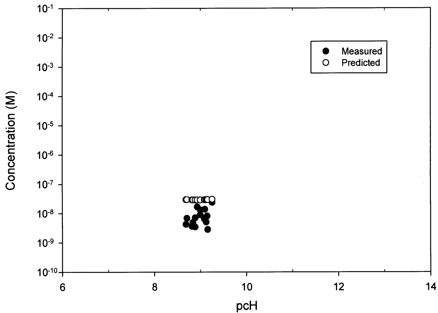
Figure 4. Comparison of the 16 Nd(III) solubilities measured in 5 M NaCl with an initial \text{CO}_3^{2-} concentration of 1 \times 10^{-3} M (Borkowski et al., 2009) with those predicted by FMT (Table 8, this report).
