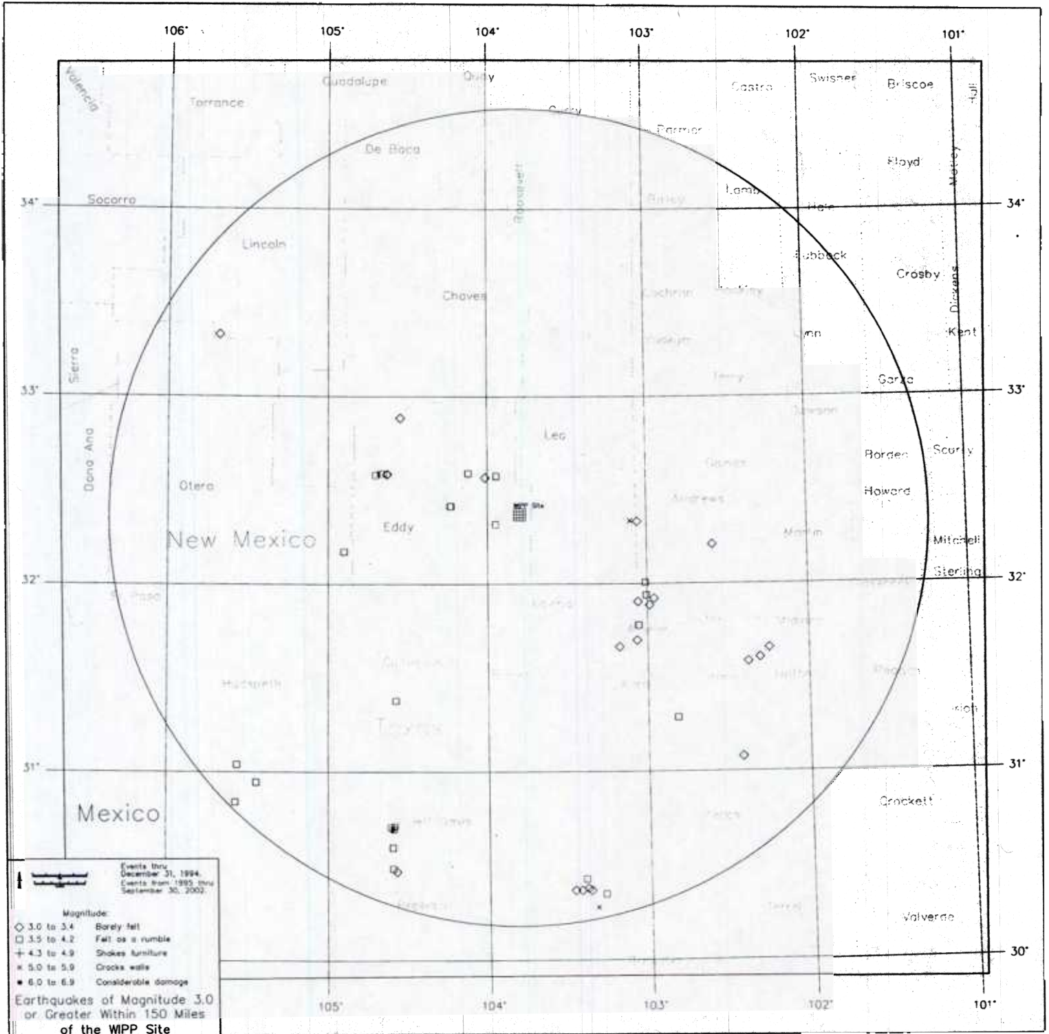
Figure 2-57. Seismic events with a magnitude greater than 3.0 within 150 miles of the WIPP site.
