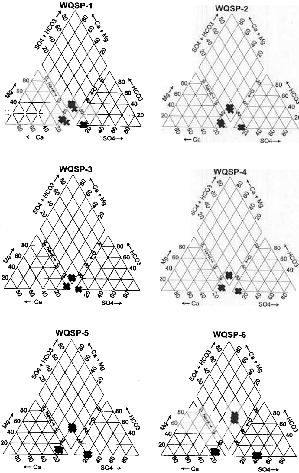
Figure 1. Piper diagrams for samples collected from WQSP wells from 1995 through 2002.
