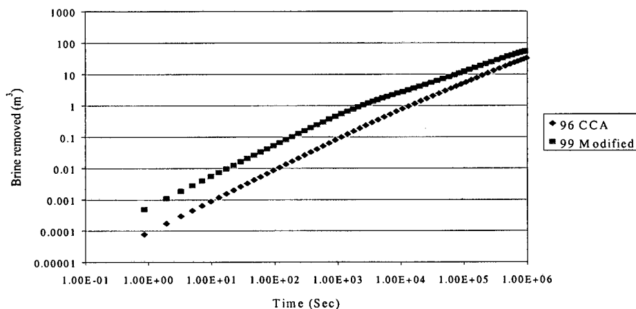
Fig. 6.5 Cumulative brine release vs. time predictions for both the 96 CCA and 99 modified calculations: logarithmic scale. (Down-dip, Replicate 1, Vector 46, Intrusion time 2000 years)
