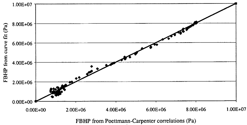
Fig. 4.2 Comparison of FBHP predictions from new curve fits and Poettmann-Carpenter correlations for brine dominated flow ( k_{rw} > k_{rg} ).
