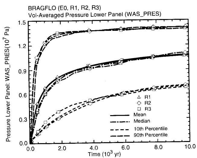
Fig. 7.4.2. Mean and percentile curves for three replicated LHSs for pressure in lower waste panel (WAS_PRES) under undisturbed conditions.
