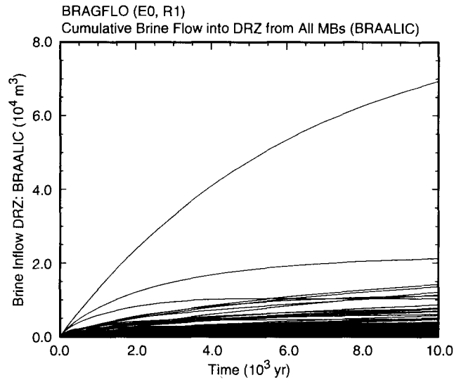
Fig. 6.10.5 Cumulative brine flow ( m^3 ) into disturbed rock zone (DRZ) from all anhydrite marker beds (MBs) under undisturbed (i.e., E0) conditions.
