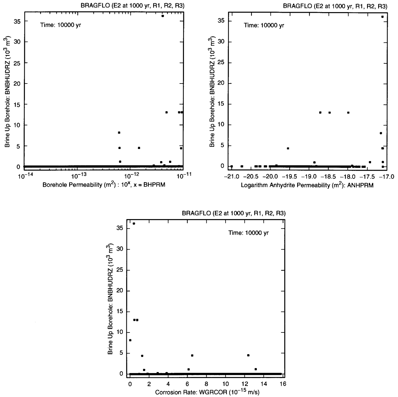
Fig. 8.6.4. Scatterplots for cumulative brine flow up borehole ( BNBHUDRZ ) over 10,000 yr for an E2 intrusion at 1000 yr into lower waste panel versus BHPRM , ANHPRM and WGRCOR .
