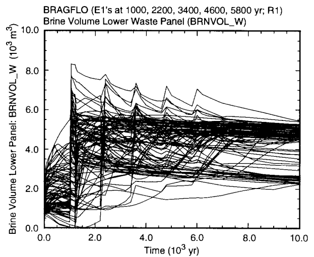
Fig. 8.11.4. Brine volume in upper ( BRNVOL_R ) and lower ( BRNVOL_W ) waste panels for multiple E1 intrusions into lower waste panel at 1000, 2200, 3400, 4600 and 5800 yr.
