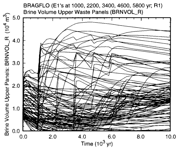
Fig. 8.11.4. Brine volume in upper ( BRNVOL_R ) and lower ( BRNVOL_W ) waste panels for multiple E1 intrusions into lower waste panel at 1000, 2200, 3400, 4600 and 5800 yr.
