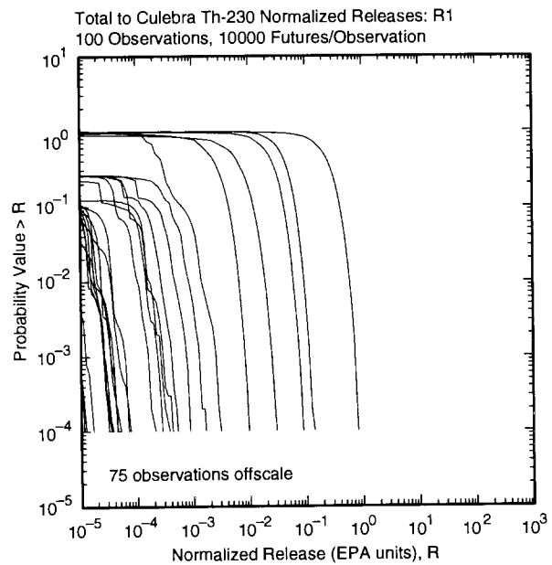
Fig. 11.2.4. Distributions of CCDFs for replicate R1 for normalized release of individual radionuclides (dissolved and colloiddally-transported) to Culebra Dolomite over 10,000 yr.
