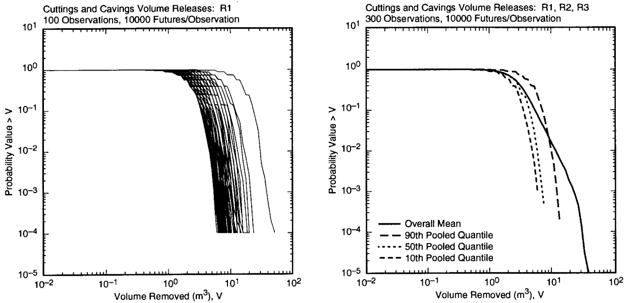
Fig. 9.2.5. Distribution of CCDFs for volume of material removed to accessible environment over 10,000 yr due to cuttings and cavings: CCDFs for replicate R1 (left frame), and mean and percentile curves obtained by pooling replicates R1, R2 and R3 (right frame).
