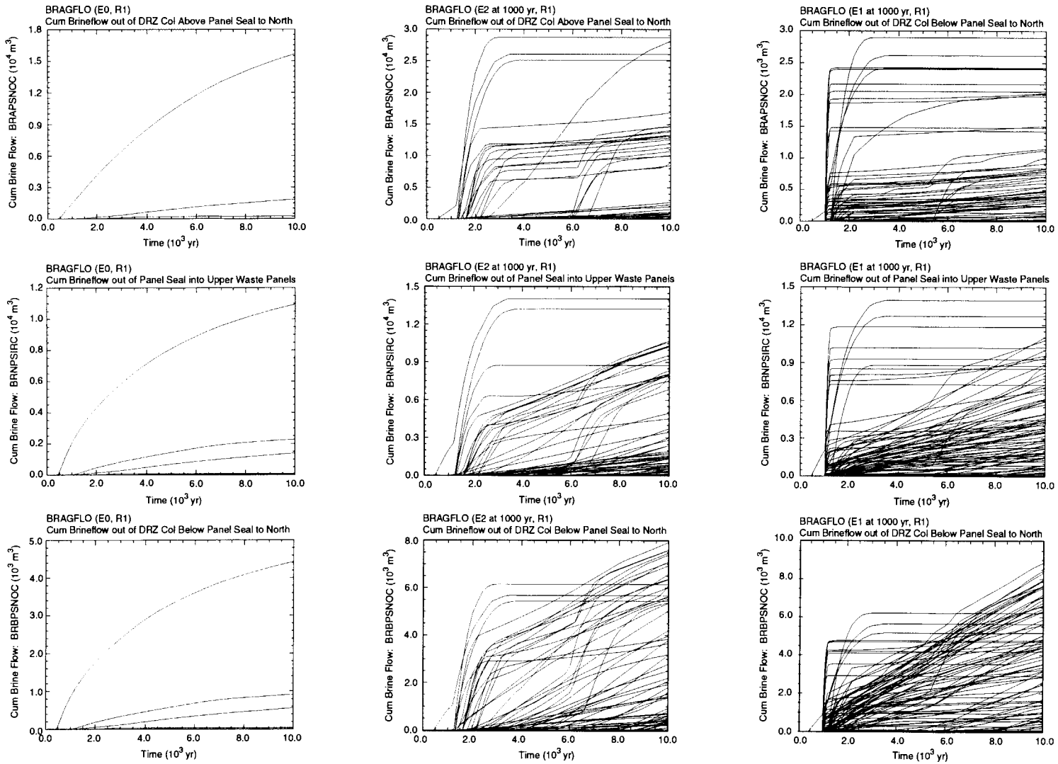
Fig. 8.9.2 Cumulative brine flow in repository and DRZ from south (i.e., downdip) end of repository to north (i.e., updip) end of repository ( BRAPSNOG , BRNPSIRC , BRBPSNOC ) for E0 (i.e., undisturbed) conditions (left column), an E2 intrusion at 1000 yr into the lower waste panel (middle column), and an E1 intrusion at 1000 yr into the lower waste panel (right column).
