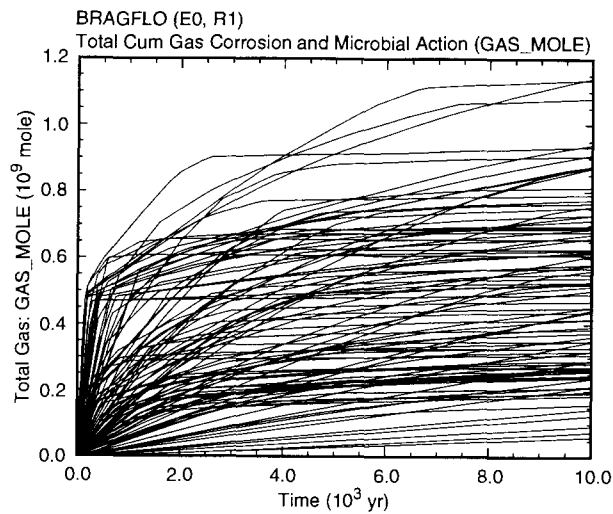
Fig. 7.3.4. Cumulative gas generation due to both corrosion and microbial degradation of cellulose ( GAS_MOLE ) under undisturbed conditions.
