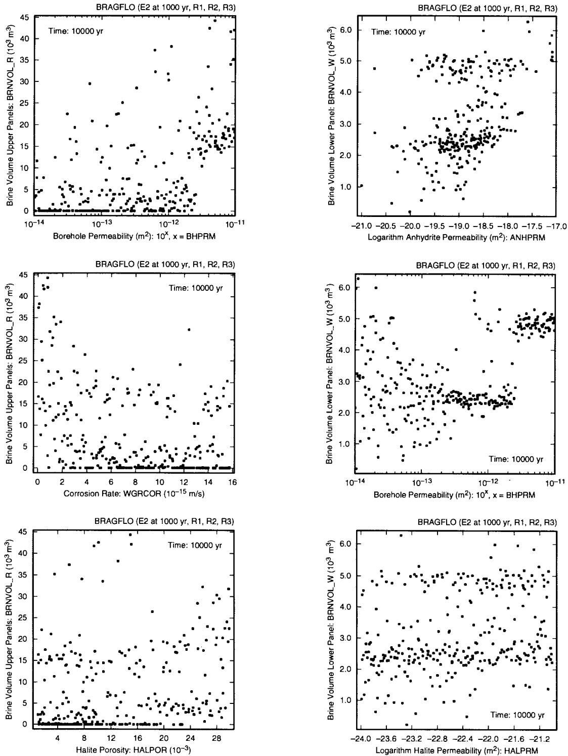
Fig. 8.5.7. Scatterplots for brine volume in upper waste panels ( BRNVOL\_R ) versus BHPRM , WGRCOR and HALPOR (left frames) and brine volume in lower waste panel ( BRNVOL\_W ) versus ANHPRM , BHPRM and HALPRM (right frames) at 10,000 yr for an E2 intrusion at 1000 yr into lower waste panel.
