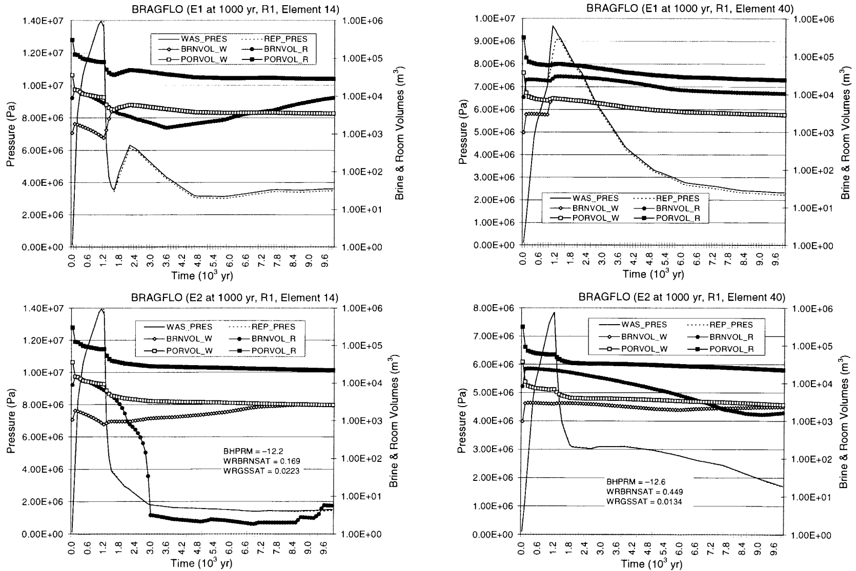
Fig. 8.6.9 Repository pressure ( REP\_PRES , WAS\_PRES ), pore volume ( PORVOL\_R , PORVOL\_W ) and brine volume ( BRNVOL\_R , BRNVOL\_W ) in upper and lower waste panels associated with E1 and E2 intrusions at 1000 yr into the lower waste panel for sample elements 14 and 40 of replicate R1.
