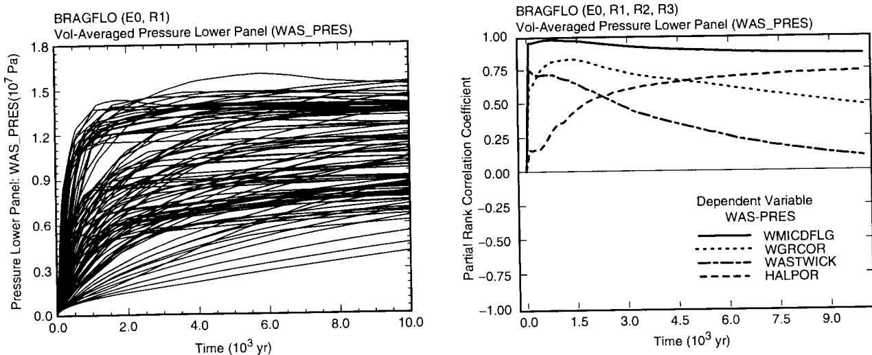
Fig. 7.4.1. Uncertainty and sensitivity analysis results for pressure in lower waste panel (WAS_PRES) under undisturbed conditions.
