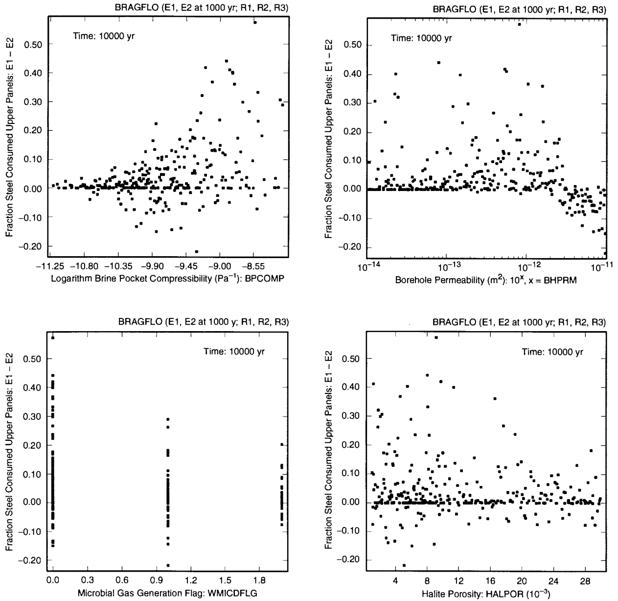
Fig. 8.3.14. Scatterplots for differences in fractions of steel consumed by corrosion in upper waste panels ( 1 - FEREM_R ) for E1 and E2 intrusions at 1000 yr into lower waste panel (i.e., Upper Waste Panels, (E1: 0 - 10,000 yr) - (E2: 0 - 10,000 yr) in Table 8.3.2) versus BPCOMP , BHPRM , WMICDFLG and HALPOR .
