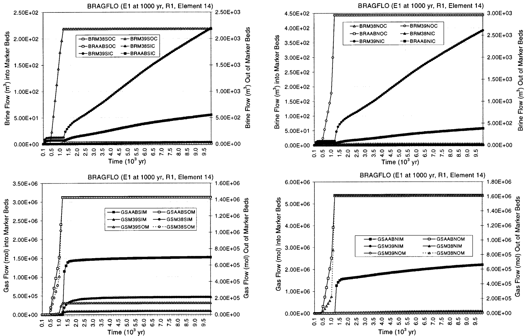
Fig. 8.7.2 Brine flow from marker beds to repository ( BRM38NIC, BRM39NIC, BRAABNIC, BRM38SIC, BRM39SIC, BRAABSIC ), brine flow from repository to marker beds ( BRM38NOC, BRM39NOC, BRAABNOC, BRM38SOC, BRM39SOC, BRAABSOC ), gas flow from marker beds to repository ( GSM38NOM, GSM39NOM, GSAABNOM, GSM38SOM, GSM39SOM, GSAABSOM ) and gas flow from repository to marker beds ( GSM38NIM, GSM39NIM, GSAABNIM, GSM38SIM, GSM39SIM, GSAABSIM ) for an E1 intrusion at 1000 yr into the lower waste panel and sample element 14 of replicate R1.
