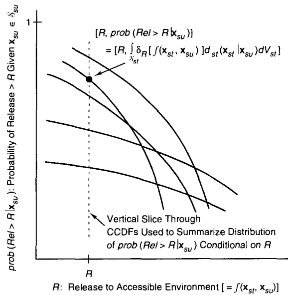
Fig. 2.4.1. Distribution of CCDFs resulting from possible values for \mathbf{x}_{su} \in \mathcal{S}_{su} .
