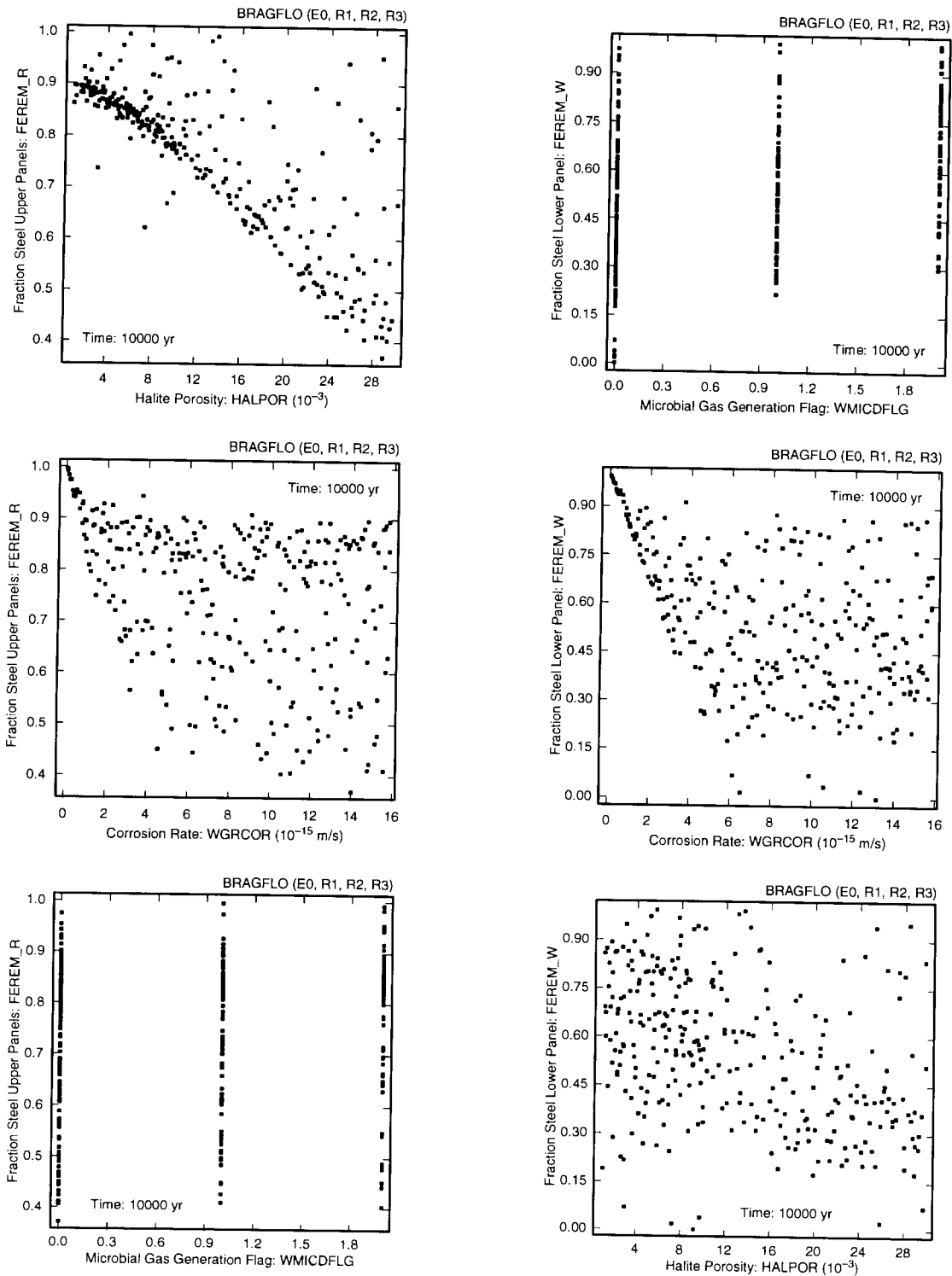
Fig. 7.3.10. Scatterplots for fraction of steel remaining in upper waste panels ( FEREM\_R ) (left frames) and lower panel ( FEREM\_W ) (right frames) for undisturbed conditions at 10,000 yr versus HALPOR, WGRCOR and WMICDFLG.
