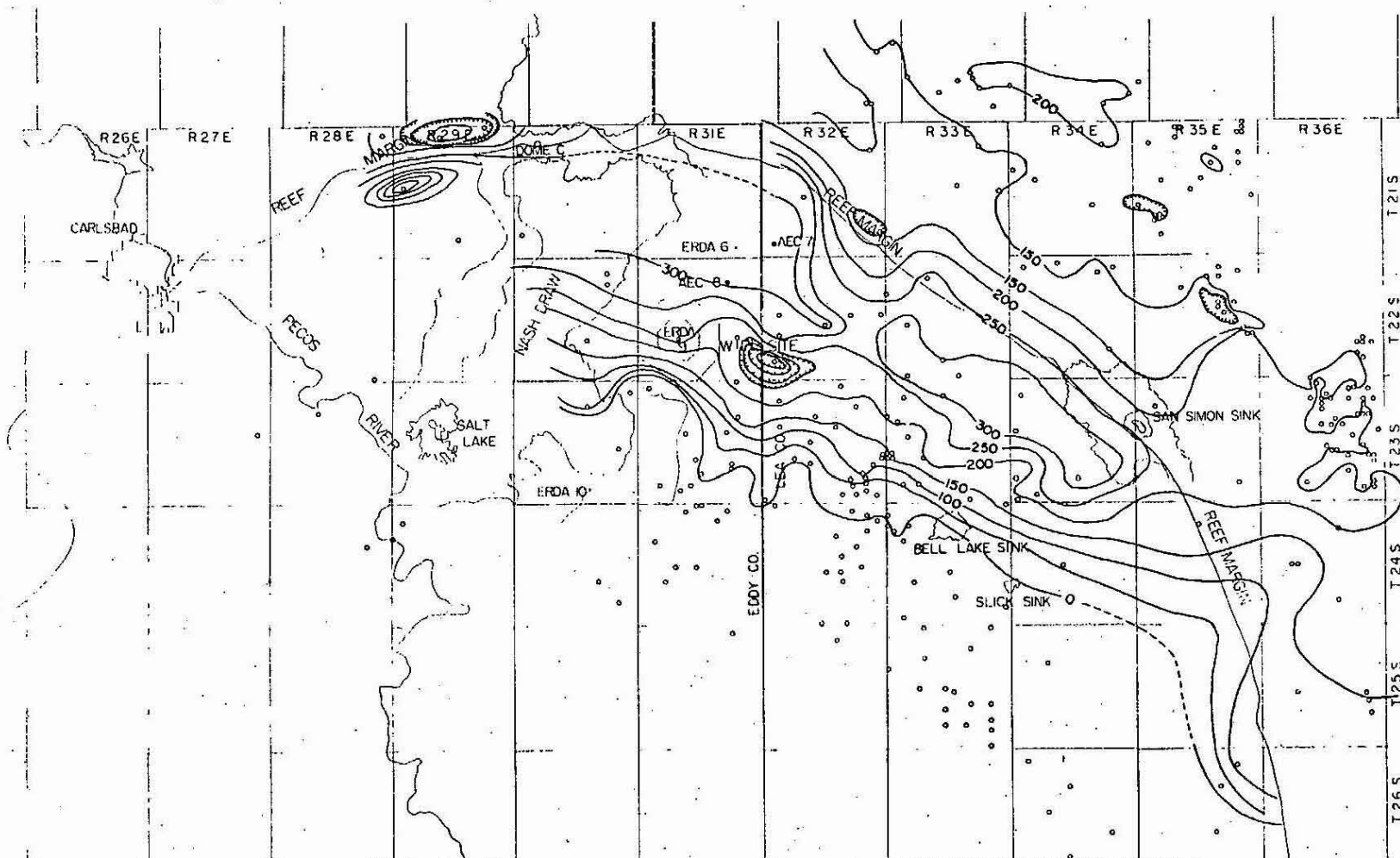
Figure 7 INFRACOWDEN SALT ISOPACH CONTOUR INTERVAL 50 ft (15.2m)
