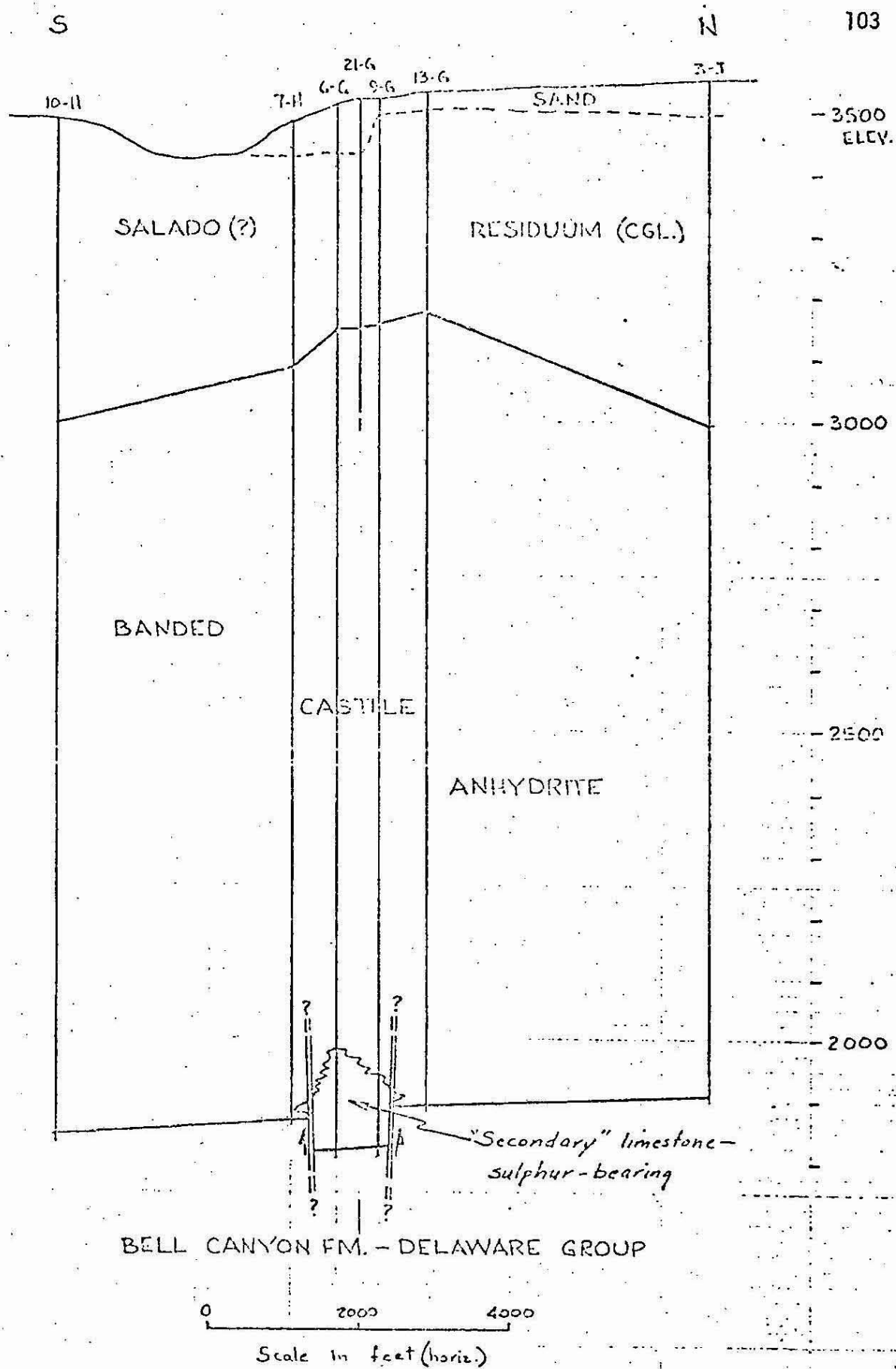
North-south cross-section through Texas Gulf Sulphur Rustler Springs deposit, PSL Blk 110
