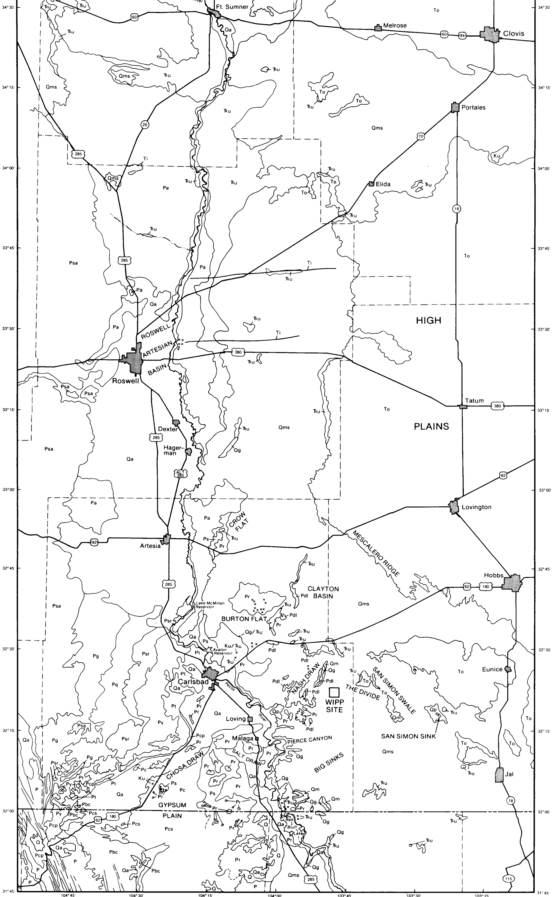
Figure 2. Geologic map of southeastern New Mexico
