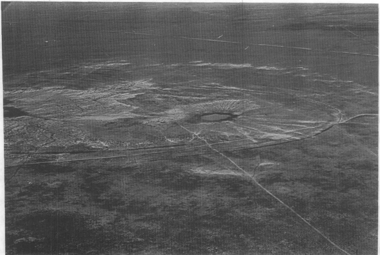
Figure 16. Aerial view of San Simon Sink, Lea County, NM. (Annular rings are visible cutting the surface around the sink. An exploratory hole (WIPP 15) was drilled to a depth of 810 ft (249 m) in the center of the sink. The upper 555 ft (168 m) consisted of Quaternary sands and clays. The lower 255 ft (78 m) was drilled in Triassic rocks).
