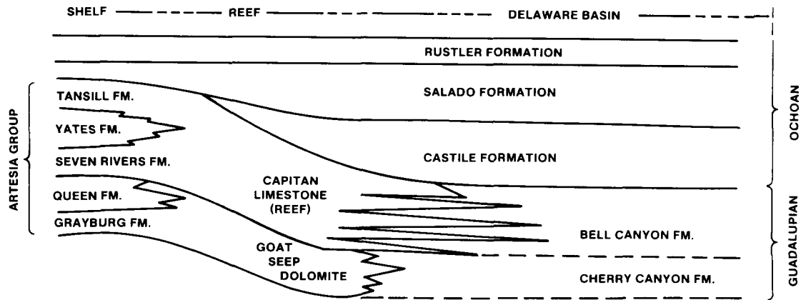
Figure 4. Diagram showing stratigraphic relationships of Permian rocks along the northern boundary of the Delaware Basin
