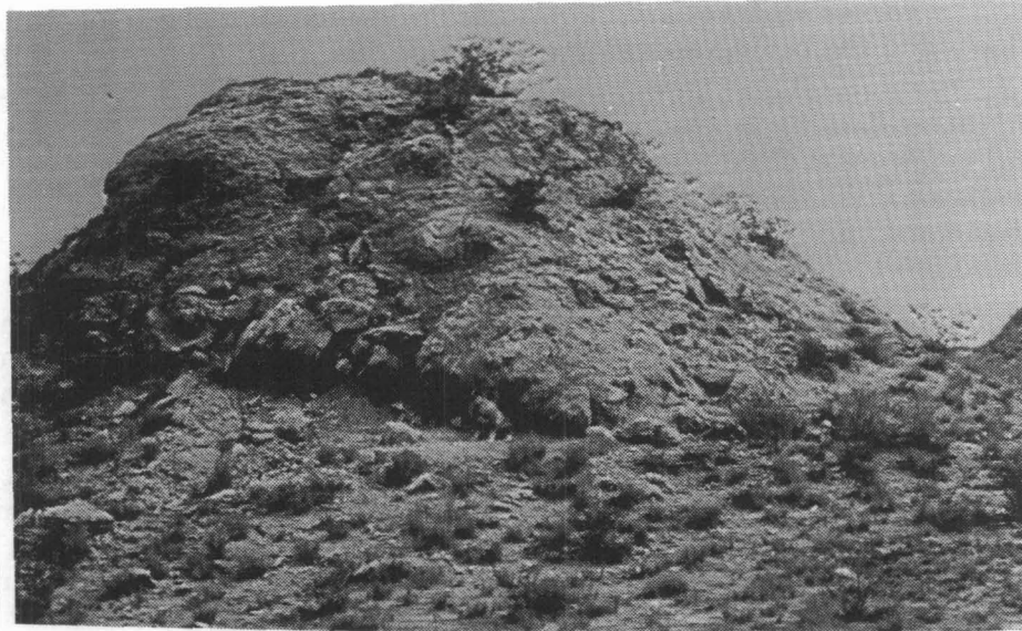
Figure 22. Karst mound. (Erosional remnant of chaotic blocks of gypsum and dolomite, intermingled with silt and clay. Mounds vary in form from conical to ovate. They are common features along the banks of the Pecos River in the southern part of Eddy County, NM, where the Rustler Formation is exposed. The mound in this photograph is ~20 ft (6 m) high and is one of several distinctly visible on aerial photographs.)
