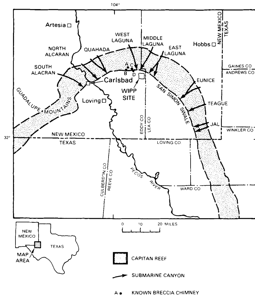
Figure 3. Index map showing location of the Capitan reef and its submarine canyon deposits relative to political boundaries. (Generalized from Hiss, 1975, Figure 11.)
