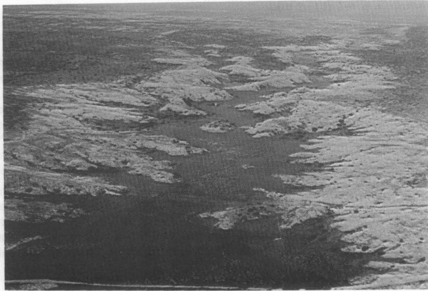
Figure 20. Aerial view of solution-subsidence trough, Gypsum Plain, southern Eddy County, NM. (This trough is ~2 mi (3.2 km) long and ~0.5 mi (0.8 km) wide at the widest part. The light areas on either side of the trough are massive gypsum of the Castile Formation.)
