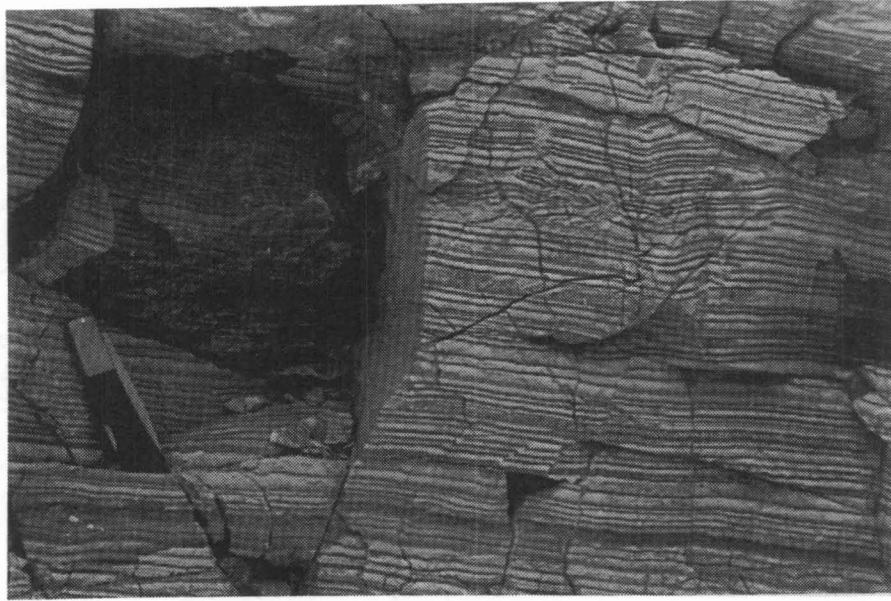
Figure 5. View of laminated gypsum in road cut, Castile Formation, Culberson County, TX. (The open fractures are typical of relatively unweathered near-surface gypsum. In nearby weathered exposures, fractures are filled with earthy gypsite.)
