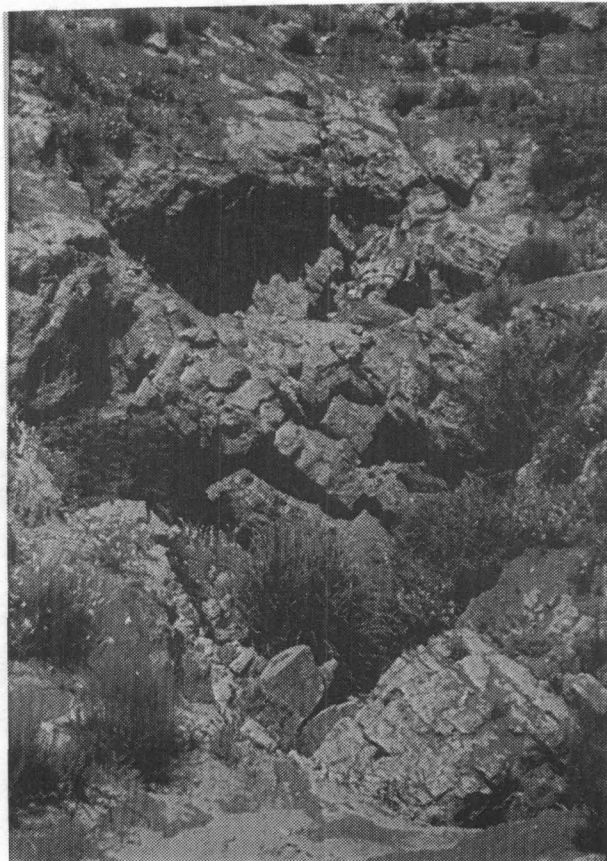
Figure 13. Gypsum and dolomite, Rustler Formation, in a collapse sink, Burton Flat, Eddy County, NM. (Rocks at the surface have collapsed into a cave that was dissolved along a fracture system. The collapse sink is linear in plan and may be followed on the surface for ~100 m. See Figure 14.)
