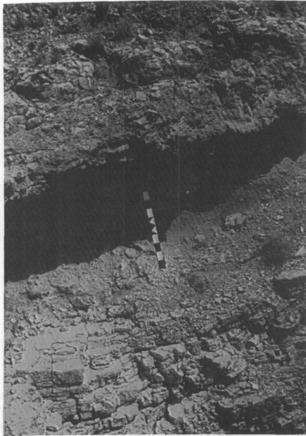
Figure 7. Photograph showing the resistant beds of the Culebra and Magenta Members of the Rustler Formation in outcrops ~12 mi (20 km) east of Artesia, Eddy County, NM (NE 1/4 Sec. 15, T.17S., R.28E.). (At this locality the intervening Tamarisk Member is represented by <5 ft (1.5 m) of insoluble residue (clay and silt). In complete undissolved stratigraphic sections in the subsurface to the southeast, the Tamarisk averages 80 to 100 ft (25 to 30 m) in thickness and consists of anhydrite or gypsum, halite, and clay. The scale is 1 m.)
