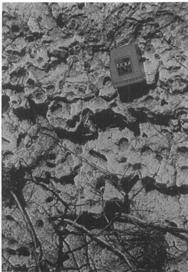
Figure 21. Scallops on the top surface of gypsum in the Rustler Formation, Burton Flat, Eddy County, NM. (At this locality the beds are nearly horizontal.)
