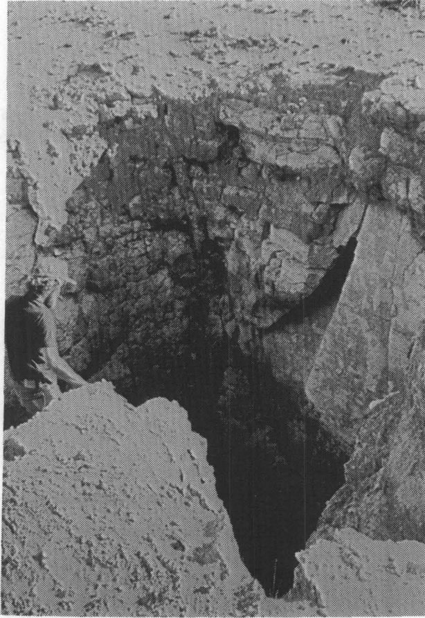
Figure 18. Collapse sink in upper part of the Rustler Formation, Nash Draw, Eddy County, NM, showing nearly vertical fractures in bedded gypsum. (More than 75 collapse sinks in various stages of formation have been observed in Nash Draw. Many of these sinks are entrances to caves.)
