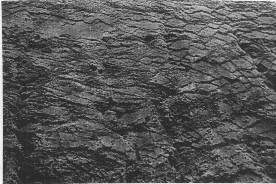
Figure 10. Aerial view of fracture (joint) pattern in gypsum on surface adjacent to collapse sink ~2 mi (3 km) south of Bottomless Lakes State Park, Chaves County, NM. (The fractures are ~3 to 10 ft (1 to 3 m) apart. Grasses grow in the fractures.)
