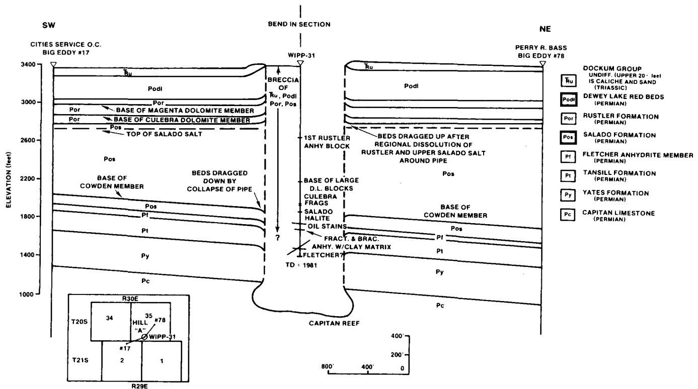
Figure 25. Southwest to northeast cross section through Hill A (after Snyder and Gard, 1982, Figure 10)
