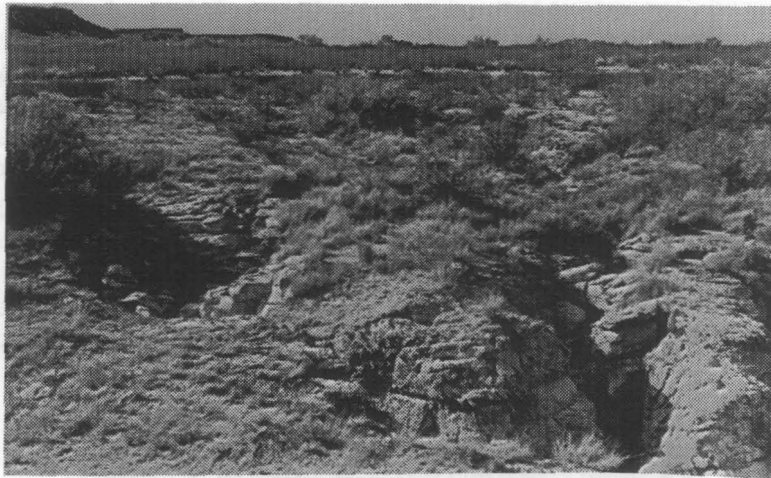
Figure 14. Collapse sinks along fractures, Nash Draw, Eddy County, NM. (Scarp in middle ground is on fan surface. See Figure 13). Livingston Ridge, capped by Mescalero caliche, is in background to left of the photograph).
