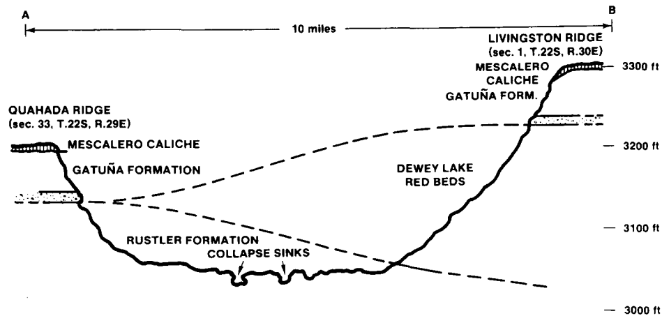
(a) Diagrammatic cross-section of Nash Draw showing stratigraphic relations of Gatuña Formation and evaporites in the Rustler Formation. (The vertical scale is greatly exaggerated).
