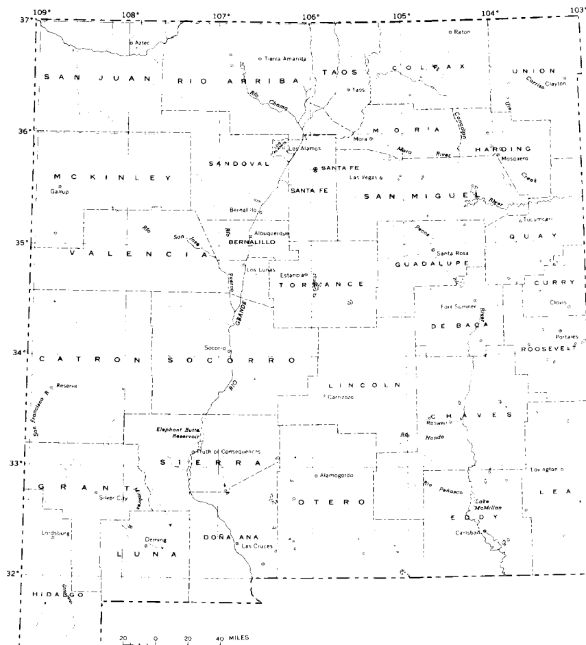
Figure 1. Index map of new Mexico showing the area of Figure 2, the area discussed in this report ( Figure 2 is a foldout on page 75 of this report )
