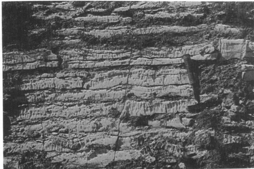
Figure 6. Fluting in horizontal beds of massive gypsum, Castile Formation, Gypsum Plain, Culberson County, TX. (The exposure is in the wall of an arroyo that drains into a cave.)
