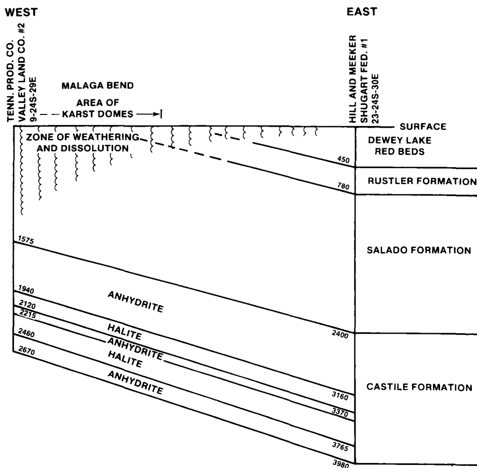
Figure 28. Diagram showing stratigraphic relationships in southeastern Eddy County, NM, where karst domes are located. (Regional dip is to the east. The eroded edges of the Salado and Rustler Formations are exposed at the surface in the vicinity of Malaga Bend, where they consist of discontinuous beds in breccia and residuum. Numbers beside drill holes indicate depth, in feet, from the surface.)
