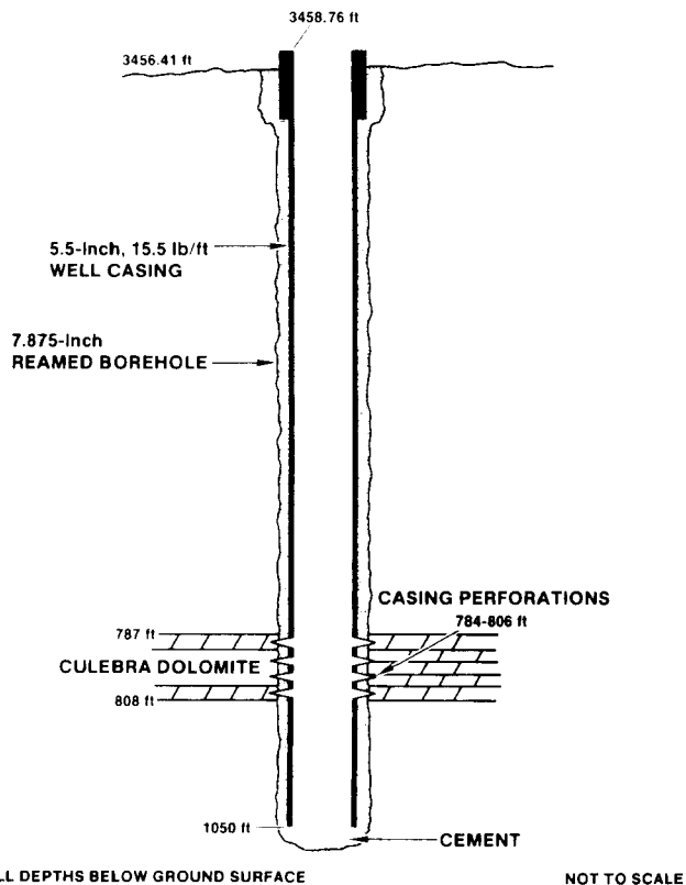
Figure 3-5. Well Configuration for WIPP-18
