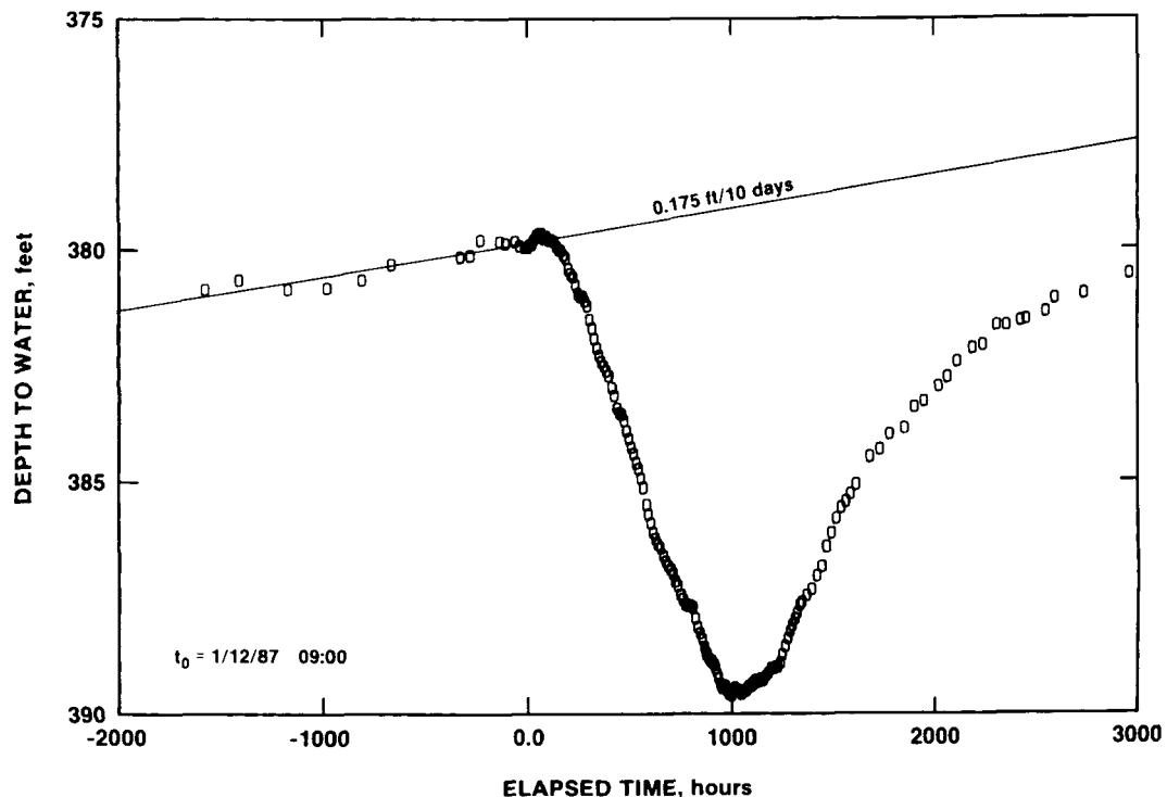
Figure 5-8. WIPP-30 Water-Level Record
