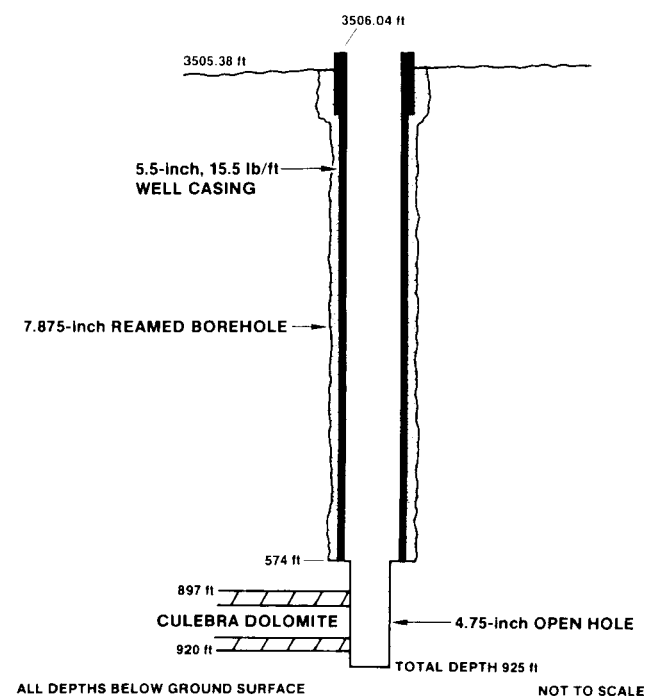
Figure 3-14. Well Configuration for H-5b
