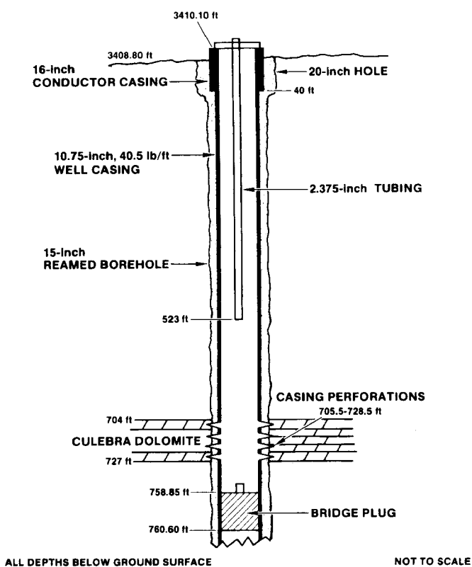
Figure 3-4. Well Configuration for ERDA-9
