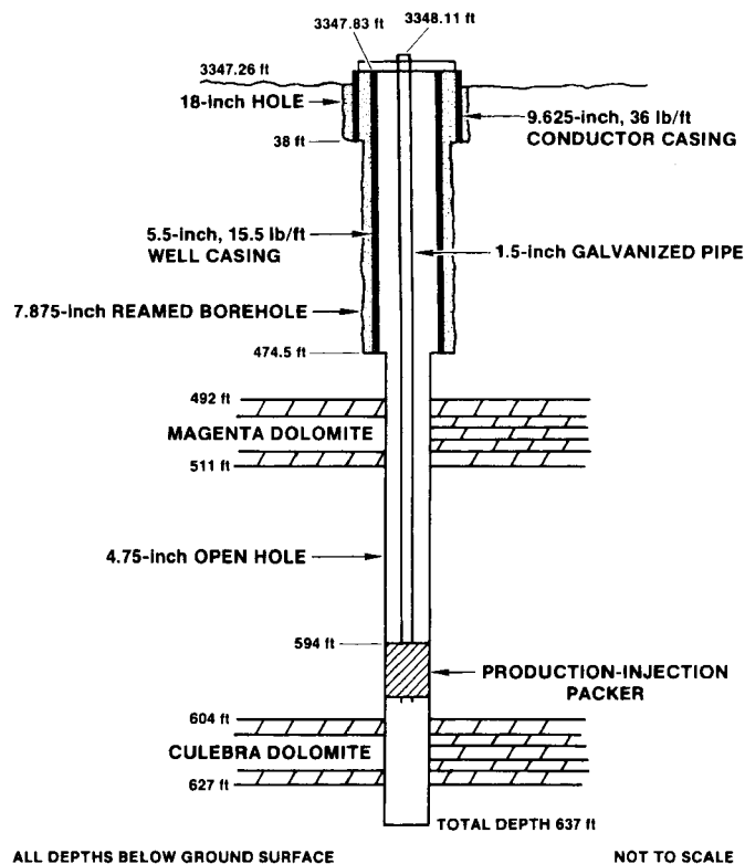
Figure 3-17. Well Configuration for H-6a
