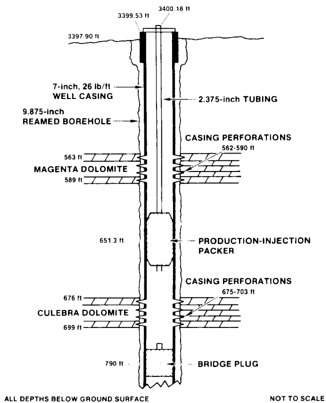
Figure 3-11. Well Configuration for H-1
