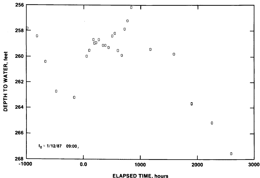
Figure 5-20. H-1 Magenta Water-Level Record
