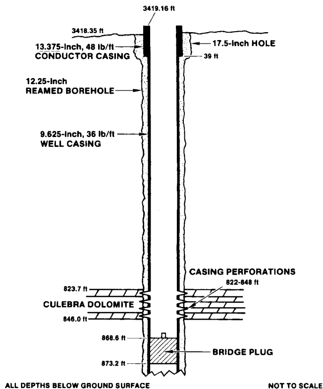
Figure 3-3. Well Configuration for DOE-2
