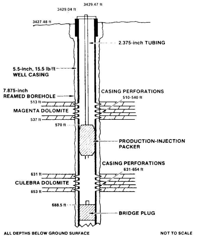
Figure 3-10. Well Configuration for WIPP-30
