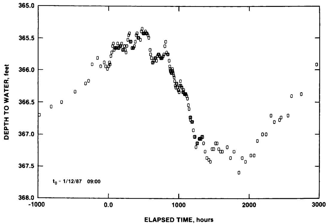
Figure 5-10. H-2b2 Water-Level Record
