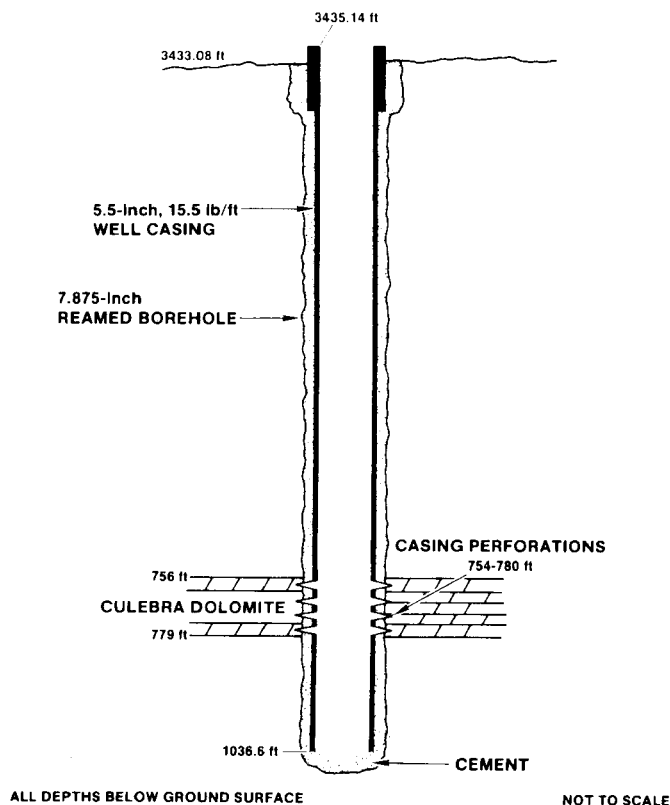
Figure 3-6. Well Configuration for WIPP-19
