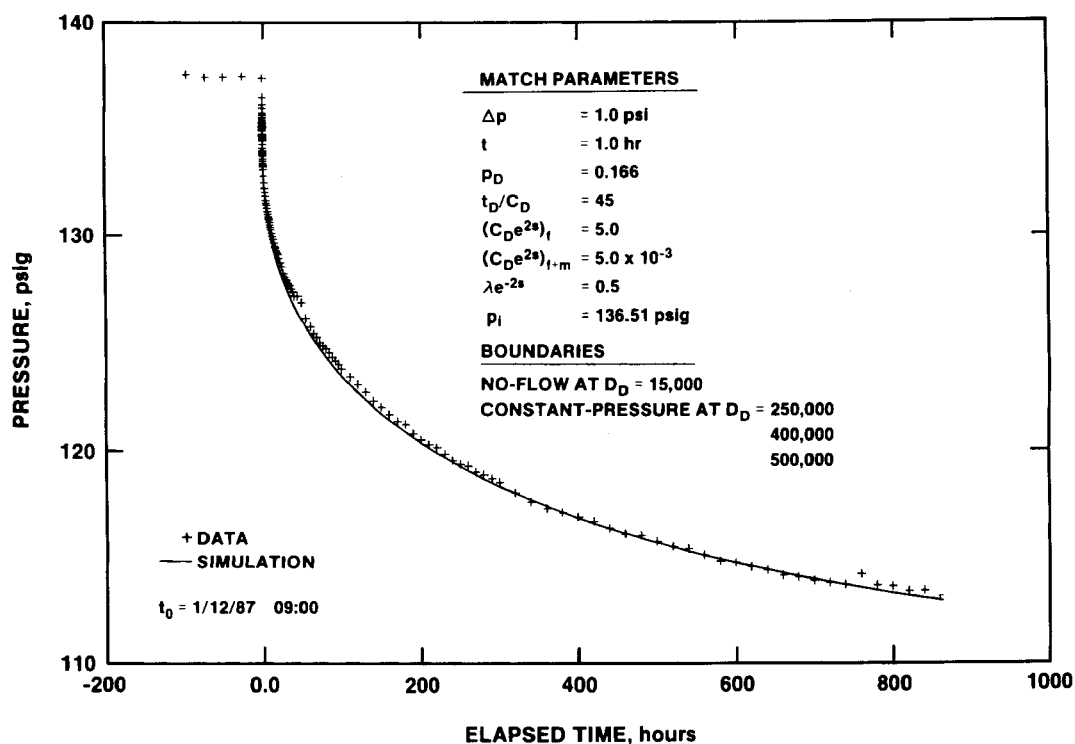
Figure 6-3. WIPP-13 Drawdown Linear-Linear Sequence Plot With INTERPRET Simulation
