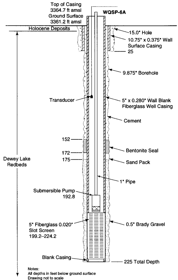
Figure 3-29. Configuration of WQSP-6A during the 1996 pumping test.
