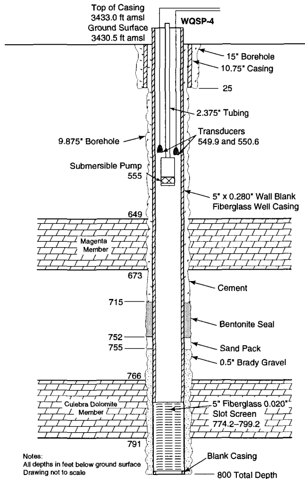
Figure 3-26. Configuration of WQSP-4 during the 1995 pumping test.
