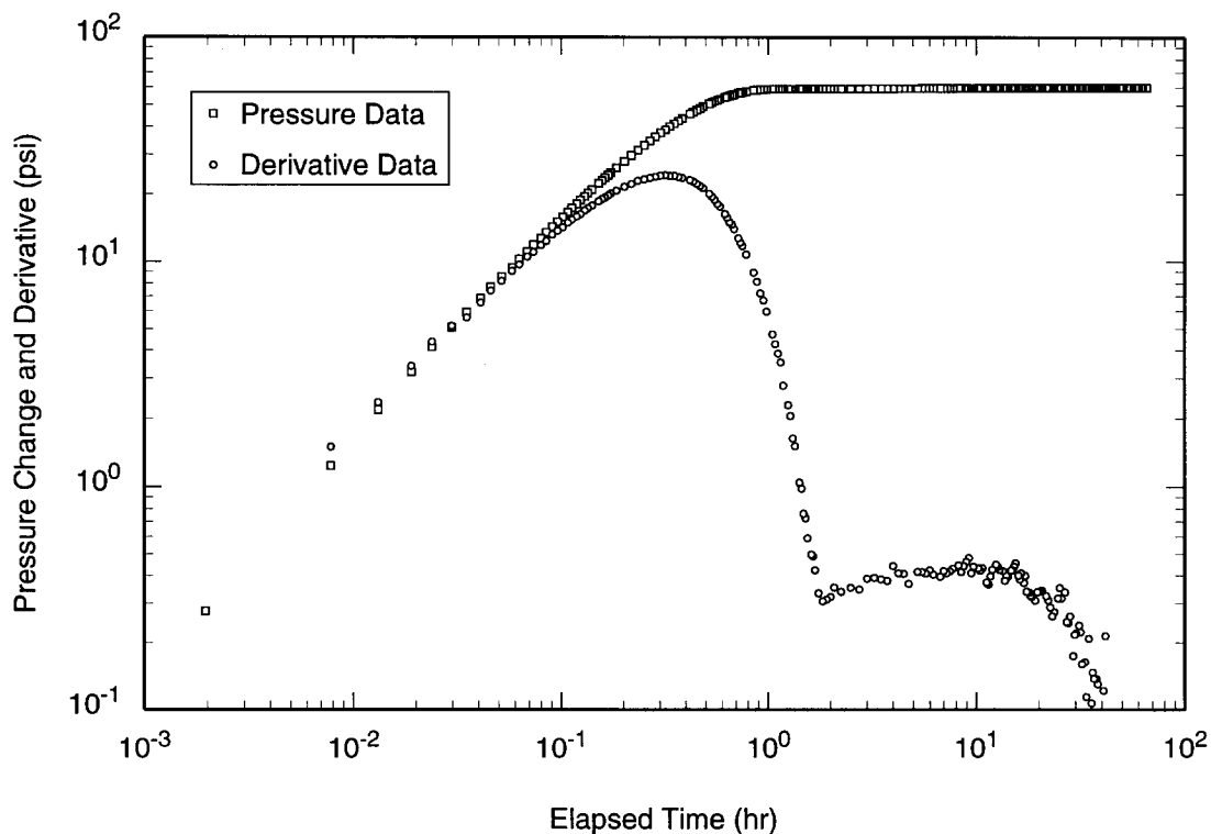
Figure 6-41. Log-log diagnostic plot of H-9c recovery data from test #1.
