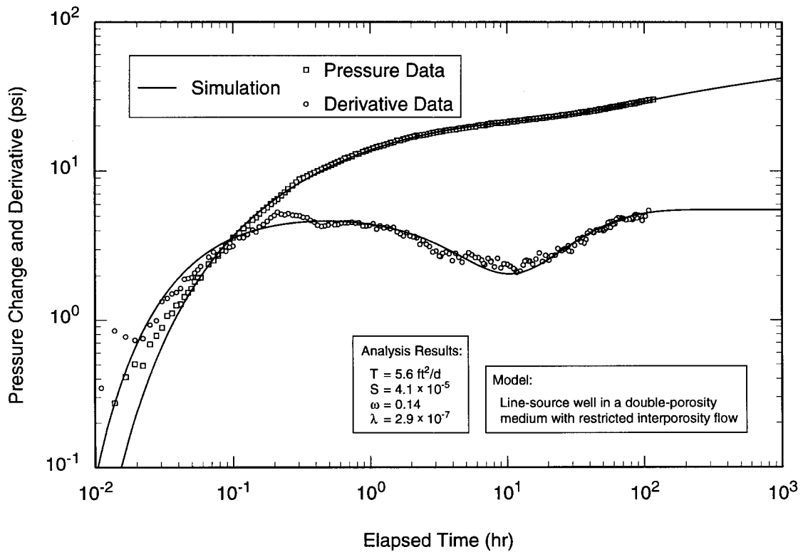
Figure 6-84. Log-log plot of H-19b2 drawdown data with Interpret/2 simulation.
