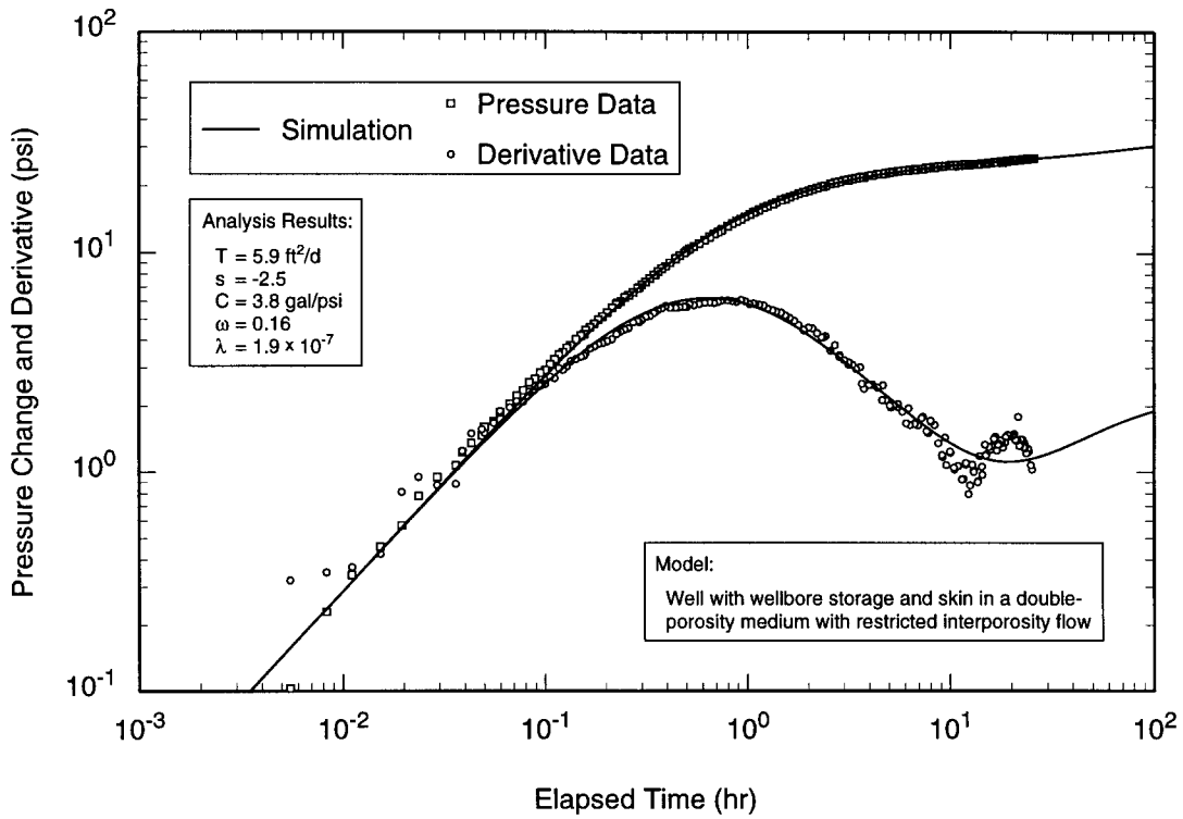
Figure A-40. Log-log plot of H-19b2 drawdown data from the second pumping period with Interpret/2 simulation.
