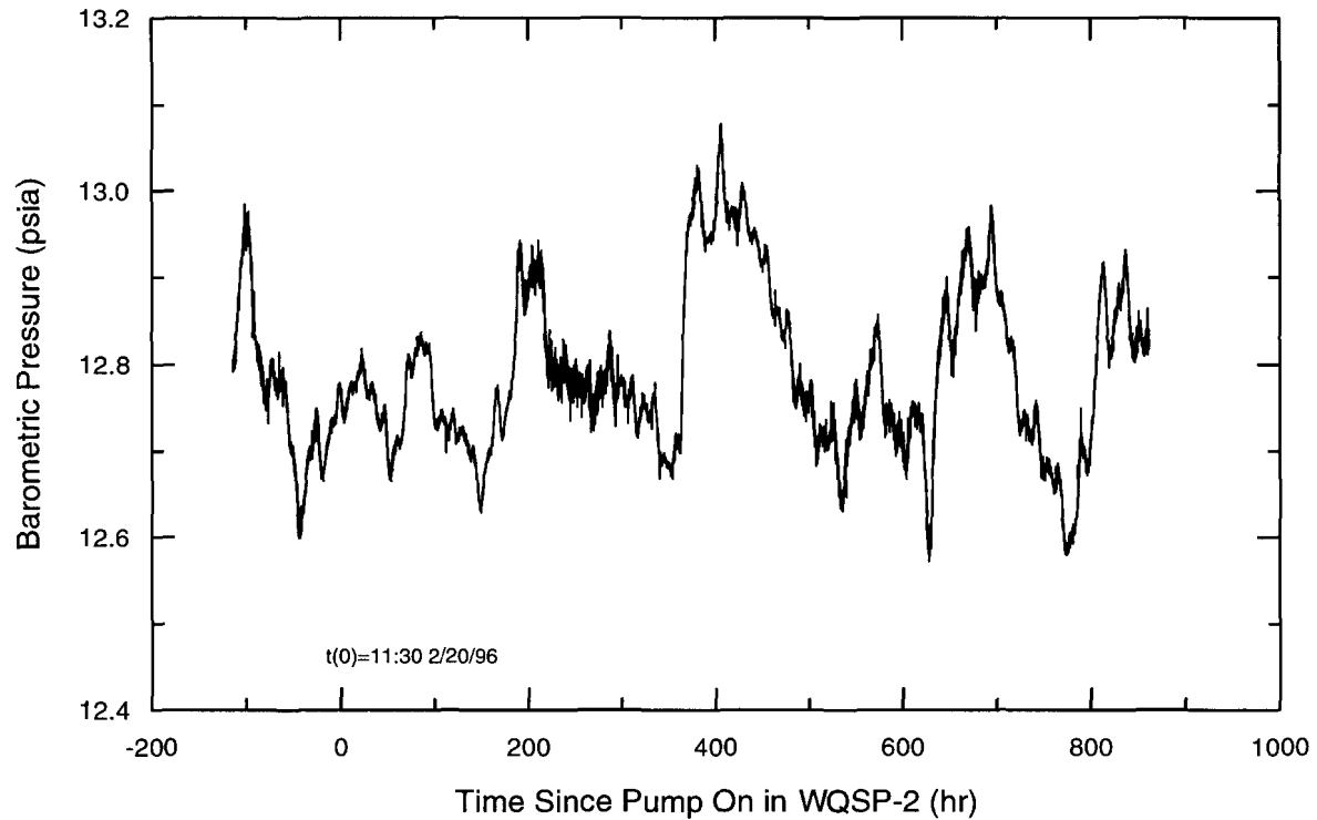
Figure 5-41. Barometric pressure during the WQSP-2 pumping test.
