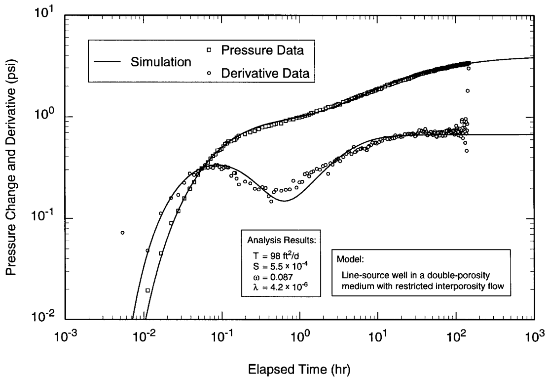
Figure 6-51. Log-log plot of H-9c recovery data from test #2 with Interpret/2 simulation.
