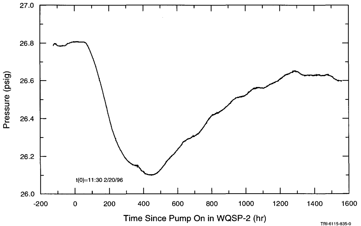
Figure 5-38. Pressure in WIPP-12 during the WQSP-2 pumping test.
