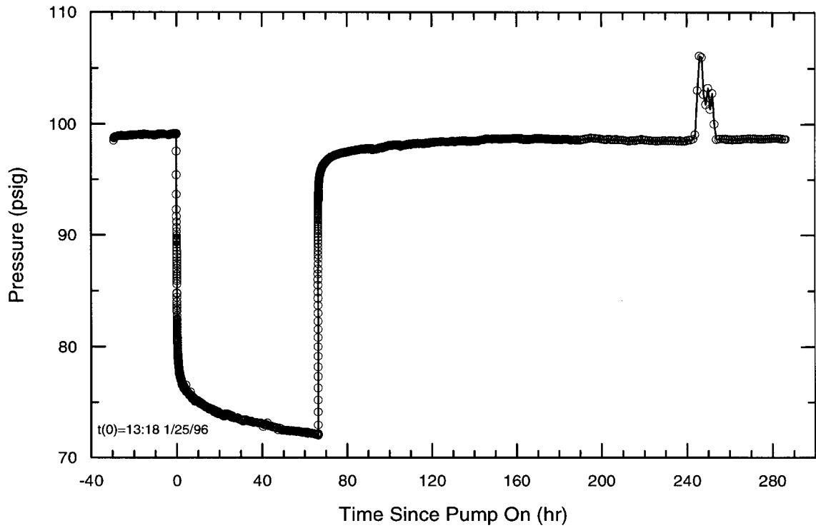
Figure 5-30. Pressure in WQSP-1 during the WQSP-1 pumping test.
