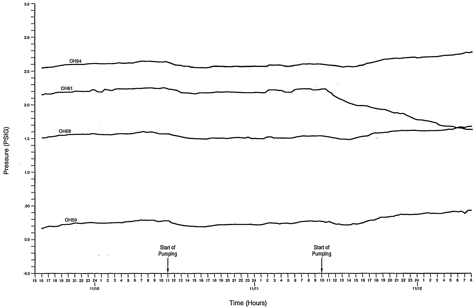
Figure E-5-11 Hydrographs of the W170 Site Testholes OH59, OH61, OH64, and OH68 Through the End of the Pumping Test, November 1992
