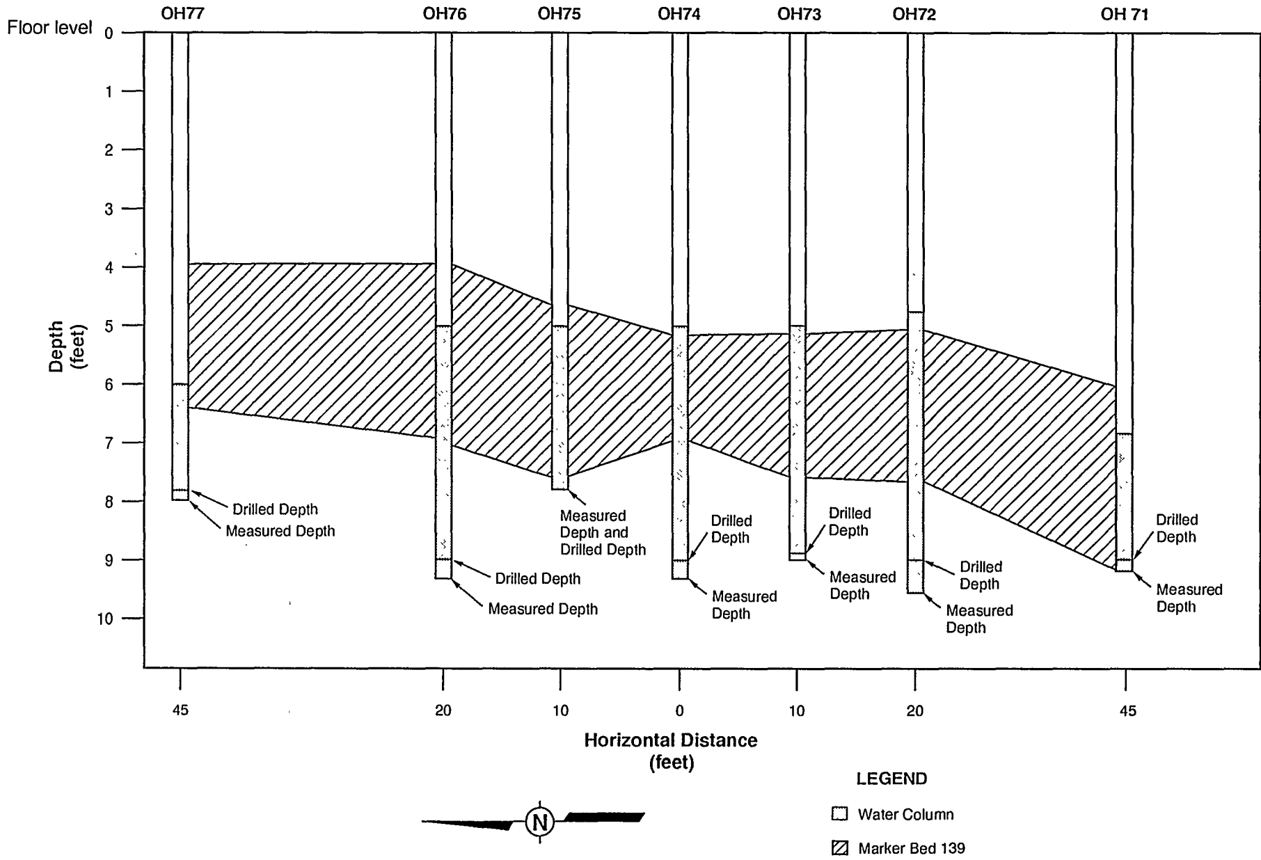
Figure E-4-1 Cross Section of Boreholes Along the E0 Drift Test Site, October 1992
