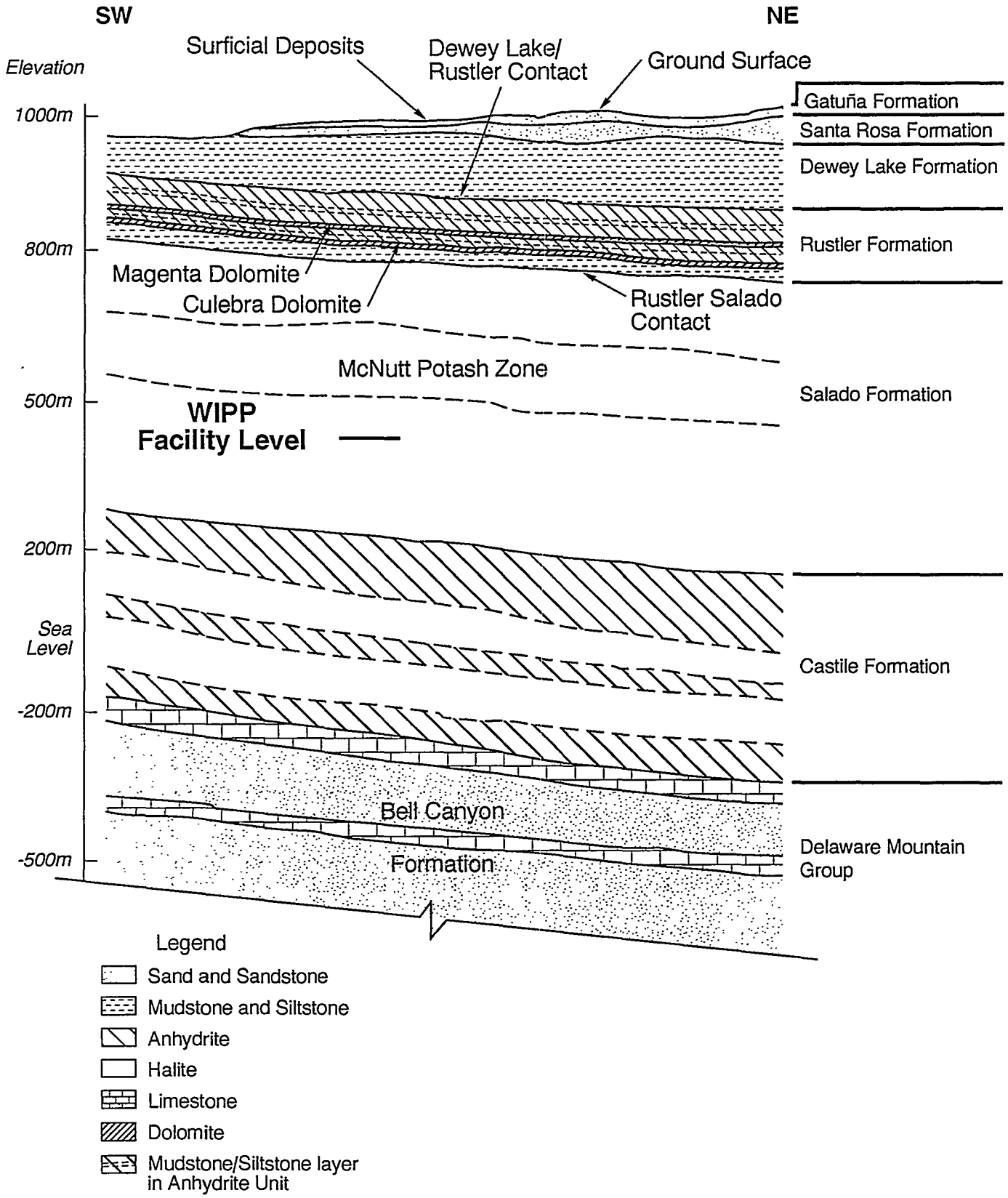
Figure 1-3 Generalized Stratigraphic Cross Section of the WIPP Site
