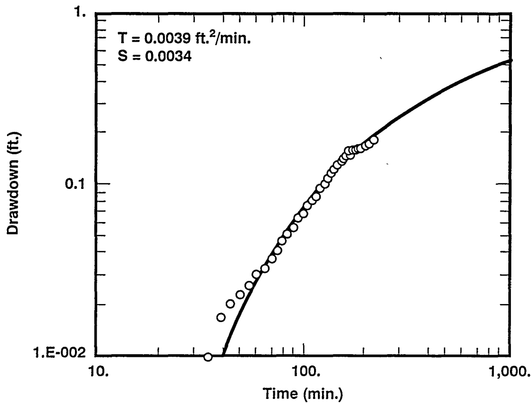
Figure E-5-6 Semi-log and Log-log Plots of Drawdown Versus Time for Observation Hole OH72
