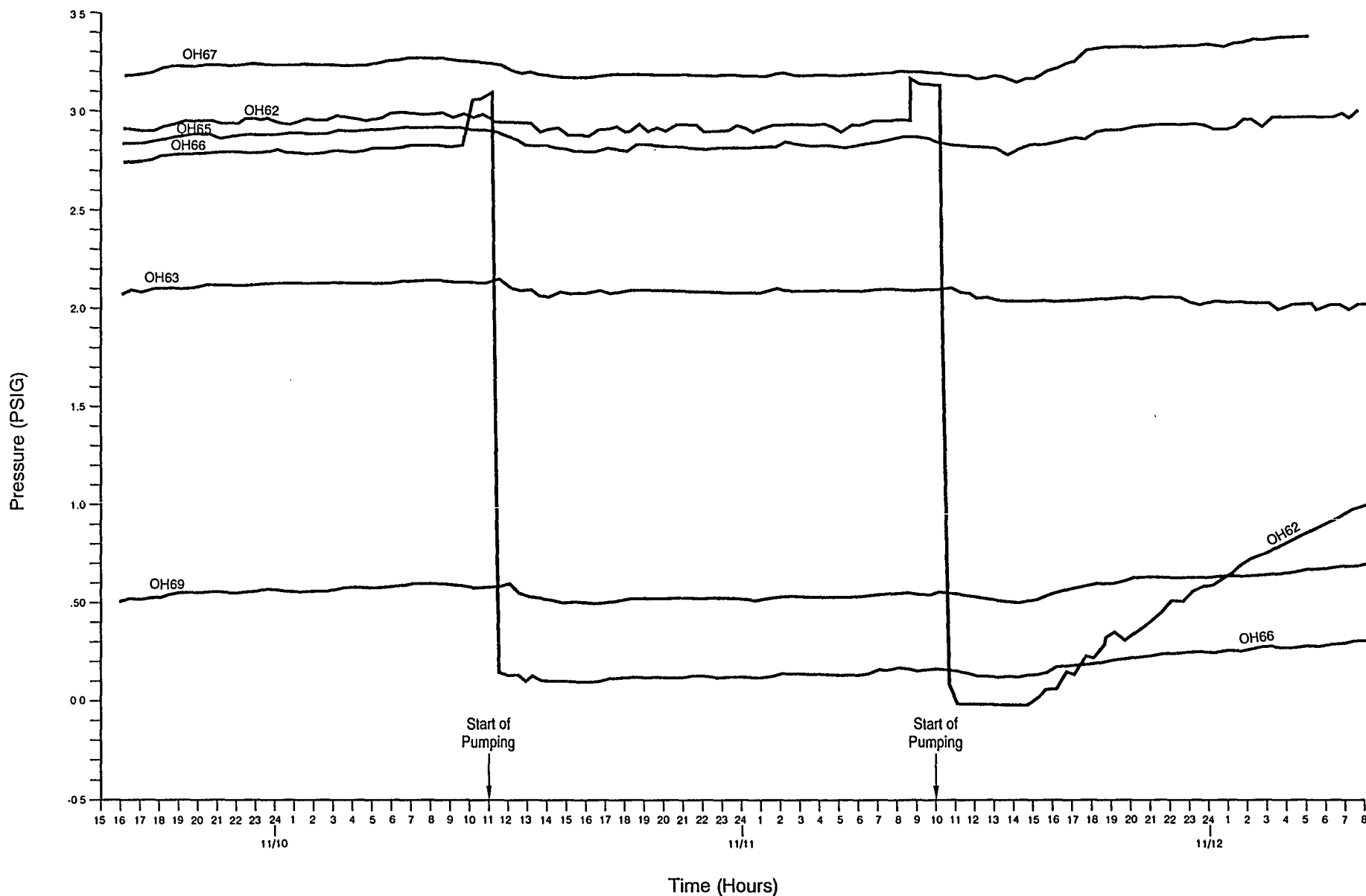
Figure E-5-10 Hydrographs of the W170 Site Testholes OH62, OH63, OH65, OH66, OH67, and OH69 Through the End of the Pumping Test, November 1992
