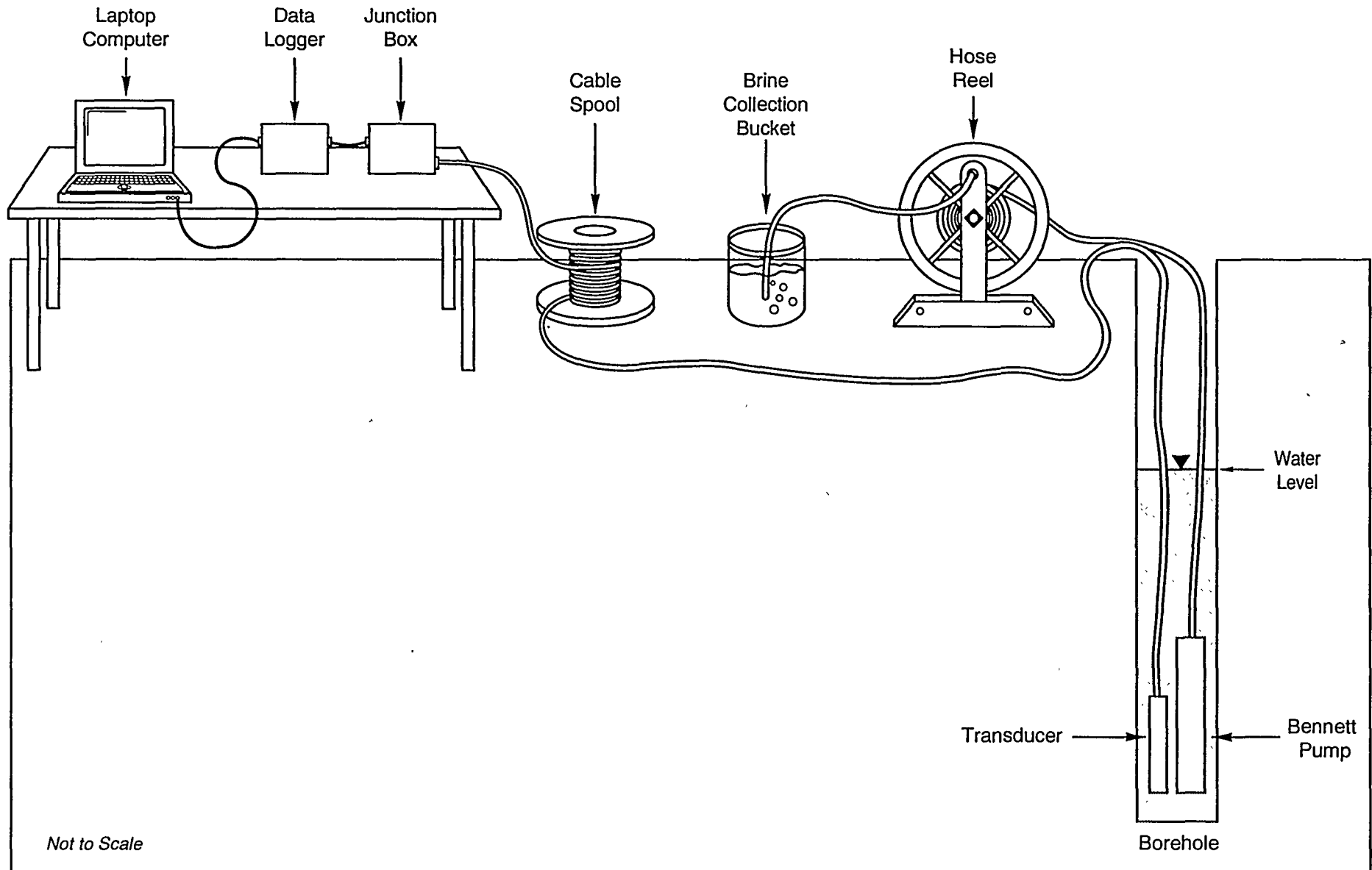
Figure E-3-1 Typical Pump Test Equipment Setup
