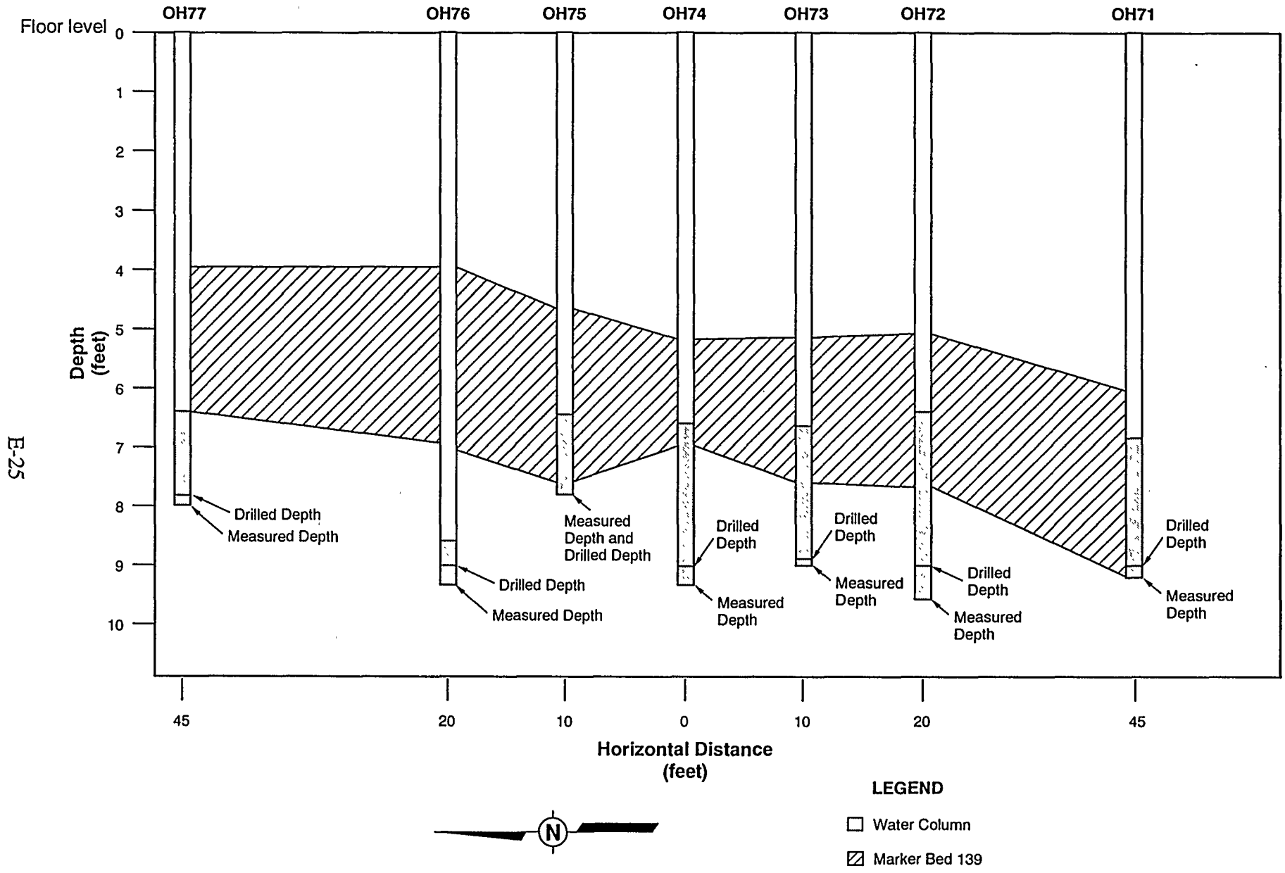
Figure E-4-5 Cross Section of Boreholes Along the E0 Drift Test Site, December 1992
