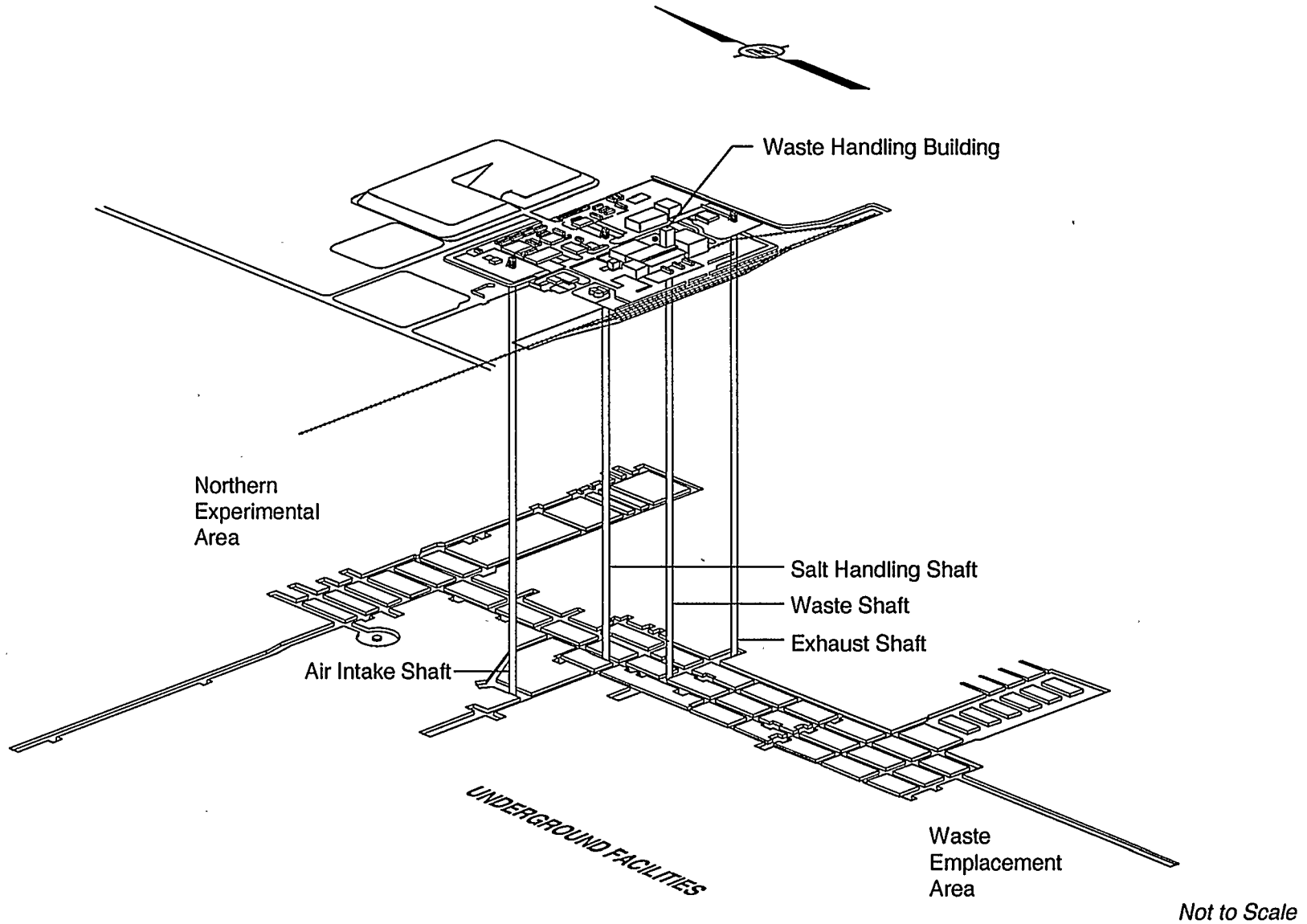
Figure 1-2 Surface and Underground Layout of the WIPP Facility
