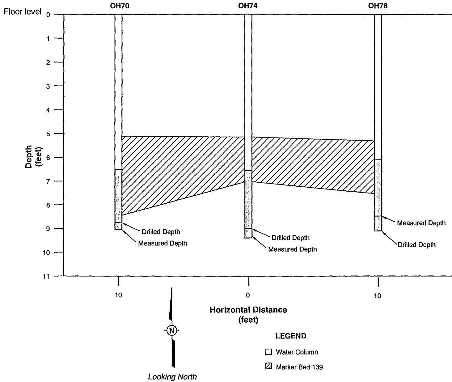
Figure E-4-6 Cross Section of Boreholes Across the E0 Drift Test Site, December 1992
