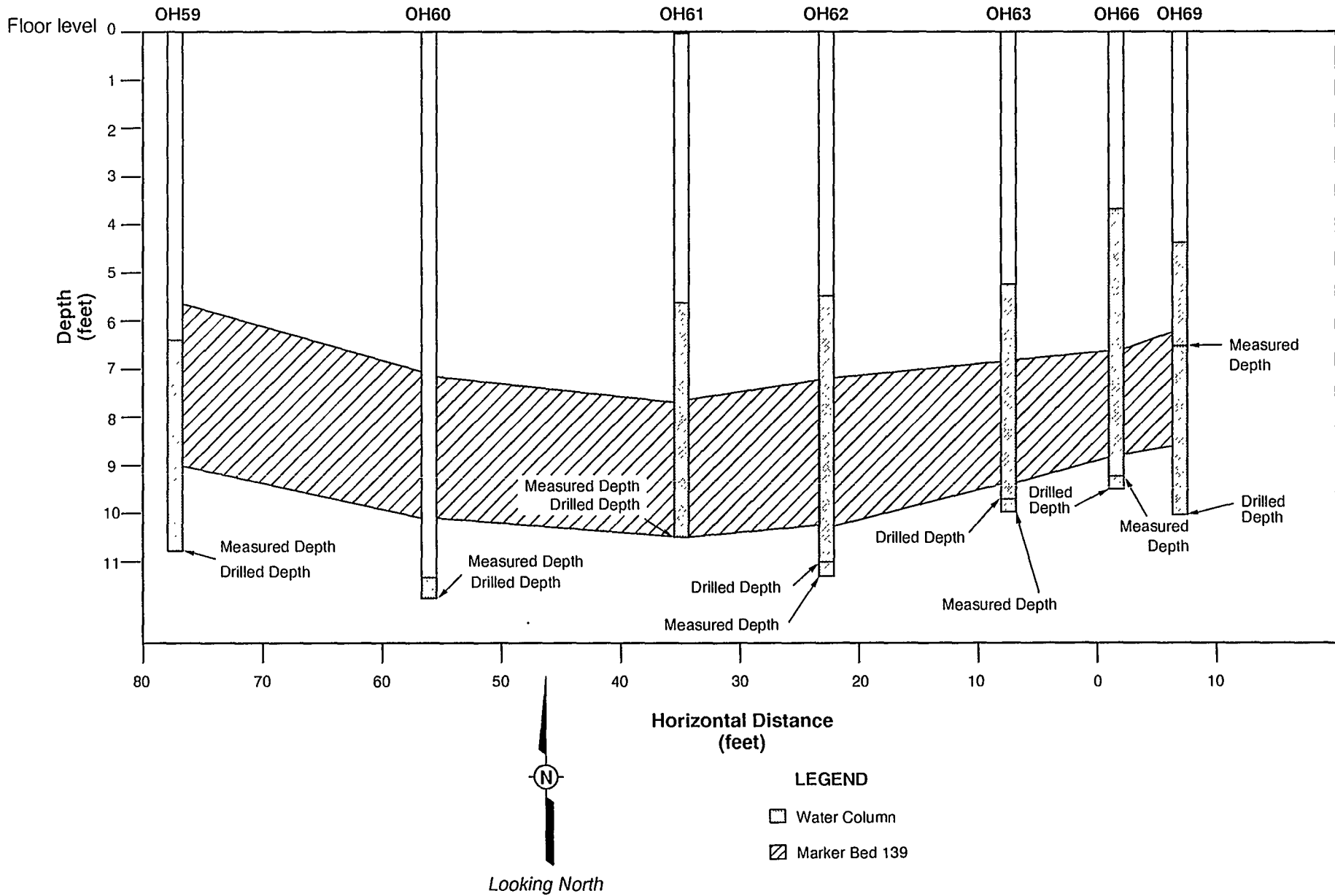
Figure E-4-4 Cross Section of Boreholes Across the W170 Drift and into the Core Library, November 1992
