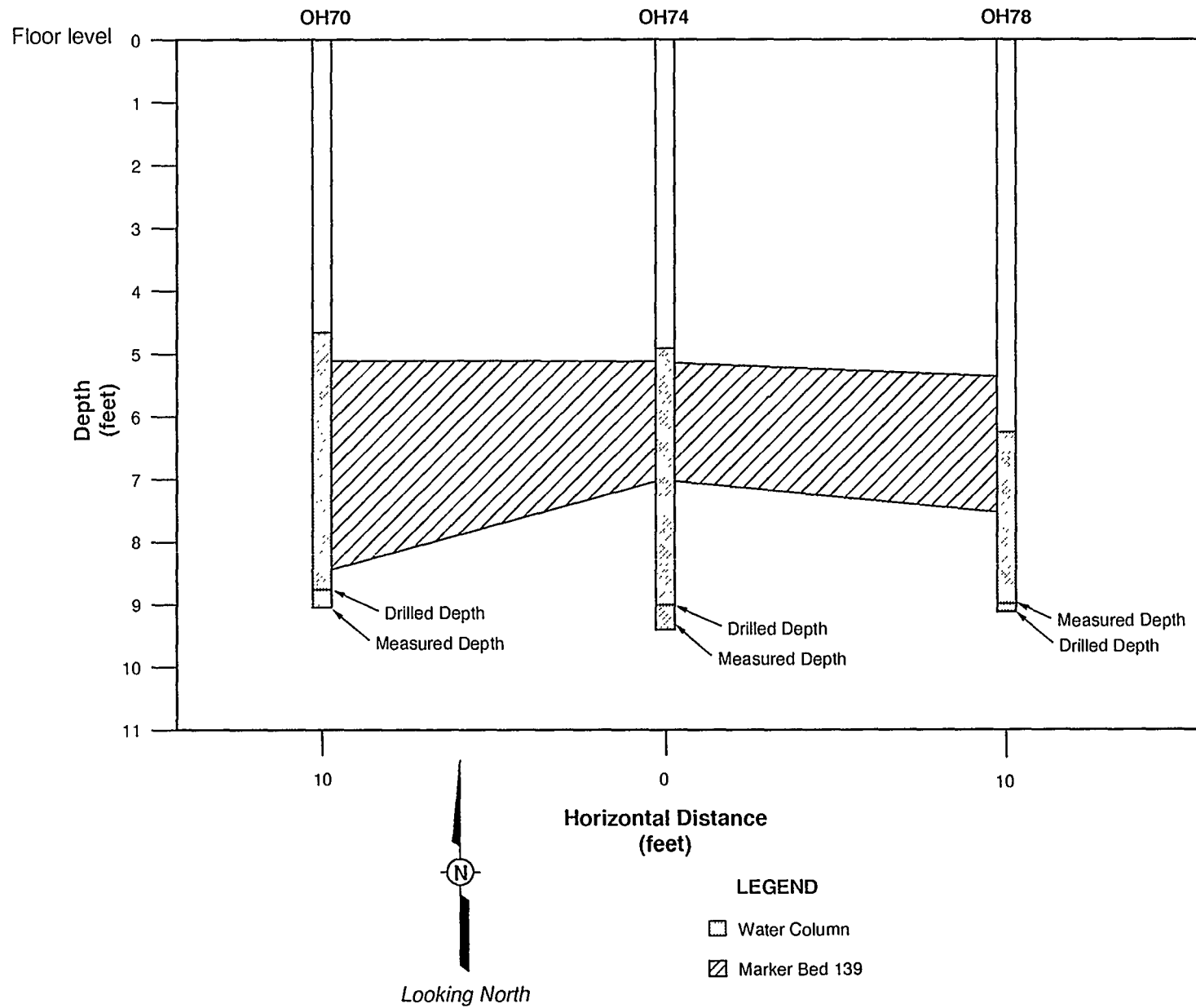
Figure E-4-2 Cross Section of Boreholes Across the E0 Drift Test Site, October 1992
