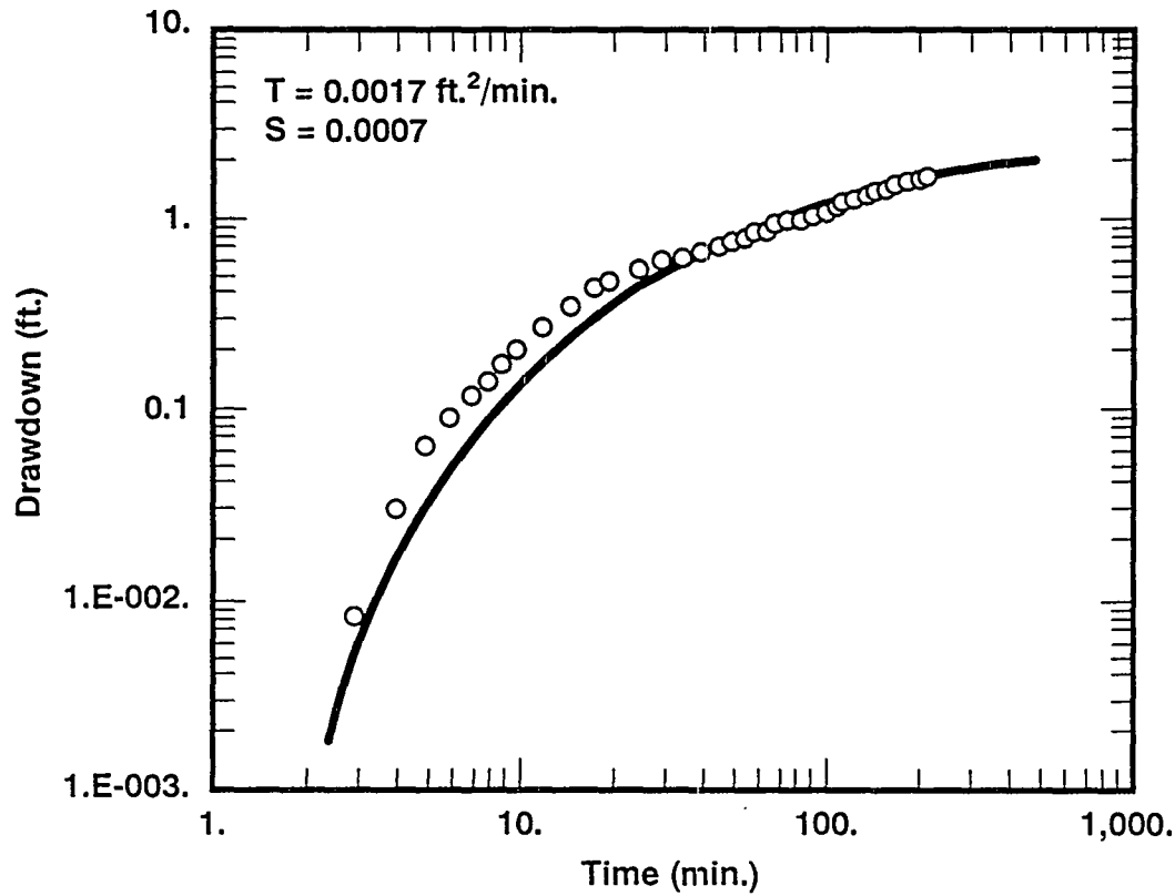
Figure E-5-7 Semilog and Log-log Plots by Drawdown Versus Time for Observation Hole OH73
