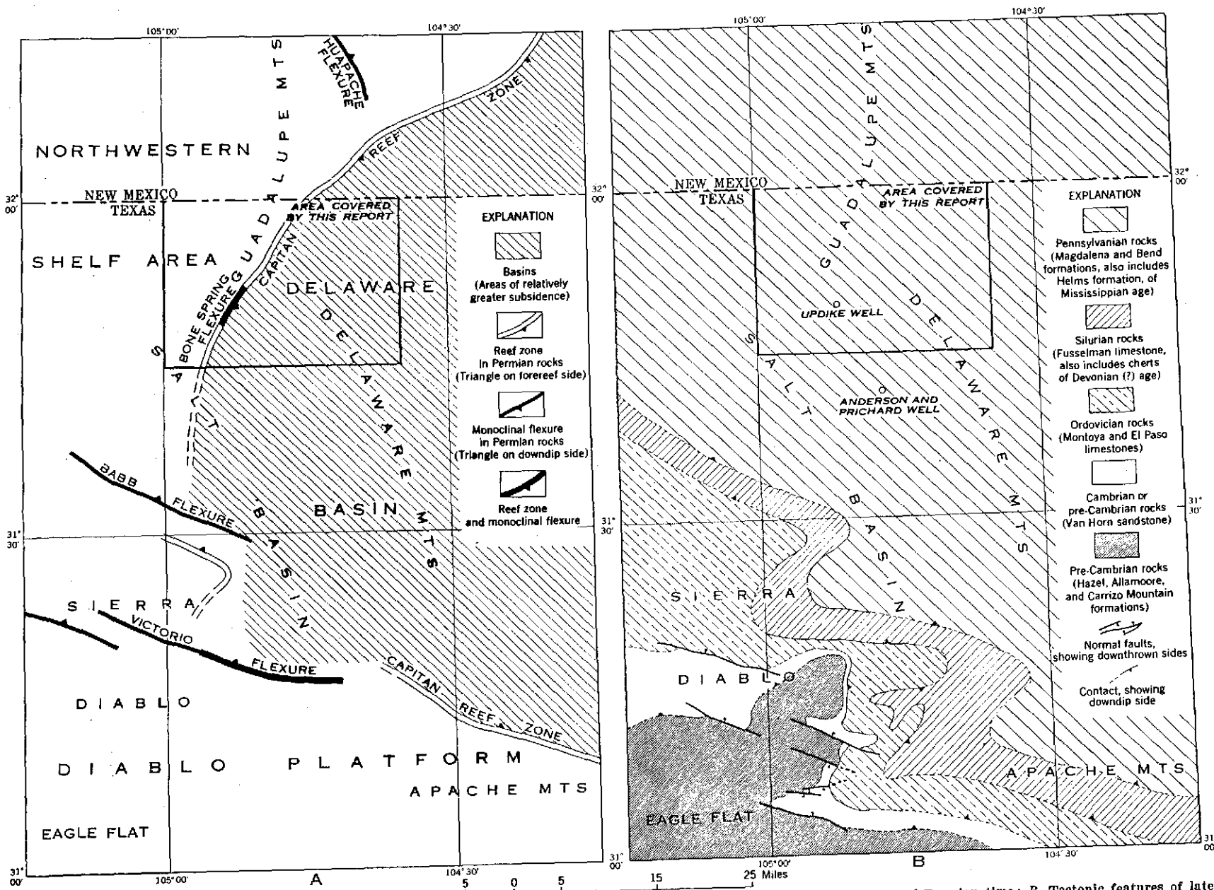
FIGURE 16.—Maps showing tectonic features of Guadalupe Mountains and vicinity during different periods. A, Tectonic features of Permian time; B, Tectonic features of late Carboniferous time, as suggested by paleogeologic map of surface on which Wolfcamp series was deposited.
