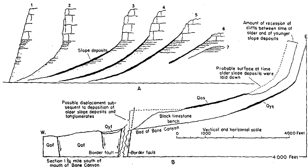
FIGURE 23.—Sections and profiles of westward-facing escarpment near Guadalupe Peak. Qos , Older slope deposits; Qof , older fanglomerates; Qys , younger slope deposits; Qyf , younger fanglomerate. A , Sketch sections showing probable past and future stages in erosion of escarpment, which has now reached stages 3 and 4; B , Profiles across escarpment near Bone Canyon, showing relation of older to younger deposits and land forms.
