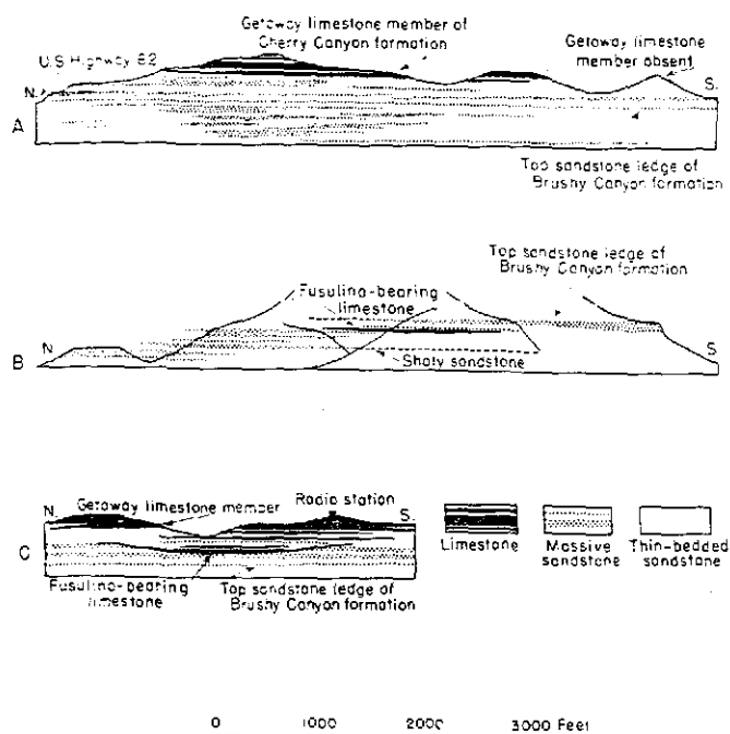
FIGURE 4.—Sections showing lenticular nature of massive sandstones of the Brushy Canyon formation, and of limestones of Getaway member of Cherry Canyon formation. A , East side of Guadalupe Canyon south of Guadalupe Pass; B , West slope of El Capitan; C , Delaware Mountain escarpment near Guadalupe Summit radio station.
