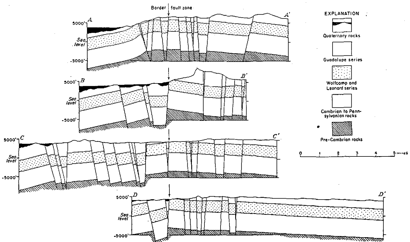
FIGURE 18.—Cross sections, the same as those on plate 3, but expanded downward to the top of the basement rocks.
