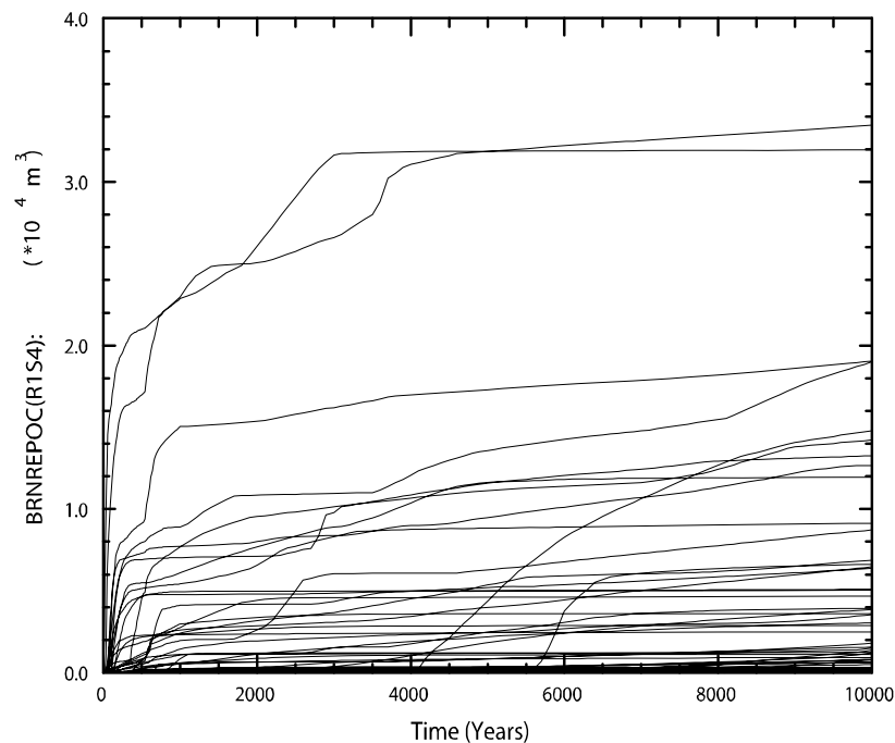
Figure PA-60. Total Cumulative Brine Outflow in Replicate R1, Scenario S4, CRA-2009 PA
