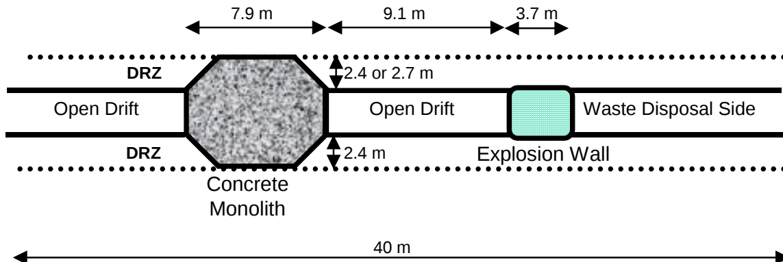
Figure PA-19. Schematic Side View of Option D Panel Closure
