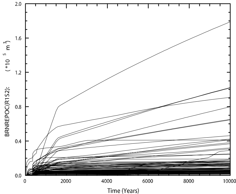
Figure PA-58. Total Cumulative Brine Outflow in Replicate R1, Scenario S2, CRA-2009 PA
