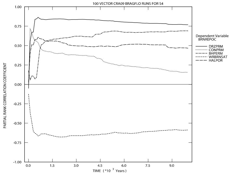
Figure PA-63. Primary Correlations of Cumulative Brine Flow Away from the Repository with Uncertain Parameters, Replicate R1, Scenario S4, CRA-2009 PA
