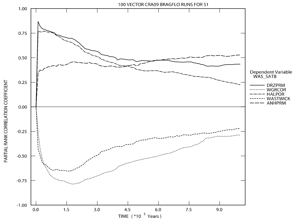
Figure PA-46. Primary Correlations of Brine Saturation in the Waste Panel Region with Uncertain Parameters, Replicate R1, Scenario S1, CRA-2009 PA
