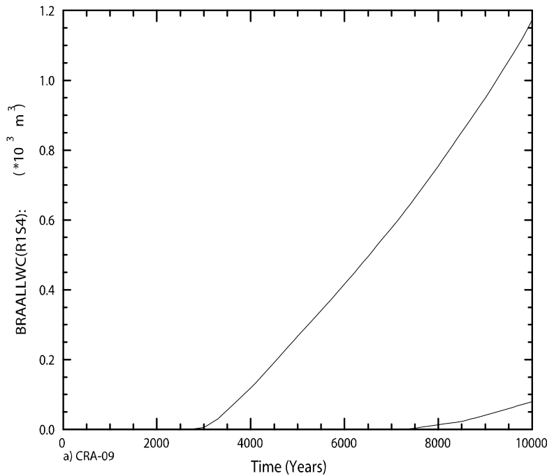
Figure PA-61. Brine Flow via All MBs Across the LWB in Replicate R1, Scenario S4, CRA-2009 PA
