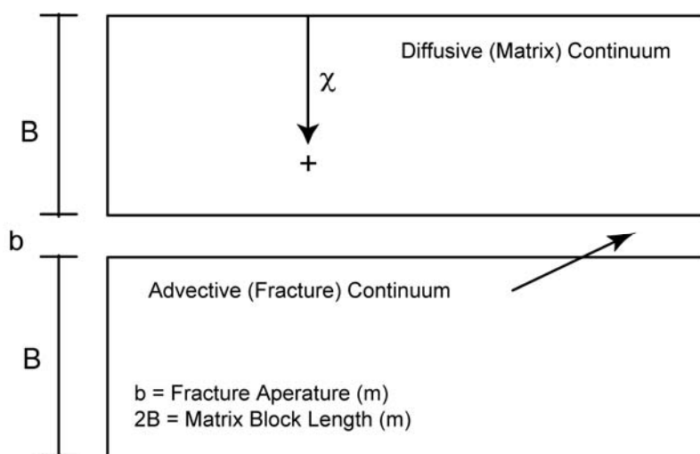
Figure PA-35. Parallel-Plate, Dual-Porosity Conceptualization
