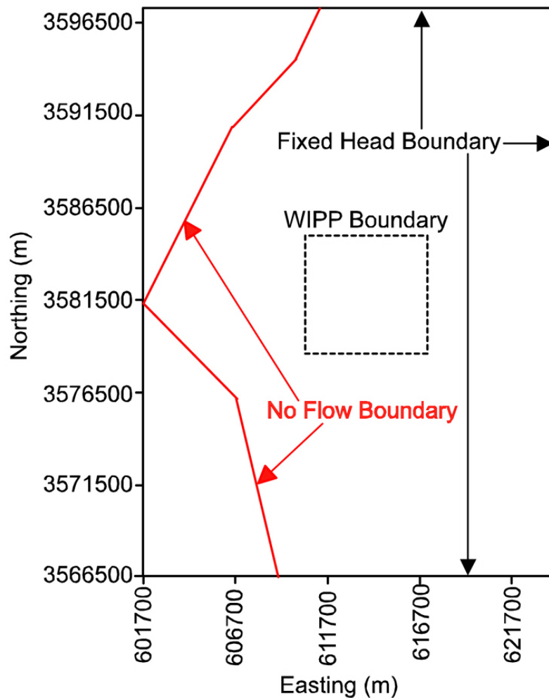
Figure PA-33. Boundary Conditions Used for Simulations of Brine Flow in the Culebra
