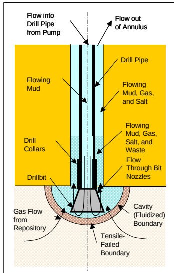
Figure PA-24. Schematic Diagram of the Flow Geometry After Repository Penetration
