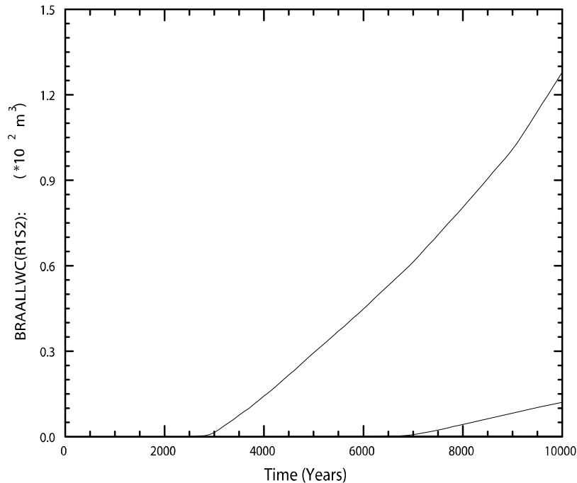
Figure PA-59. Brine Flow via All MBs Across the LWB in Replicate R1, Scenario S2, CRA-2009 PA
