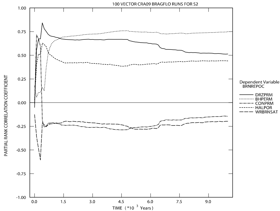
Figure PA-62. Primary Correlations of Cumulative Brine Flow Away from the Repository with Uncertain Parameters, Replicate R1, Scenario S2, CRA-2009 PA
