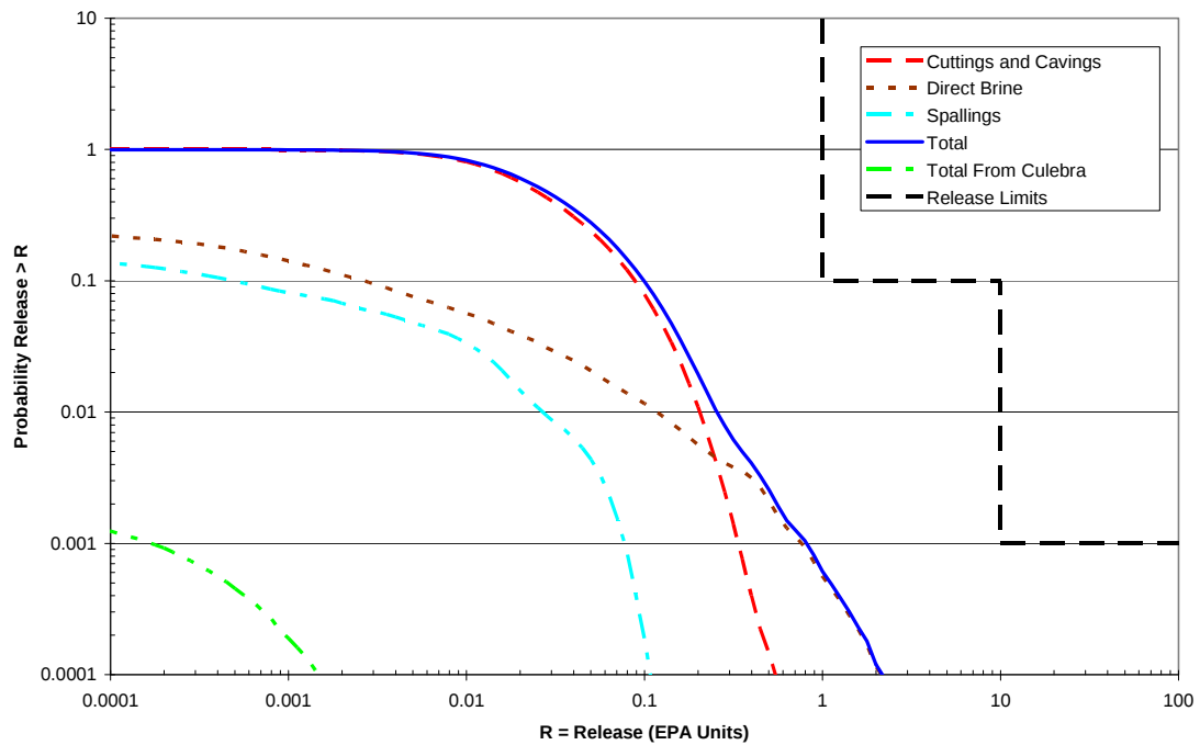
Figure PA-82. Mean CCDFs for Components of Total Normalized Releases, Replicate R2, CRA-2009 PA
