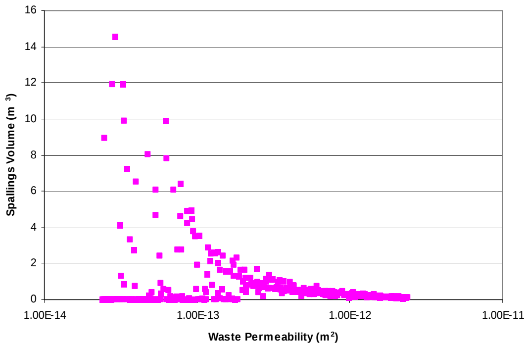
Figure PA-72. Scatterplot of Waste Permeability Versus Spallings Volume, CRA-2009 PA
