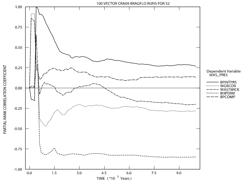
Figure PA-52. Primary Correlations of Pressure in the Waste Panel Region with Uncertain Parameters, Replicate R1, Scenario S2, CRA-2009 PA
