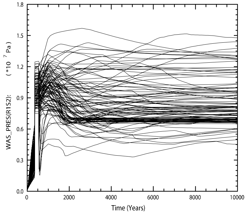
Figure PA-50. Pressure in the Waste Panel Region for Replicate R1, Scenario S2, CRA-2009 PA
