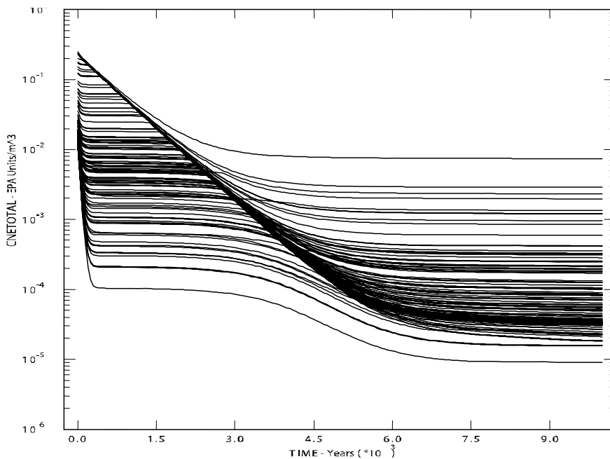
Figure PA-65. Total Mobilized Concentrations in Castile Brine, Replicate R1, CRA-2009 PA
