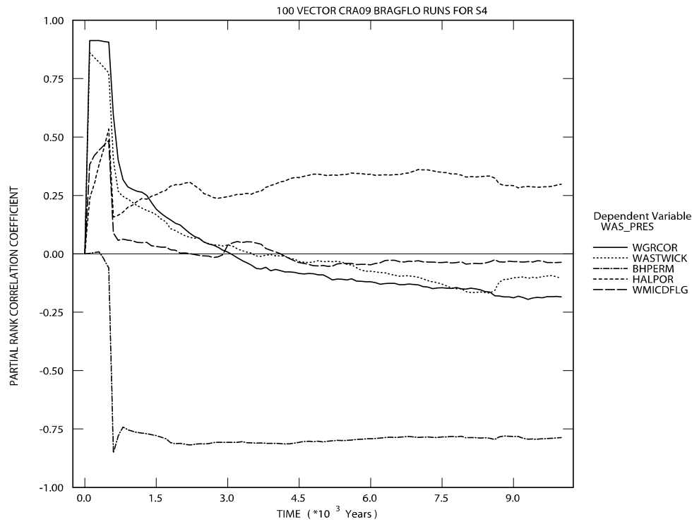
Figure PA-53. Primary Correlations of Pressure in the Waste Panel Region with Uncertain Parameters, Replicate R1, Scenario S4, CRA-2009 PA
