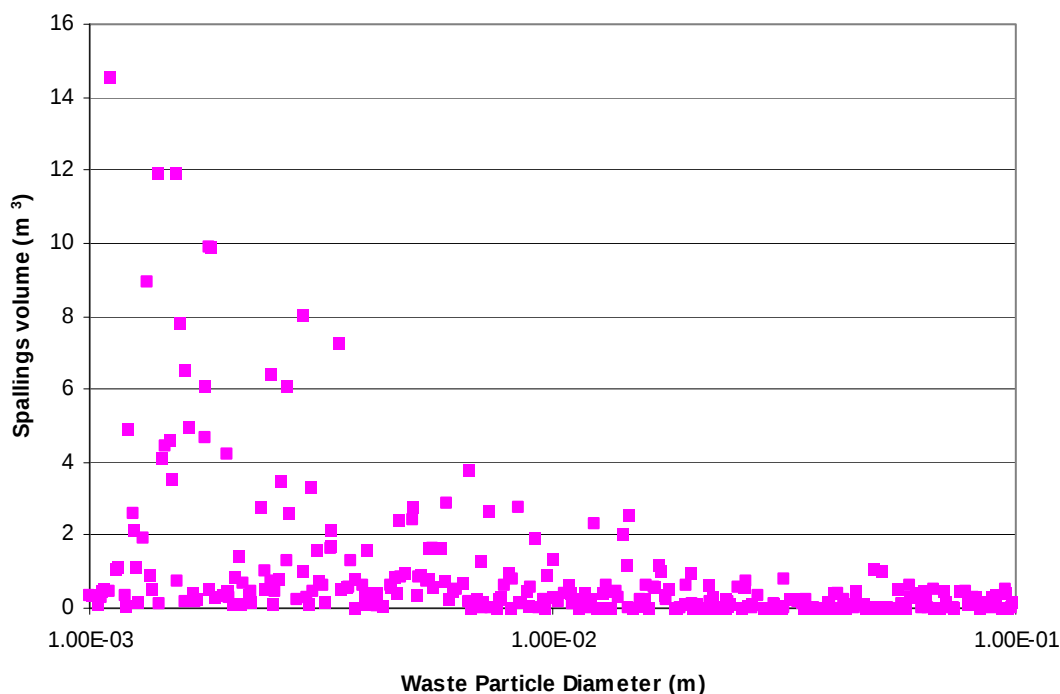
Figure PA-71. Scatterplot of Waste Particle Diameter Versus Spallings Volume, CRA-2009 PA
