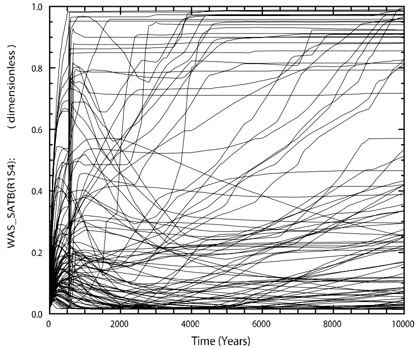
Figure PA-55. Brine Saturation in the Waste Panel Region for Replicate R1, Scenario S4, CRA-2009 PA
