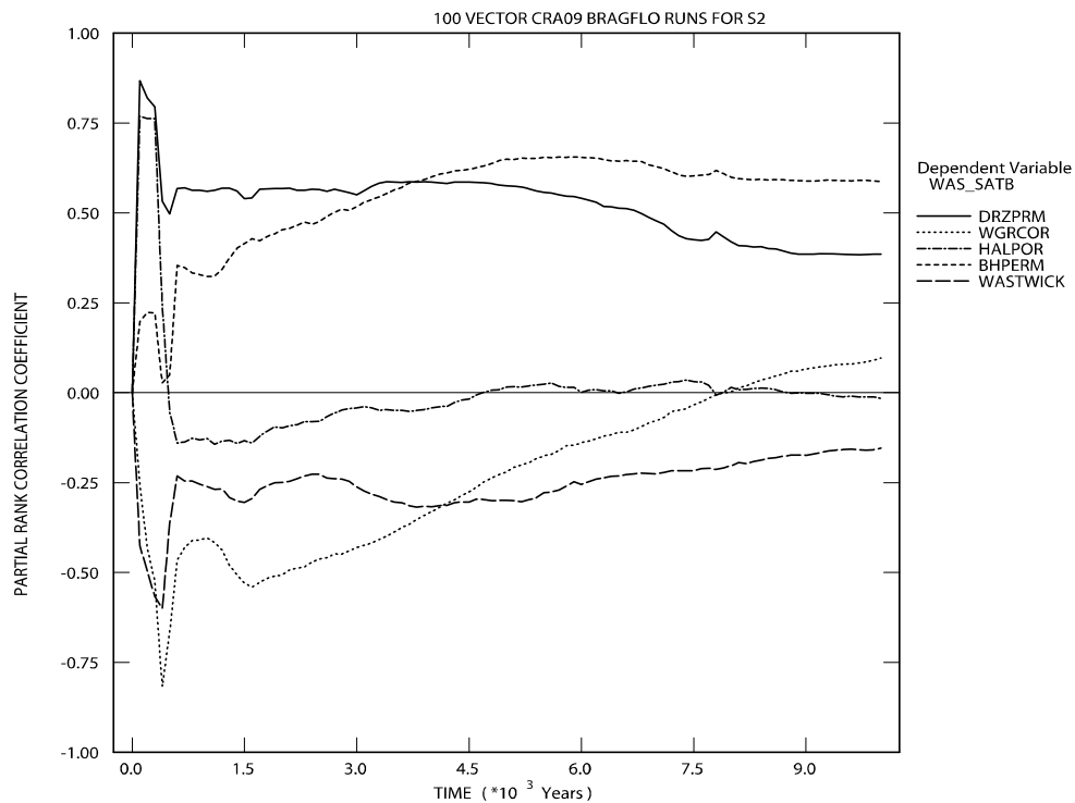
Figure PA-56. Primary Correlations of Brine Saturation in the Waste Panel Region with Uncertain Parameters, Replicate R1, Scenario S2, CRA-2009 PA
