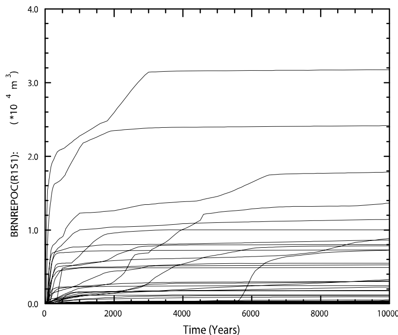
Figure PA-47. Brine Flow Away From the Repository, Replicate R1, Scenario S1, CRA-2009 PA
