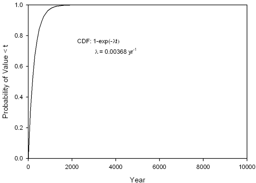
Figure PA-13. CDF for Time Between Drilling Intrusions
