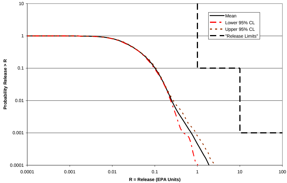
Figure PA-5. Example Mean Probability of Release and the Confidence Limits on the Mean from CRA-2009 PA
