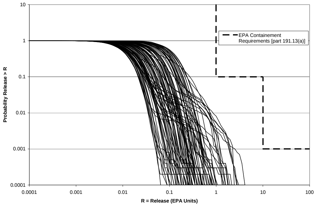
Figure PA-6. Example CCDF Distribution From CRA-2009 PA (Replicate 1)
