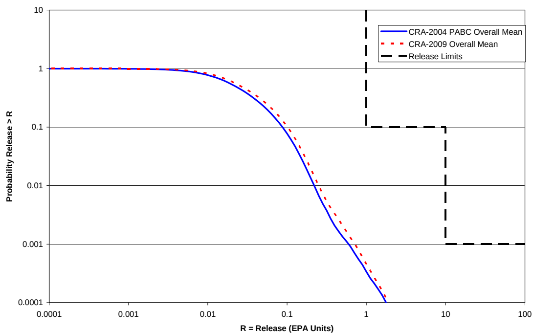
Figure PA-84. Overall Mean CCDFs for Total Normalized Releases: CRA-2009 PA and CRA-2004 PABC
