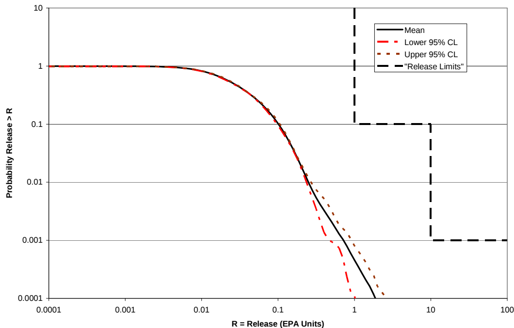
Figure PA-80. Confidence Interval on Overall Mean CCDF for Total Normalized Releases, CRA-2009 PA
