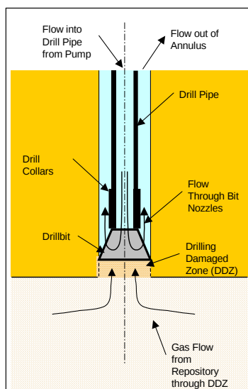
Figure PA-23. Schematic Diagram of the Flow Geometry Prior to Repository Penetration
