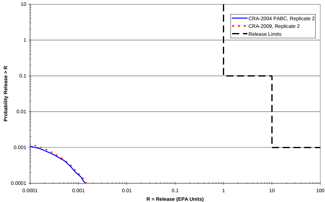
Figure PA-77. Mean CCDFs for Releases from the Culebra for Replicate R2: CRA-2009 PA and CRA-2004 PABC
