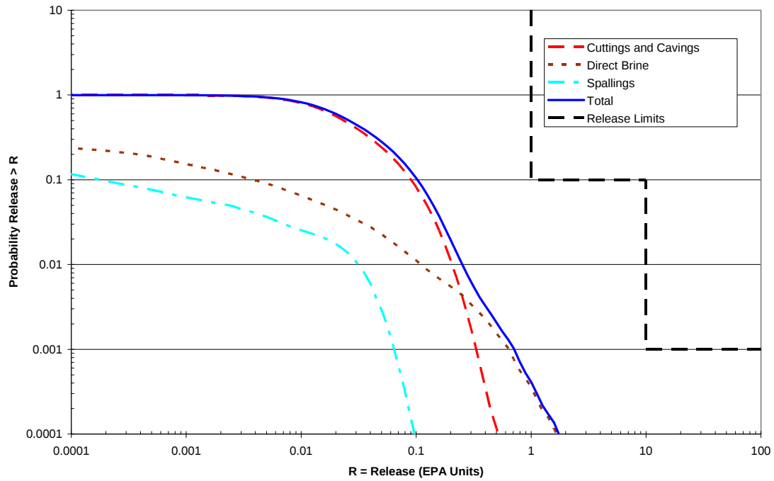
Figure PA-81. Mean CCDFs for Components of Total Normalized Releases, Replicate R1, CRA-2009 PA
