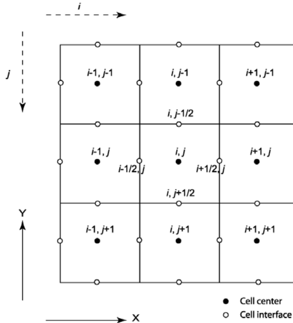
Figure PA-34. Finite-Difference Grid Showing Cell Index Numbering Convention Used by MODFLOW
