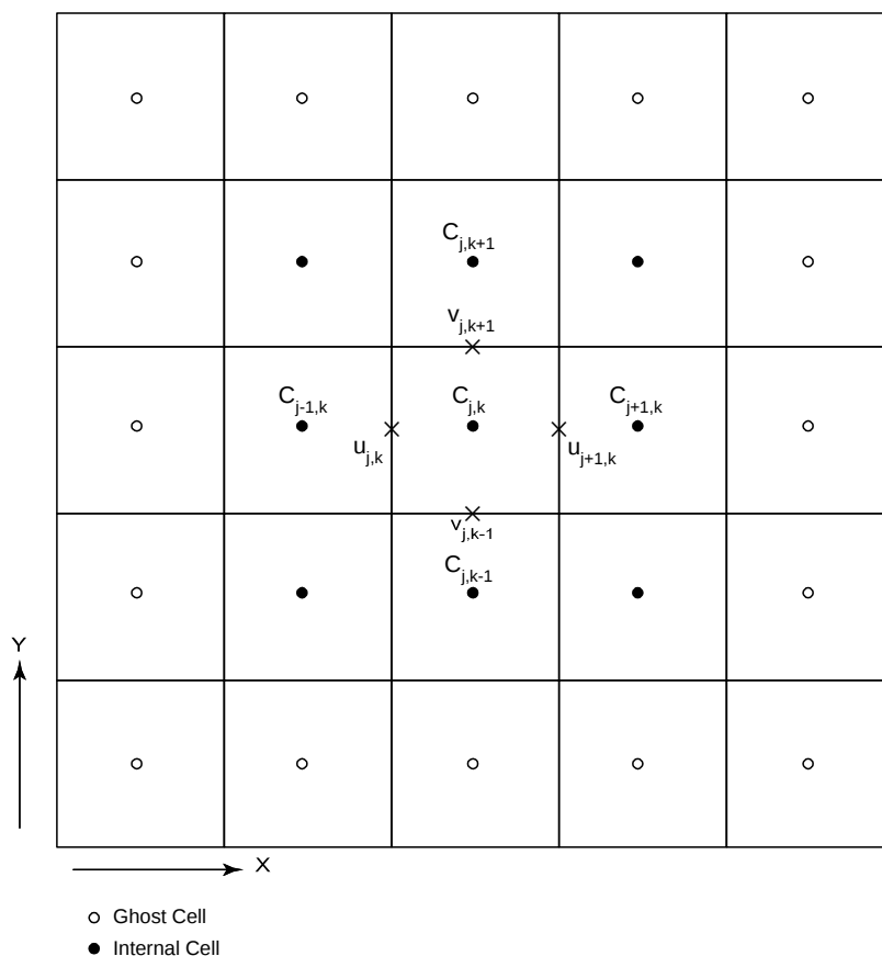
Figure PA-36. Schematic of Finite-Volume Staggered Mesh Showing Internal and Ghost Cells
