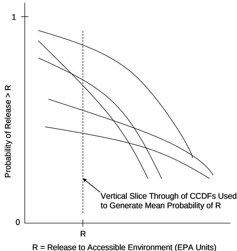
Figure PA-4. Distribution of CCDFs Resulting from Possible Values for the Sampled Parameters
