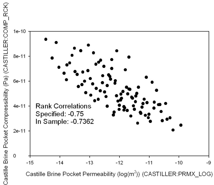
Figure PA-39. Correlation between CASTILLER:PRMX_LOG and CASTILLER:COMP_RCK
