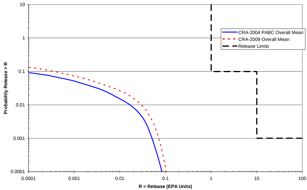
Figure PA-75. Overall Mean CCDFs for Spallings Releases: CRA-2009 PA and CRA 2004 PABC
