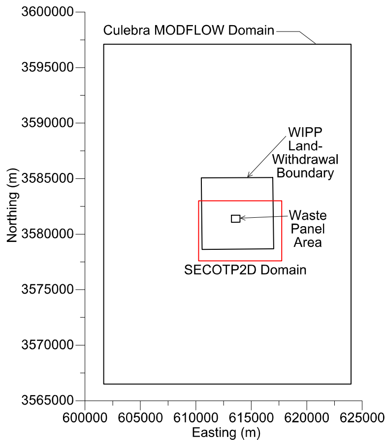
Figure PA-32. Modeling Domain for Groundwater Flow (MODFLOW) and Radionuclide Transport (SECOTP2D) in the Culebra
