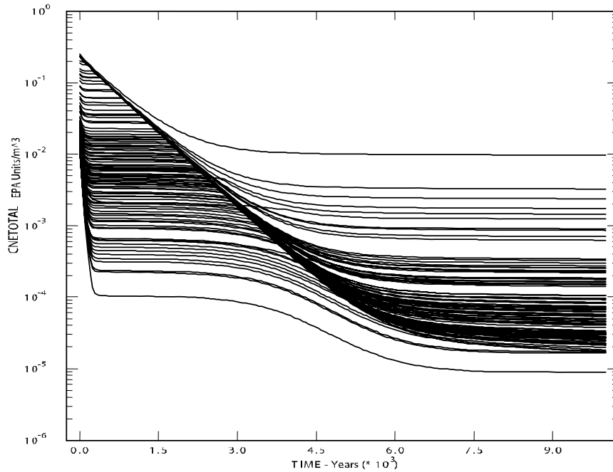
Figure PA-64. Total Mobilized Concentrations in Salado Brine, Replicate R1, CRA-2009 PA
