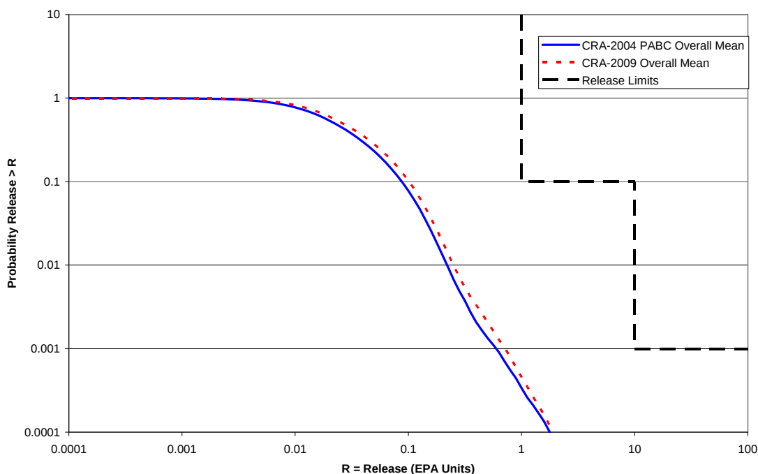
Figure PA-1. Overall Mean CCDFs for Total Normalized Releases: CRA-2009 PA and CRA-2004 PABC
