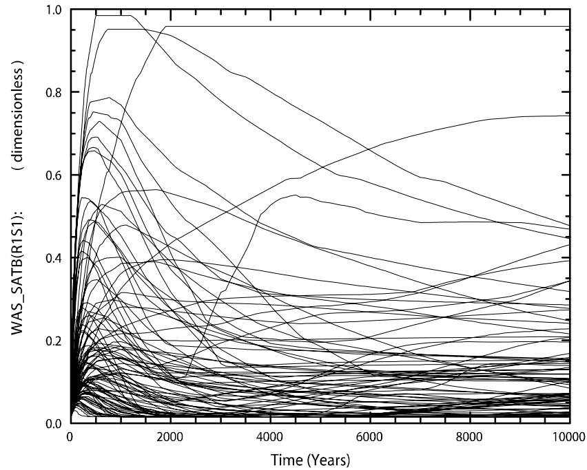
Figure PA-45. Brine Saturation in the Waste Panel Region, Replicate R1, Scenario S1, CRA-2009 PA
