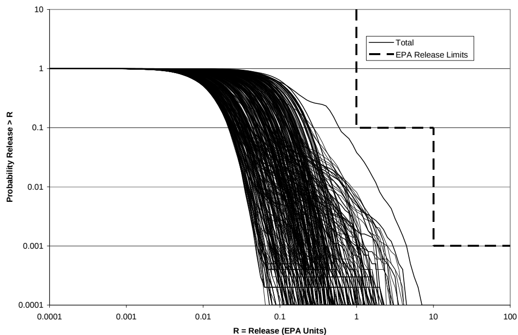
Figure PA-79. Total Normalized Releases, Replicates R1, R2, and R3, CRA-2009 PA
