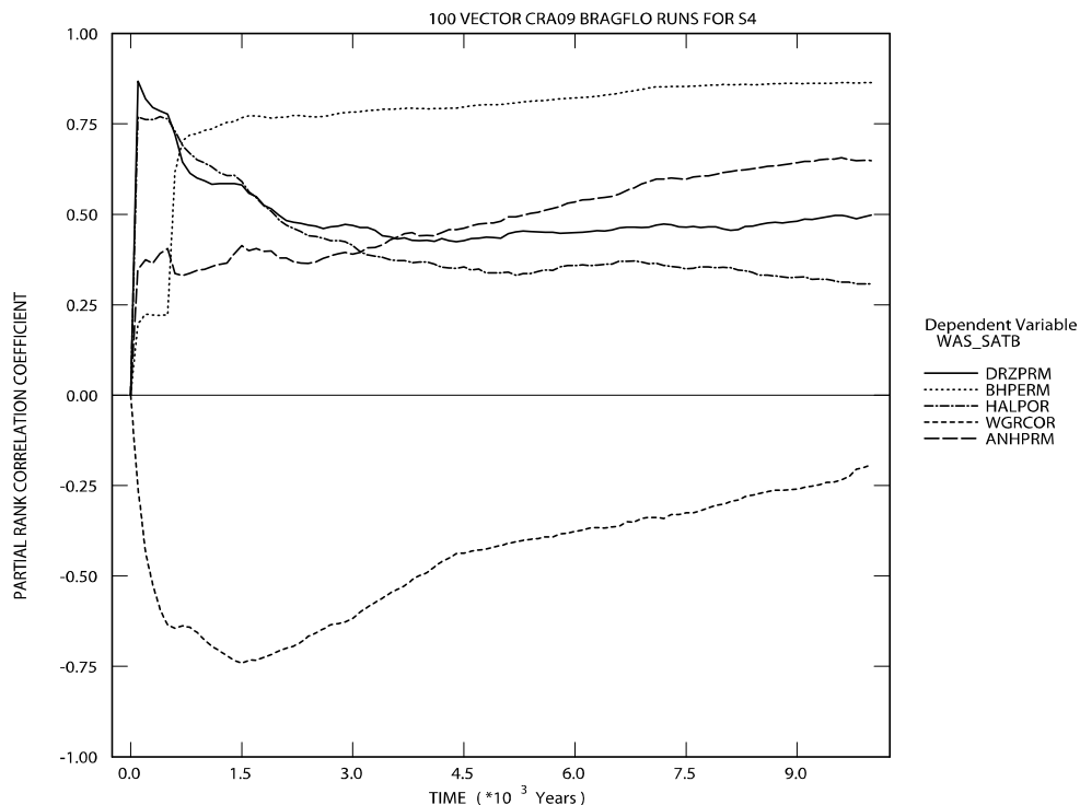
Figure PA-57. Primary Correlations of Brine Saturation in the Waste Panel Region with Uncertain Parameters, Replicate R1, Scenario S4, CRA-2009 PA
