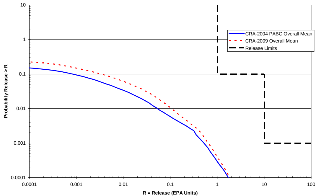
Figure PA-76. Overall Mean CCDFs for DBRs: CRA-2009 PA and CRA-2004 PABC
