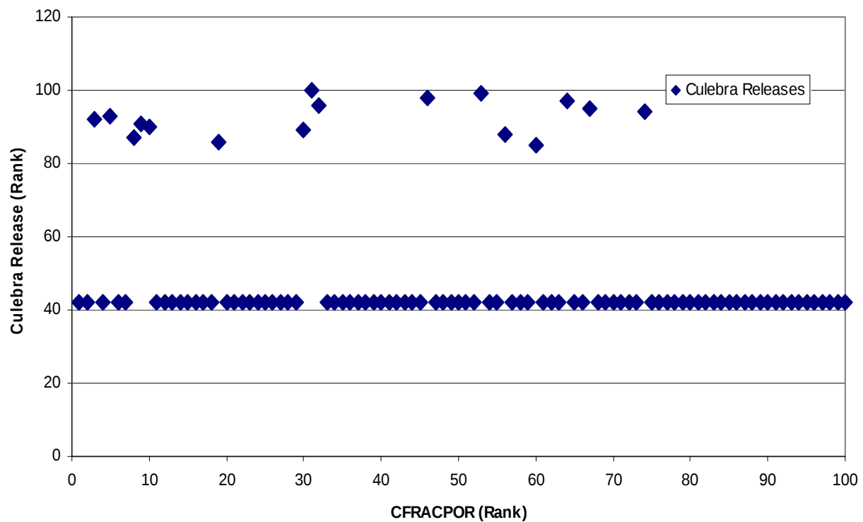
Figure PA-78. The Preponderance and Distribution of Zeros Can Control the Regression
