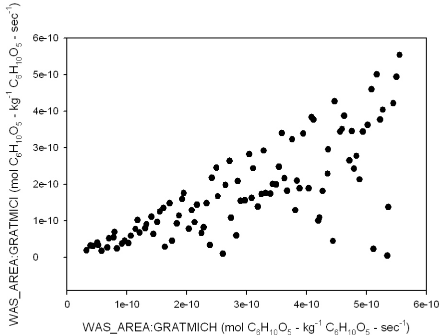
Figure PA-40. Dependency between WAS_AREA:GRATMICH and WAS_AREA:GRATMICI
