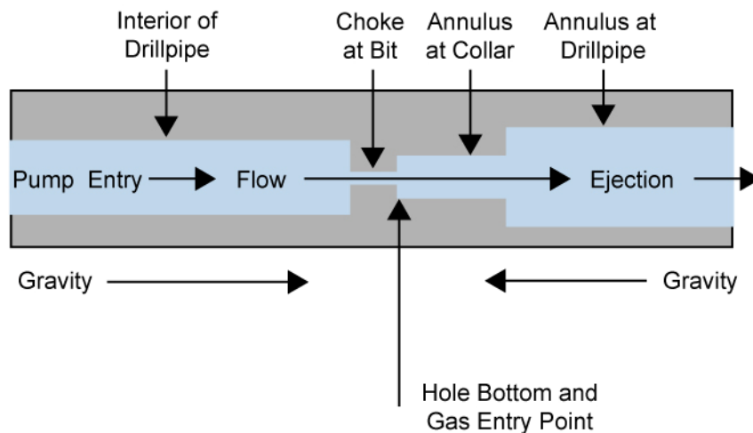
Figure PA-25. Effective Wellbore Flow Geometry Before Bit Penetration
