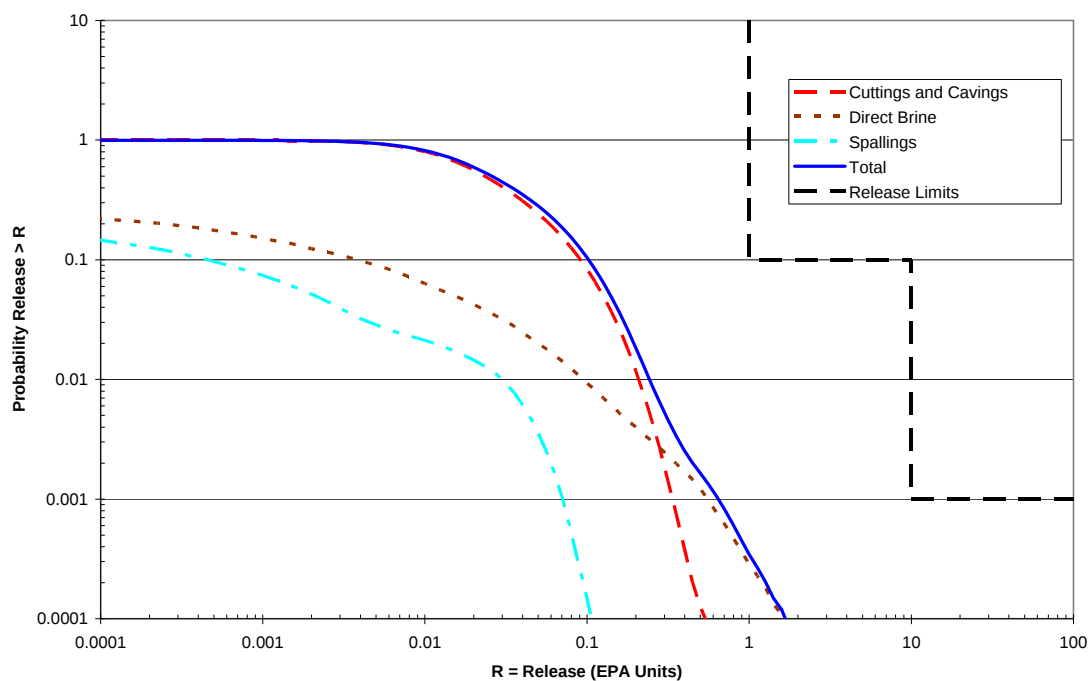
Figure PA-83. Mean CCDFs for Components of Total Normalized Releases, Replicate R3, CRA-2009 PA
