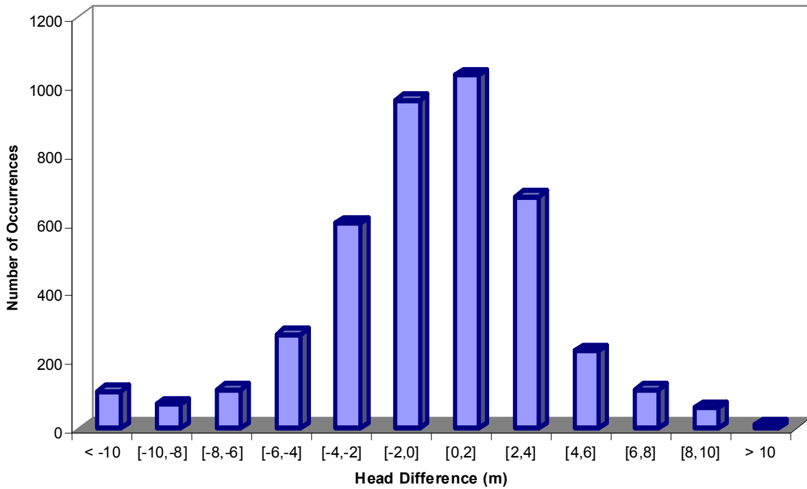
Figure TFIELD-61. Histogram of Differences Between Measured and Modeled Steady-State Heads
