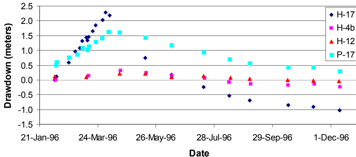
Figure TFIELD-34. Observed Drawdowns for the H-11 Hydraulic Test
