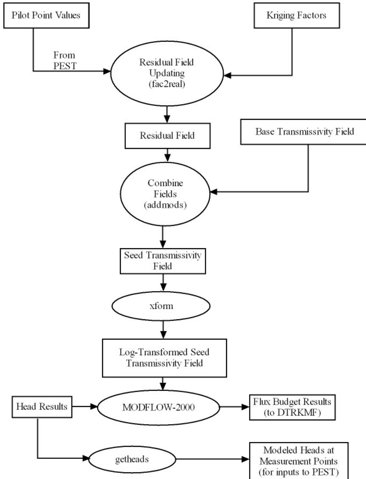
Figure TFIELD-42. Flow Chart of the Core of the Inversion Process Highlighting the Connection Between PEST and MODFLOW-2000
