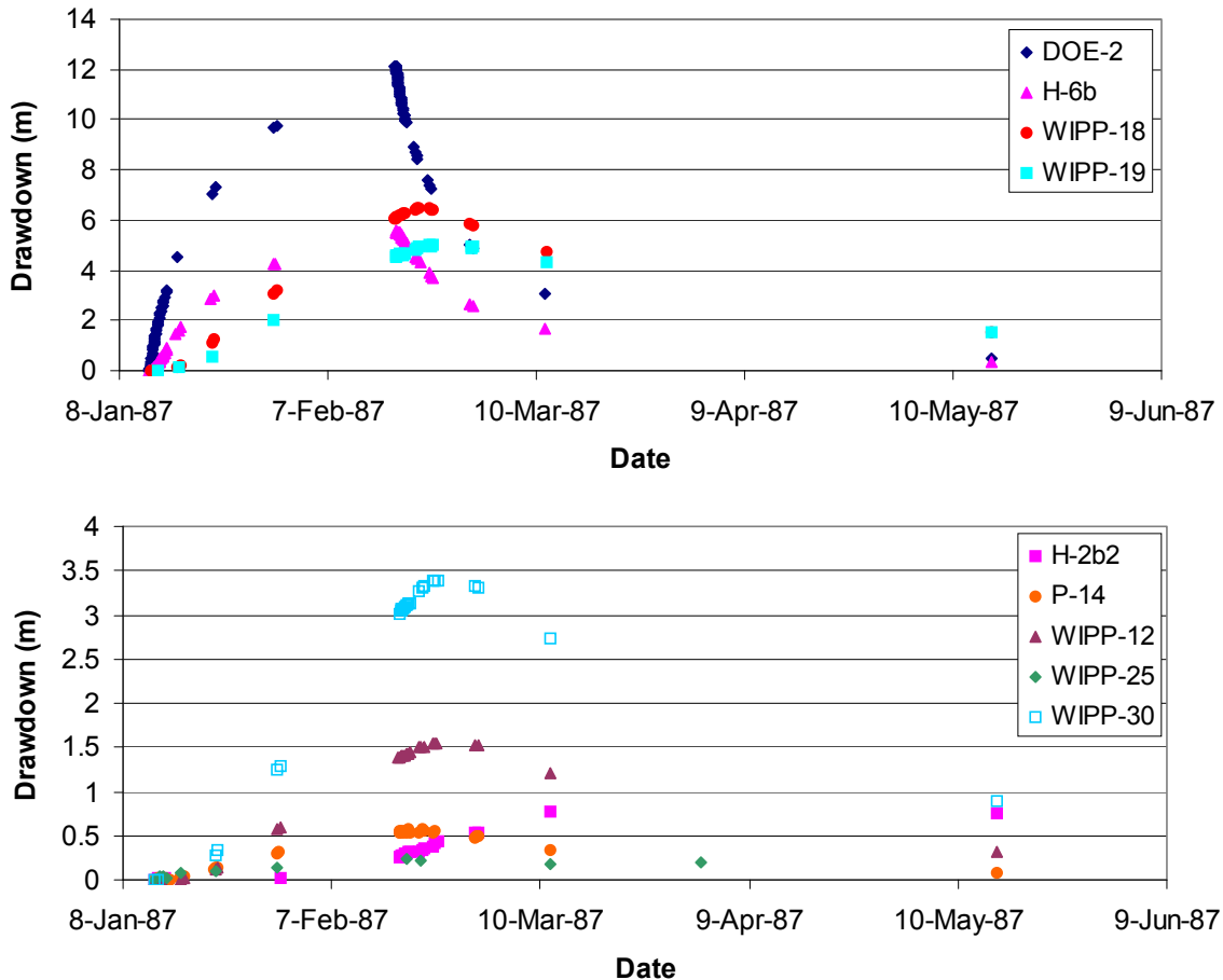
Figure TFIELD-26. Observed Drawdowns for the WIPP-13 Hydraulic Test. Note the Change in the Scale of the Y-Axis from the Upper to the Lower Image.
