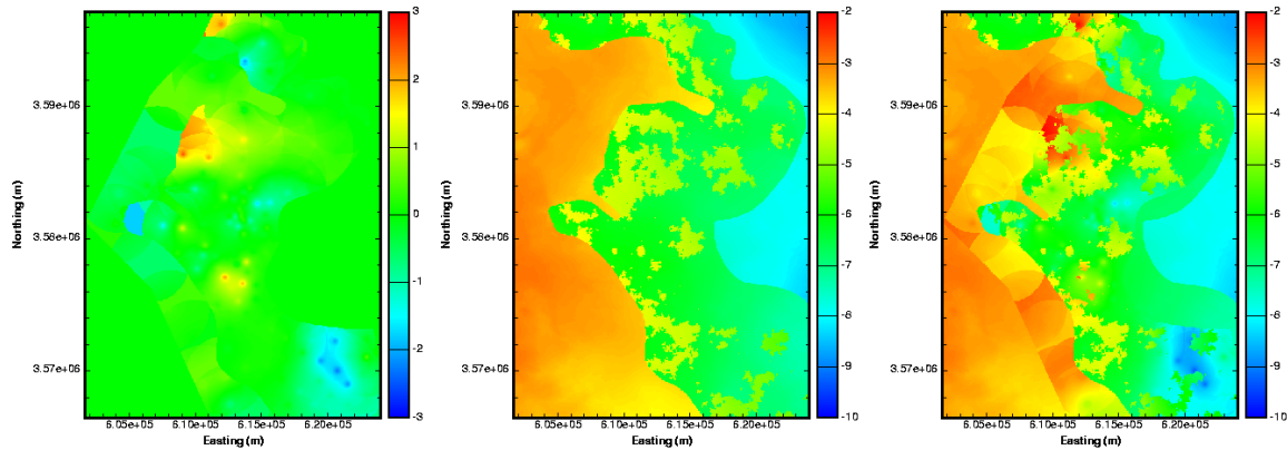
Figure TFIELD-43. Example Final Steps in the Creation of a Calibrated T Field. The Calibrated Residual Field (Left Image) is Added to the Base T Field (Middle Image) to Get the Final Calibrated T Field (Right Image). All Color Scales are in Units of \log_{10} Transmissivity ( m^2/s ).
