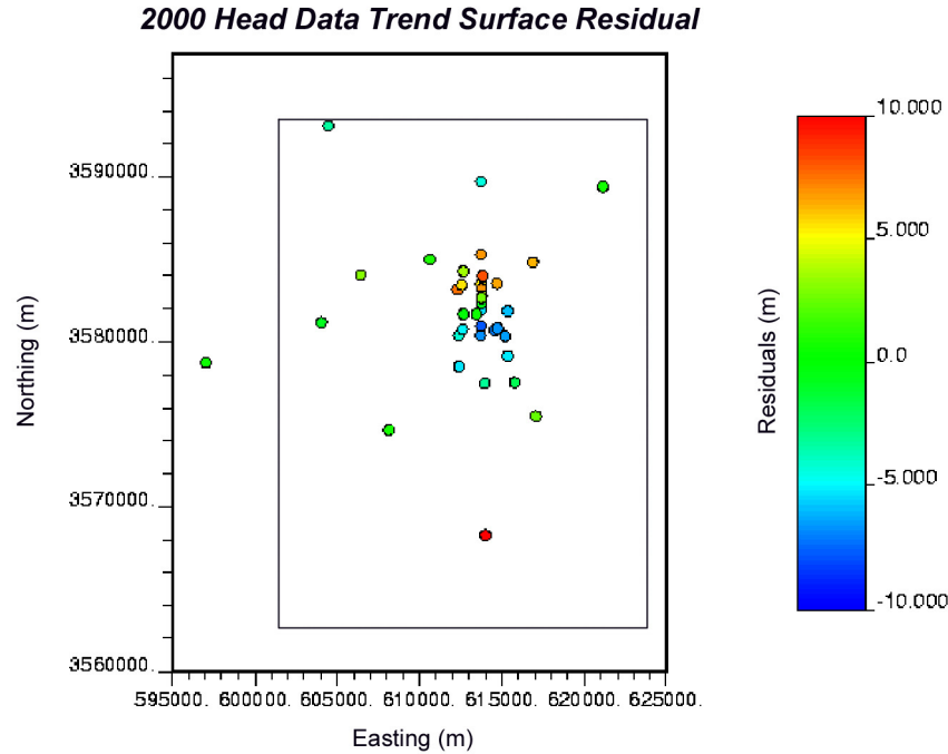
Figure TFIELD-18. Locations and Values of the Residuals Between the Gaussian Trend Surface Model and the Observed Head Data. The Approximate Boundary of the Flow Model is Shown as a Black Rectangle in the Image.
