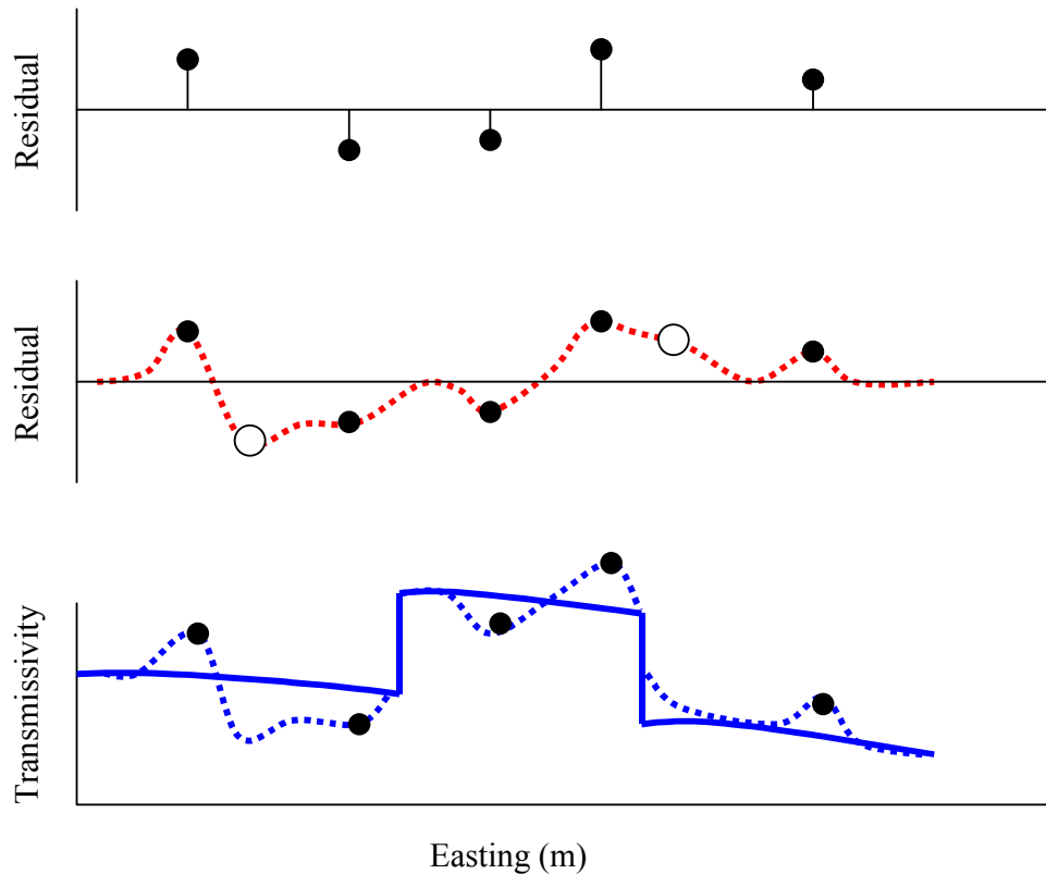
Figure TFIELD-40. Conceptual Cross-Section Showing the Addition of Pilot Points to the Optimization Process
