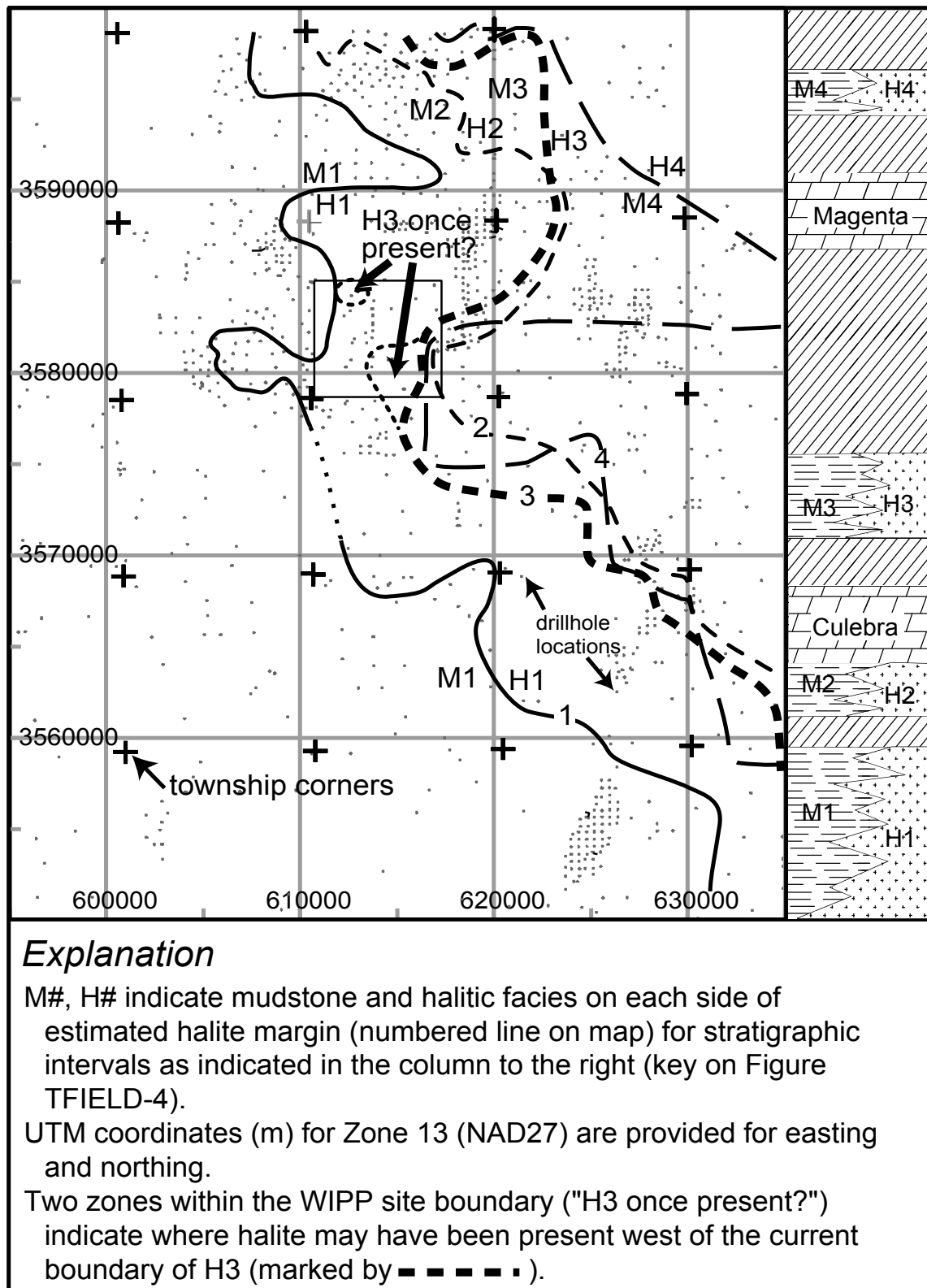
Figure TFIELD-3. Rustler Halite Margins. See Figure TFIELD-4 for Key to Stratigraphic Column.
