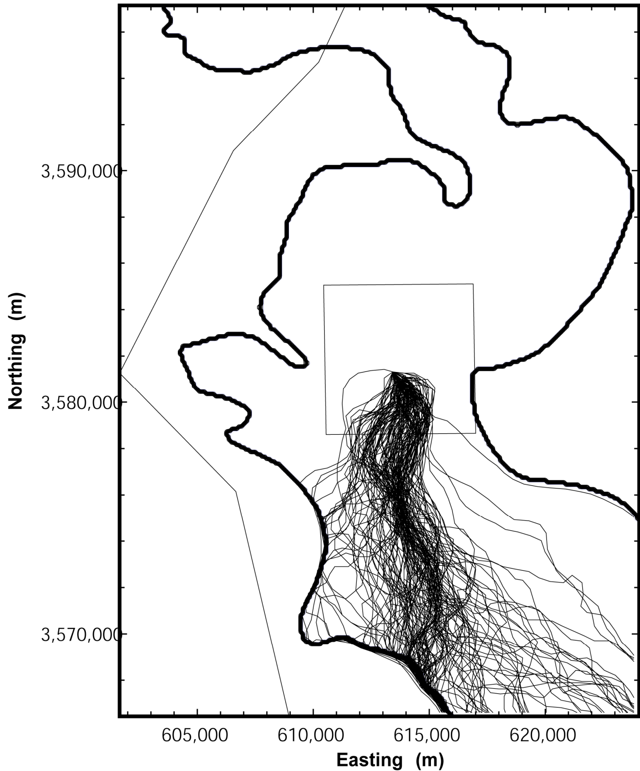
Figure TFIELD-59. All Particle Tracks Within the Model Domain. The Bold Lines Show the Boundaries of the High-T (Left) and Low-T (Right) Zone Boundaries. The No-Flow and WIPP Site Boundaries are Also Shown.
