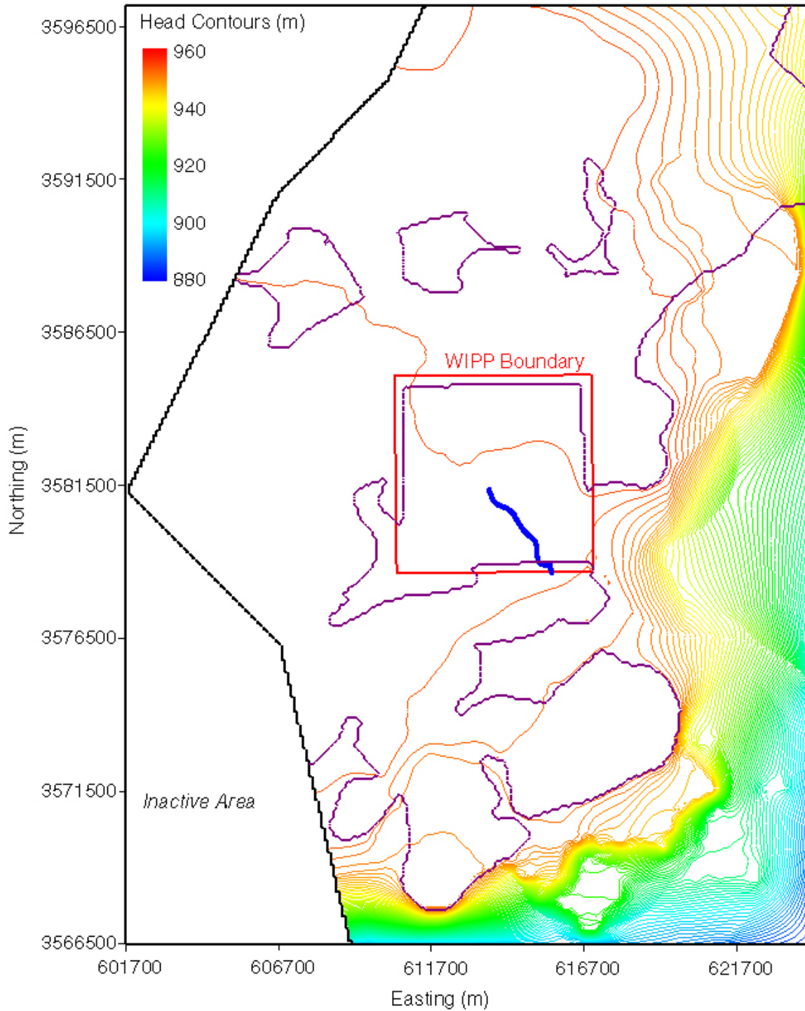
Figure TFIELD-82. Head Contours and Particle Track for the Median-Travel-Time T Field (d13r07-R2) for the Partial-Mining Case. The WIPP LWB is the Red Box in the Center of the Figure and the Particle Track is the Blue Track Originating from the Approximate Center of the WIPP.
