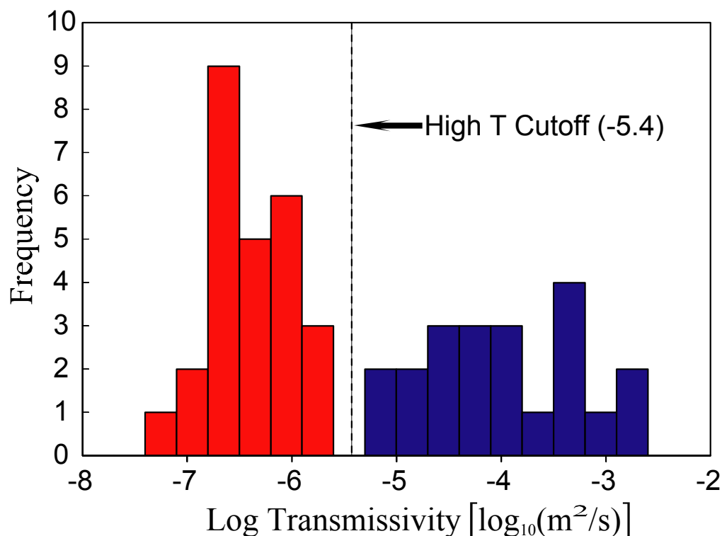
Figure TFIELD-5. Histogram of log 10 Culebra Transmissivity. Data from U.S. Department of Energy (1996), Beauheim and Ruskauff (1998), and Beauheim (2002c).
