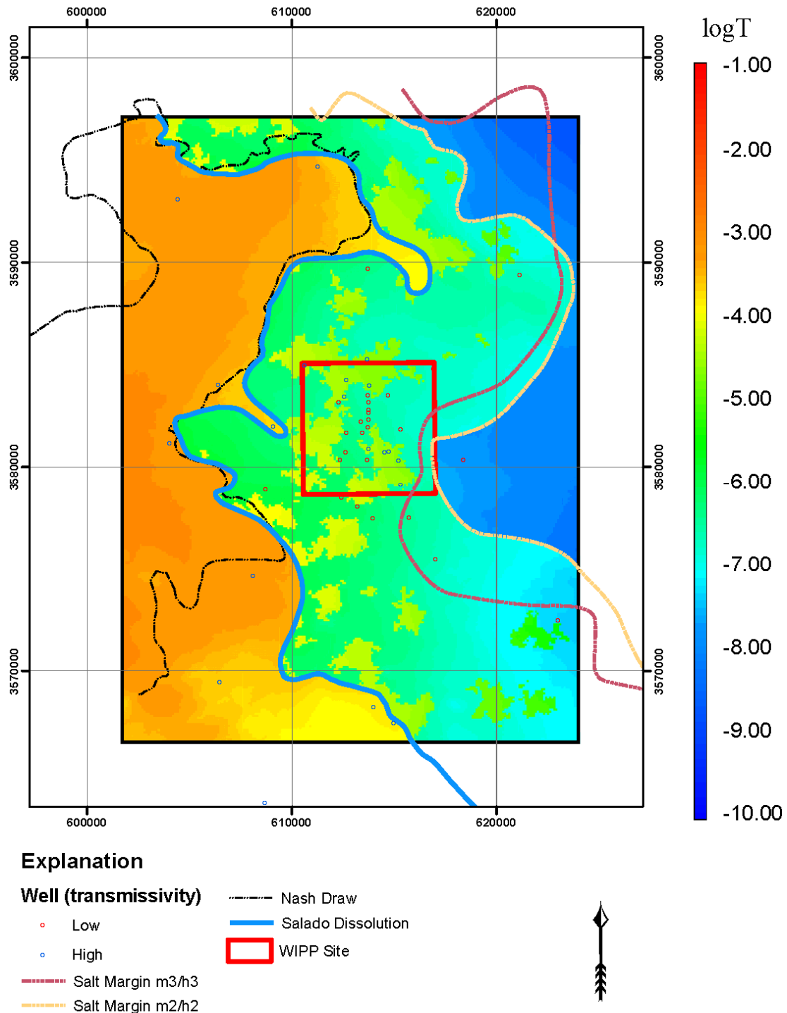
Figure TFIELD-11. Example Base T Field
