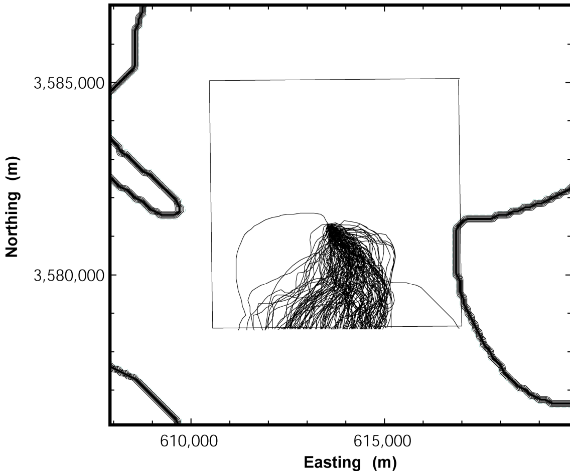
Figure TFIELD-58. All Particle Tracks Within the WIPP LWB. The Bold Lines Show the Boundaries of the High-T (Left Side) and Low-T (Right Side) Zones.
