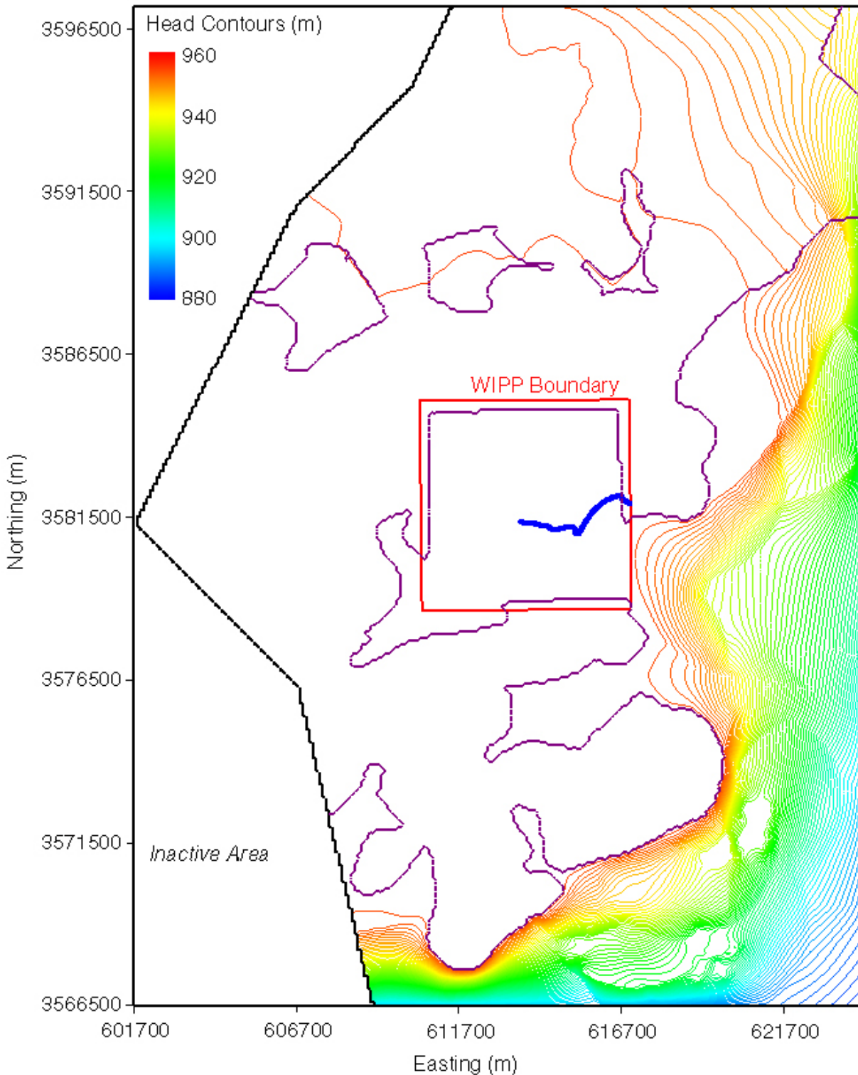
Figure TFIELD-80. Head Contours and Particle Track for the Maximum-Travel-Time T Field (d03r01-R3) for the Partial-Mining Case. The WIPP LWB is the Red Box in the Center of the Figure and the Particle Track is the Blue Track Originating from the Approximate Center of the WIPP.
