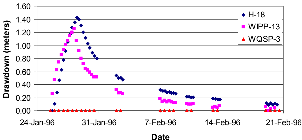
Figure TFIELD-30. Observed Drawdowns for the WQSP-1 Hydraulic Test
