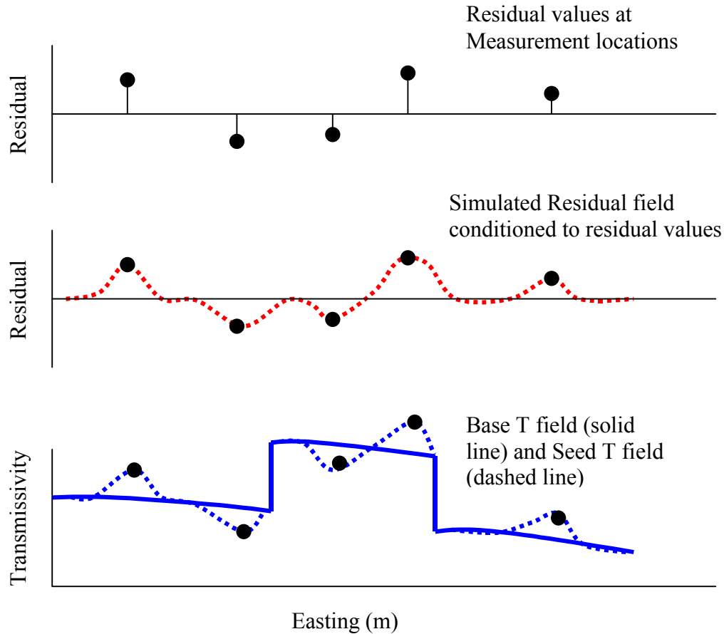
Figure TFIELD-12. Conceptual Cross Section Showing the Updating of the Residual Field and the Base T Field into the Seed T Field
