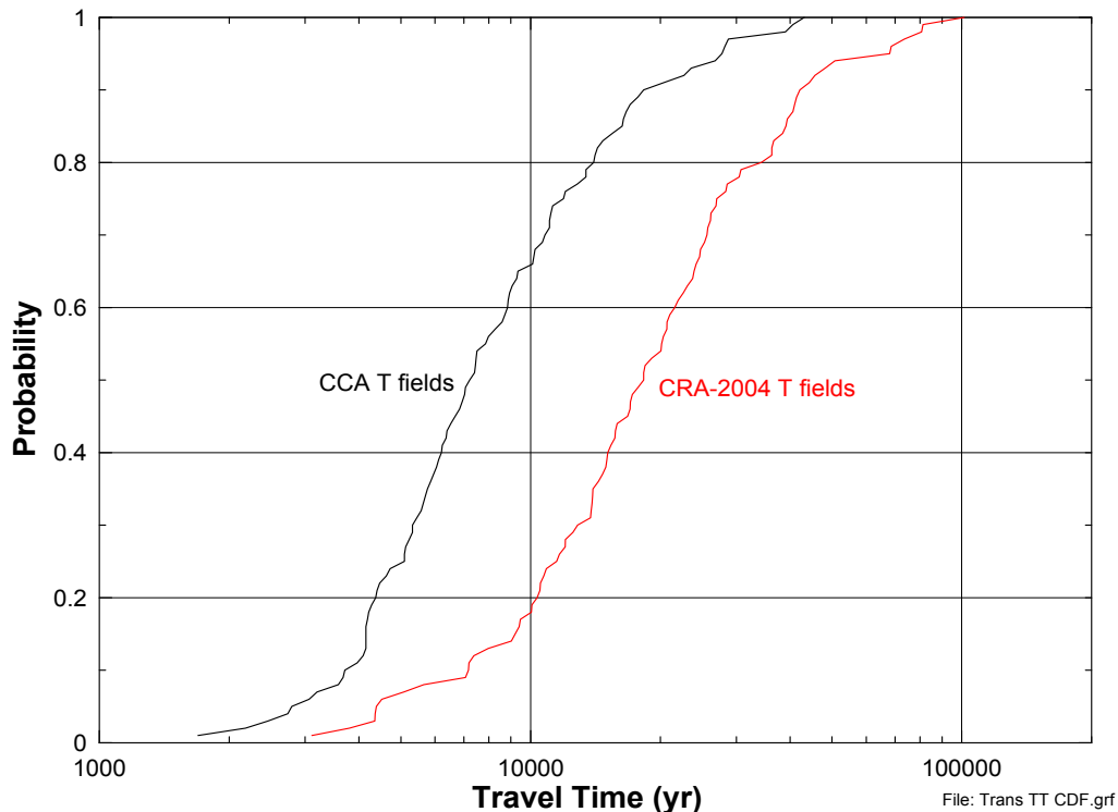
Figure TFIELD-57. Travel-Time CDFs for CCA and CRA-2004 T Fields
