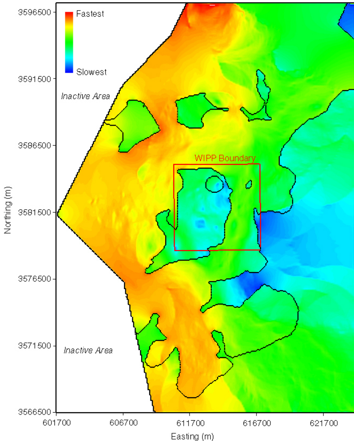
Figure TFIELD-72. Normalized Pore Velocities for the Full-Mining Case. Red Indicates Zones of High Velocity. The Black Outline Shows the Full-Mining Zones and the Red Box is the WIPP LWB. The T Field Used to Produce the Velocity Profile is Averaged Across All T Field/Replicate Combinations for the Full-Mining Scenario (300 T Fields in Total).
