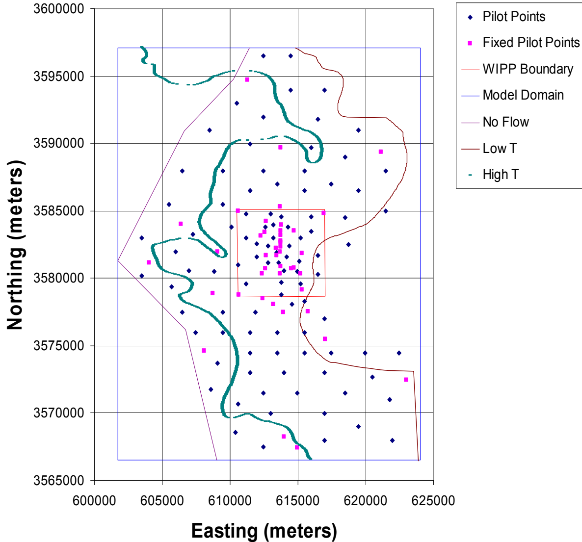
Figure TFIELD-38. Locations of the Adjustable and Fixed Pilot Points Within the Model Domain
