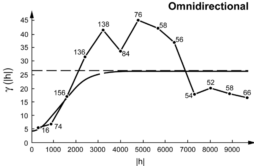
Figure TFIELD-19. Omnidirectional Experimental (Straight-Line Segments) and Model Variograms of the Head Residuals (Curves) for the 2000 Heads. The Numbers Indicate the Number of Pairs of Values That Were Used to Calculate Each Point and the Horizontal Dashed Line Denotes the Variance of the Residual Data Set.
