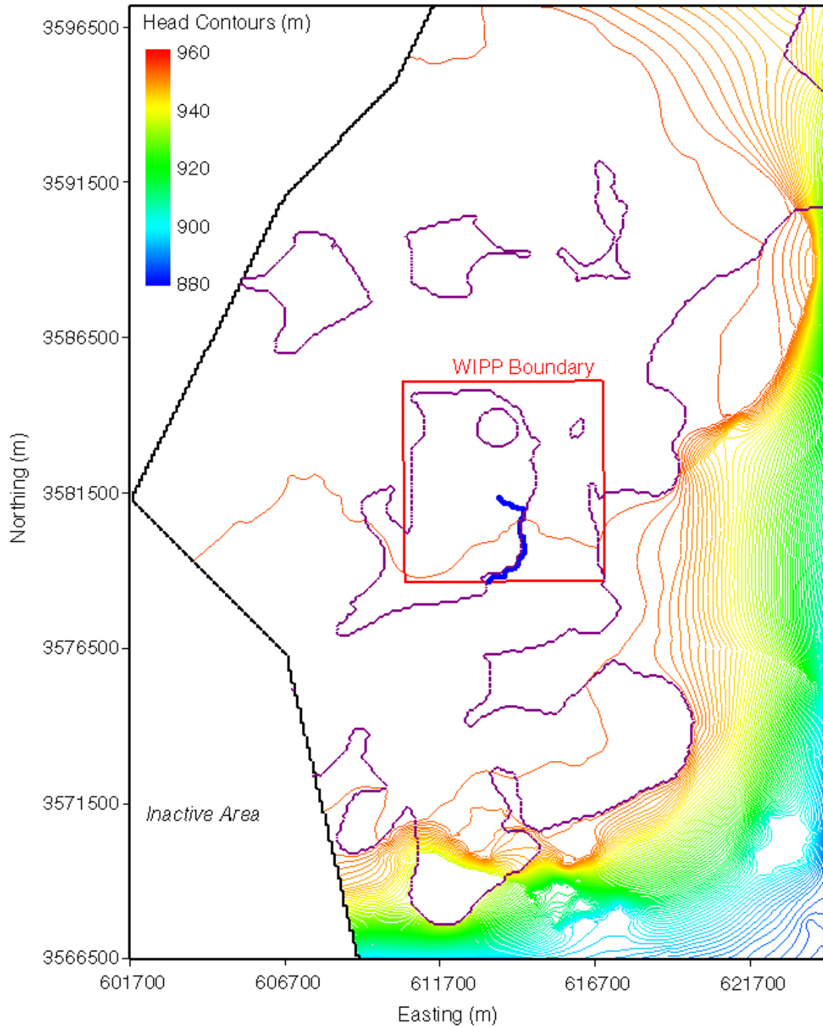
Figure TFIELD-85. Head Contours and Particle Track for the Median-Travel-Time T Field (d12r08-R3) for the Full-Mining Case. The WIPP LWB is the Red Box in the Center of the Figure and the Particle Track is the Blue Track Originating from the Approximate Center of the WIPP.
