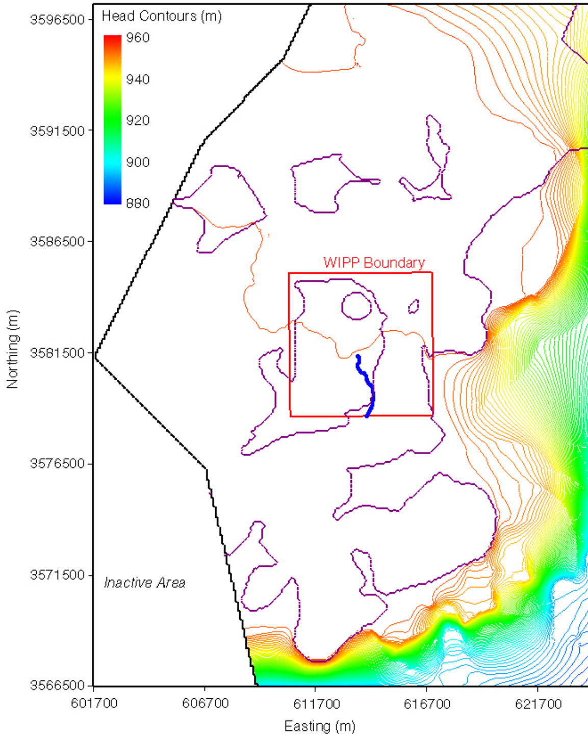
Figure TFIELD-83. Head Contours and Particle Track for the Maximum-Travel-Time T Field (d22r06-R2) for the Full-Mining Case. The WIPP LWB is the Red Box in the Center of the Figure and the Particle Track is the Blue Track Originating from the Approximate Center of the WIPP.
