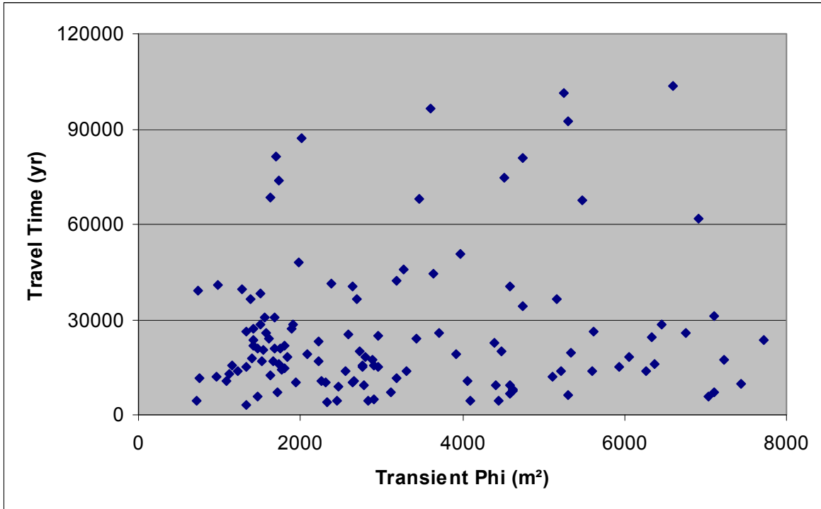
Figure TFIELD-51. Transient Phi Versus Travel Time for \Phi < 8,000 \text{ m}^2
