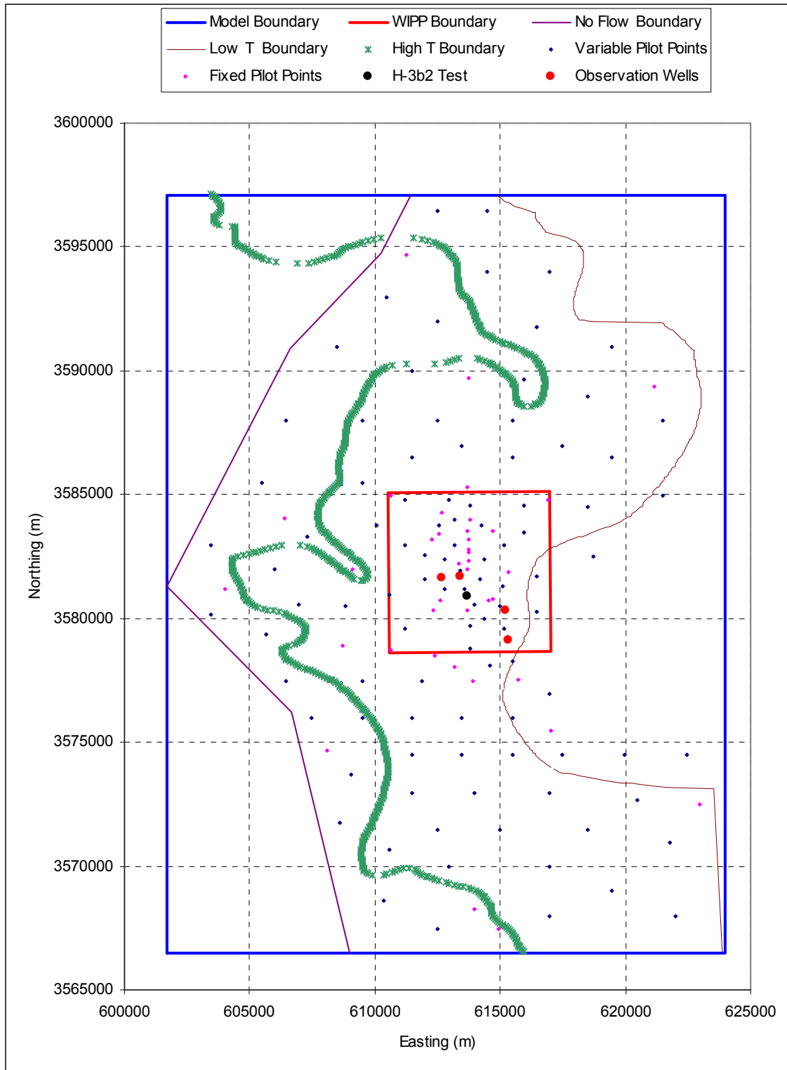
Figure TFIELD-23. Locations of the H-3b2 Hydraulic Test Well and Observation Wells
