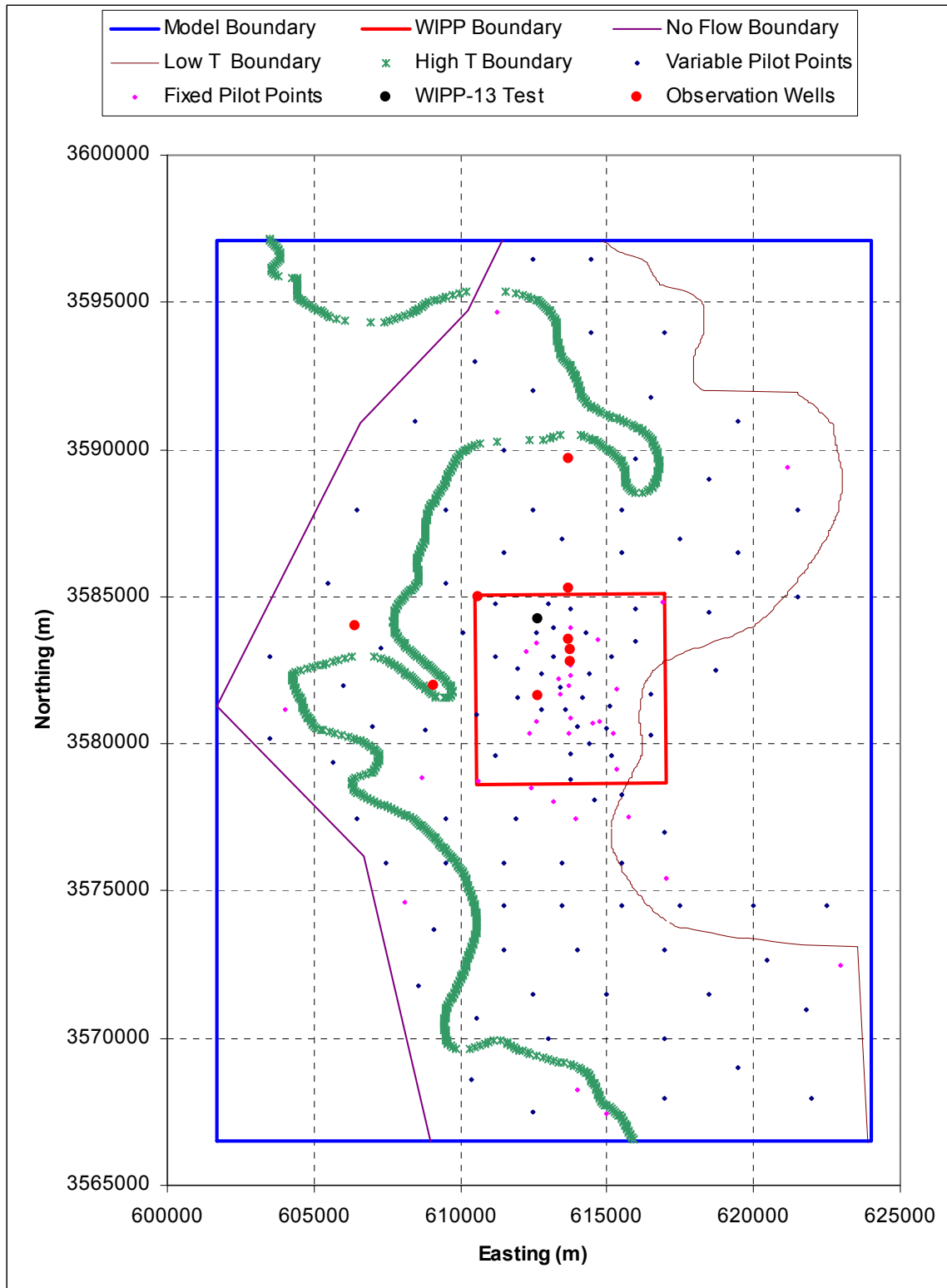
Figure TFIELD-25. Locations of the WIPP-13 Hydraulic Test Well and Observation Wells
