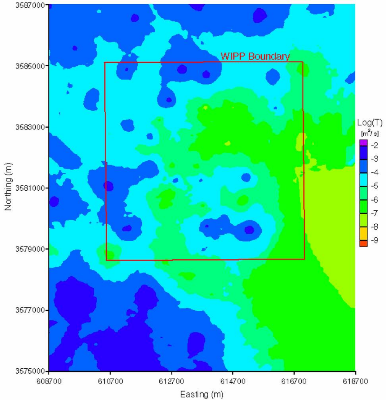
Figure TFIELD-65. Close-Up View of the Ensemble Average T Field Near the WIPP Site. Note the Different \log_{10} Color Scale from Figure TFIELD-64.
