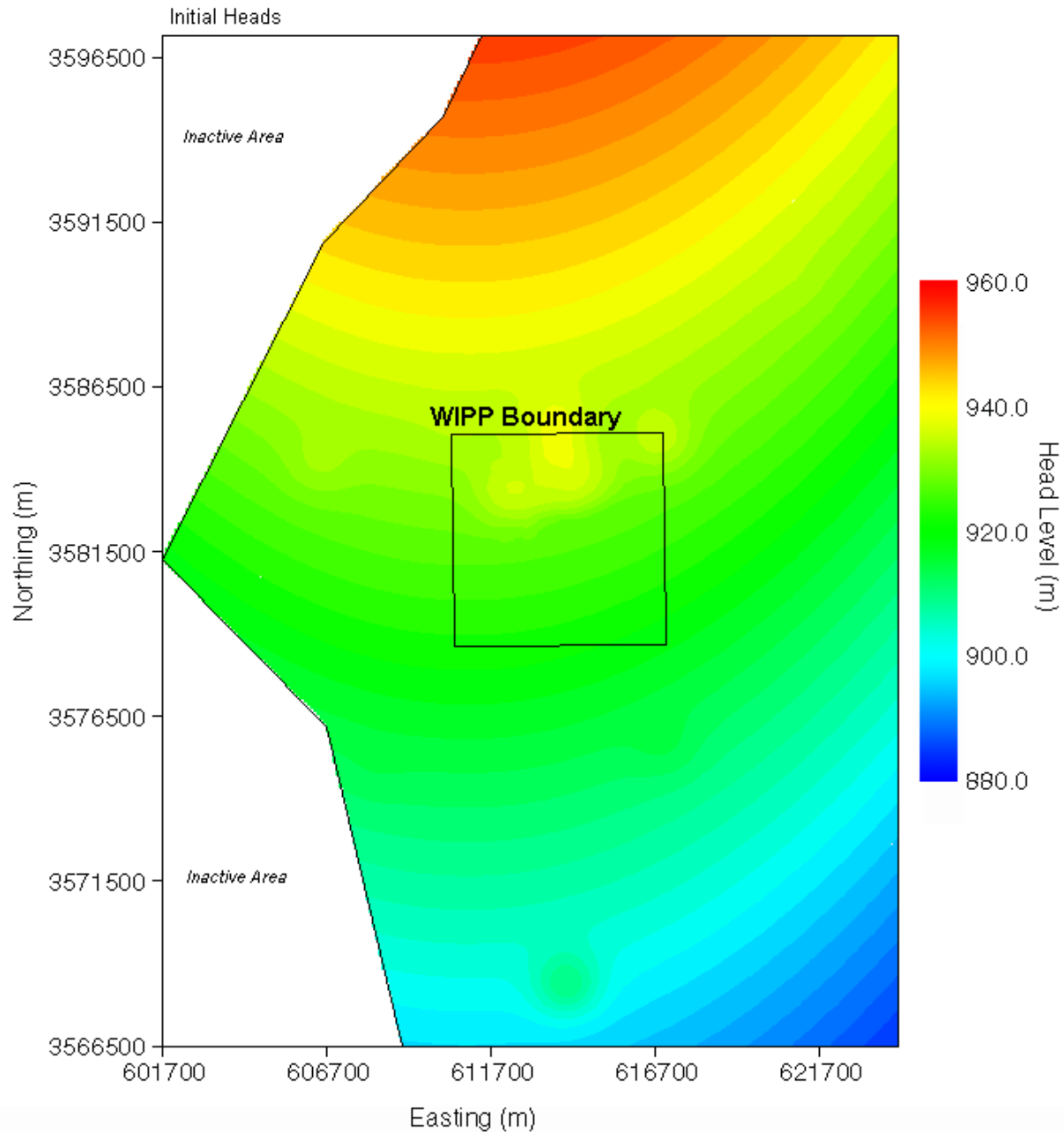
Figure TFIELD-20. Map of Initial Heads Created Through Kriging and Used to Assign Fixed-Head Boundary Conditions
