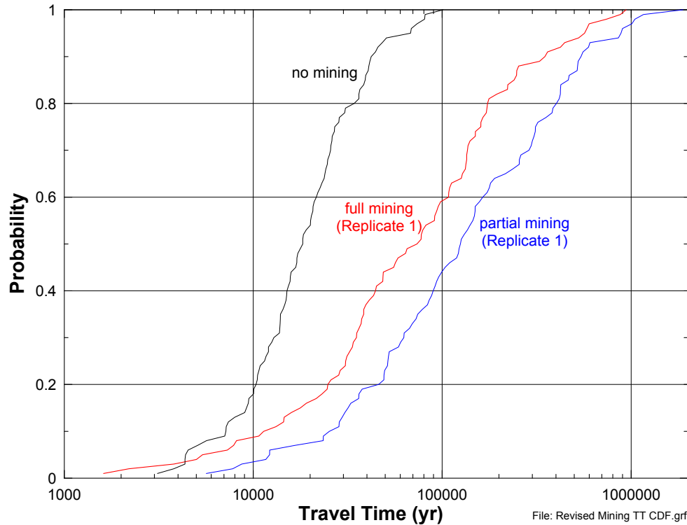
Figure TFIELD-69. CDFs of Travel Times for the Full-, Partial-, and No-Mining Scenarios
