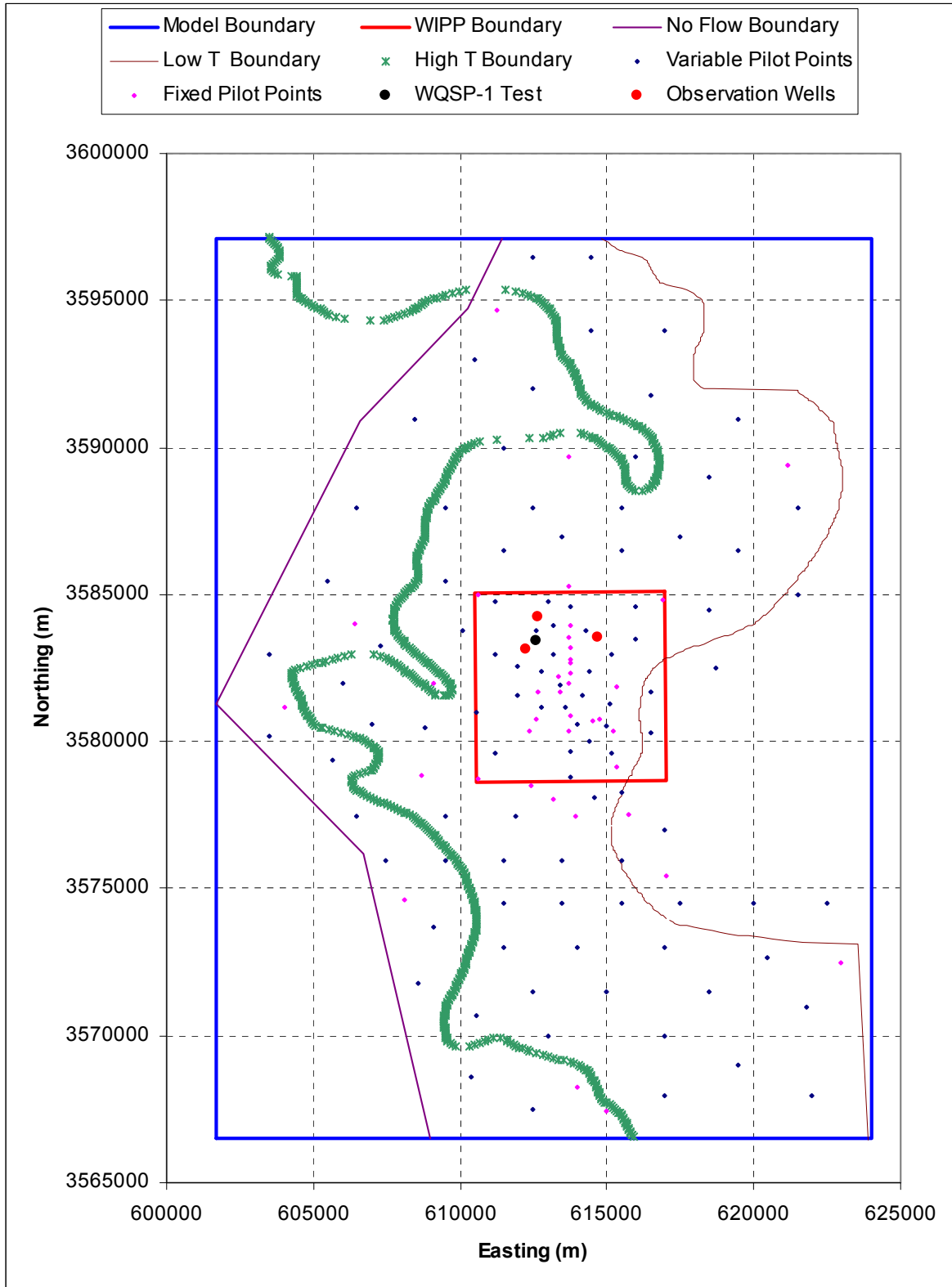
Figure TFIELD-29. Locations of the WQSP-1 Hydraulic Test Well and Observation Wells
