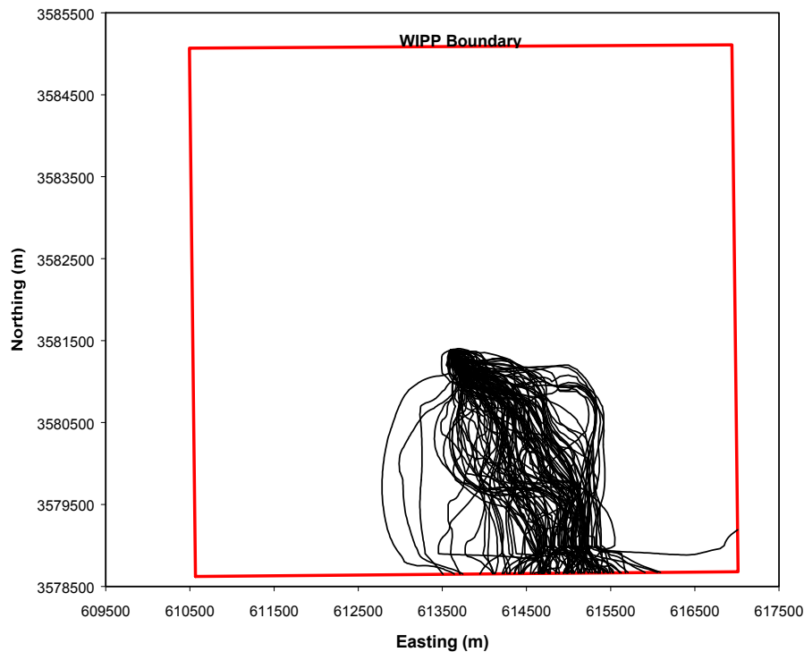
Figure TFIELD-73. Particle Tracks for Replicate 1 for the Partial-Mining Scenario
