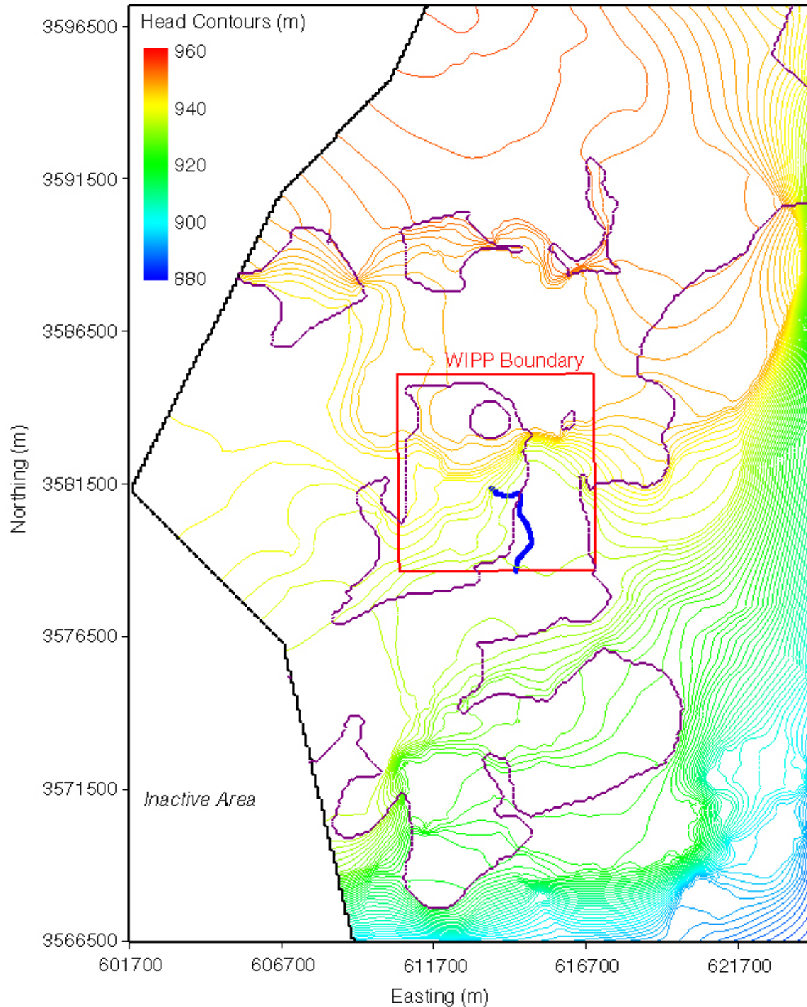
Figure TFIELD-84. Head Contours and Particle Track for the Minimum-Travel-Time T Field (d03r03-R3) for the Full-Mining Case. The WIPP LWB is the Red Box in the Center of the Figure and the Particle Track is the Blue Track Originating from the Approximate Center of the WIPP.
