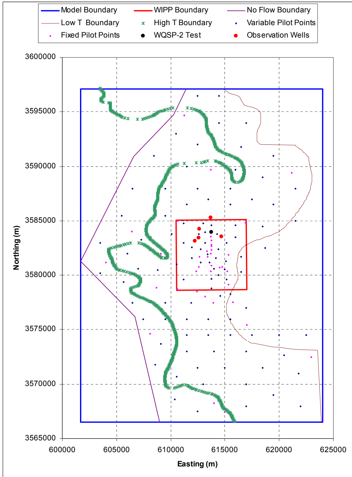
Figure TFIELD-31. Locations of the WQSP-2 Hydraulic Test Well and Observation Wells
