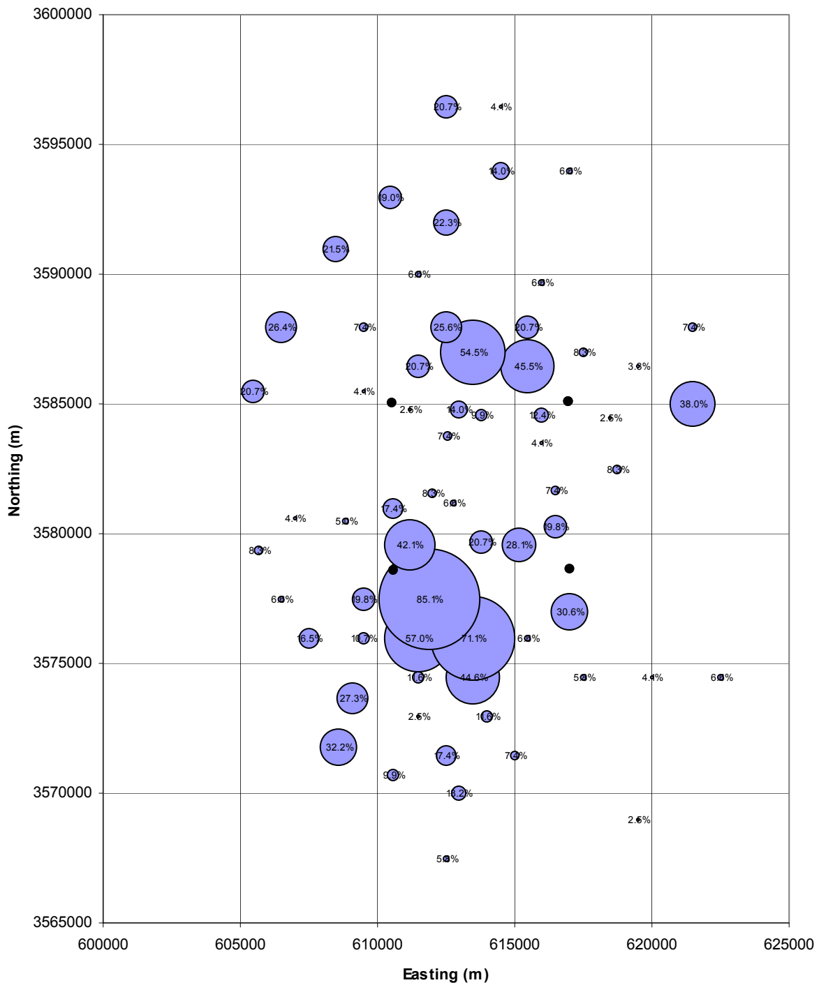
Figure TFIELD-62. Percentage of T Fields in which Pilot Points Hit Maximum Allowable Values. Corners of WIPP LWB are Shown by Unlabeled Black Dots.
