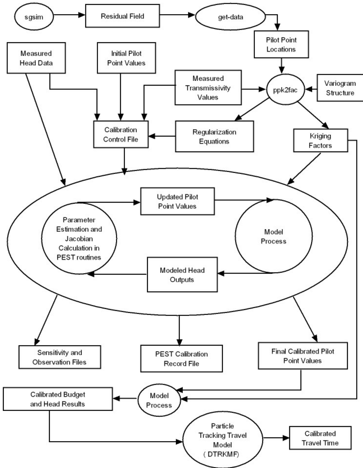
Figure TFIELD-41. Flow Chart of the Stochastic Inverse Calibration Process Used to Create the Final Calibrated T Fields
