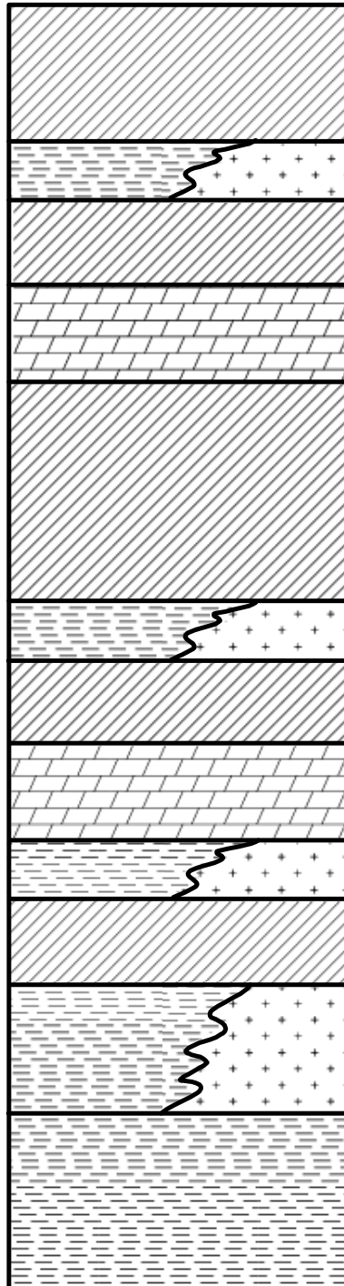
Figure TFIELD-4. Stratigraphic Subdivisions of the Rustler
