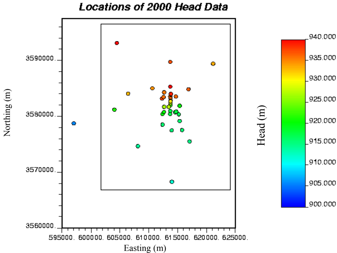
Figure TFIELD-16. Locations and Values of the 2000 Head Measurements Considered in the Steady-State Calibrations. The Approximate Extent of the Numerical Model Domain is Shown by the Black Rectangle in the Image.
