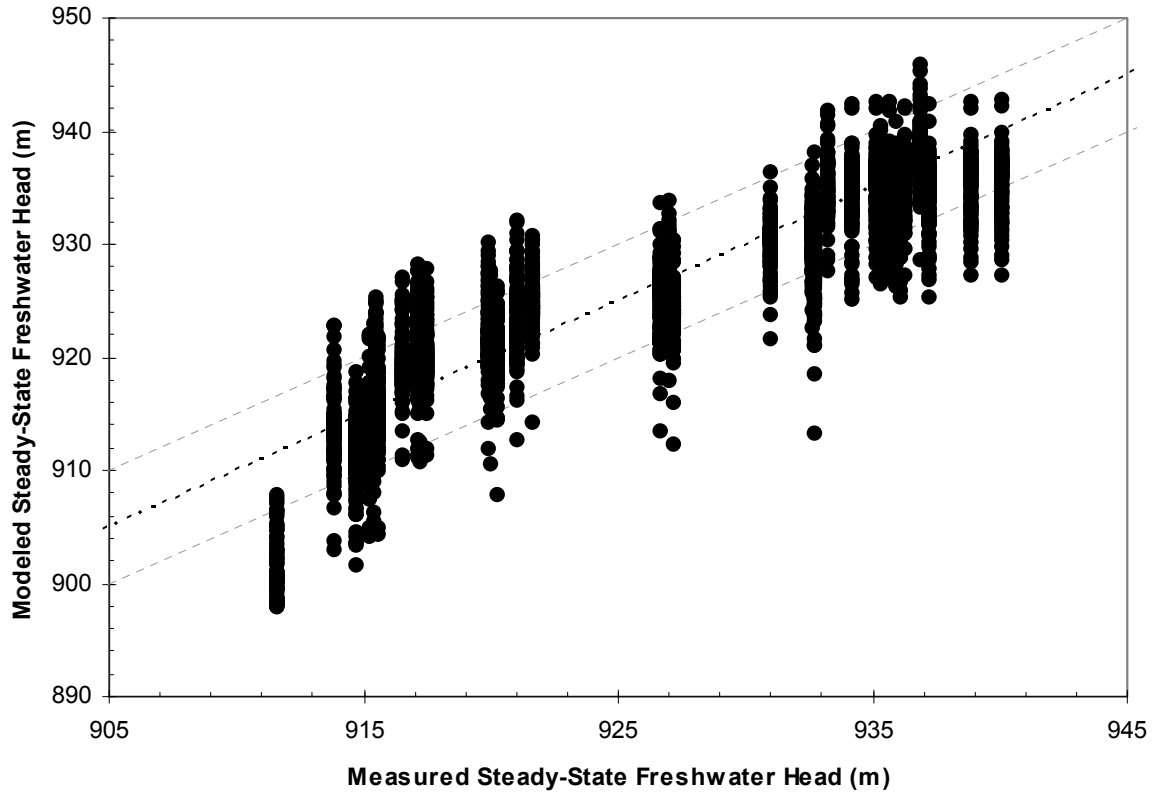
Figure TFIELD-60. Scatterplot of Measured Versus Modeled Steady-State Heads
