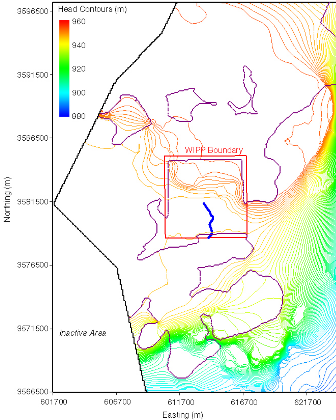
Figure TFIELD-81. Head Contours and Particle Track for the Minimum-Travel-Time T Field (d09r06-R2) for the Partial-Mining Case. The WIPP LWB is the Red Box in the Center of the Figure and the Particle Track is the Blue Track Originating from the Approximate Center of the WIPP.
