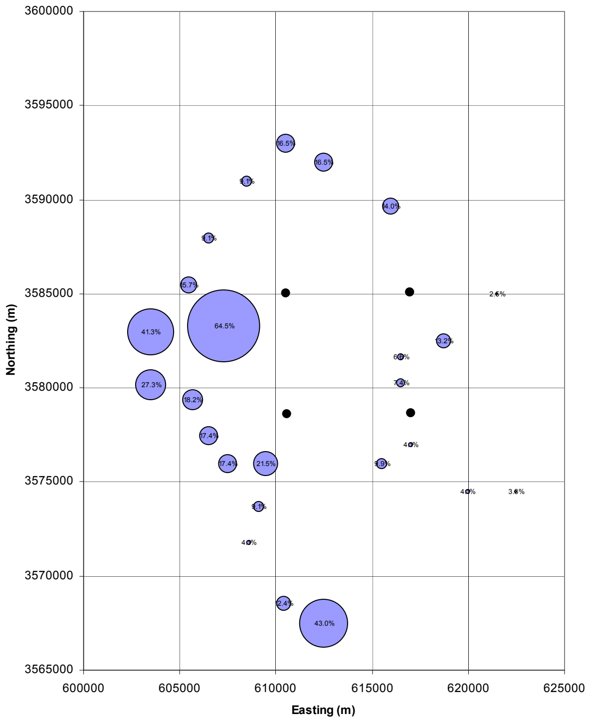
Figure TFIELD-63. Percentage of T Fields in which Pilot Points Hit Minimum Allowable Values. Corners of WIPP LWB are Shown by Unlabeled Black Dots.
