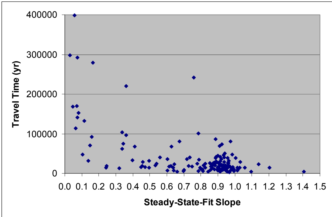
Figure TFIELD-48. Steady-State-Fit Slope Versus Travel Time for All Fields
