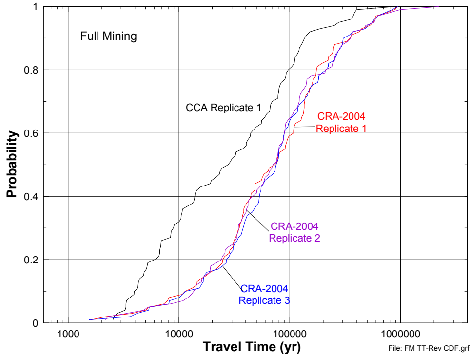
Figure TFIELD-71. CDFs of Full-Mining Travel Times for Three CRA-2004 Replicates and One CCA Replicate
