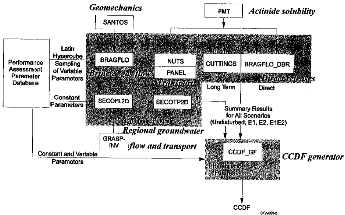
Figure 4-1. Illustration of Conceptual Model Integration
