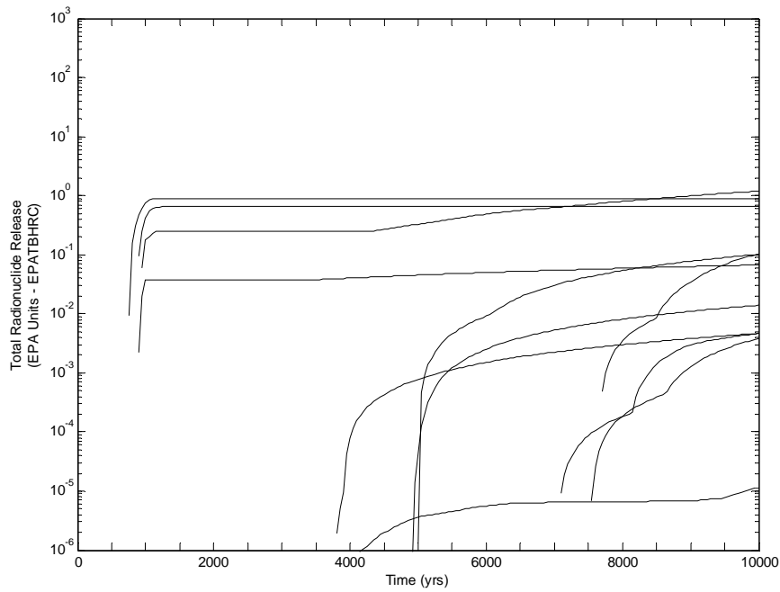
Figure 5-34. Cumulative Normalized Release Up the Borehole, Replicate R1, Scenario S4 for CRA-2004 PABC.
