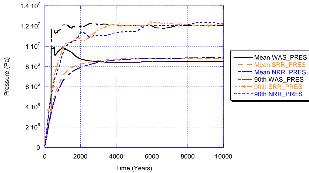
Figure 5-5. Mean And 90 th Percentile Values for Pressure in the Waste Areas Regions of the Repository, Replicate R1, Scenario S2, from the CRA-2004 PABC.
