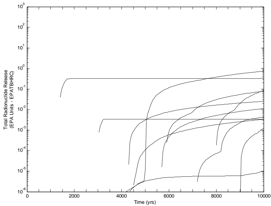
Figure 5-35. Cumulative Normalized Release Up the Borehole, Replicate R1, Scenario S5 for CRA-2004 PABC.
