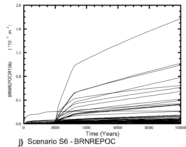
Figure 5-23 (cont). Total Cumulative Brine Outflow and Brine Flow Up the Borehole in All Scenarios, Replicate R1, CRA-2004 PABC.
