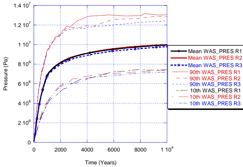
Figure 4-6. Comparison of Pressure in the Waste Panel Between All Replicates, Scenario S1, from the CRA-2004 PABC.
