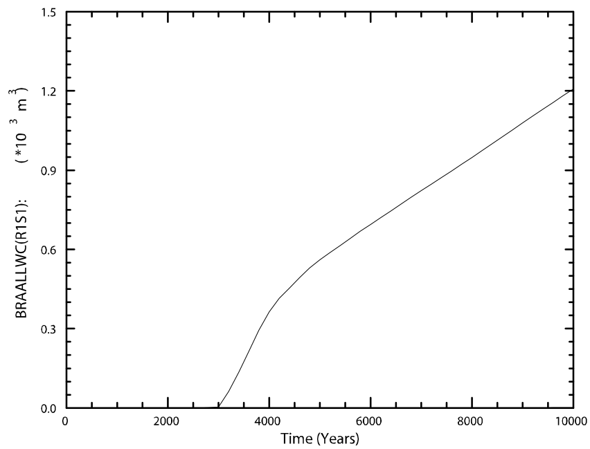
Figure 4-17. Brine Flow via All MBs across the LWB, Replicate R1, Scenario S1, from the CRA-2004 PABC.
