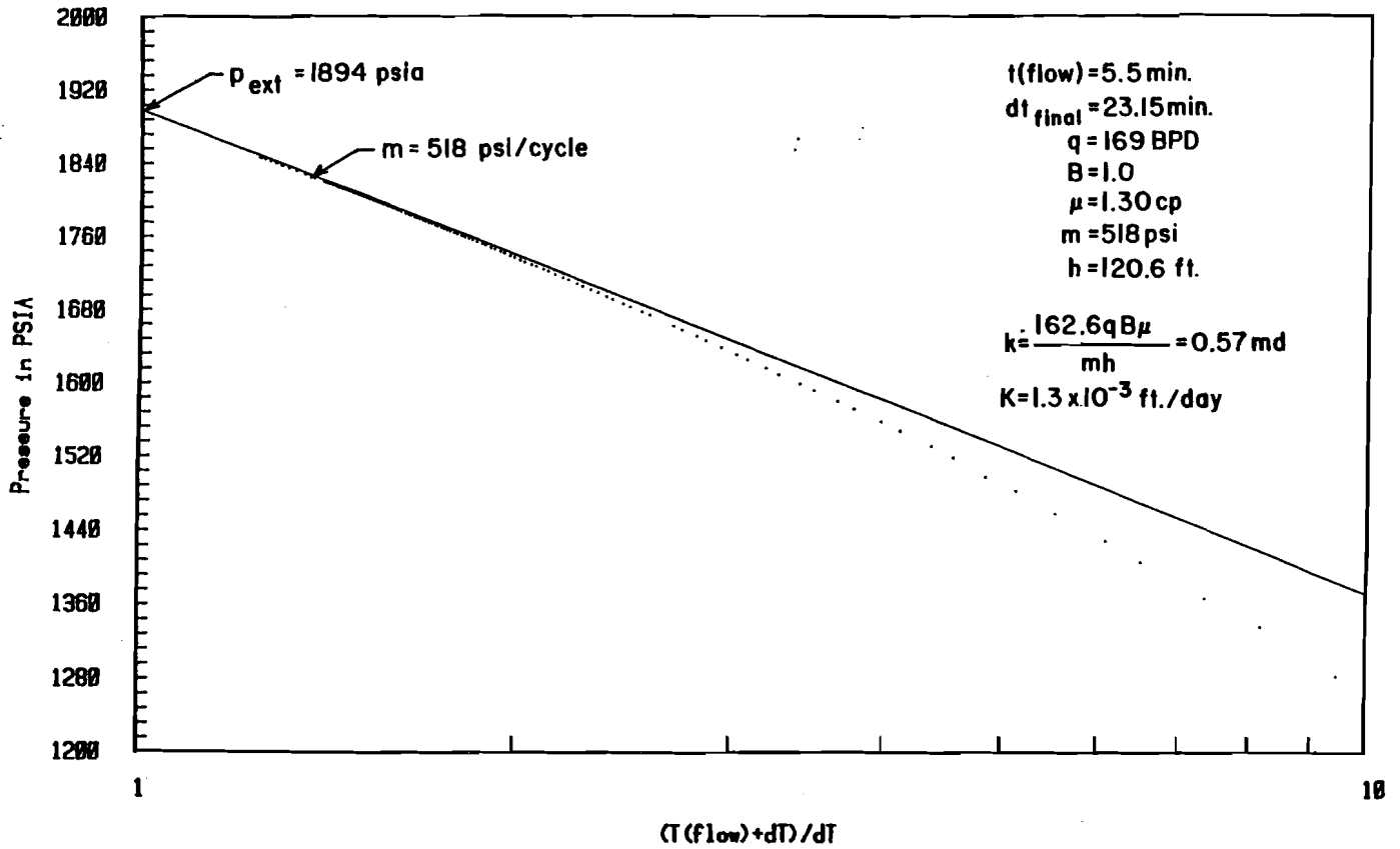
FIGURE 9 HORNER PLOT OF DST-4178/FBU
