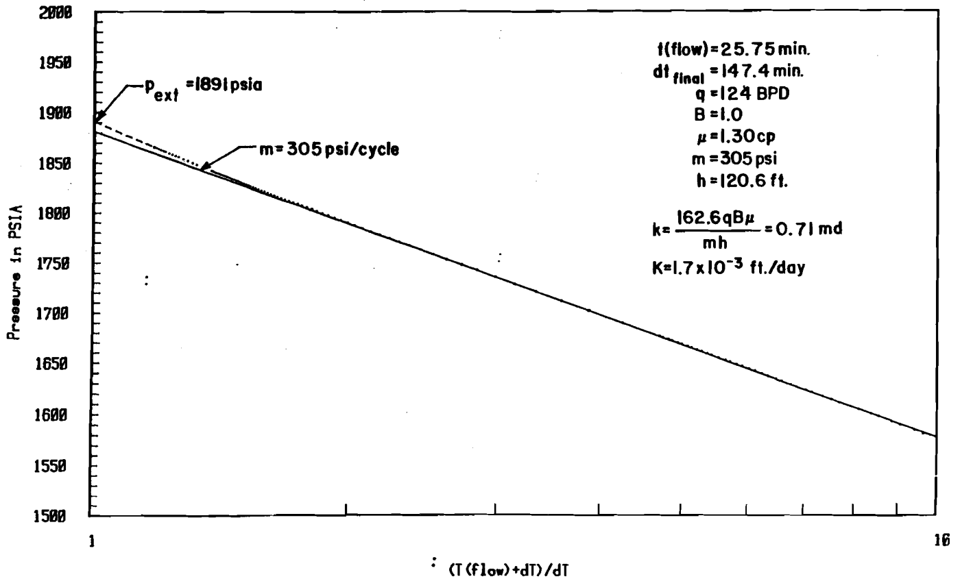
FIGURE 10 HORNER PLOT OF DST-4178/SBU
