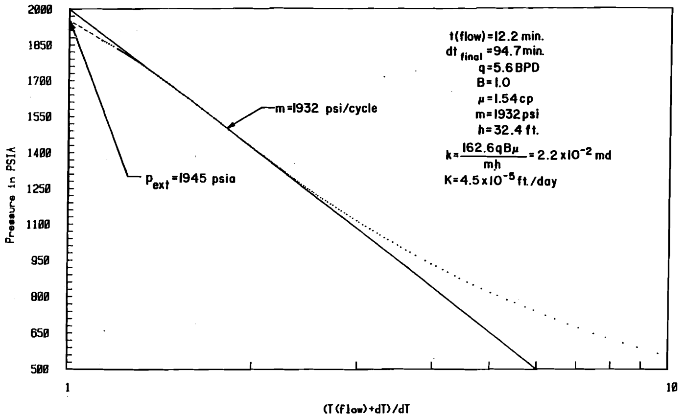
FIGURE 14 HORNER PLOT OF DST-4138/FBU
