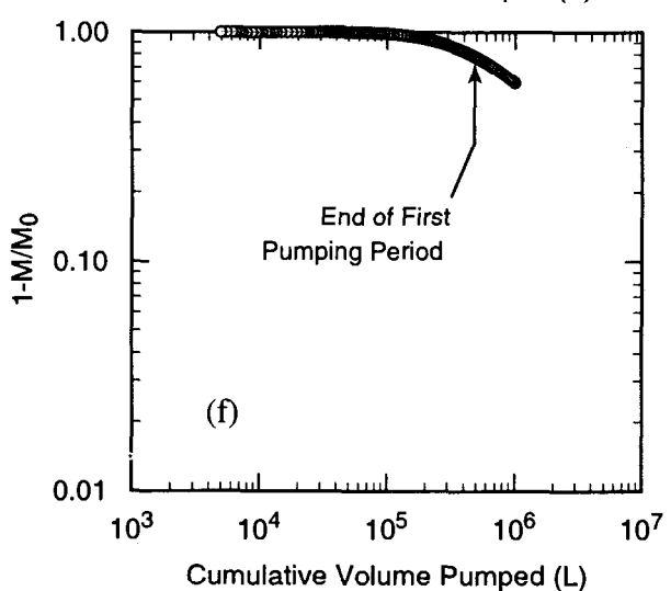
Figure C-27. 2,6-DFBA data from H-11b2 to H-11b1 pathway, H-11 1996 test, round 1 (Q=0.22 L/s).
