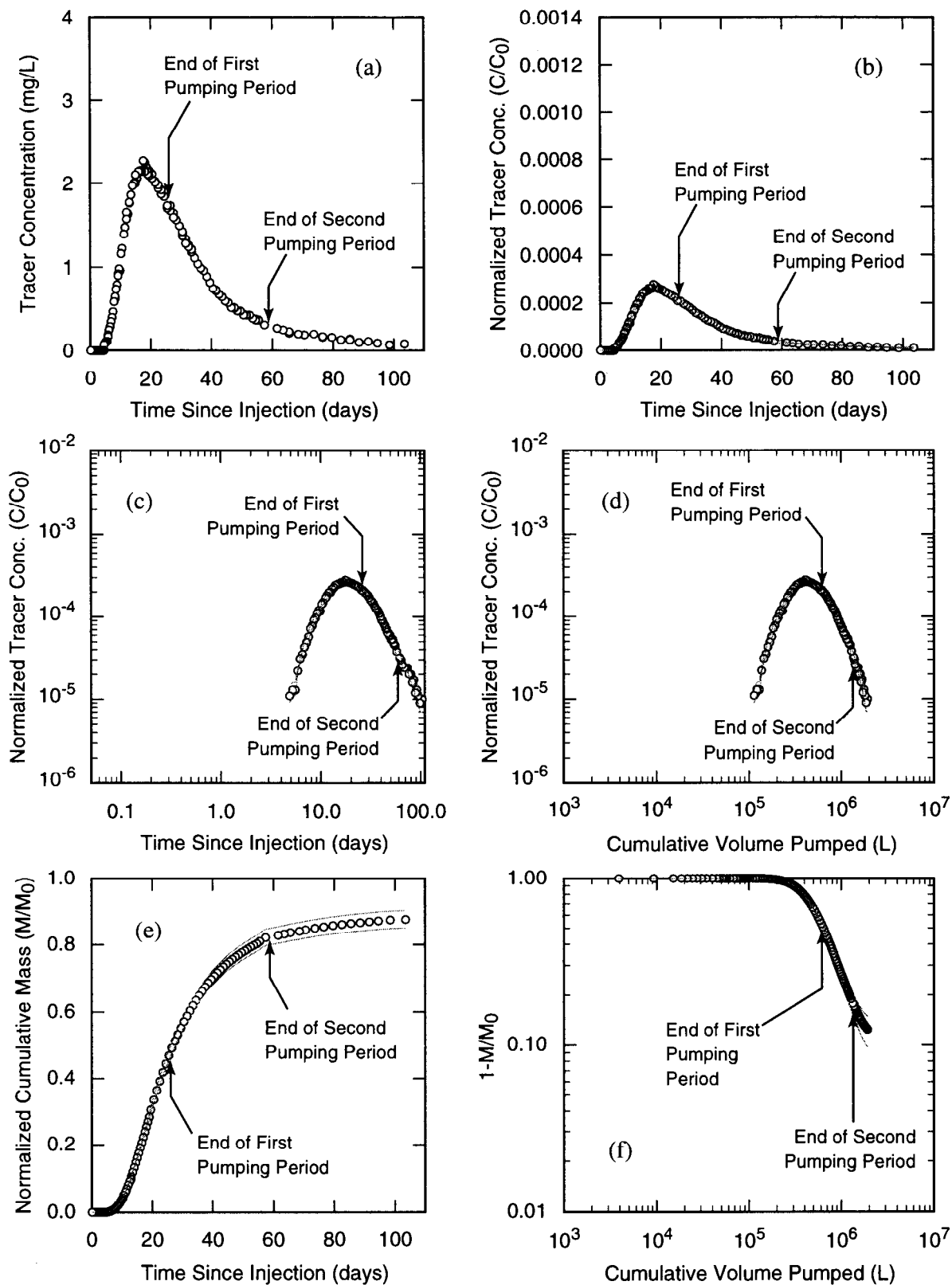
Figure C-2. 2,3,4-TFBA data from H-19b2 to H-19b0 pathway, H-19 7-well test, round 1 ( Q=0.27 L/s), full Culobra injection.
