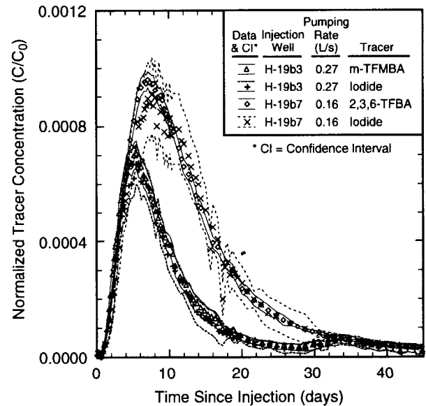
Figure 3-10. Comparison of benzoic-acid and iodide data for (a) one pathway at H-11 and (b) two pathways at H-19.
