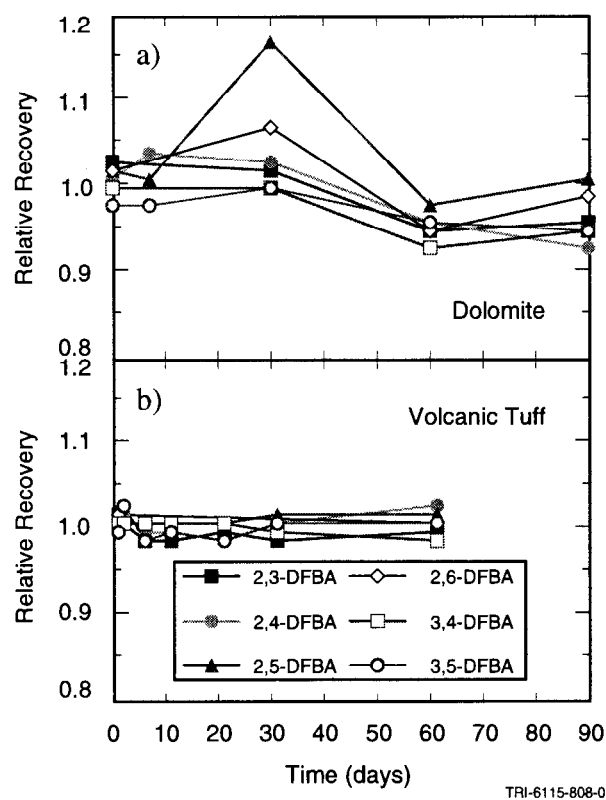
Figure H-3. Results of batch tests for difluorobenzoates in (a) dolomite and (b) volcanic tuff.
