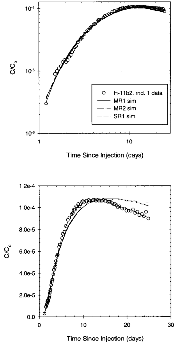
Figure S-16 Single-rate and multirate diffusion transport model calibrations to the tracer-breakthrough curve for the H-11 hydropad, pathway H-11b2 to H-11b1, for Round 1 pumping rate, benzoic-acid tracer.
