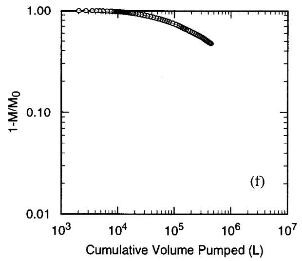
Figure C-31. Iodide data from H-11b3 to H-11b1 pathway, H-11 1996 test, round 2 ( Q=0.38 L/s) analyzed using a high performance liquid chromatograph.
