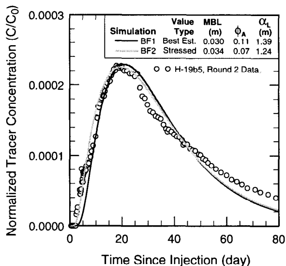
Figure P-5. Observed and simulated tracer-breakthrough curves for the H-19b5 Round 2 data. Simulations show the best fits to the observed data assuming both best-estimate (black curve) and stressed (gray curve) values for the fixed parameters. All simulations assumed a homogeneous hydraulic-conductivity field.
