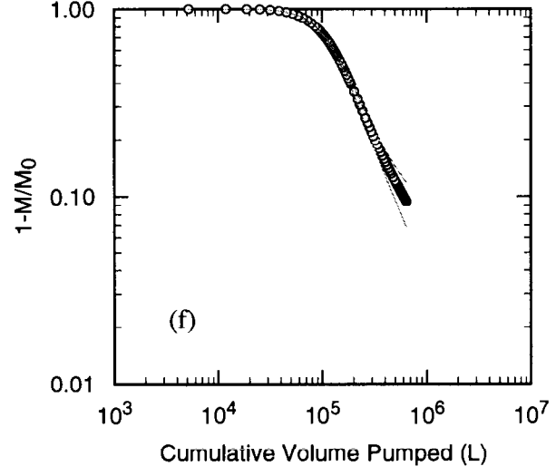
Figure C-17. 2,3,6-TFBA data from H-19b7 to H-19b0 pathway, H-19 7-well test, round 3 (Q=0.16 L/s), full Culebra injection.
