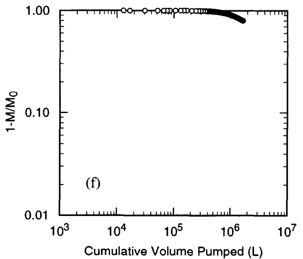
Figure C-35. m-TFMBA data from H-6a to H-6c pathway, H-6 1981 test 1 (Q=1.04 L/s).
