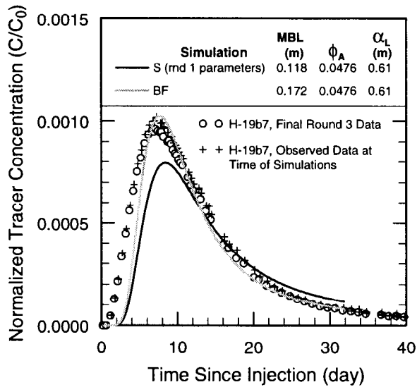
Figure P-7. Observed and simulated tracer-breakthrough curves for the H-19b7 Round 3 data. Two sets of observed data are shown; one set is the final data (open circles) and the other set is the data at the time of the simulations (plus signs). Simulations show the results predicted for the Round 3 data using the parameter values determined from calibration to the Round 1 data (black curve) and the best fit to the Round 3 data (gray curve). All simulations assumed best-estimate values for the fixed parameters and a homogeneous hydraulic-conductivity field.
