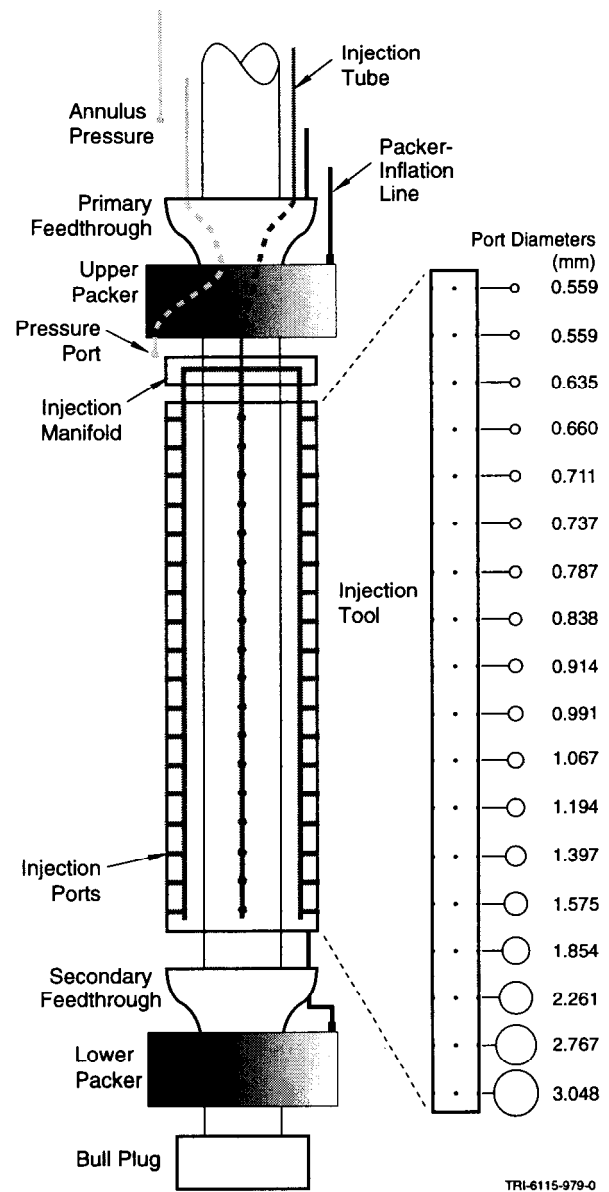
Figure D-9. Downhole equipment in H-19b2, H-19b4, and H-19b6 during the 1995-96 7-well tracer test.
