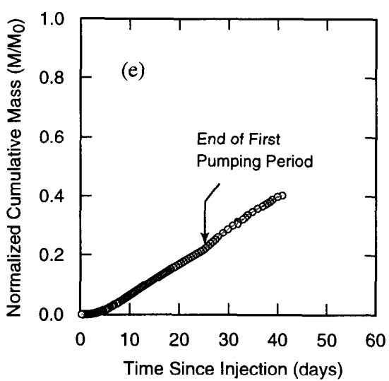
Figure C-27. 2,6-DFBA data from H-11b2 to H-11b1 pathway, H-11 1996 test, round 1 (Q=0.22 L/s).
