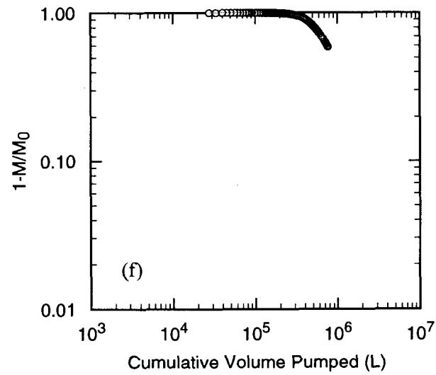
Figure C-24. 2,6-DFBA data from H-19b4 to H-19b0 pathway, H-19 4-well test (Q=0.24 L/s).
