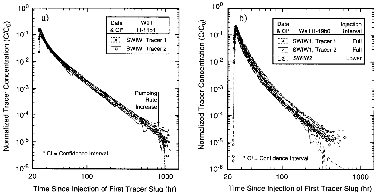
Figure 3-3. SWIW tracer-recovery curves from (a) one test at the H-11 hydropad and (b) two tests at the H-19 hydropad.
