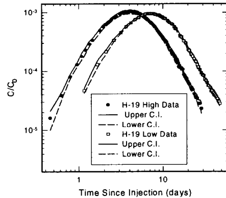
Figure 7-3. Observed breakthrough curve data and the limits of the 95% confidence intervals for the two H-19b7 to b0 tracer tests.
