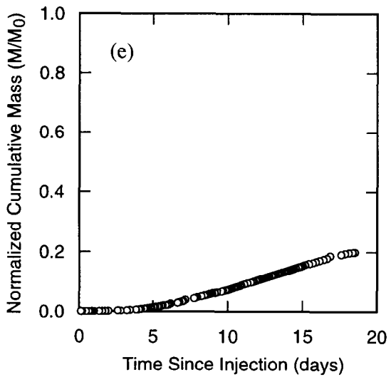
Figure C-35. m-TFMBA data from H-6a to H-6c pathway, H-6 1981 test 1 (Q=1.04 L/s).
