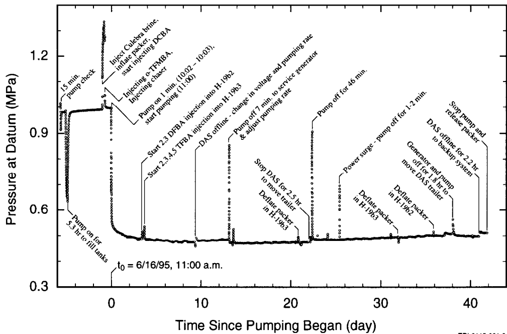
Figure D-13. H-19b0 Culebra pressure (P2) during the 1995 4-well tracer test.
