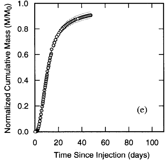
Figure C-17. 2,3,6-TFBA data from H-19b7 to H-19b0 pathway, H-19 7-well test, round 3 (Q=0.16 L/s), full Culebra injection.
