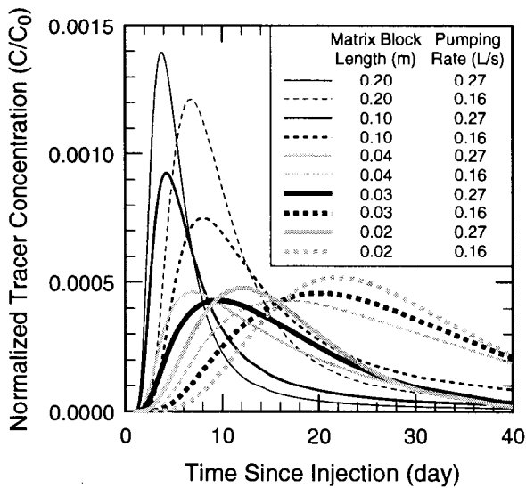
Figure P-3. Sensitivity of the simulated results from a conventional double-porosity model to a reduction in the pumping rate as a function of the matrix-block length.
