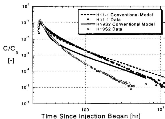
Figure 6-2. Best fits of conventional double-porosity models to the H11-1 and H19S2 data. Parameters are given in Table 6-2.
