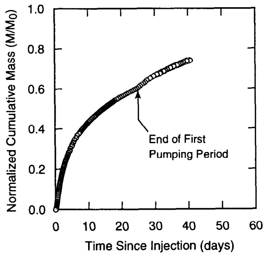
Figure C-28. 2,3,4,5-TFBA data from H-11b3 to H-11b1 pathway, H-11 1996 test, round 1 ( Q=0.22 L/s).
