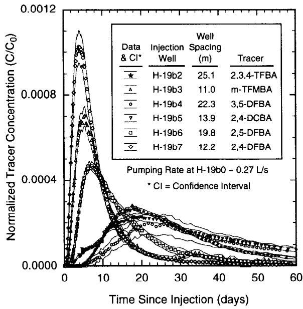
Figure 3-8. MWCF tracer-breakthrough curves from full-thickness injections for the high-pumping-rate H-19 hydrograd data.
