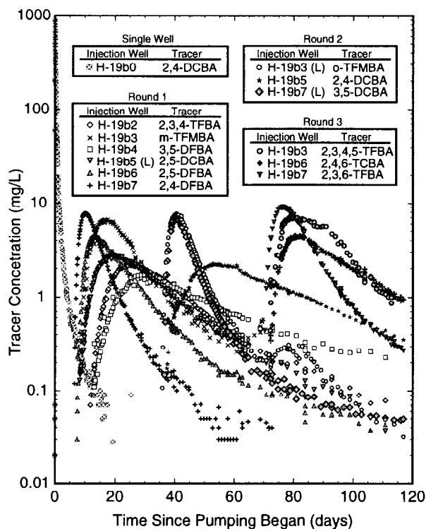
Figure H-8. Breakthrough curves for tracers used at H-19 at WIPP. Not shown are the tracers used in the less transmissive zone (2,3-DCBA, PFBA, p-TFMBFA) and the tracers used in the preliminary test (2,6-DFBA, 2,3-DFBA, 2,3,4,5-Te FBA and 2,6-DCBA).
