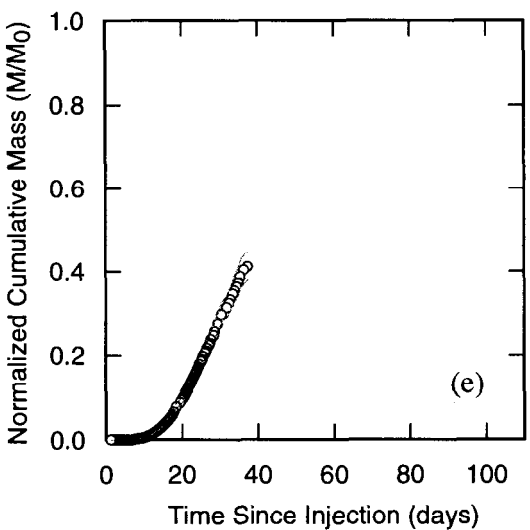
Figure C-24. 2,6-DFBA data from H-19b4 to H-19b0 pathway, H-19 4-well test (Q=0.24 L/s).
