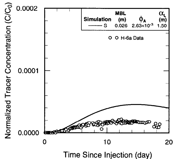
Figure P-20. Observed and simulated tracer-breakthrough curves for the H-6a Test #1 m-TFMB data. The simulation shows the best match to the observed data assuming best-estimate values for the fixed parameters and a homogeneous hydraulic-conductivity field.
