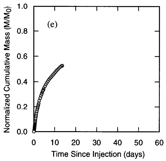
Figure C-31. Iodide data from H-11b3 to H-11b1 pathway, H-11 1996 test, round 2 ( Q=0.38 L/s) analyzed using a high performance liquid chromatograph.
