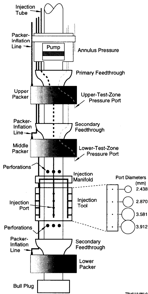
Figure D-7. Downhole equipment in H-19b0 during the 1995-96 7-well tracer test.
