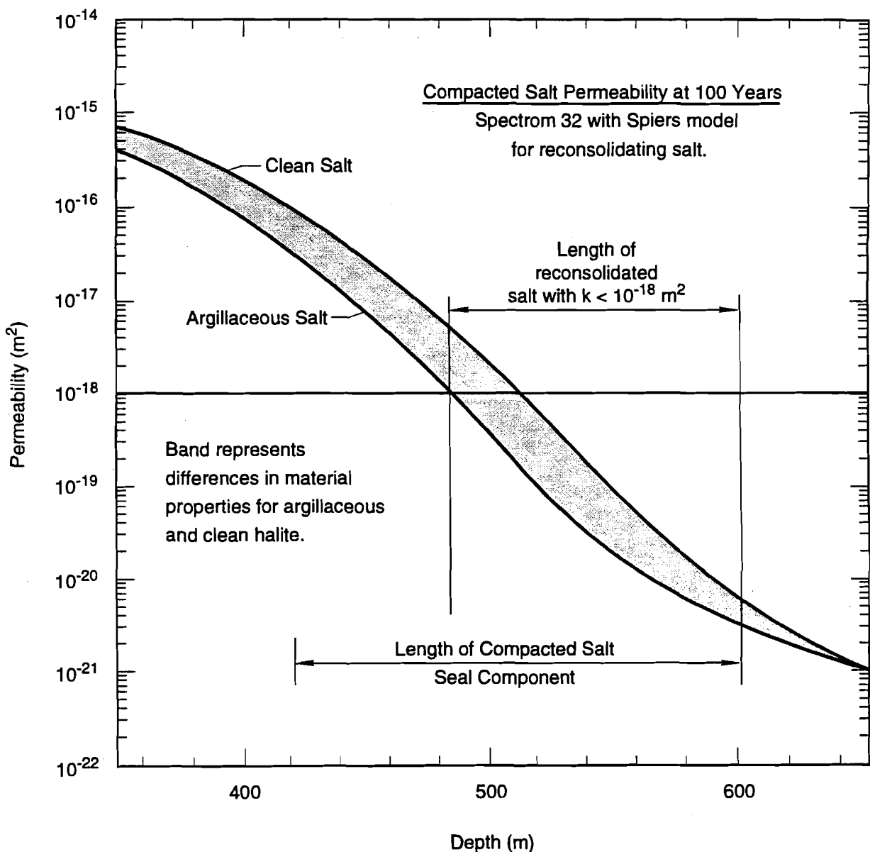
Figure 4-2. Estimated permeability of the Salado salt column at 100 years.
