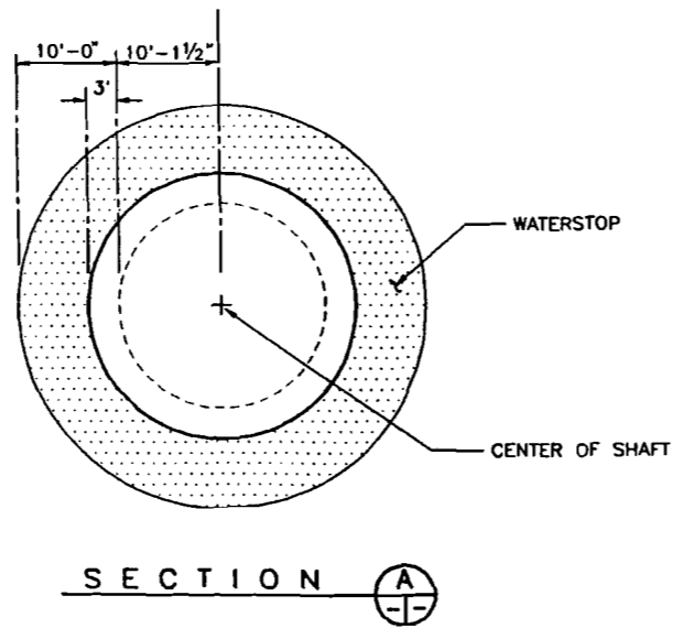
TYPICAL SALADO MASS CONCRETE PLUG WITH WATERSTOP (3 LOCATIONS)
