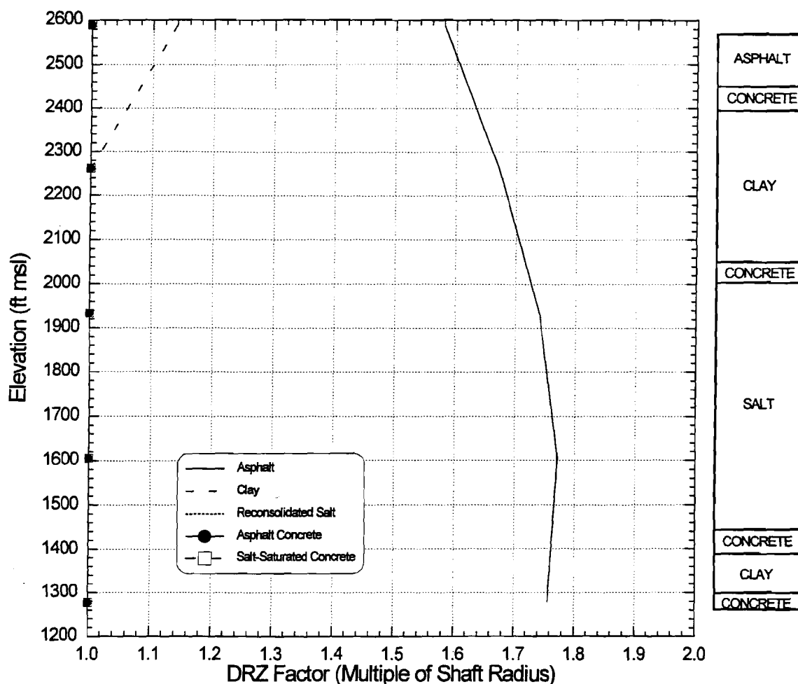
Figure D-7. Maximum DRZ extent at 100 years after closure.
