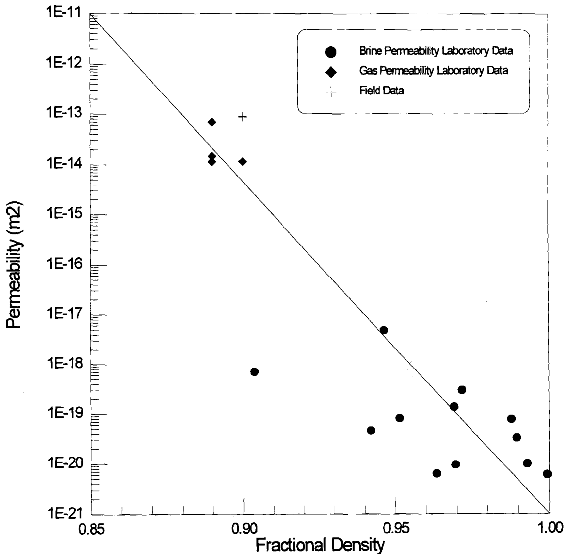
Figure D-8. Knowles-Hansen fractional density versus permeability relationship for WIPP crushed salt.
