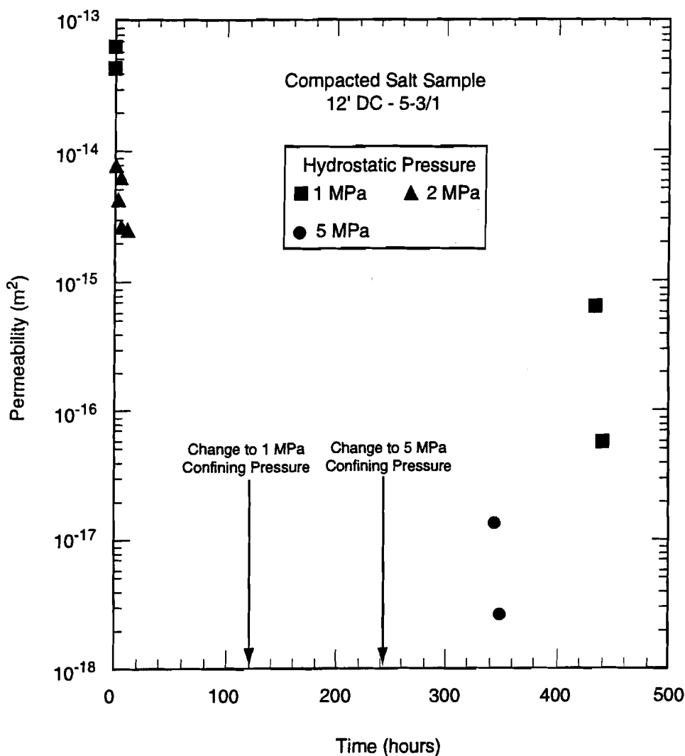
Figure 4-1. Permeability of compacted salt at low hydrostatic stresses.
