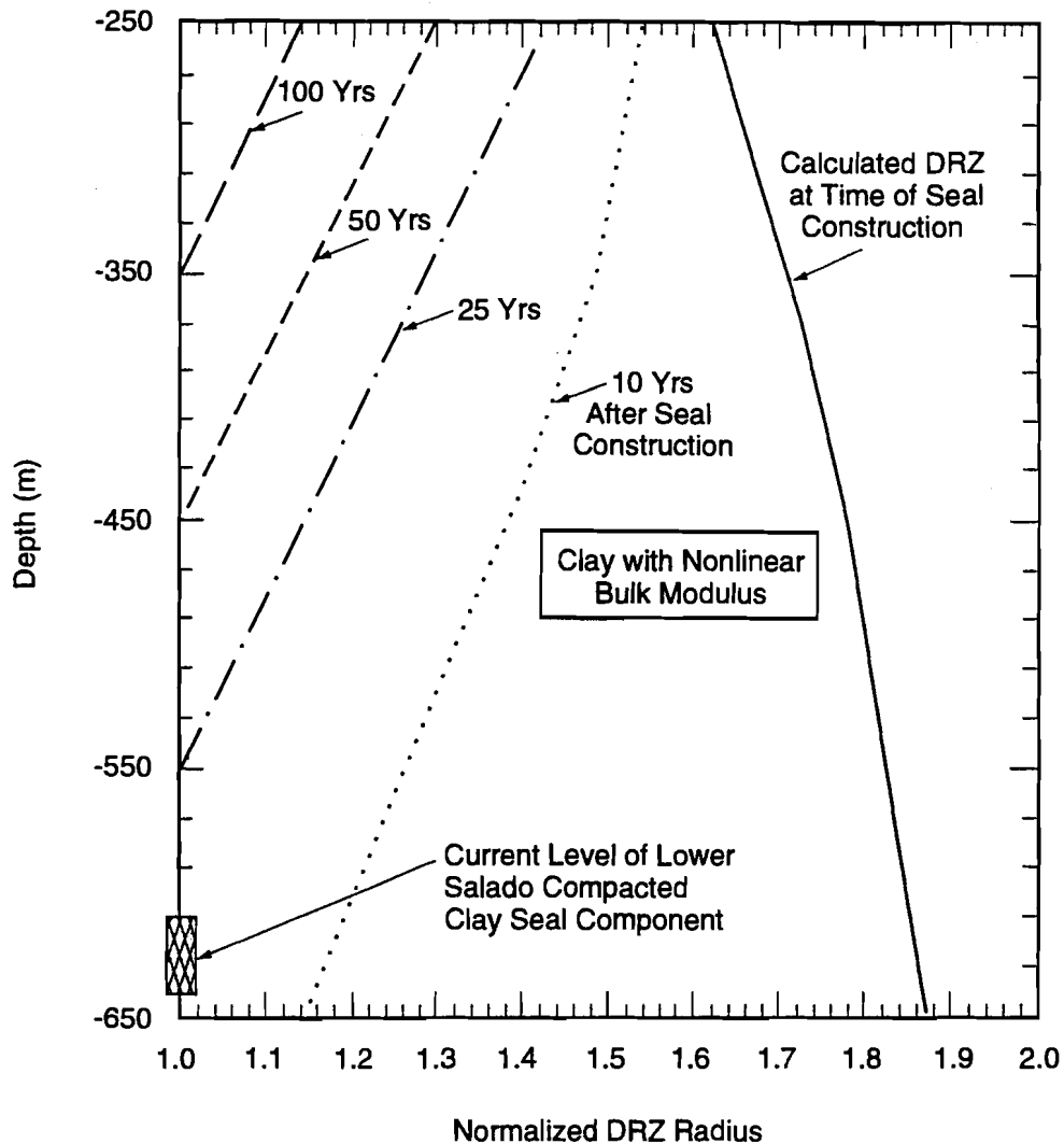
Figure 4-3. Extent of DRZ at various depths within the shaft.
