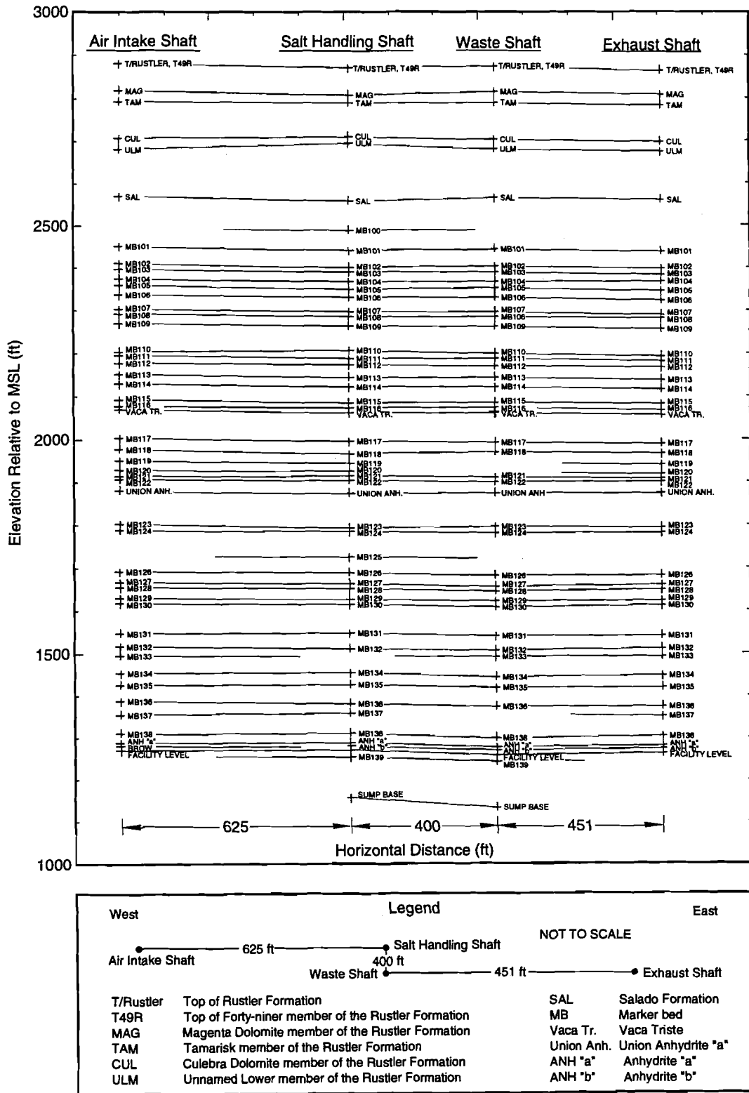
Figure 2. Structural Cross-section through excavated shafts, top of Rustler Formation to total depth.
