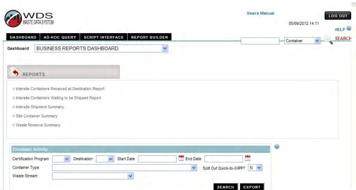
Figure 6-M – Business Reports Dashboard
