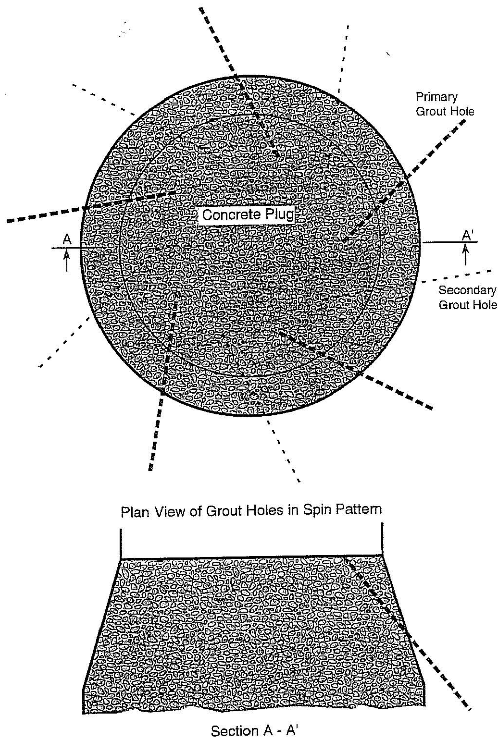
Figure I2-9 Plan and section views of downward spin pattern of grout holes
