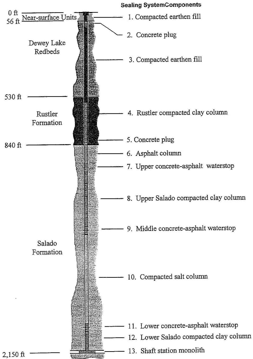
Figure I2- Arrangement of the Air Intake Shaft sealing system
