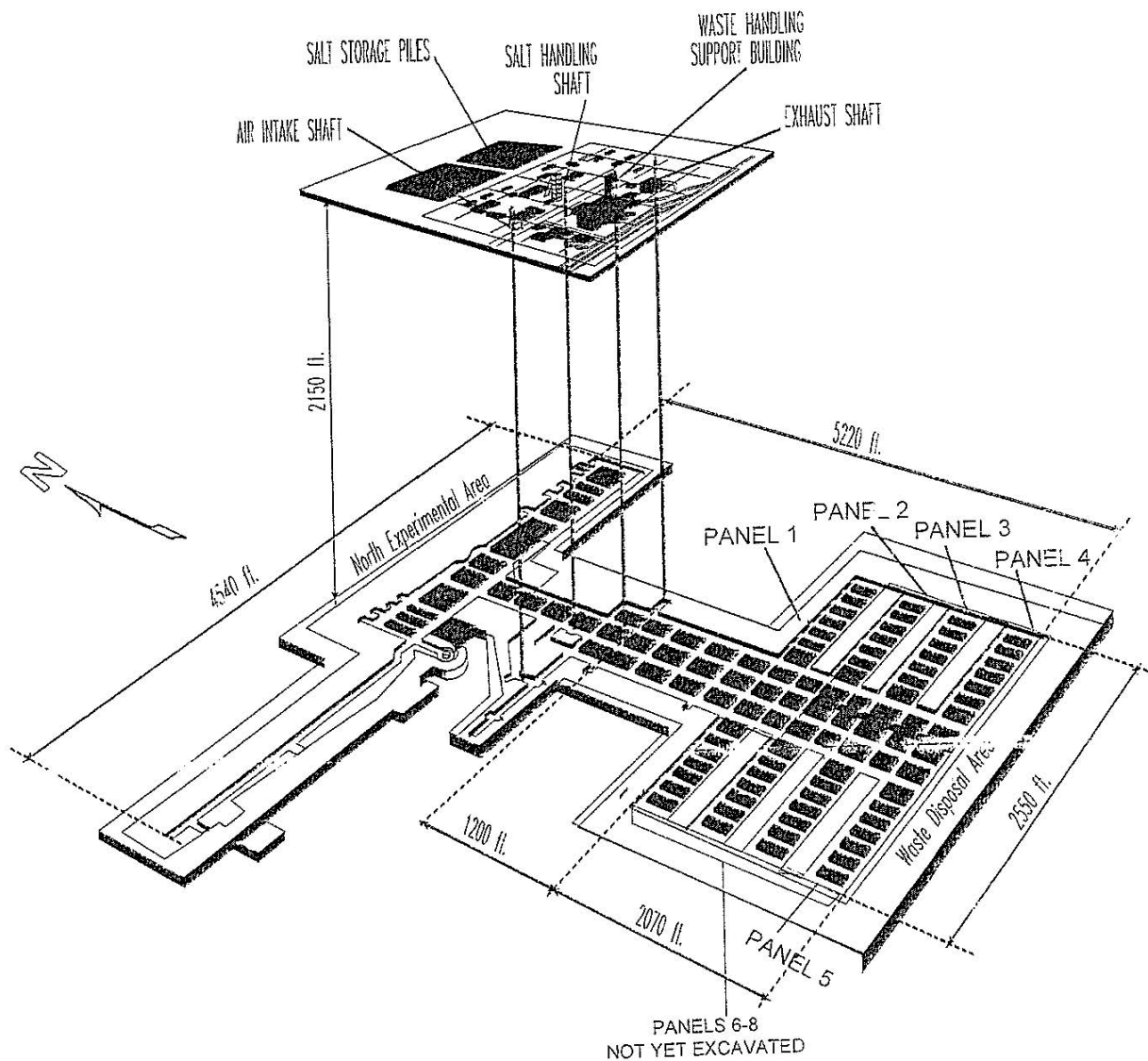
Figure I2-1 View of the WIPP underground facility
