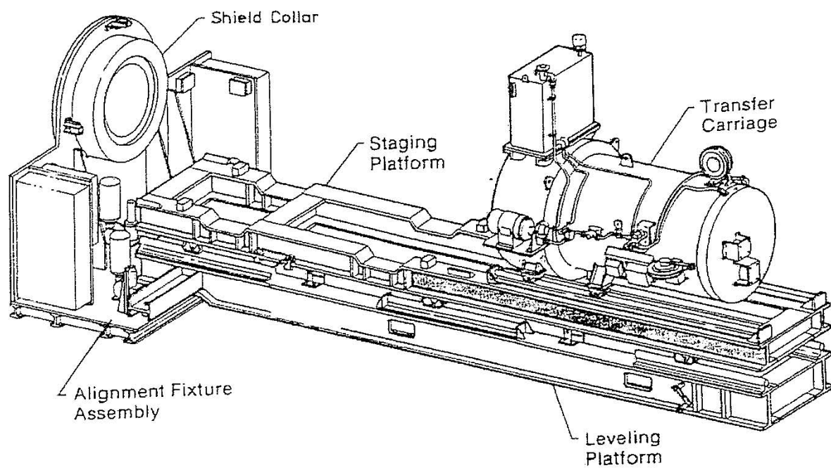
Figure M2-15 Horizontal Emplacement and Retrieval Equipment
