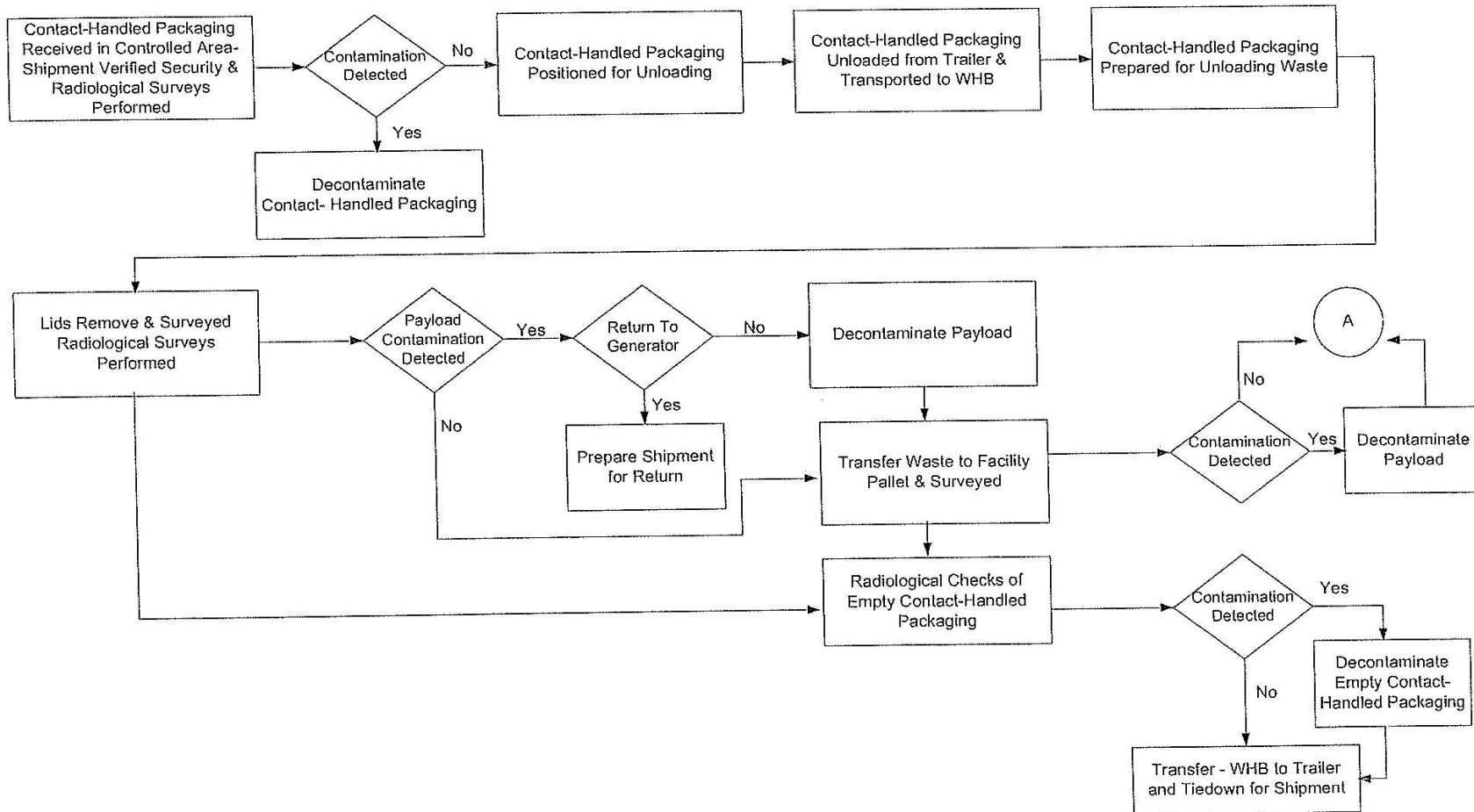
Figure M2-12 WIPP Facility Surface and Underground CH Transuranic Mixed Waste Process Flow Diagram
