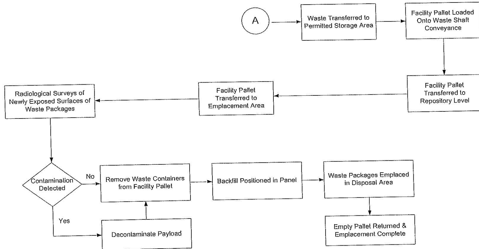
Figure M2-12 WIPP Facility Surface and Underground CH Transuranic Mixed Waste Process Flow Diagram (Continued)
