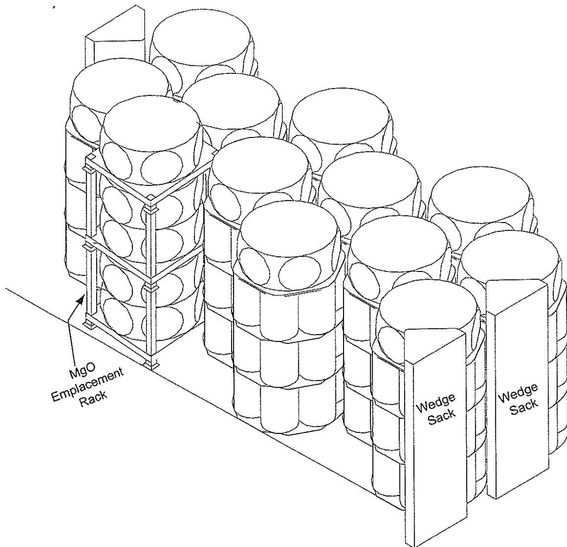
Figure M2-5a Potential MgO Emplacement Configurations
