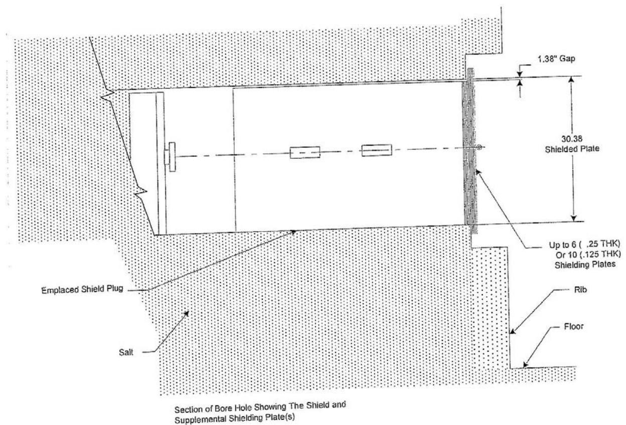
Figure M2-19 Shield Plug Supplemental Shielding Plate(s)
