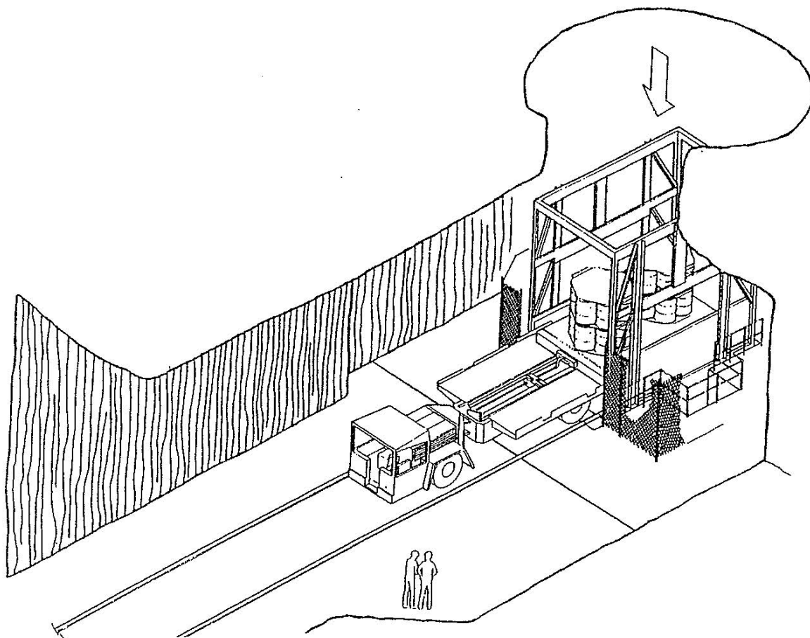
Figure M2-6 Waste Transfer Cage to Transporter
