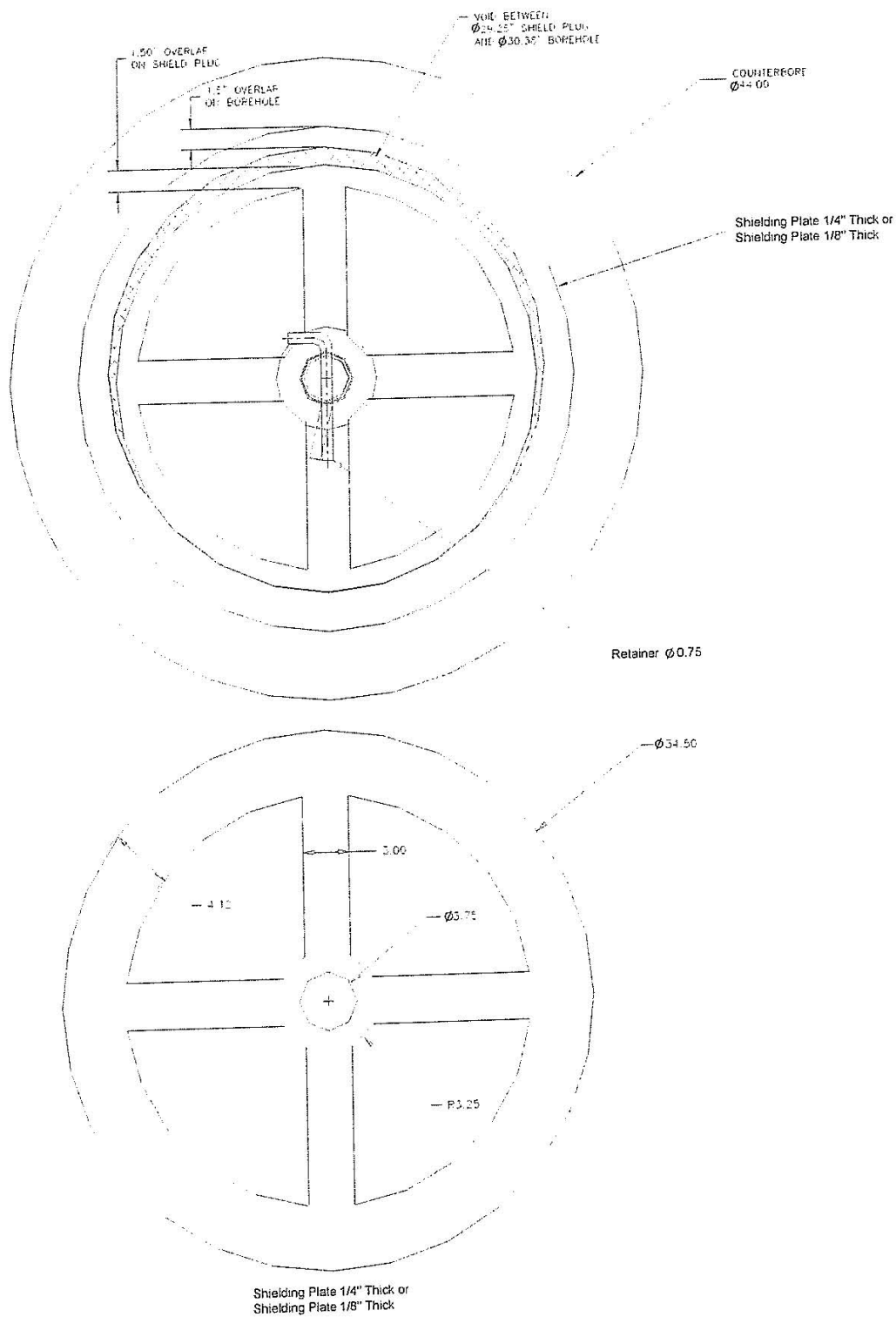
Figure M2-20 Shielding Layers to Supplement RH Borehole Shield Plugs
