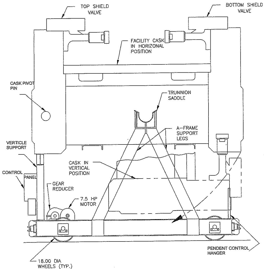
Figure M2-14 Facility Cask Transfer Car (Side View)
