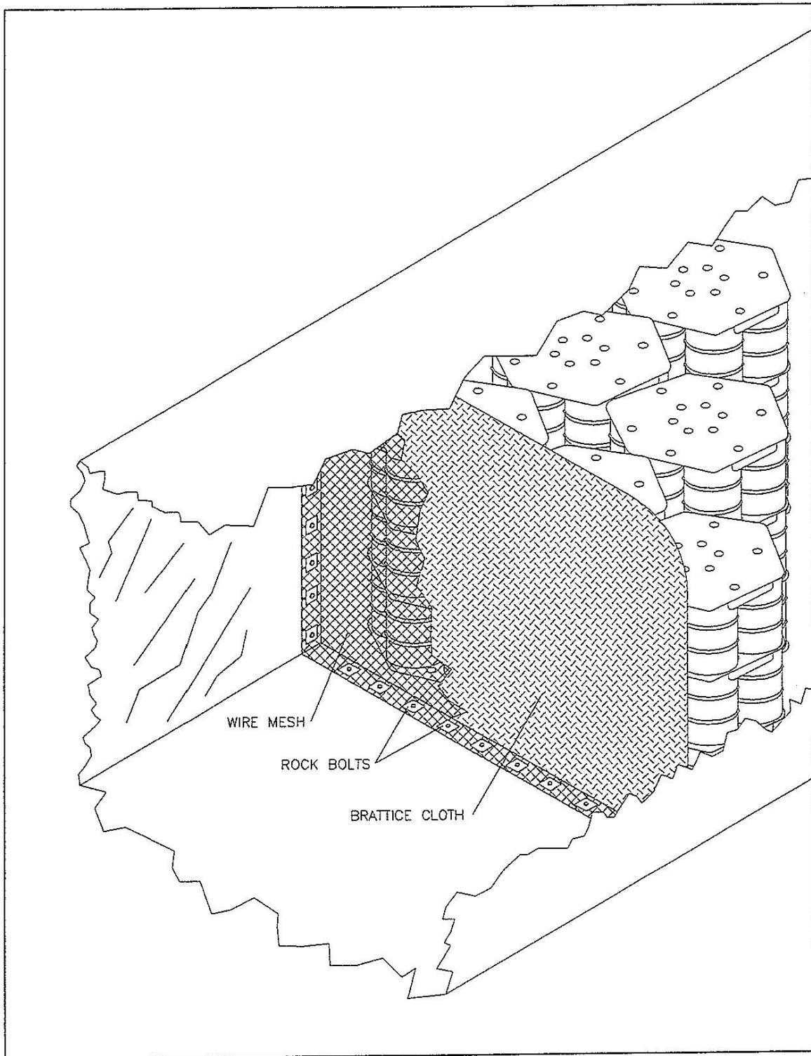
Figure M2-11 Typical Room Barricade
