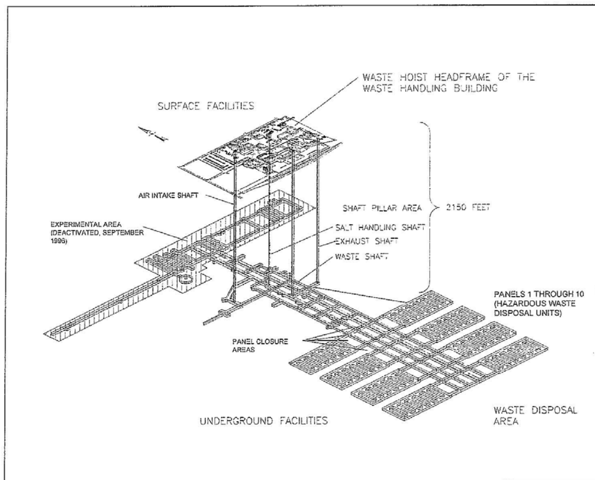
Figure M2-2 Spatial View of the Miscellaneous Unit and Waste Handling Facility
