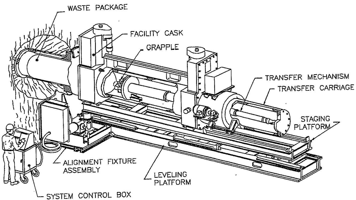
Figure M2-17 Facility Cask Installed on the Horizontal Emplacement and Retrieval Equipment
