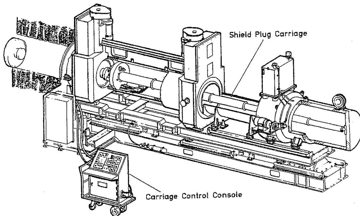
Figure M2-18 Installing Shield Plug
