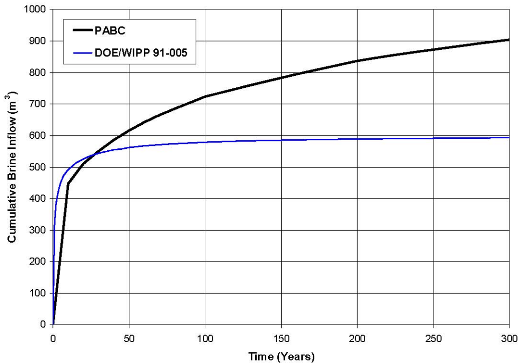
4 5 Figure 3. Predicted Cumulative Brine Inflow into a Closed Waste Panel for the PABC and 6 Original Performance Demonstrations
