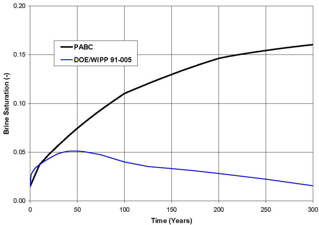
4 5 Figure 5. Predicted Average Brine Saturation in the Panel for the PABC 6 and Original Performance Demonstrations
