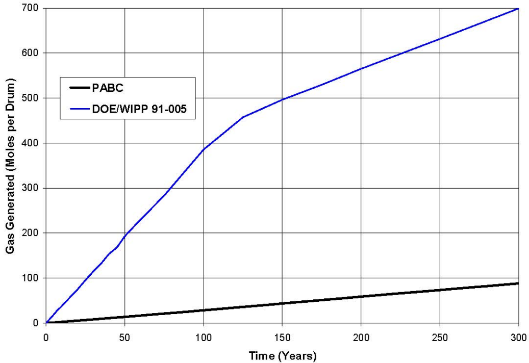
1 2 Figure 2. Predicted Cumulative Moles of Gas Generated Per Drum of Waste for the PABC 3 and Original Performance Demonstrations
