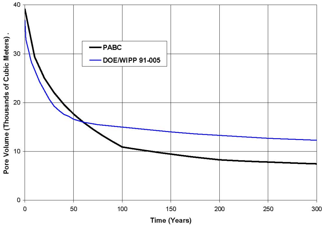
1 2 Figure 4. Predicted Change in Panel Pore Volume Due to Creep Closure for the PABC and 3 Original Performance Demonstrations
