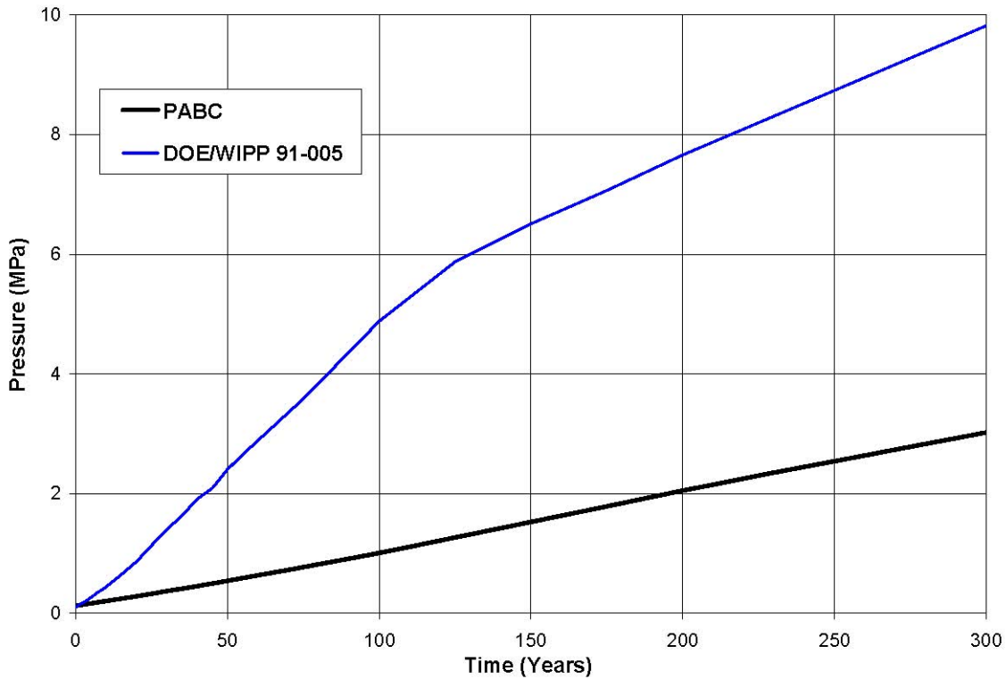
13 14 Figure 1. Predicted Change in Repository Pressure Following Closure for the 15 PABC and Original Performance Demonstrations
